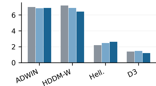
RADAR - resets / 100k rows
