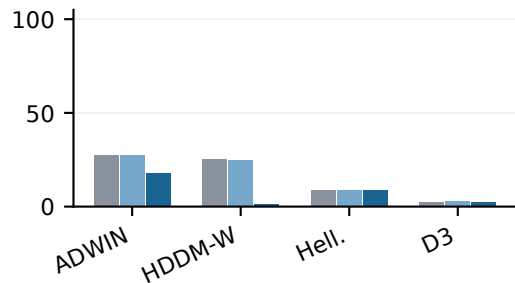
SEA - alarm blocks (%)
