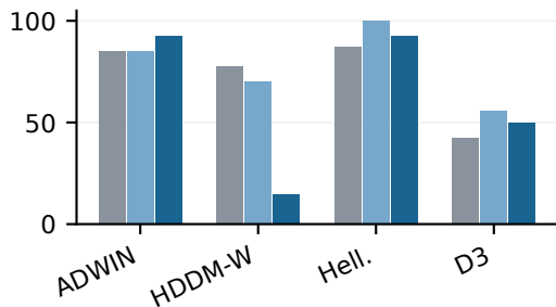
SEA - event recall (%)
