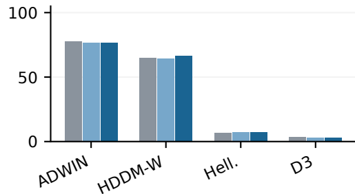
RADAR - alarm blocks (%)
