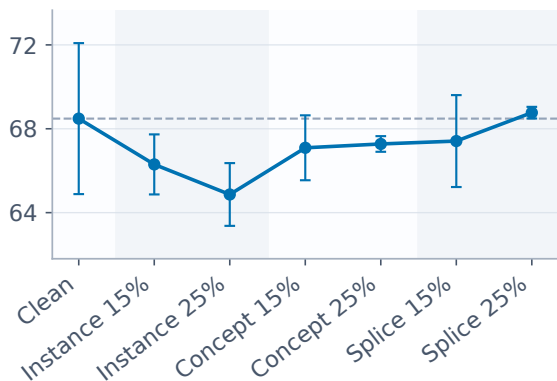
Macro recall (%)
