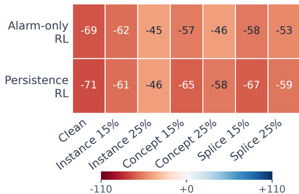
ROC-AUC change ( \times 10^{-3} )
