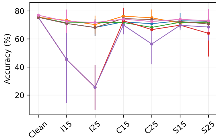
radar - adwin - confirmed reset with screening
