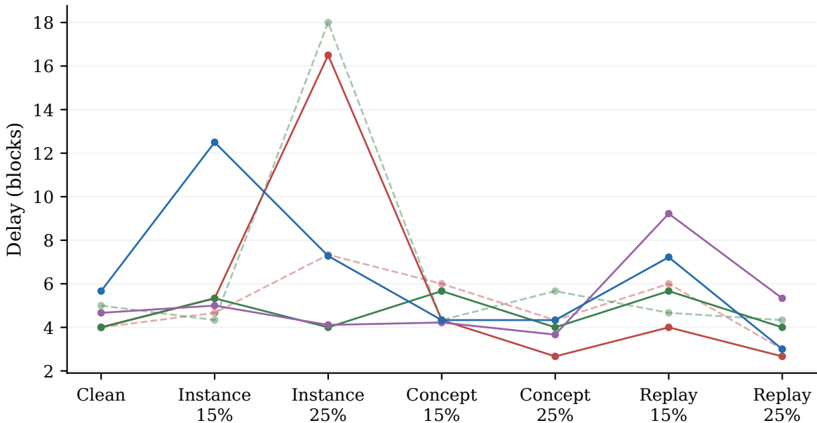
RBF, ADWIN: Detection delay
