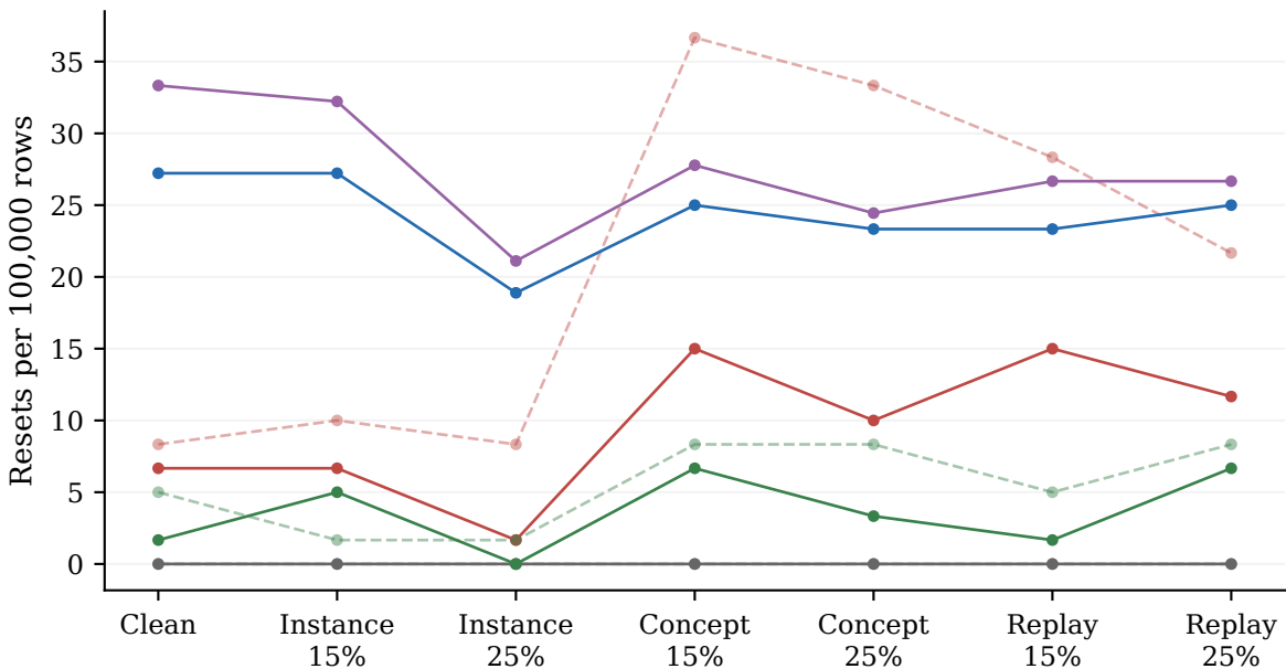
RBF, ADWIN: Reset frequency
