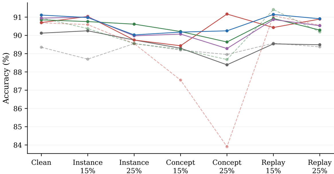
SEA, ADWIN: Host accuracy
