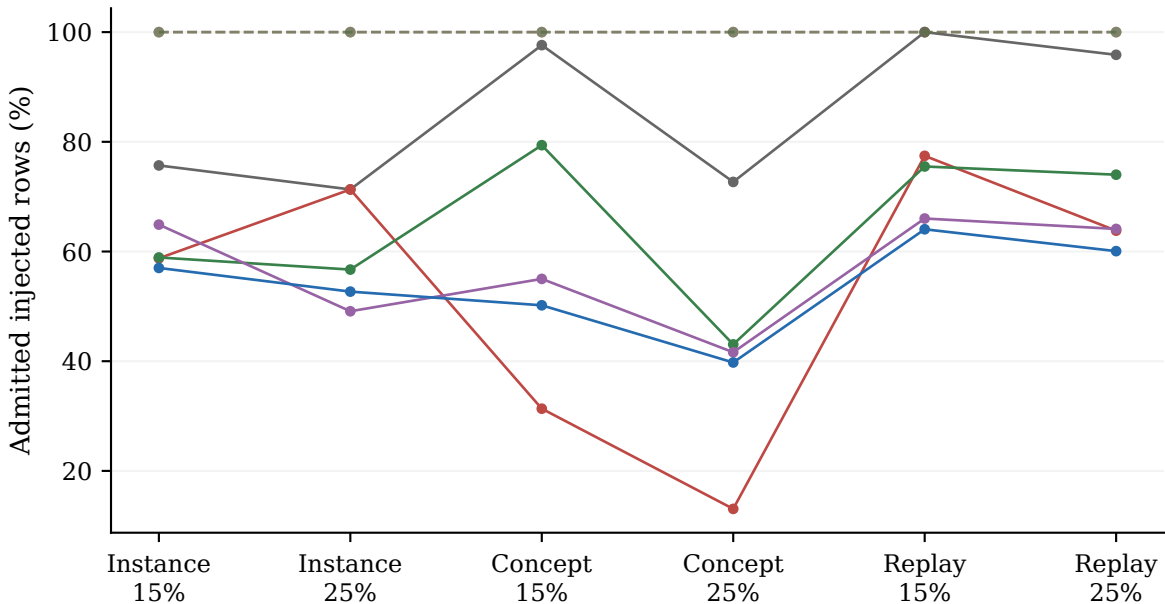
SEA, ADWIN: Poison admission
