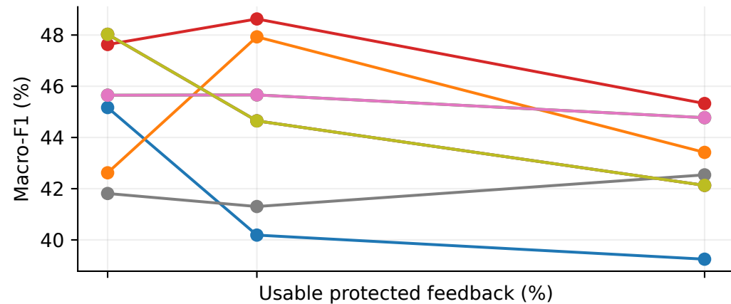
Hellinger
