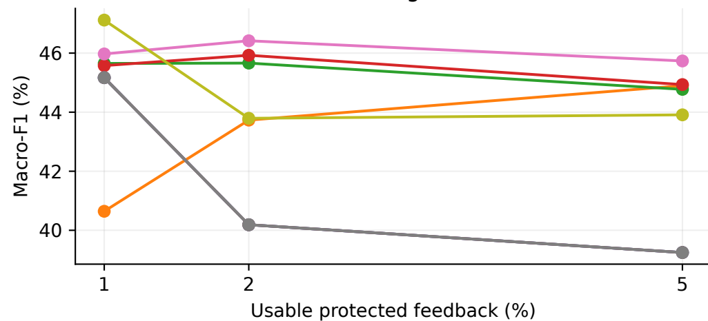
Hellinger
