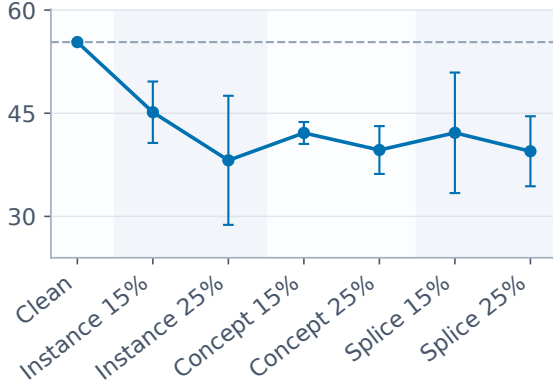
Macro recall (%)
