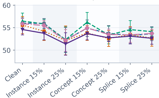
Poison admission (%)
