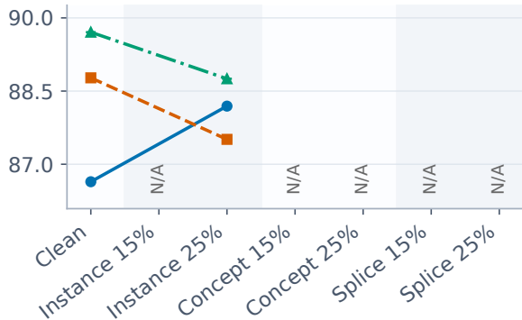
Accuracy (%)
