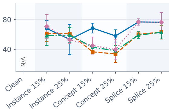
Poison admission (%)
