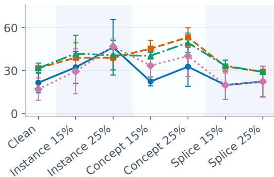
Legitimate withholding (%)
