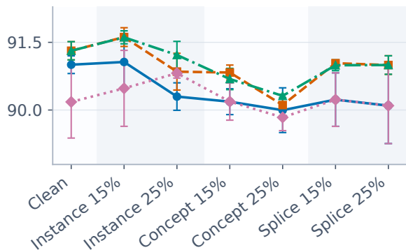
Accuracy (%)
