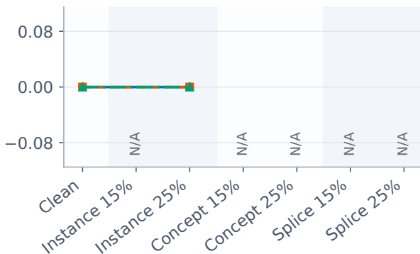
Macro-F1 (%) difference
