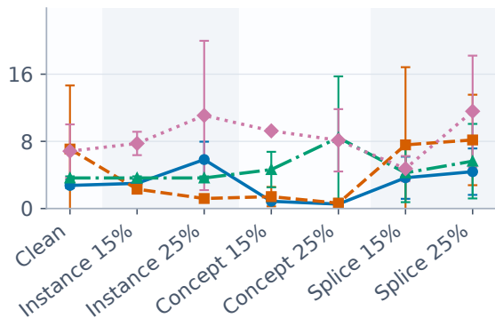
Detection delay (blocks)
