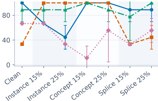
Drift-event recall (%)
