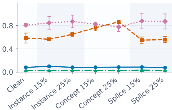
Monitor time (s / 100k rows)
