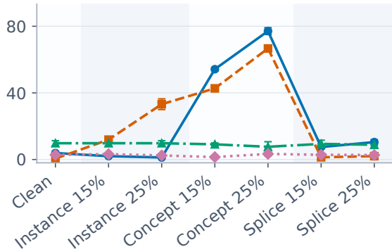
Alarm blocks (%)
