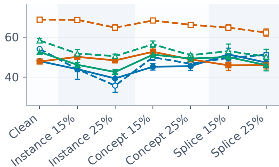
Macro recall (%)
