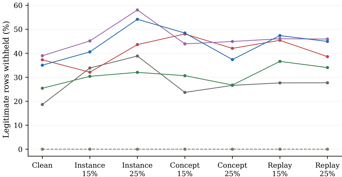
RBF, ADWIN: Legitimate withholding
