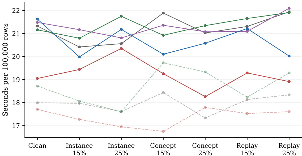
RBF, ADWIN: Execution time
