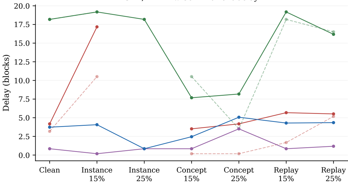
SEA, ADWIN: Commitment delay
