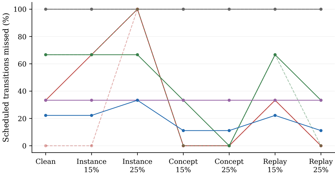
SEA, ADWIN: Missed commitments
