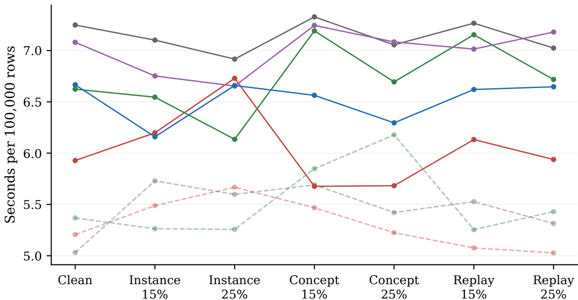
SEA, ADWIN: Execution time
