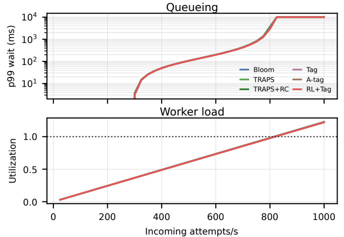
Fig. 6: Method-specific bounded-worker queueing with measured Argon2 service time and an 8% valid-attempt mix.
