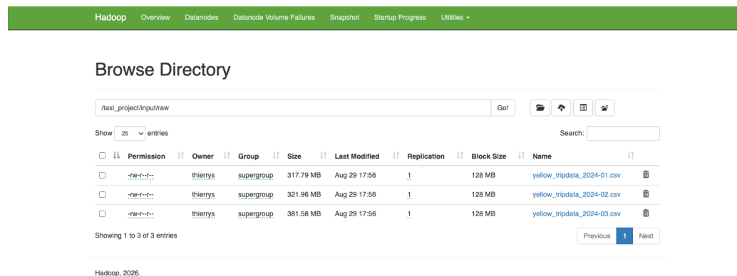
Screenshot 4 — the dataset in HDFS, with block information. The three uploaded CSV files with size, replication factor and block size — the visual counterpart to hdfs fsck , which reported 9 blocks averaging 118.99 MB.
