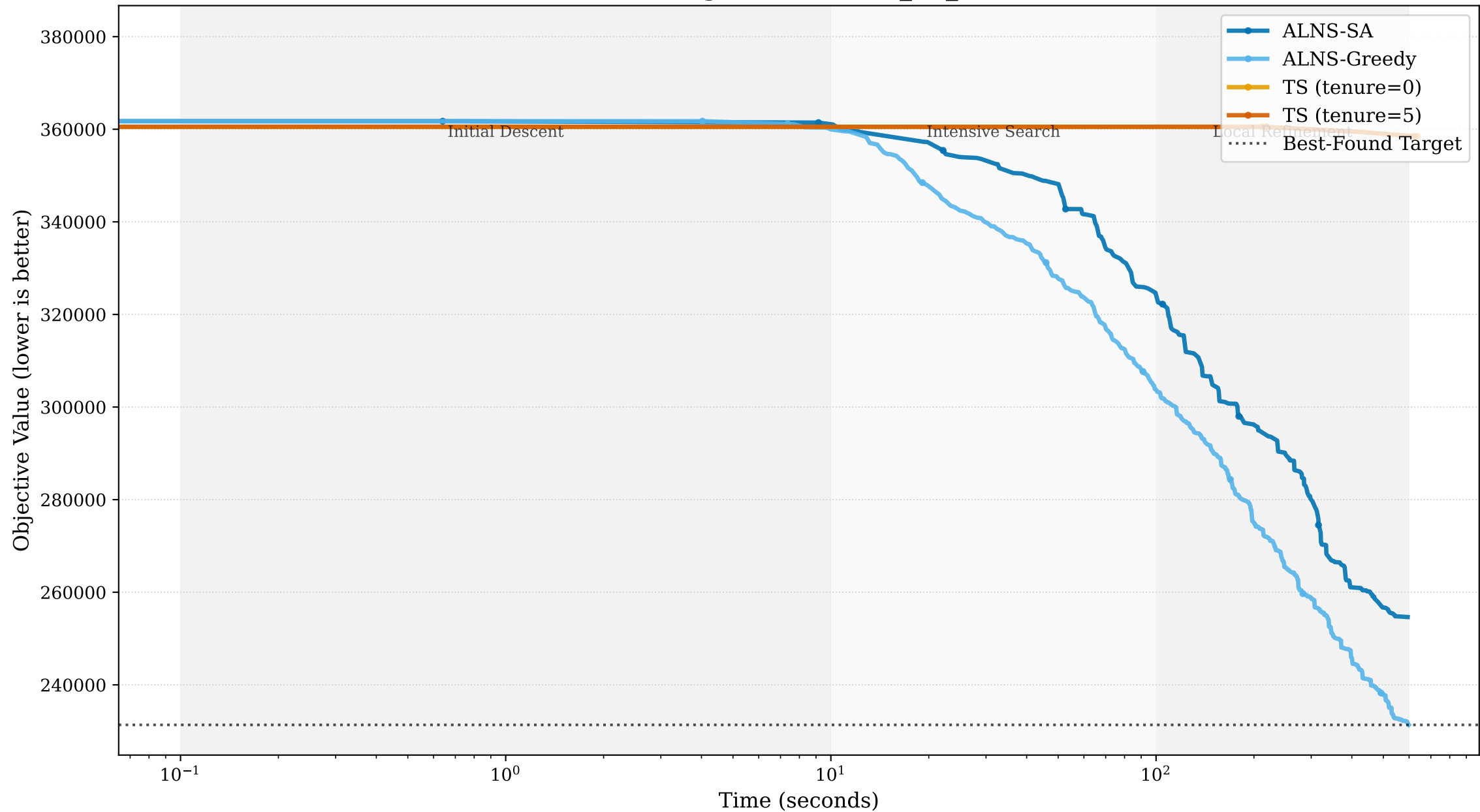
Convergence Plot: C1_10_10
