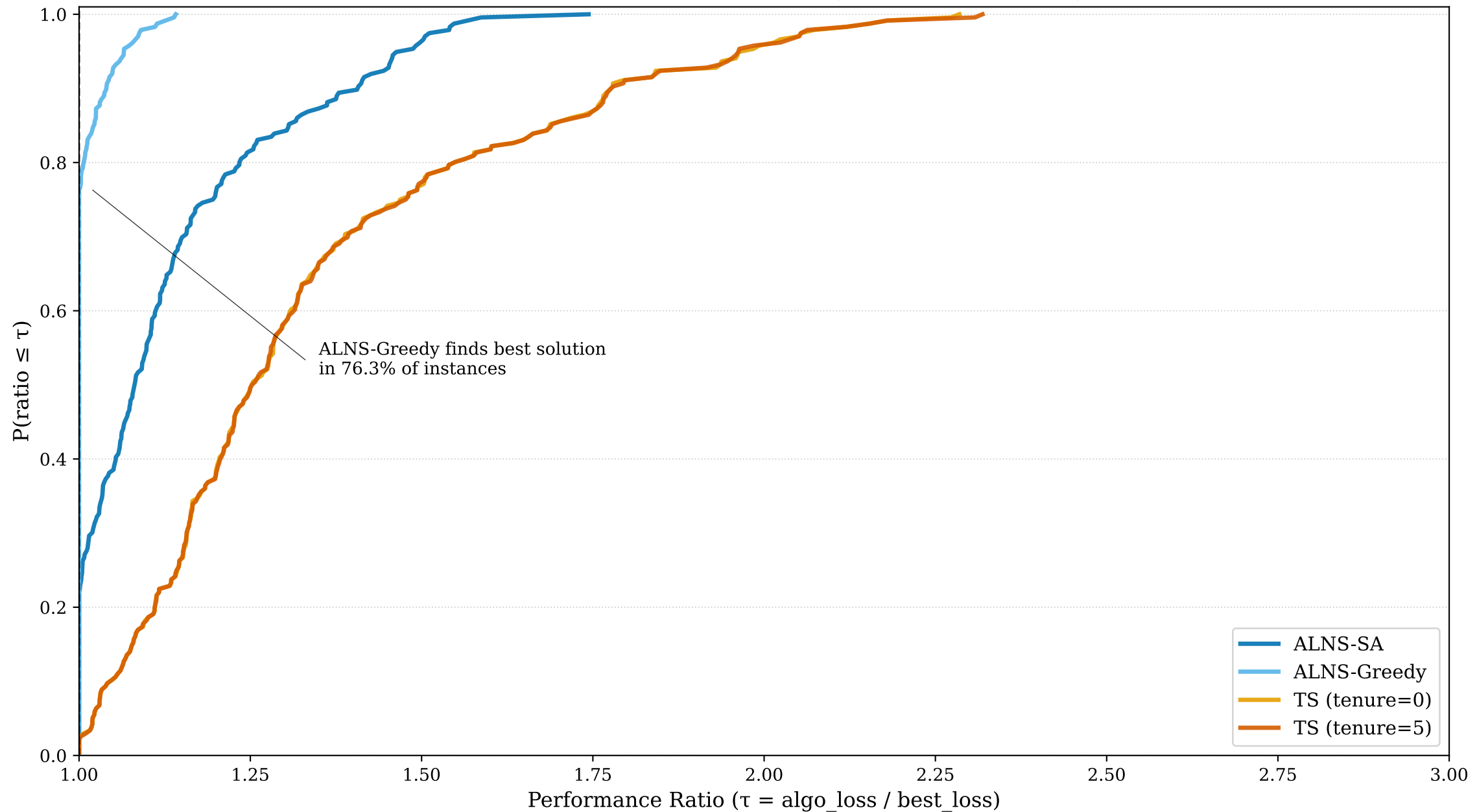
Overall Performance Profile (All 236 Instances)
