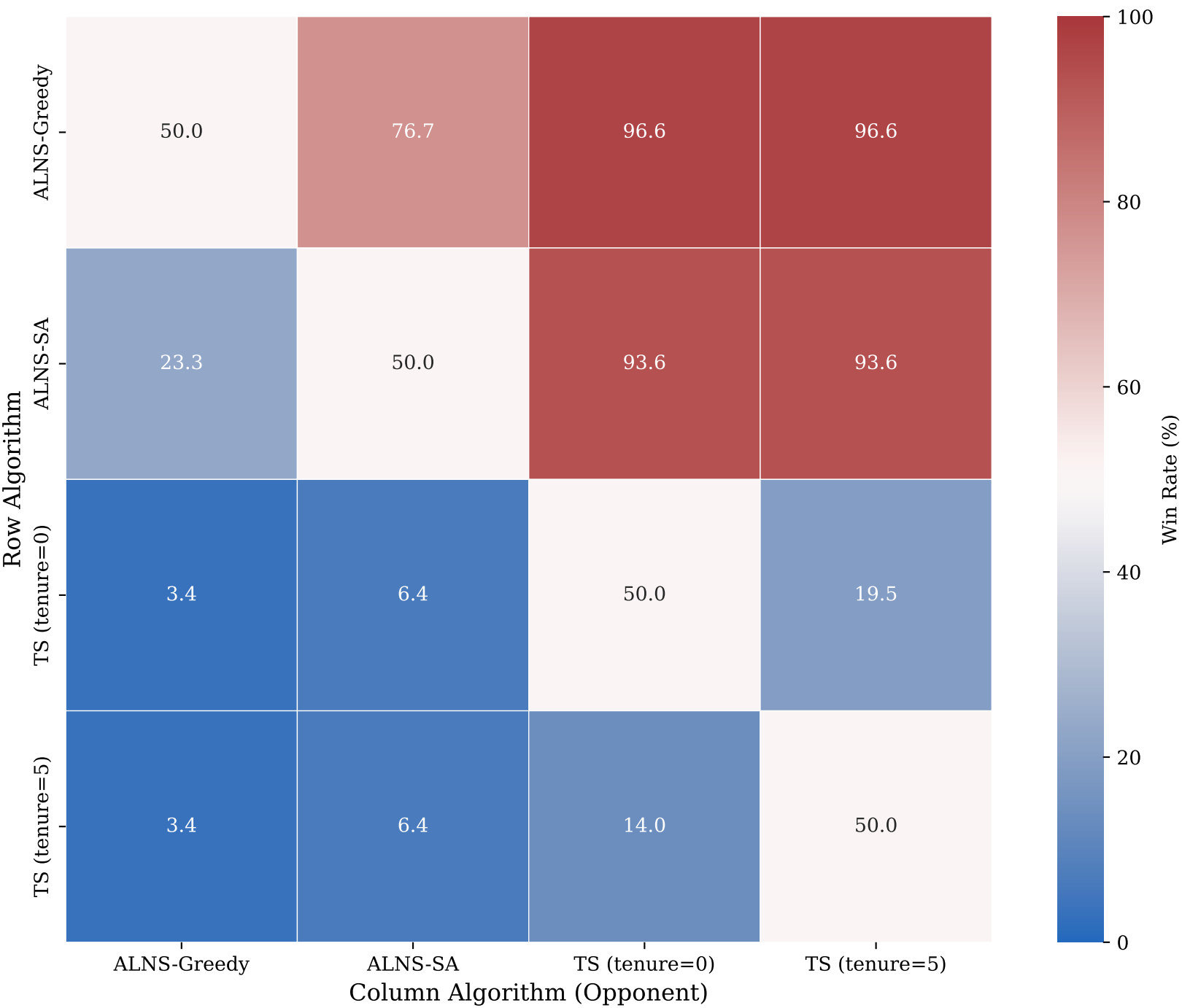
Pairwise Dominance Heatmap (% Wins) Row Algorithm beats Column Algorithm
