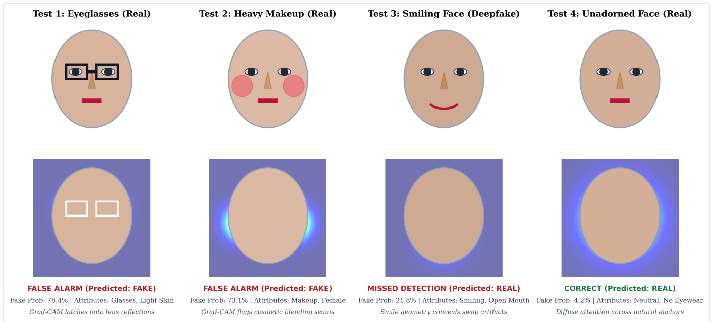
Fig. 6. Qualitative Test Scenarios and Explainable Grad-CAM Forensic Heatmaps - Experimental evaluations of the FairFake framework on genuine and manipulated faces. Test 1: Real face with eyeglasses falsely flagged as manipulated ( p_{\text{fake}} = 78.4\% ) due to rim reflection gradients. Test 2: Real face with heavy makeup misclassified ( p_{\text{fake}} = 73.1\% ) due to cosmetic powder blending edges. Test 3: Manipulated deepfake evading detection ( p_{\text{fake}} = 21.8\% ) because smiling geometry masks forgery seams. Test 4: Genuine unadorned face correctly verified ( p_{\text{fake}} = 4.2\% ) with diffuse attention across anatomical facial anchors.
