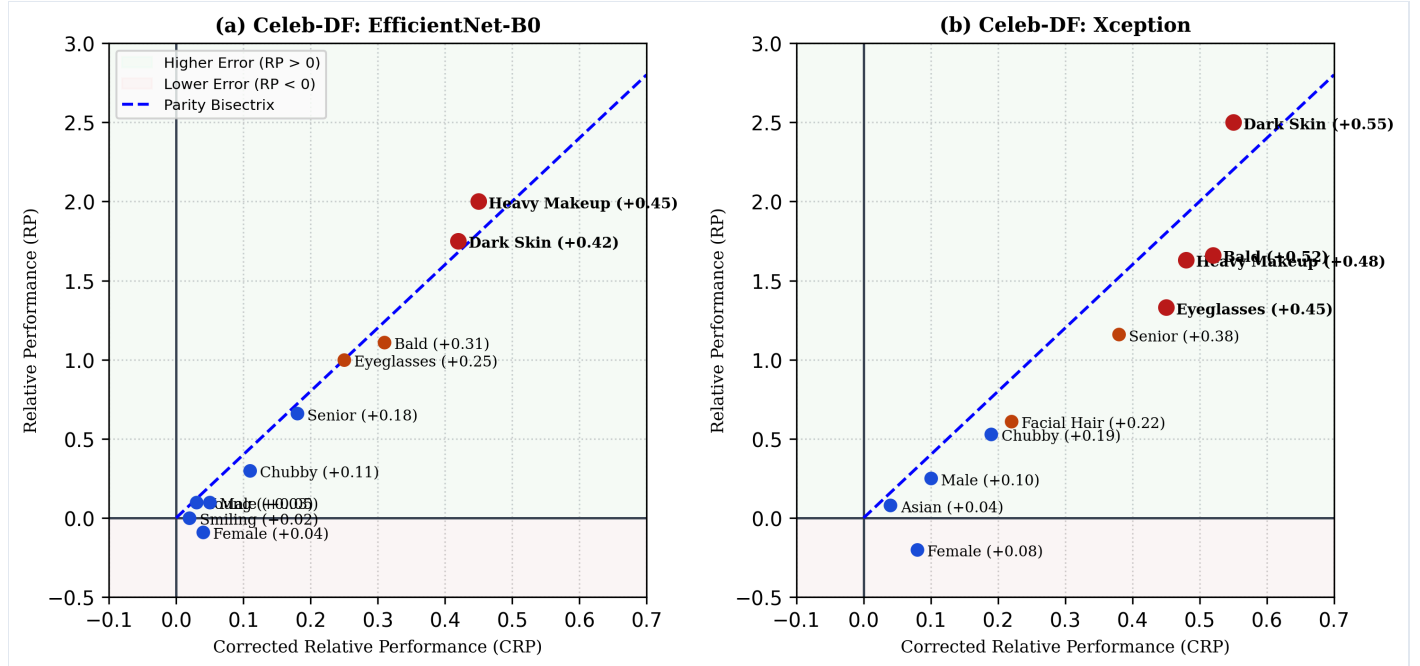
Fig. 3. Bias analysis - The relative performance RP is reported with respect to the corrected relative performance CRP using EfficientNet-B0 and Xception. The blue dashed line indicates parity bisectrix. Attributes falling in the upper quadrant indicate substantially higher error rates when the attribute is present.
