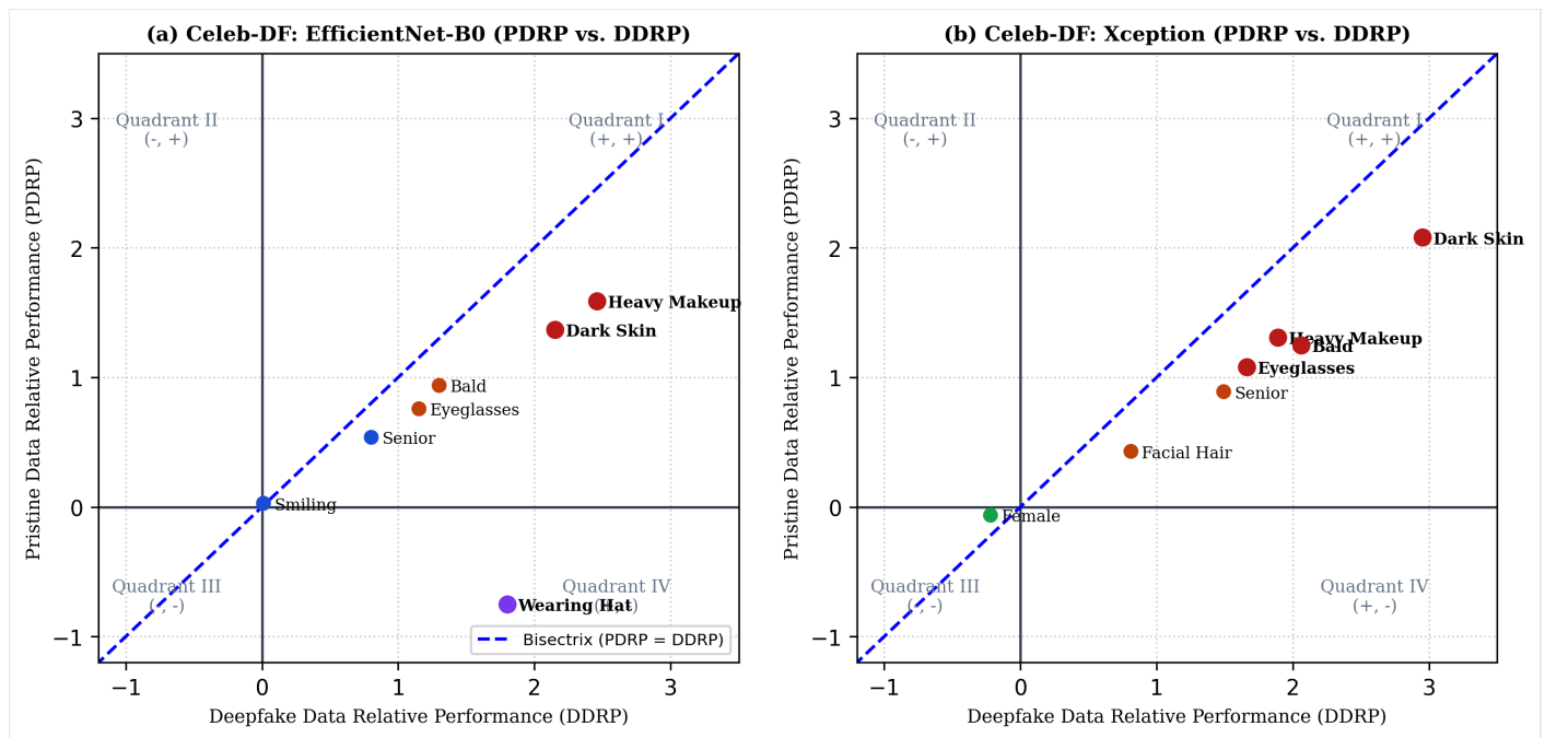
Fig. 4. Bias analysis on Pristine Data and Deepfake Data - The CRP on pristine data (PDRP) is reported with respect to the CRP on Deepfake data (DDRP). Attributes in Quadrant I with DDRP > PDRP (below the bisectrix line) allow fake media to evade detection at severe rates, creating security vulnerabilities.
