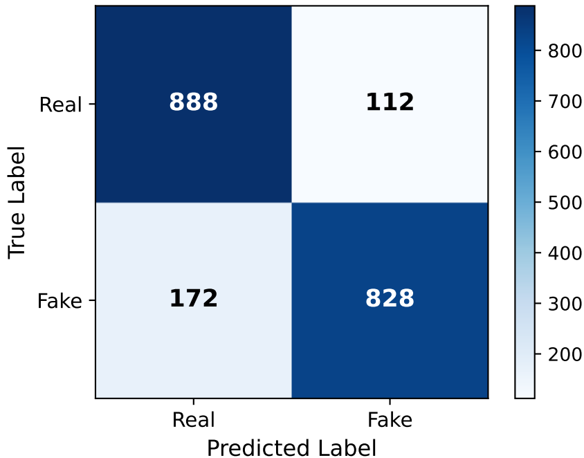
Test 1: Baseline Confusion Matrix (N=2,000)
