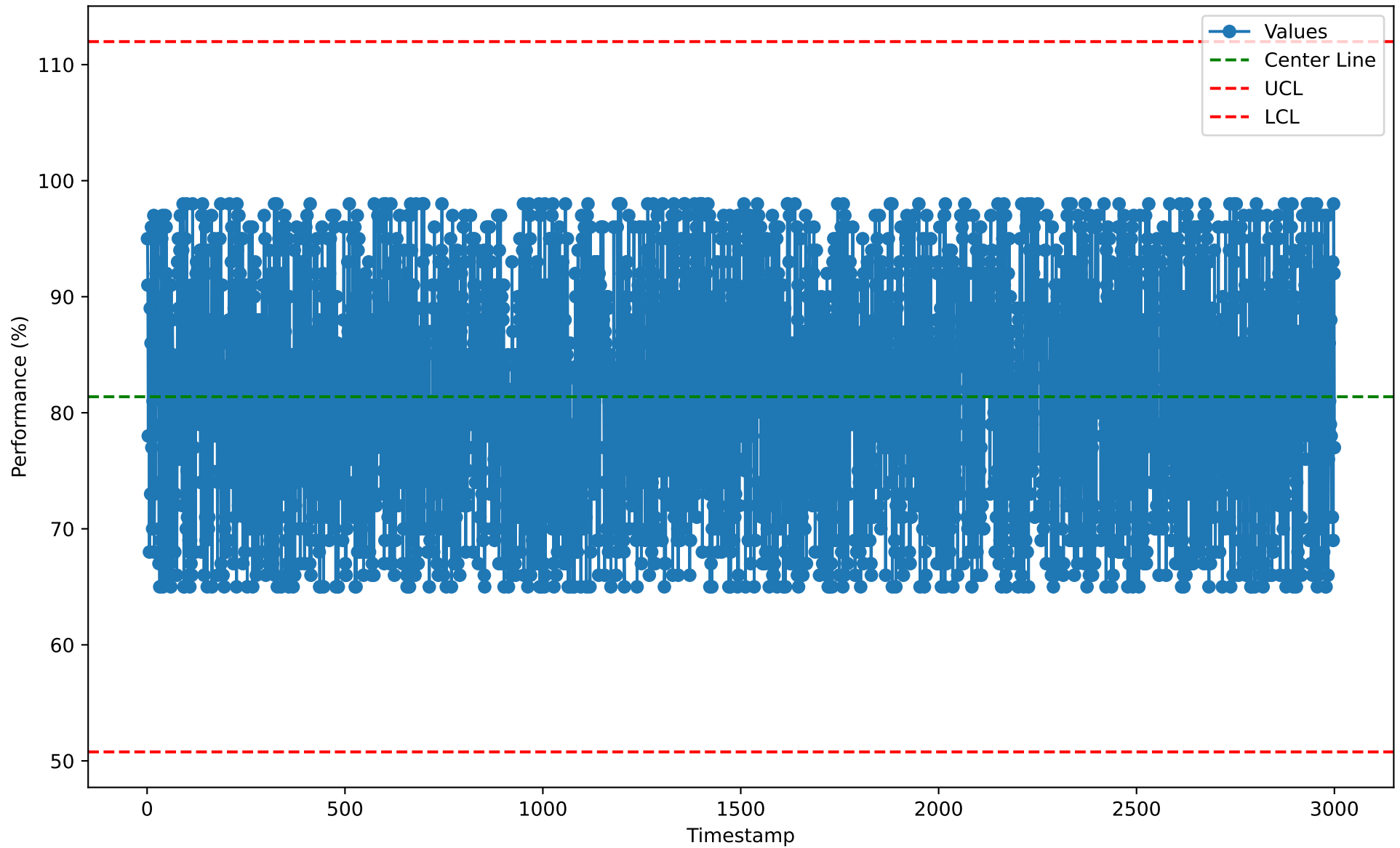
Individuals Chart for DAM10102 (2026-01-07)
