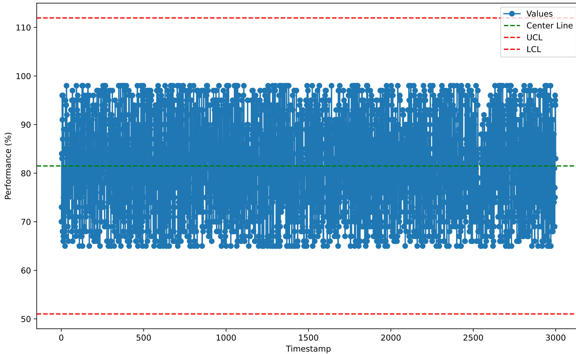
Individuals Chart for BTP10102 (2026-01-07)
