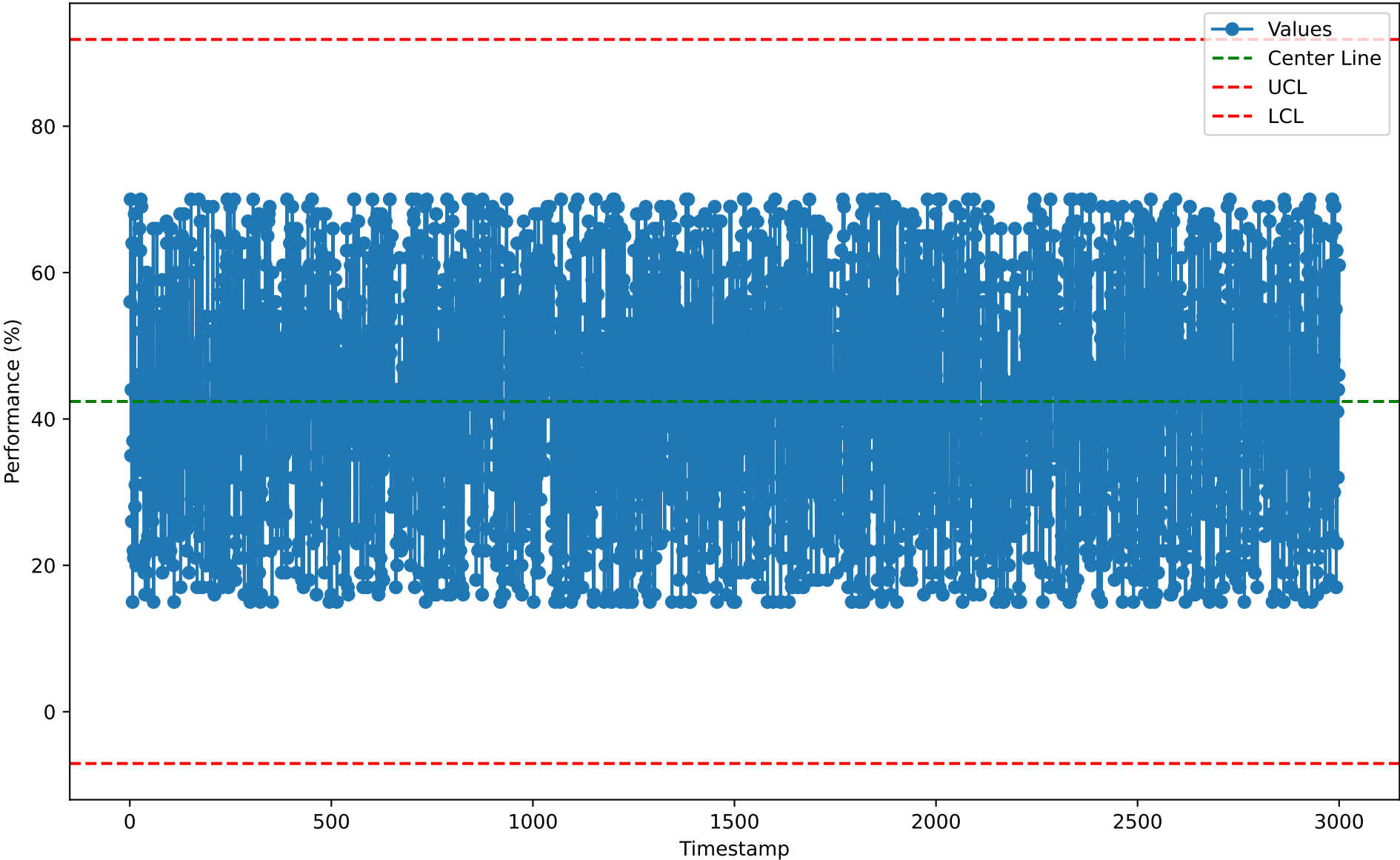
Individuals Chart for EPR10110 (2026-01-07)
