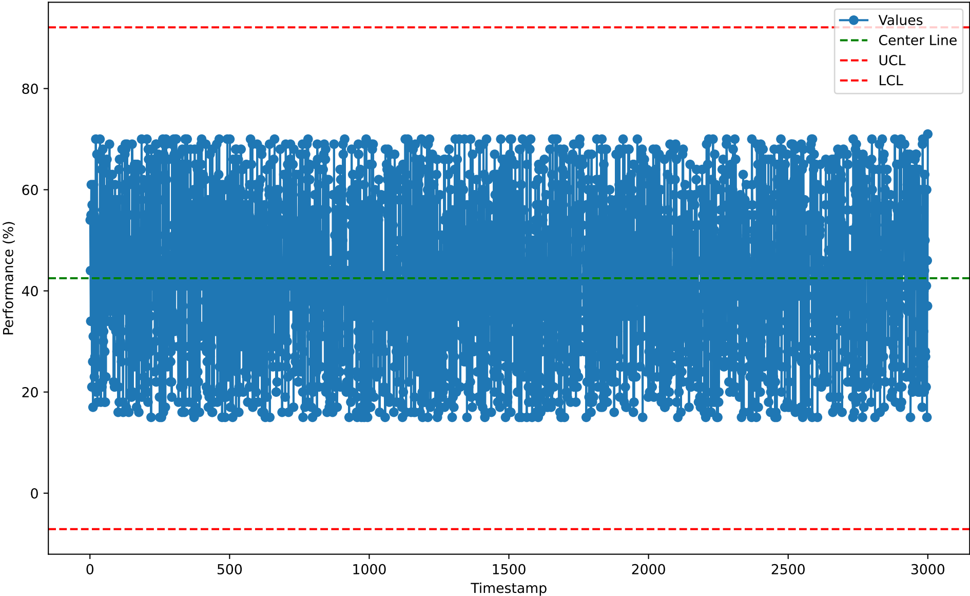
Individuals Chart for EKW10123 (2026-01-07)
