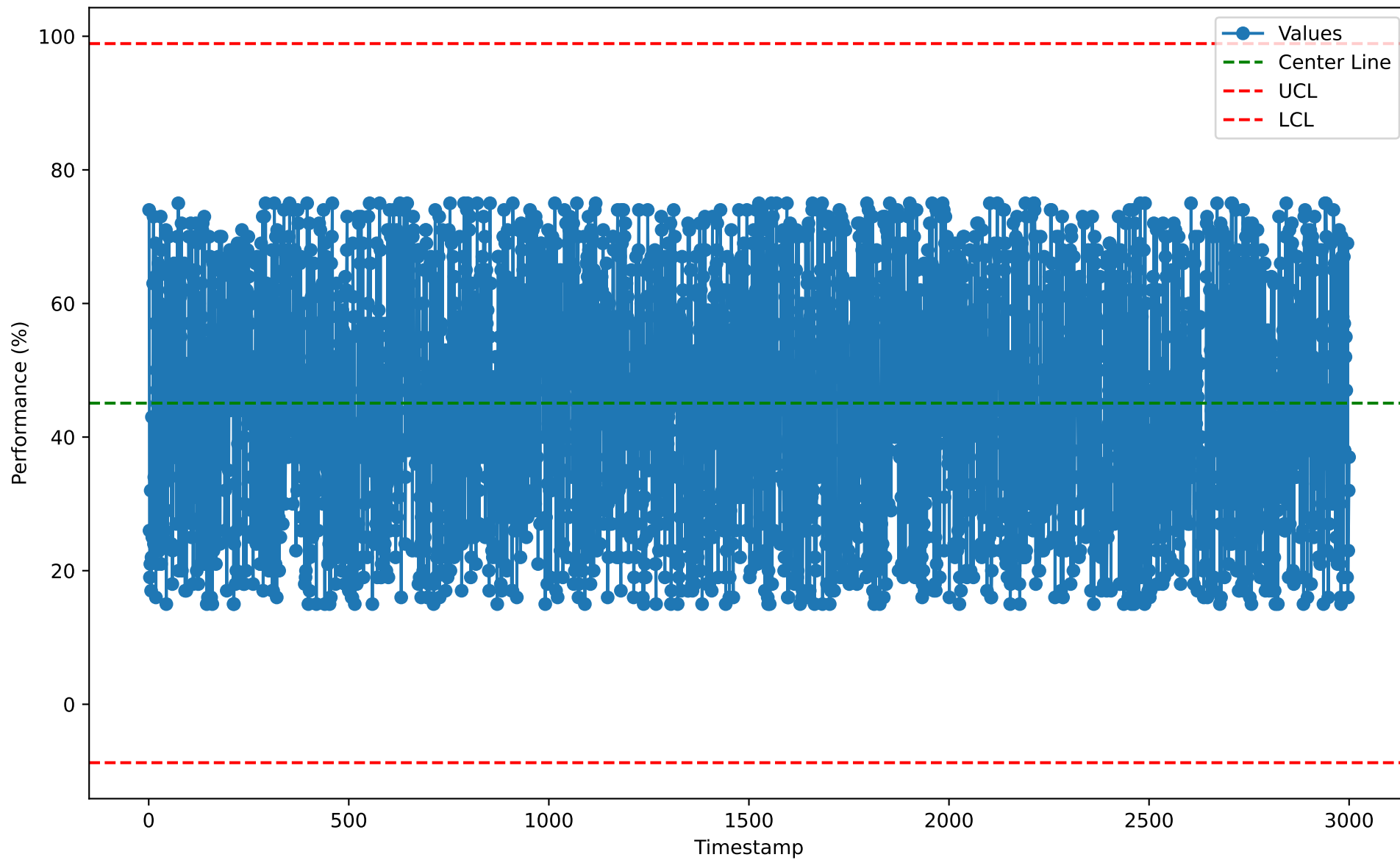
Individuals Chart for ECF10126 (2026-01-07)
