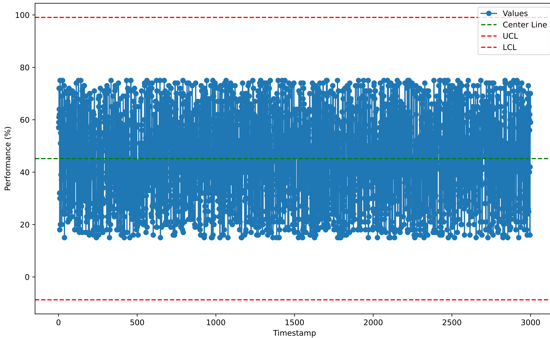
Individuals Chart for EIF10106 (2026-01-07)
