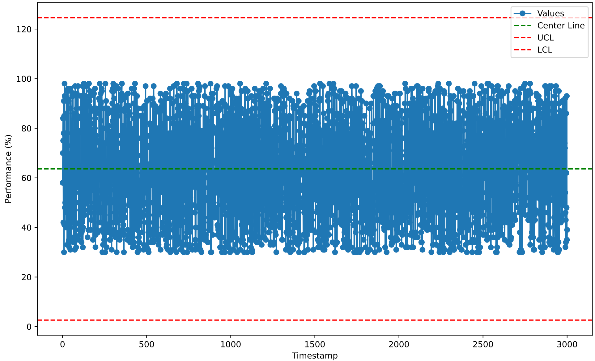
Individuals Chart for CMM10104 (2026-01-07)
