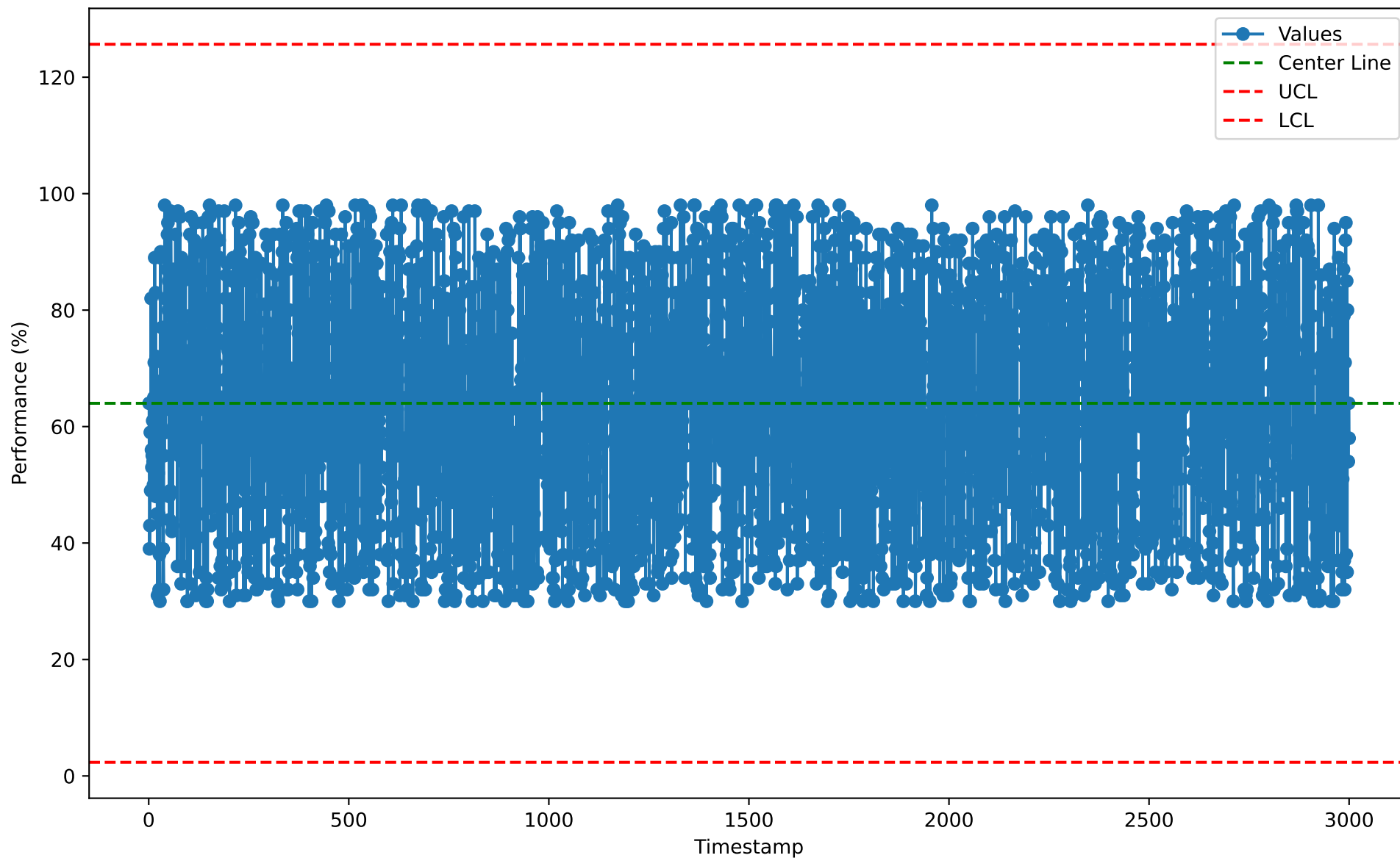
Individuals Chart for SYA10102 (2026-01-07)
