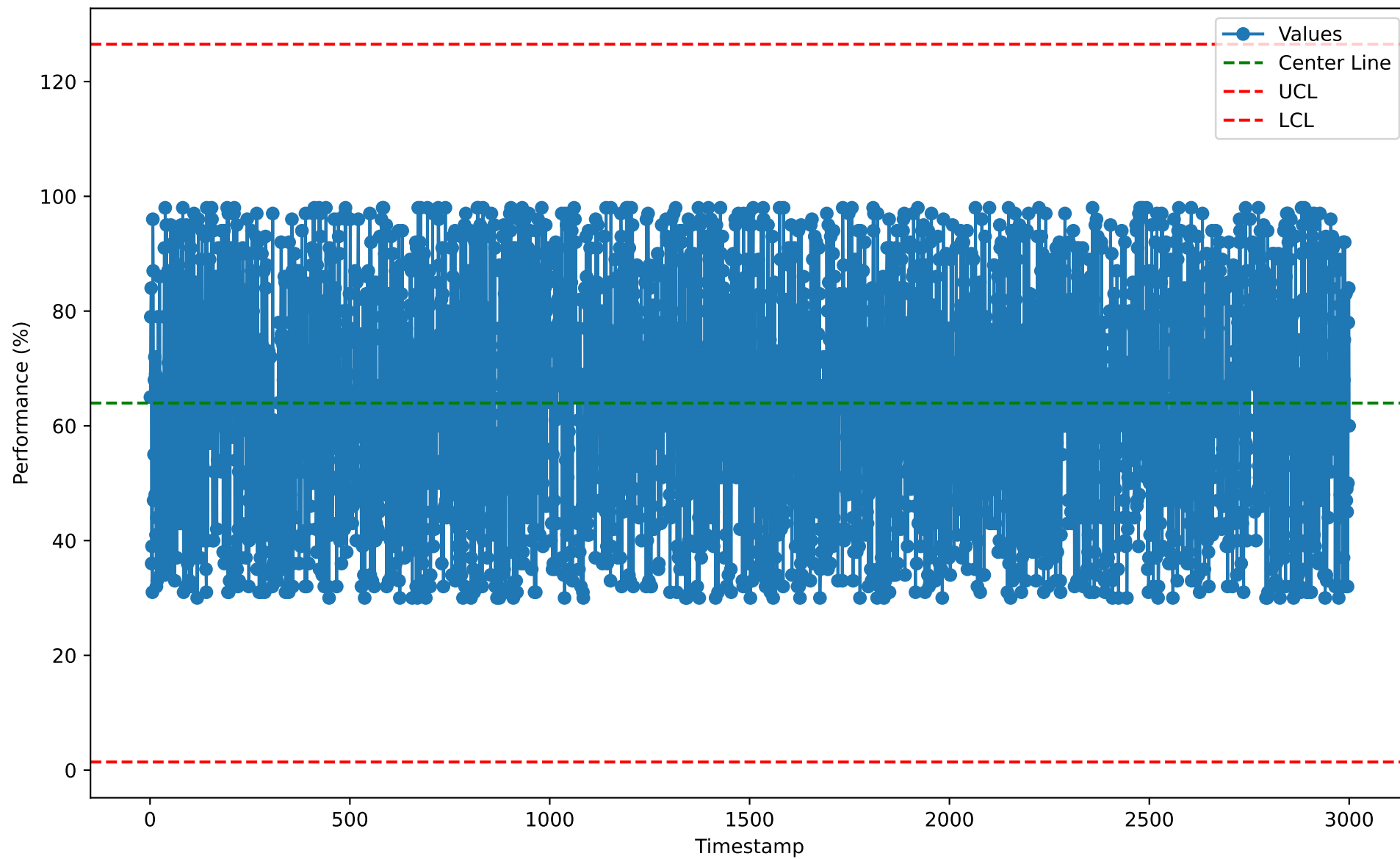
Individuals Chart for MDM10106 (2026-01-07)
