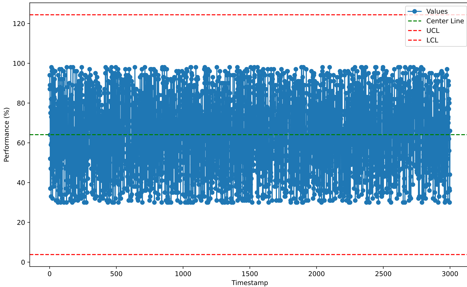
Individuals Chart for BPT10110 (2026-01-07)
