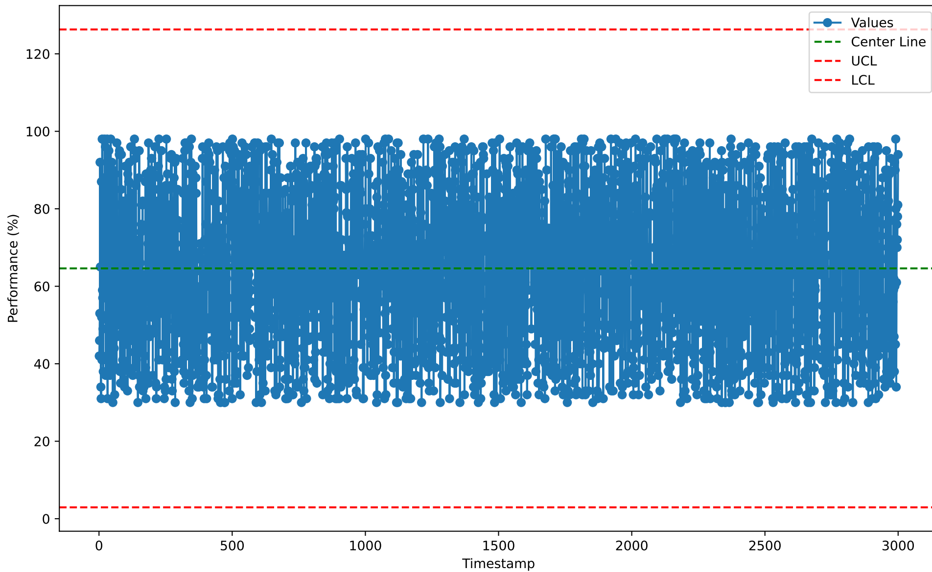
Individuals Chart for BPT10115 (2026-01-07)
