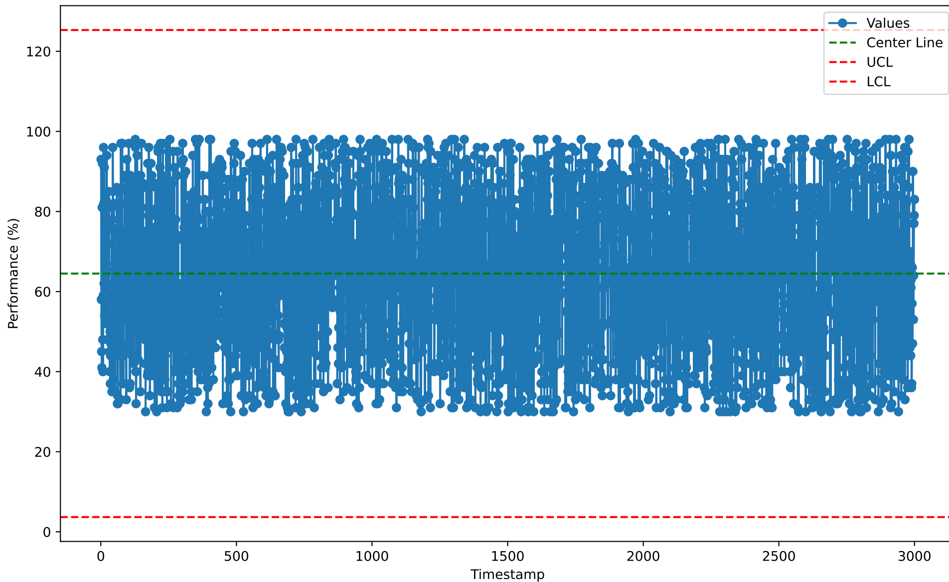
Individuals Chart for PJM10112 (2026-01-07)
