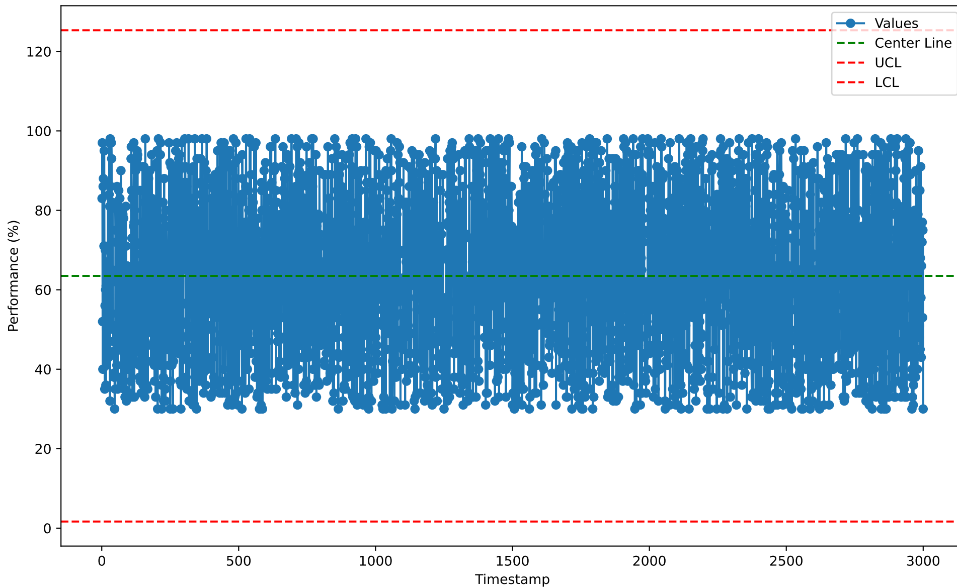
Individuals Chart for IDP10103 (2026-01-07)
