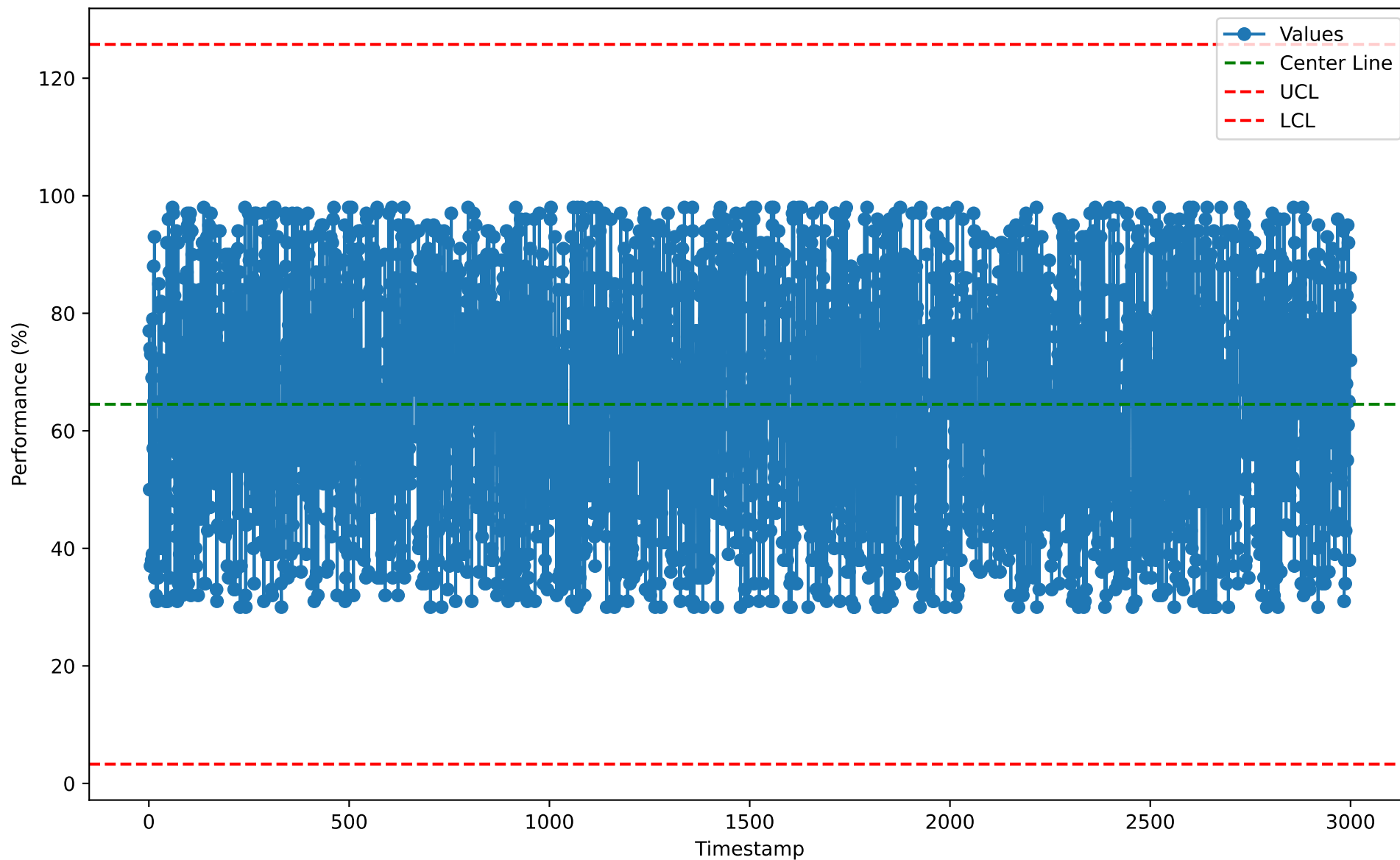
Individuals Chart for PTY10123 (2026-01-07)
