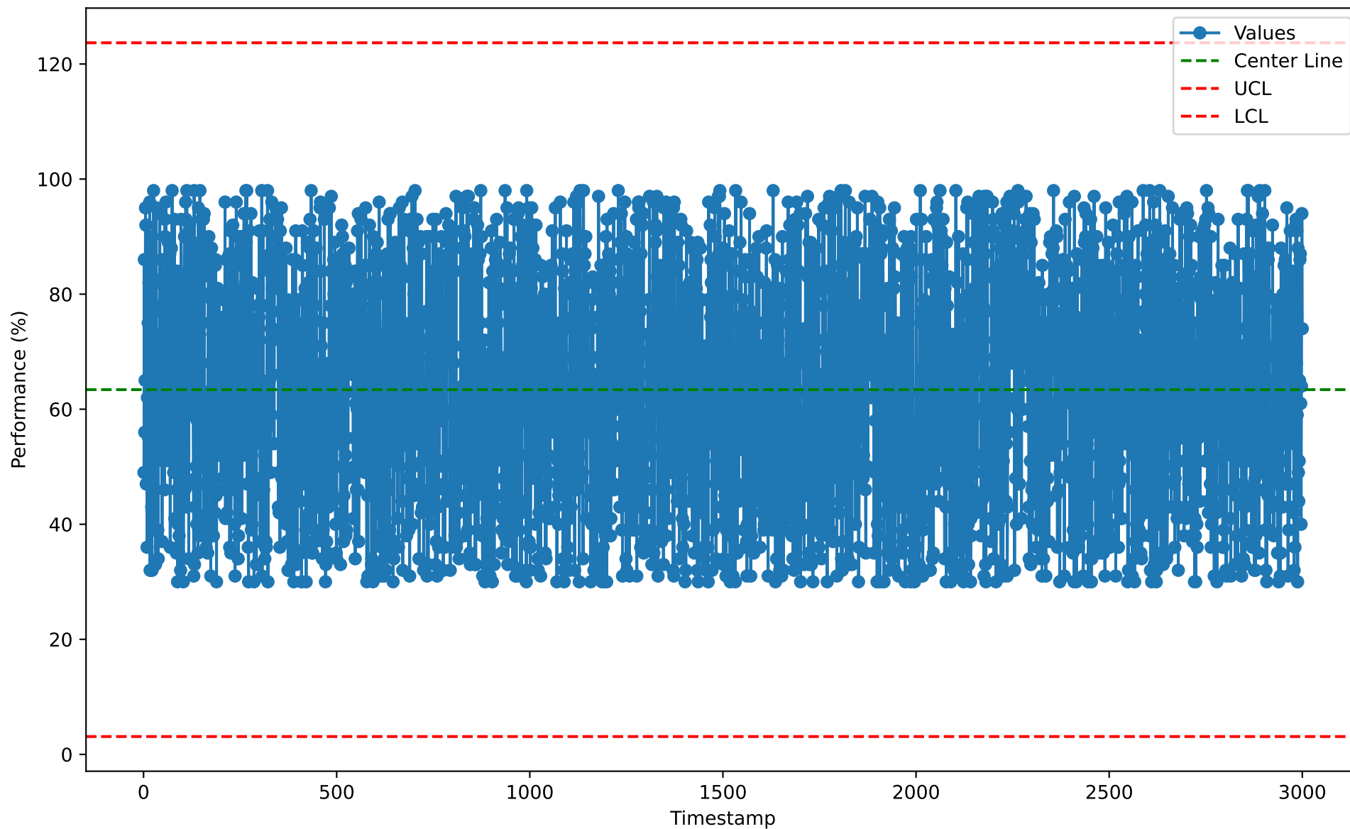
Individuals Chart for FLO10103 (2026-01-07)
