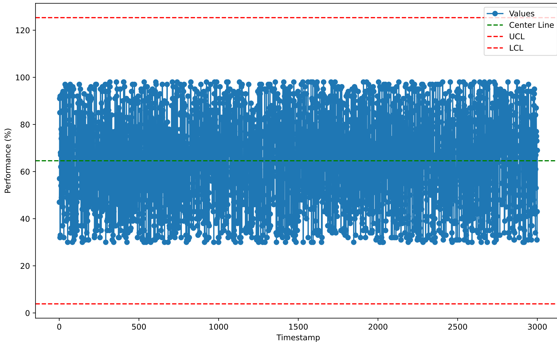
Individuals Chart for SYA10110 (2026-01-07)
