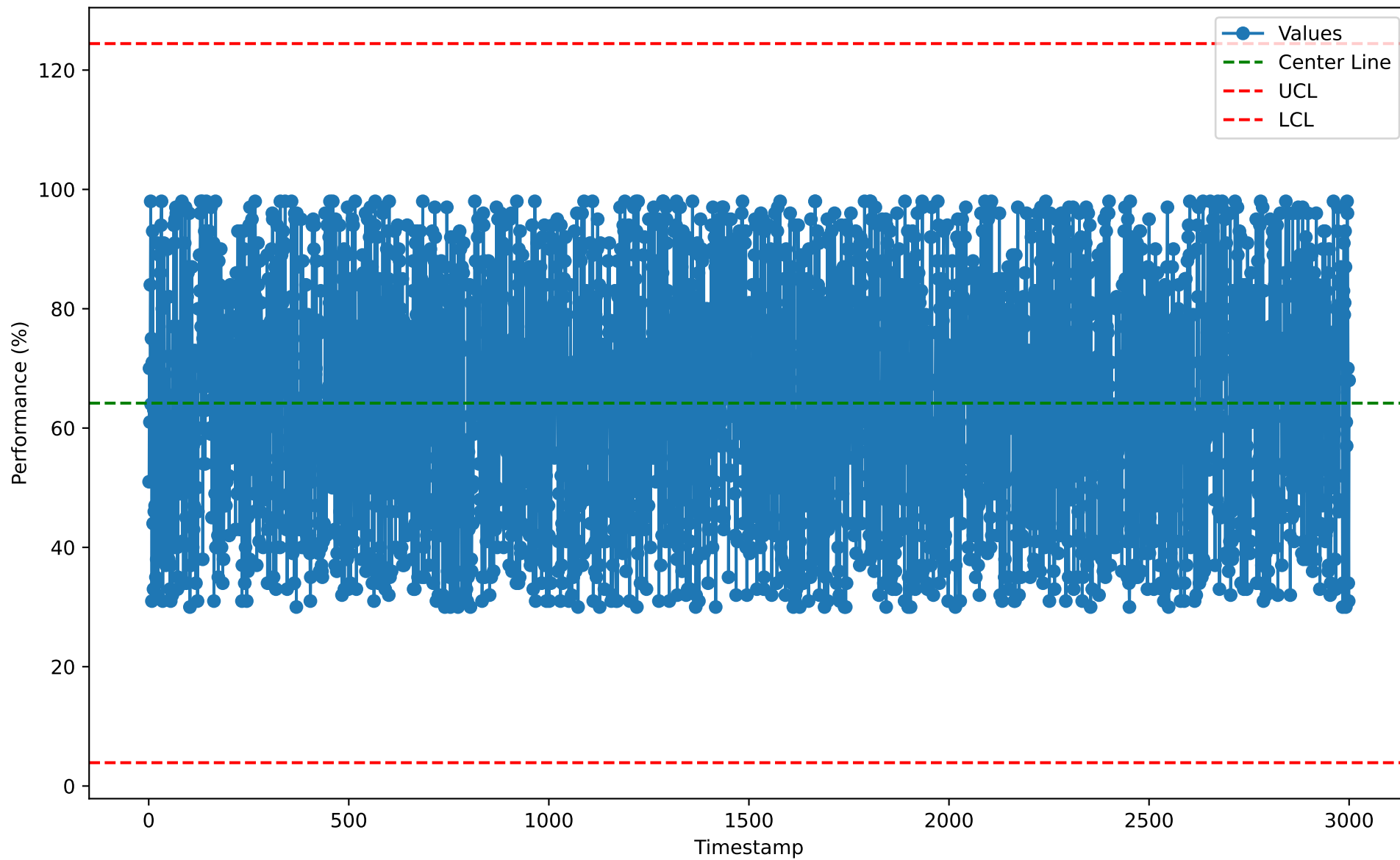
Individuals Chart for BPT10126 (2026-01-07)
