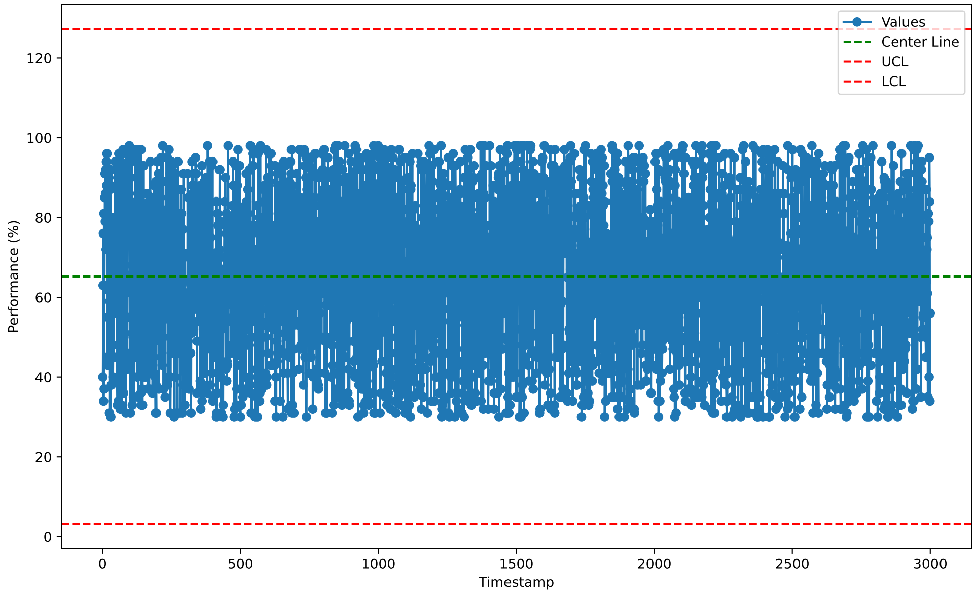
Individuals Chart for CMM10122 (2026-01-07)
