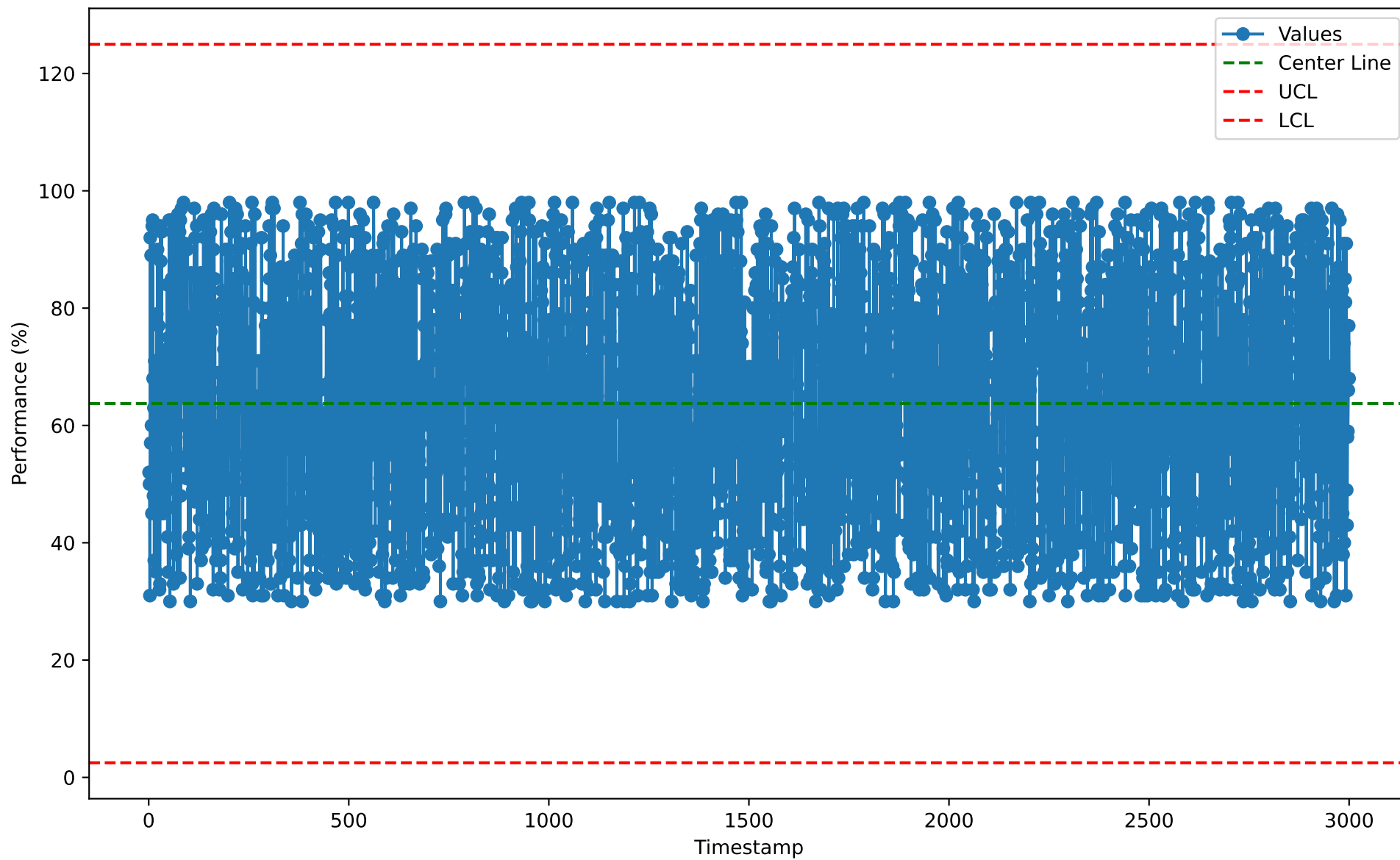
Individuals Chart for SYA10121 (2026-01-07)
