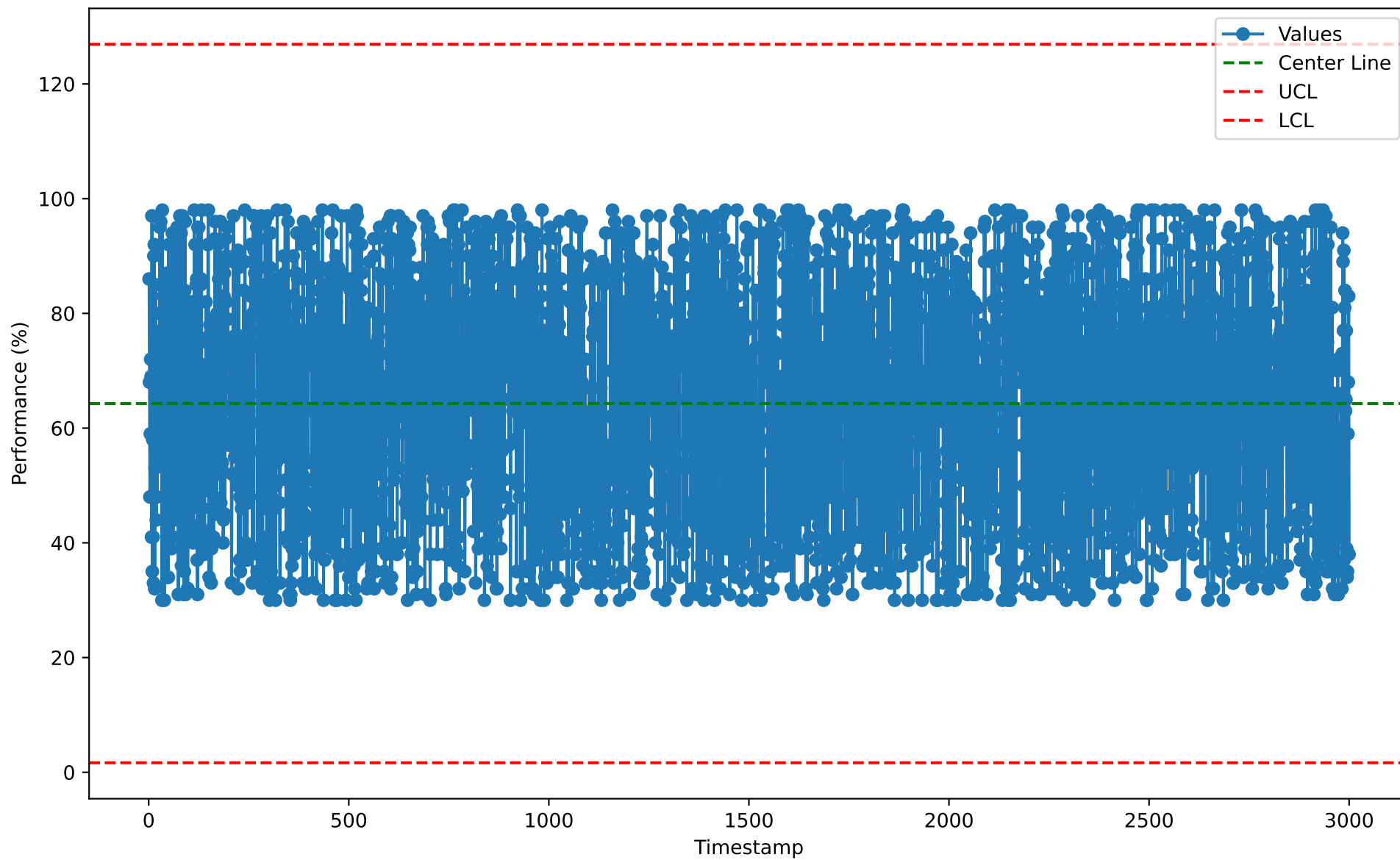
Individuals Chart for SYA10113 (2026-01-07)
