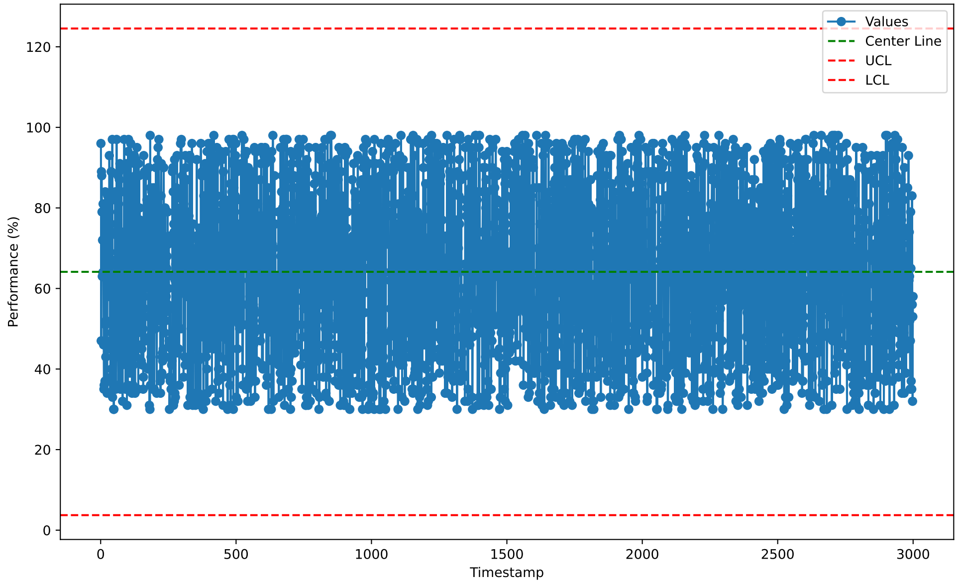
Individuals Chart for MDM10128 (2026-01-07)
