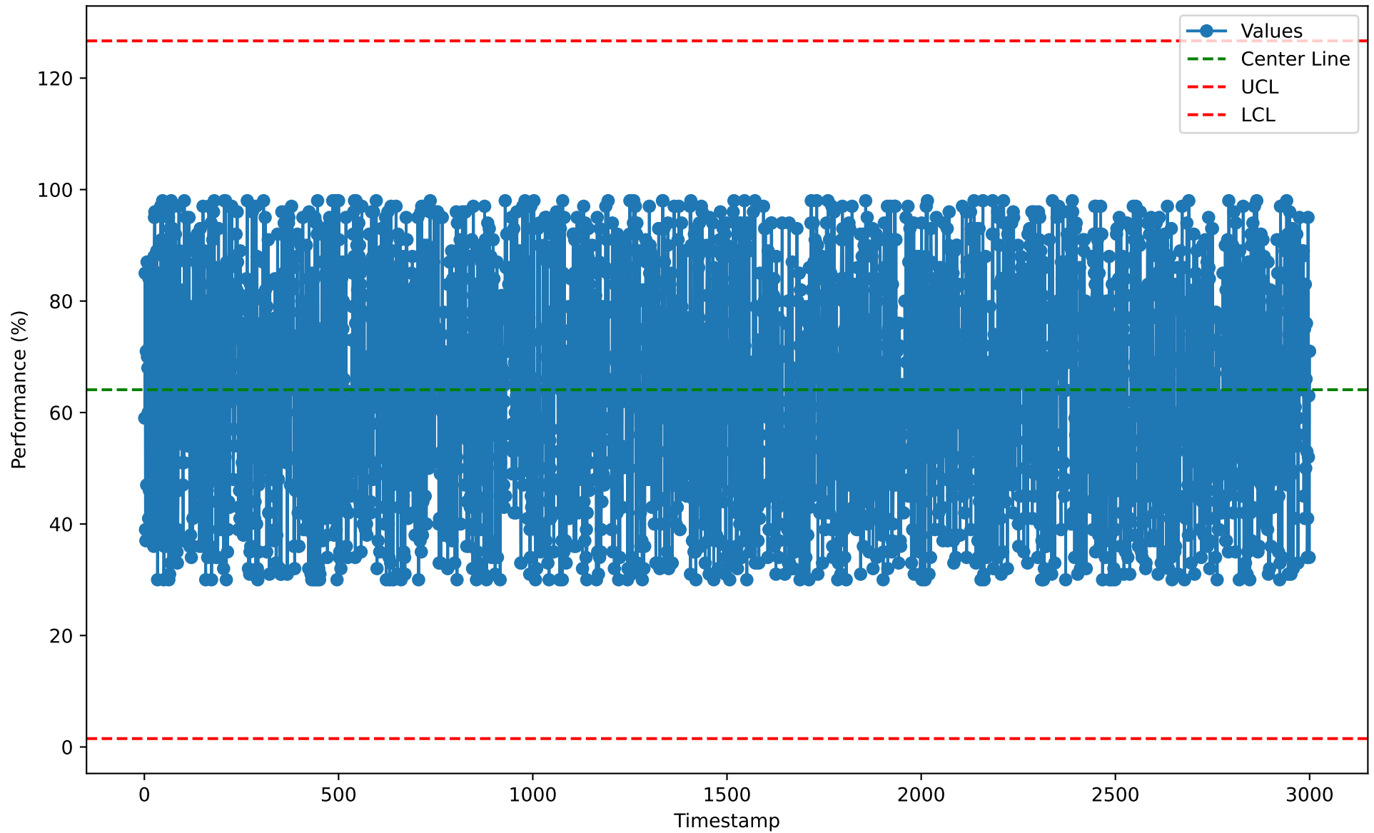
Individuals Chart for PTY10106 (2026-01-07)
