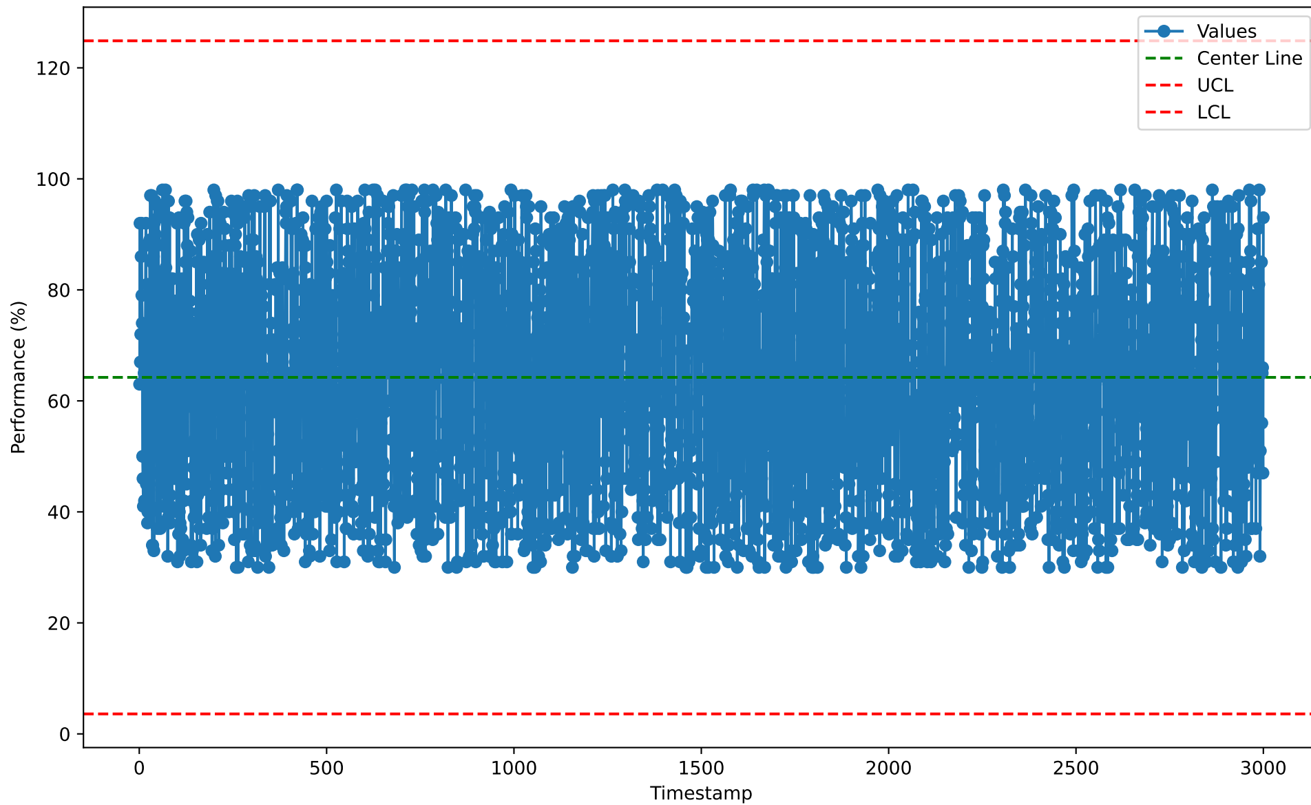
Individuals Chart for DLY10132 (2026-01-07)
