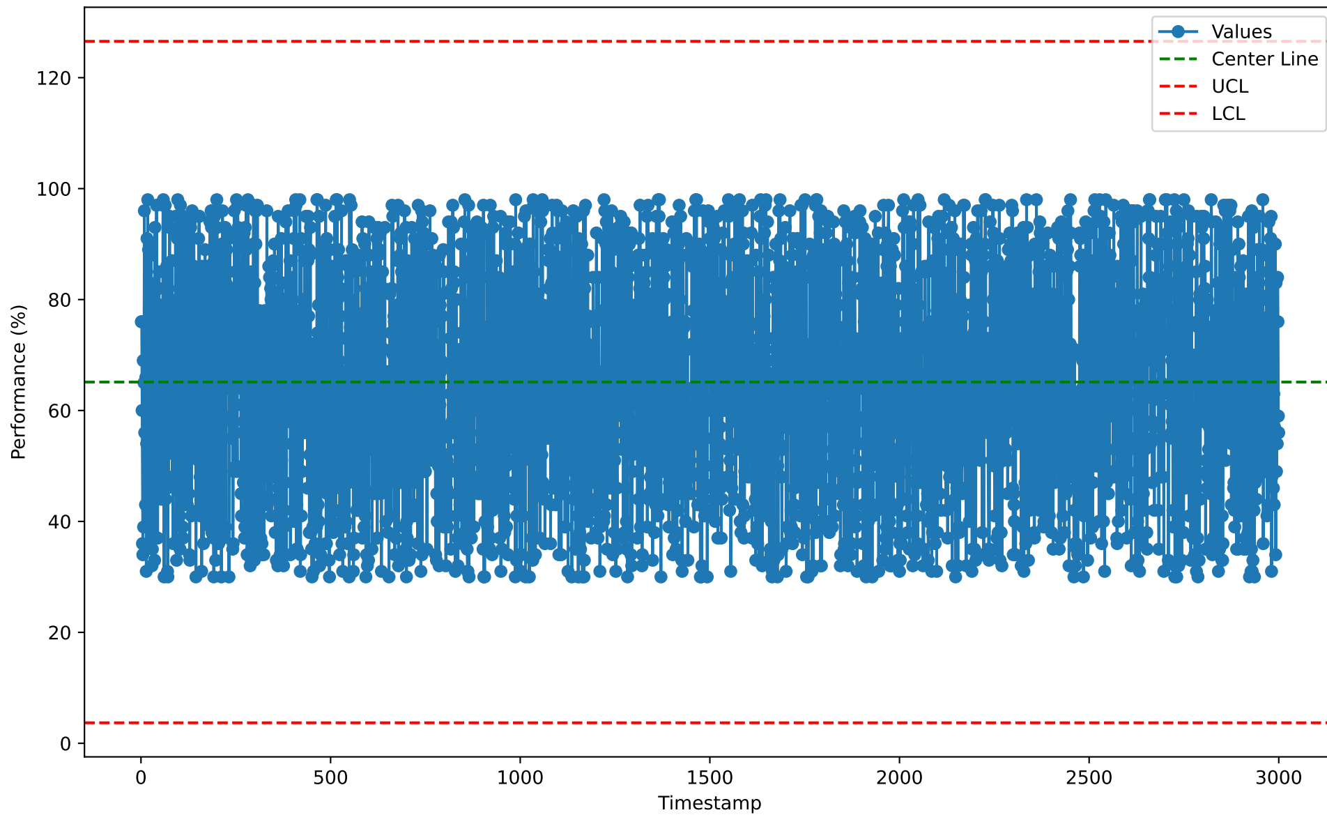
Individuals Chart for BPT10106 (2026-01-07)
