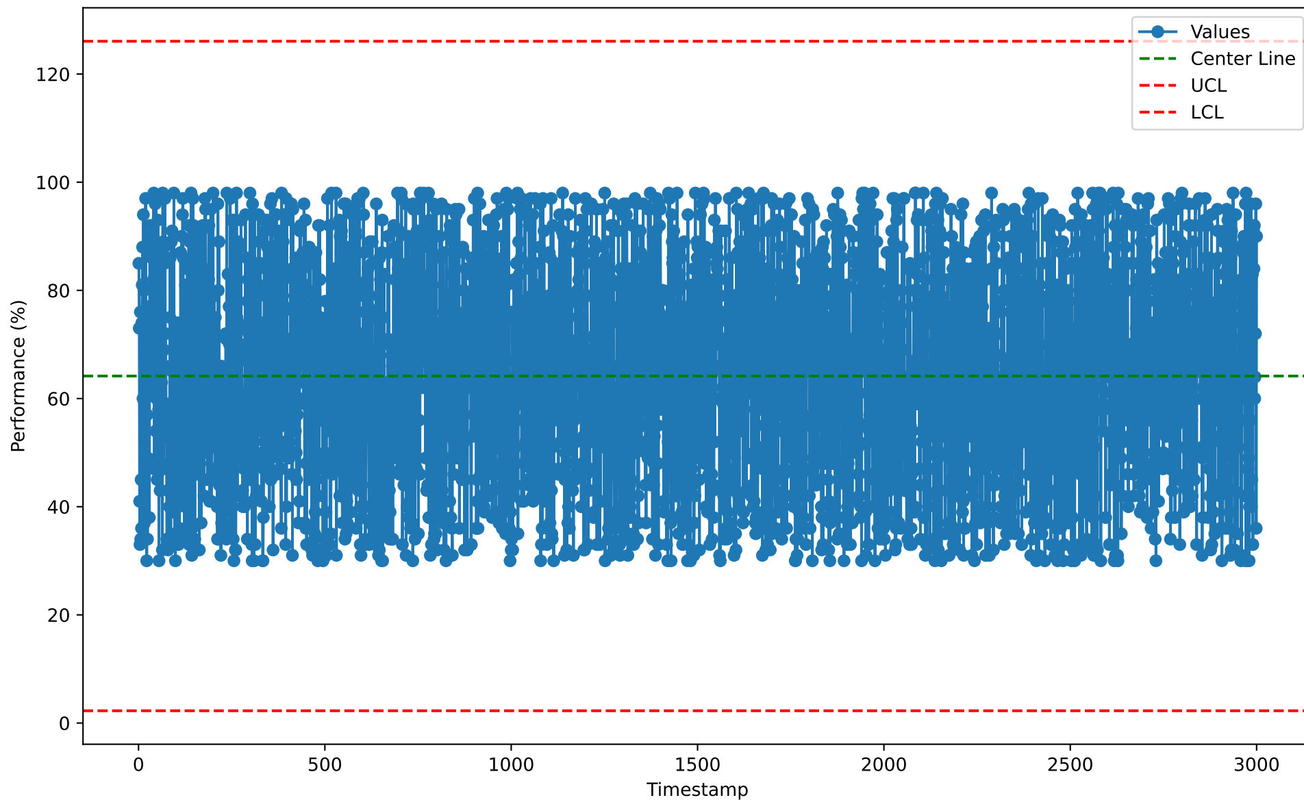
Individuals Chart for FLO10111 (2026-01-07)
