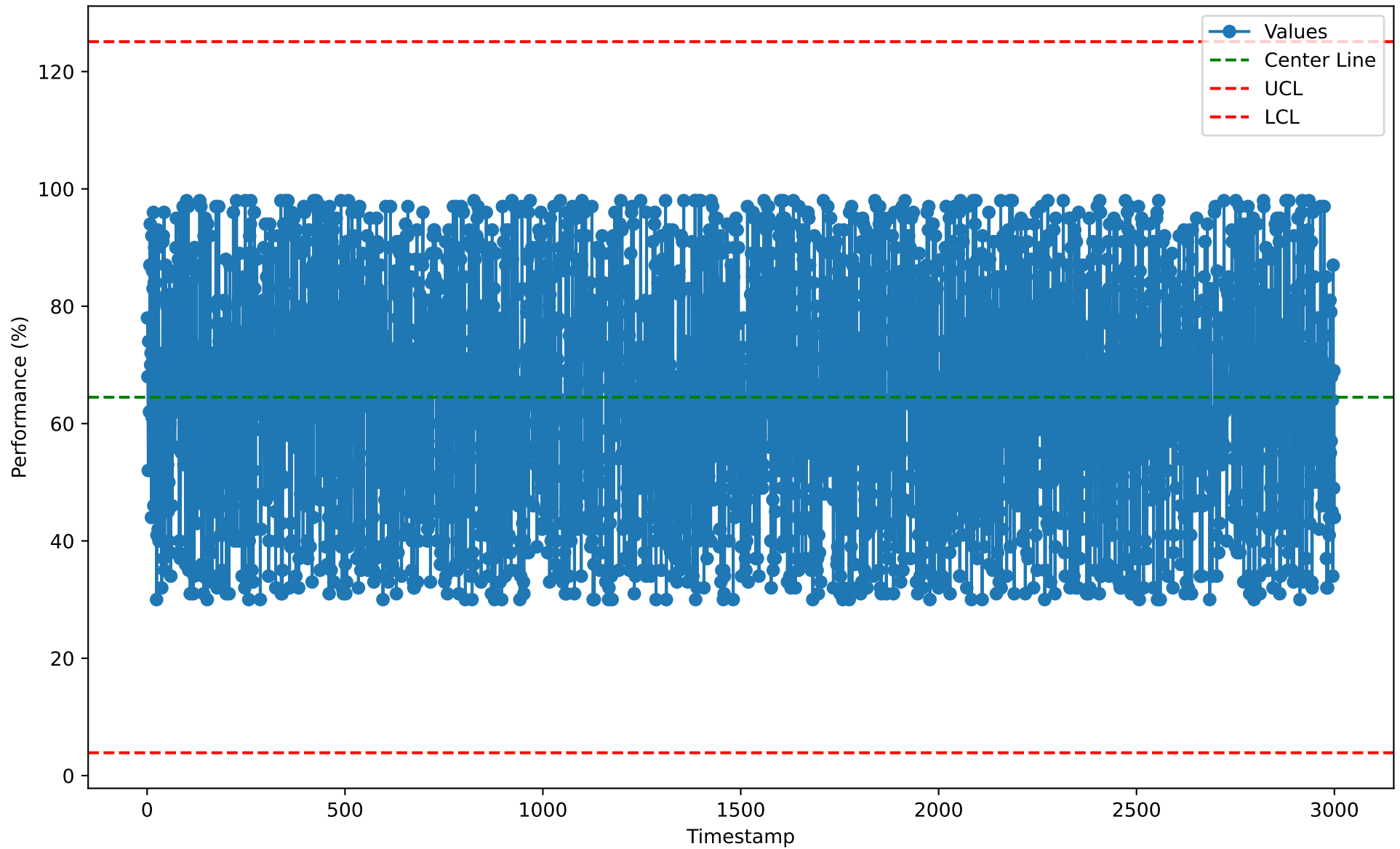
Individuals Chart for CMM10111 (2026-01-07)
