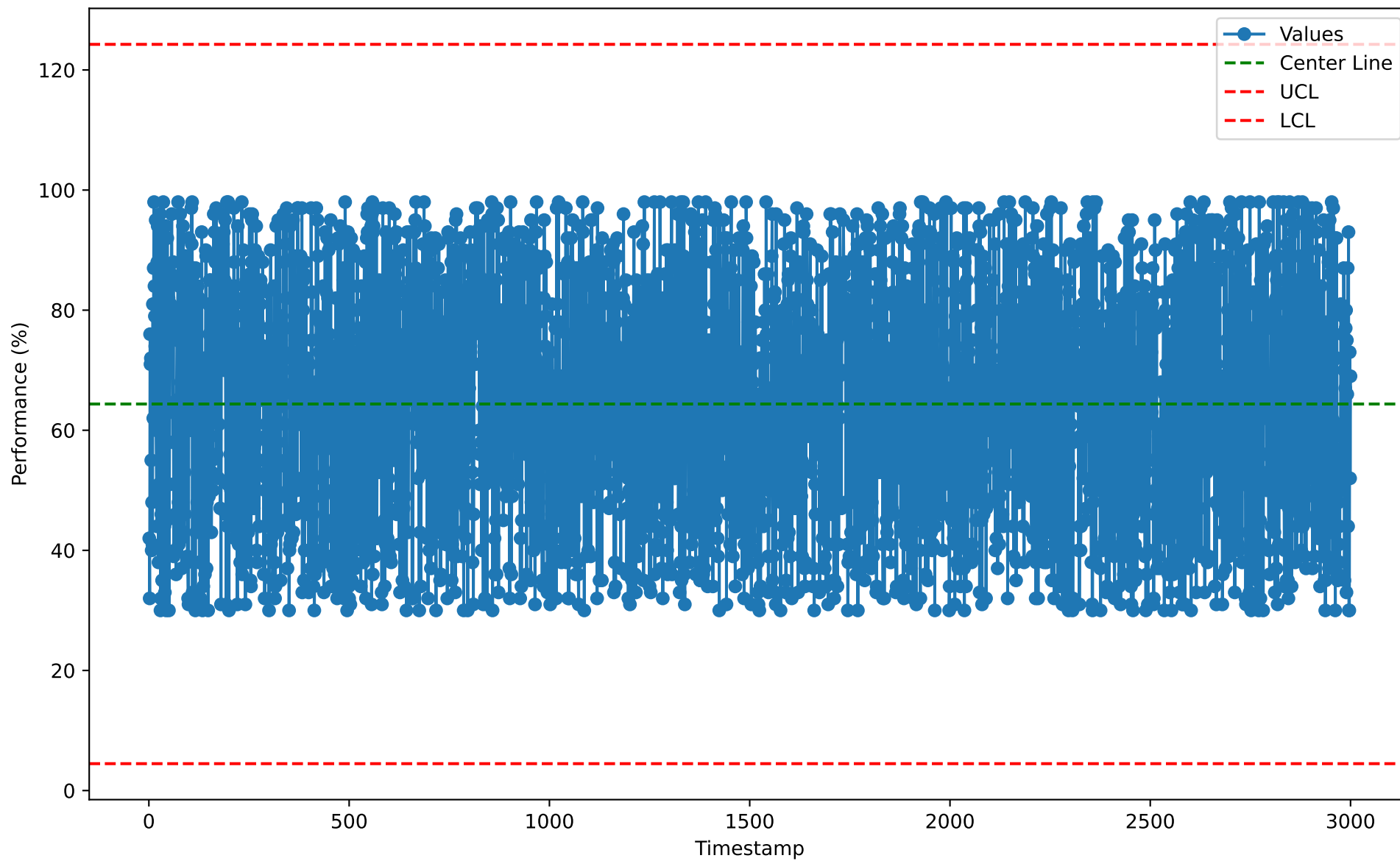
Individuals Chart for DLY10120 (2026-01-07)
