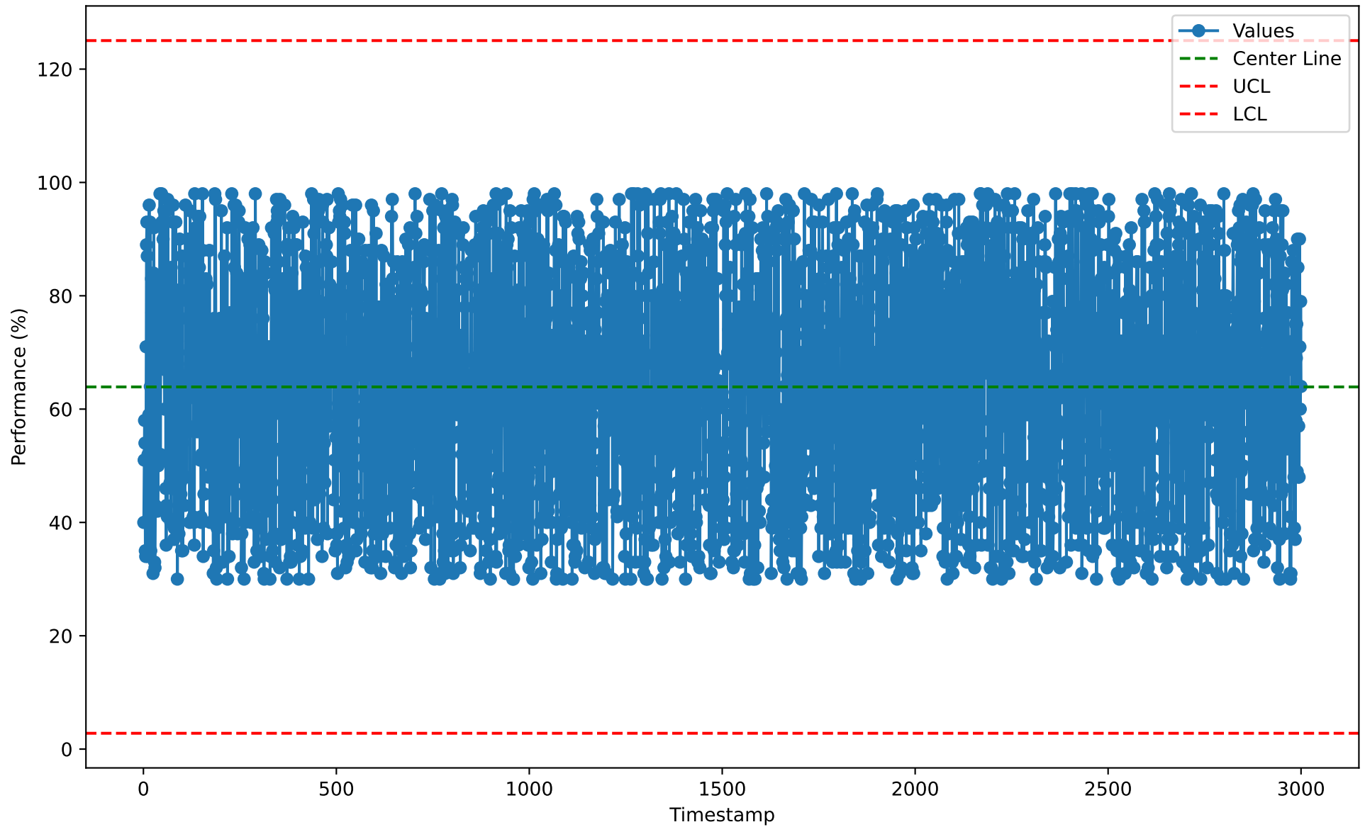
Individuals Chart for MDM10127 (2026-01-07)
