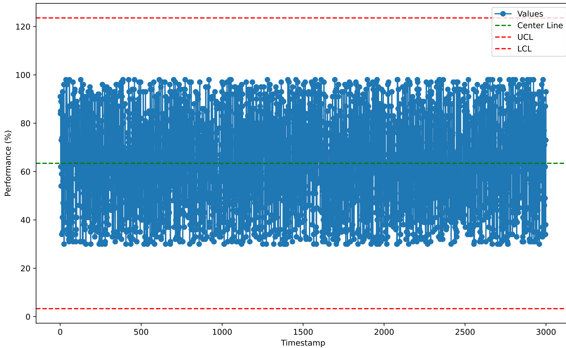
Individuals Chart for DLY10112 (2026-01-07)
