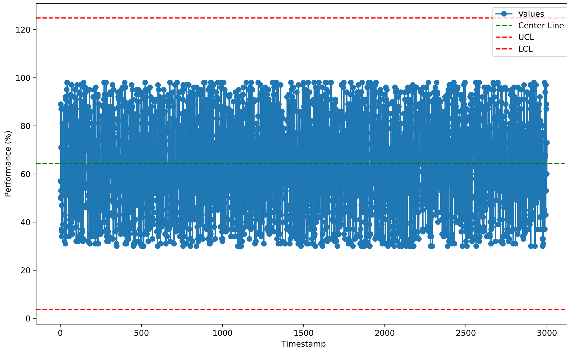
Individuals Chart for IDP10126 (2026-01-07)
