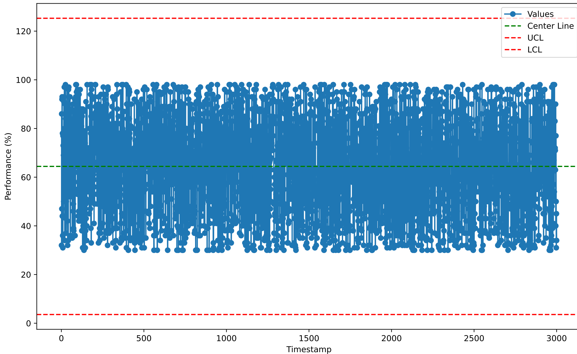
Individuals Chart for DLY10103 (2026-01-07)
