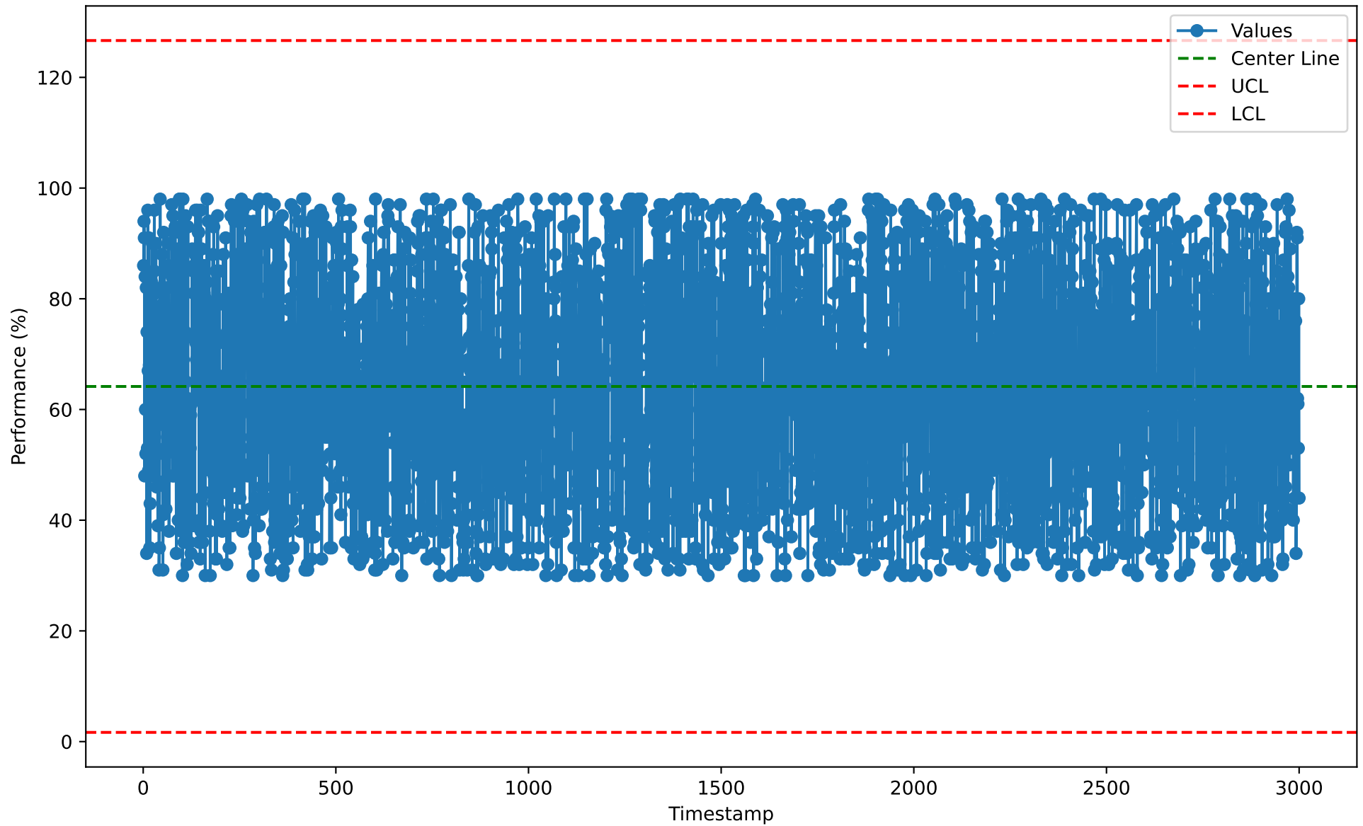
Individuals Chart for MDM10107 (2026-01-07)
