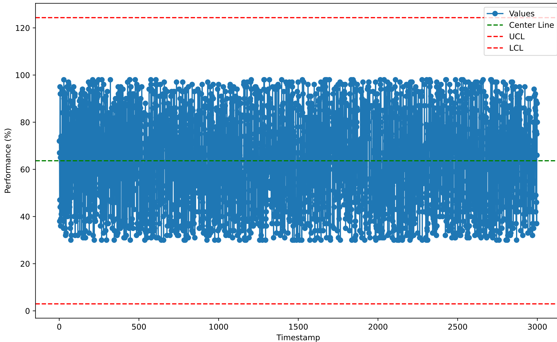
Individuals Chart for IDP10125 (2026-01-07)
