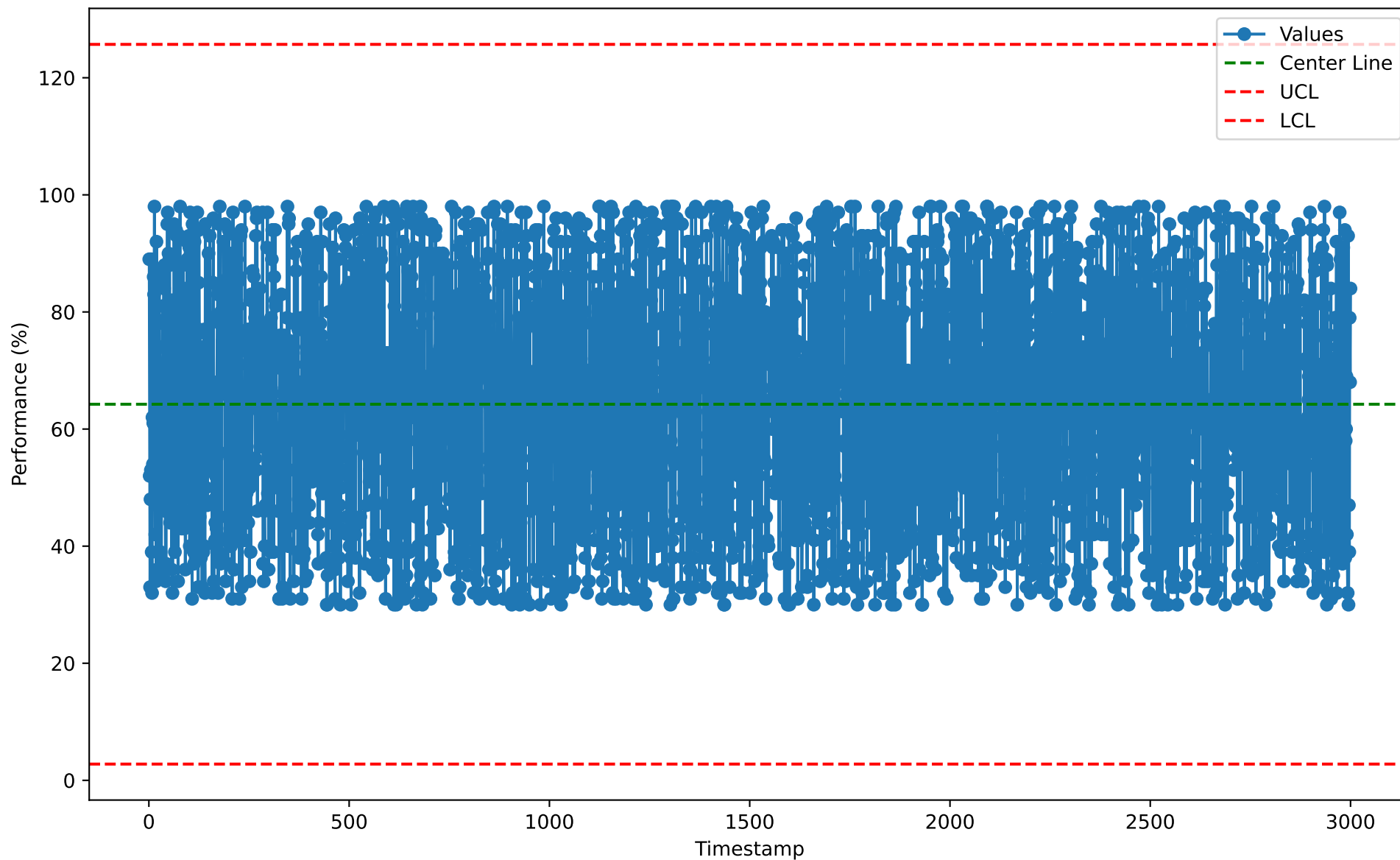
Individuals Chart for BPT10108 (2026-01-07)
