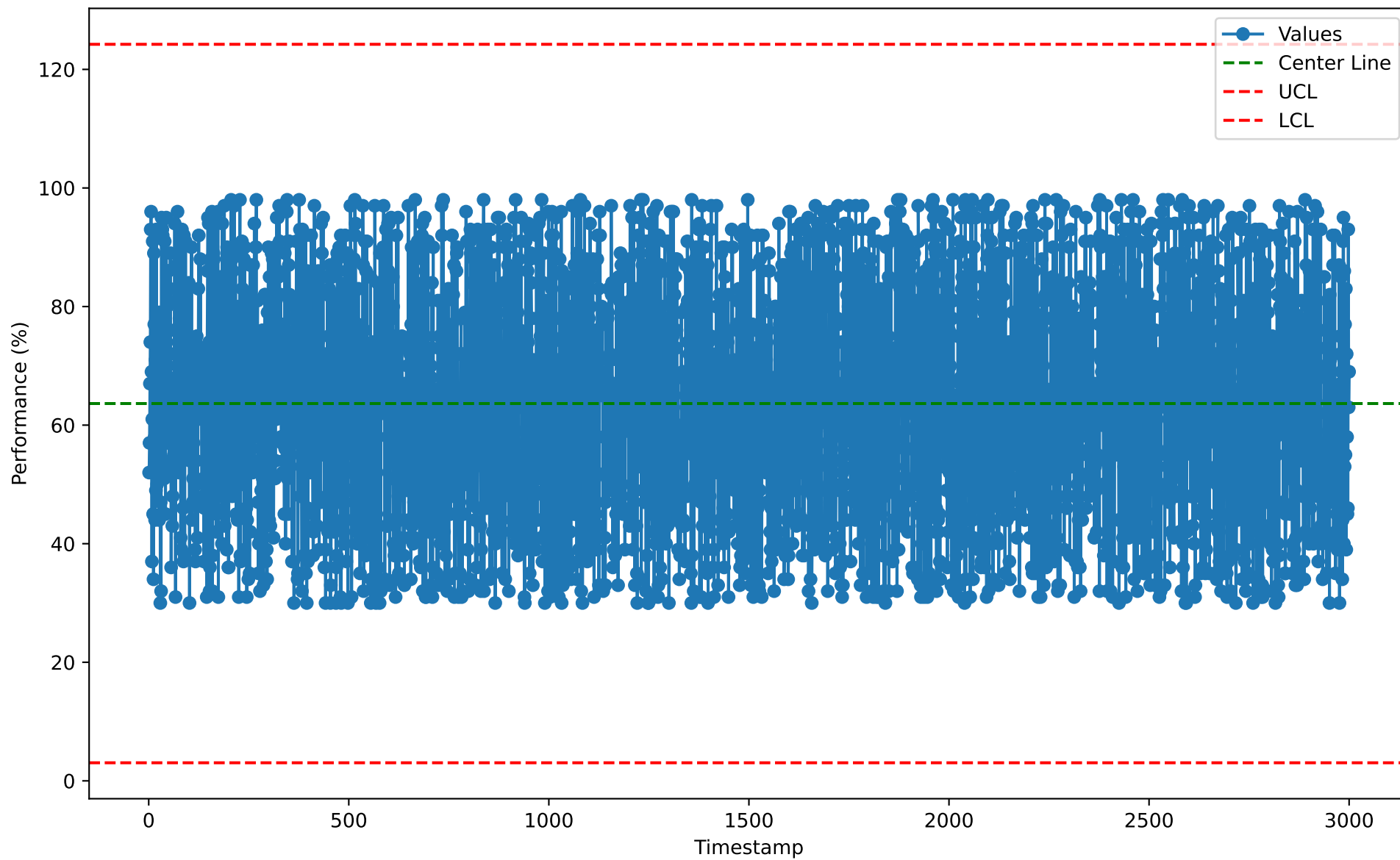
Individuals Chart for PJM10118 (2026-01-07)
