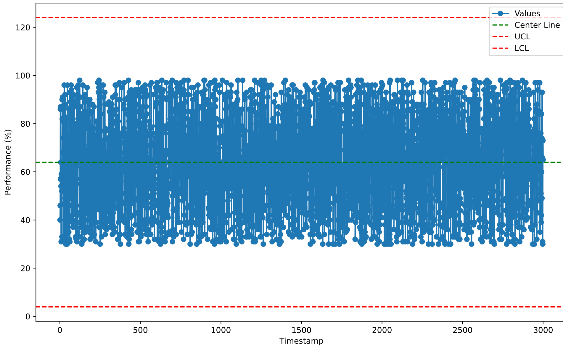
Individuals Chart for PJM10120 (2026-01-07)
