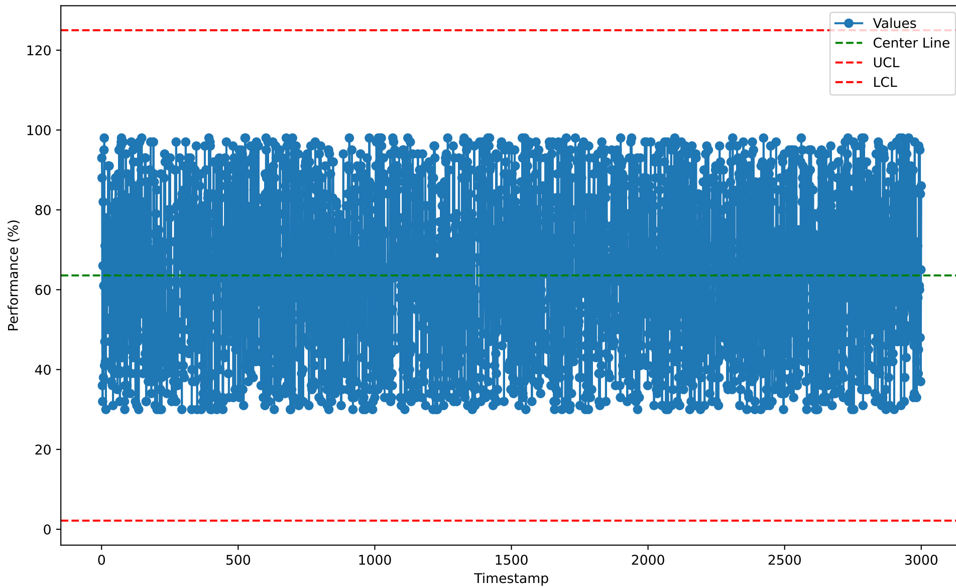
Individuals Chart for PJM10124 (2026-01-07)
