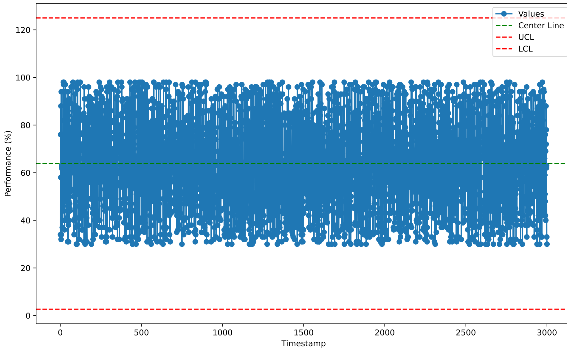
Individuals Chart for PTY10112 (2026-01-07)
