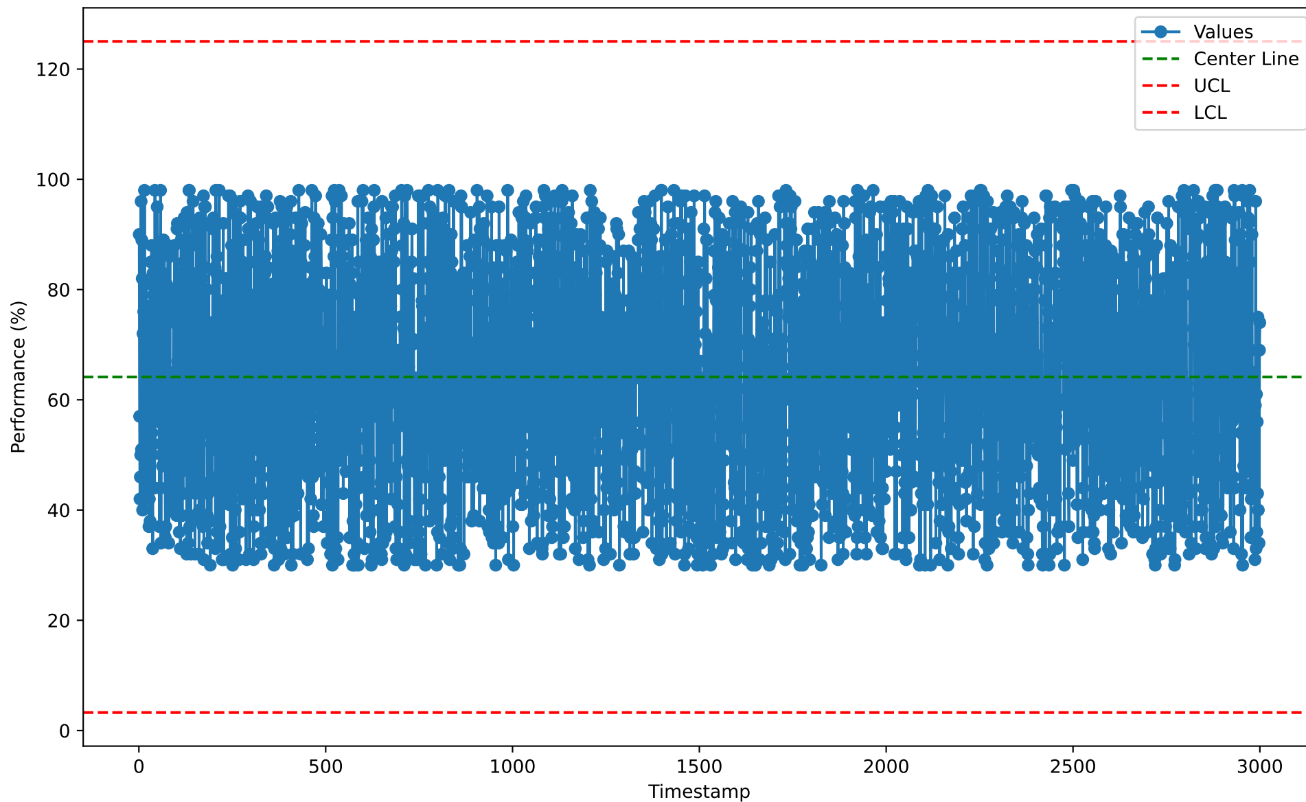
Individuals Chart for SYA10123 (2026-01-07)
