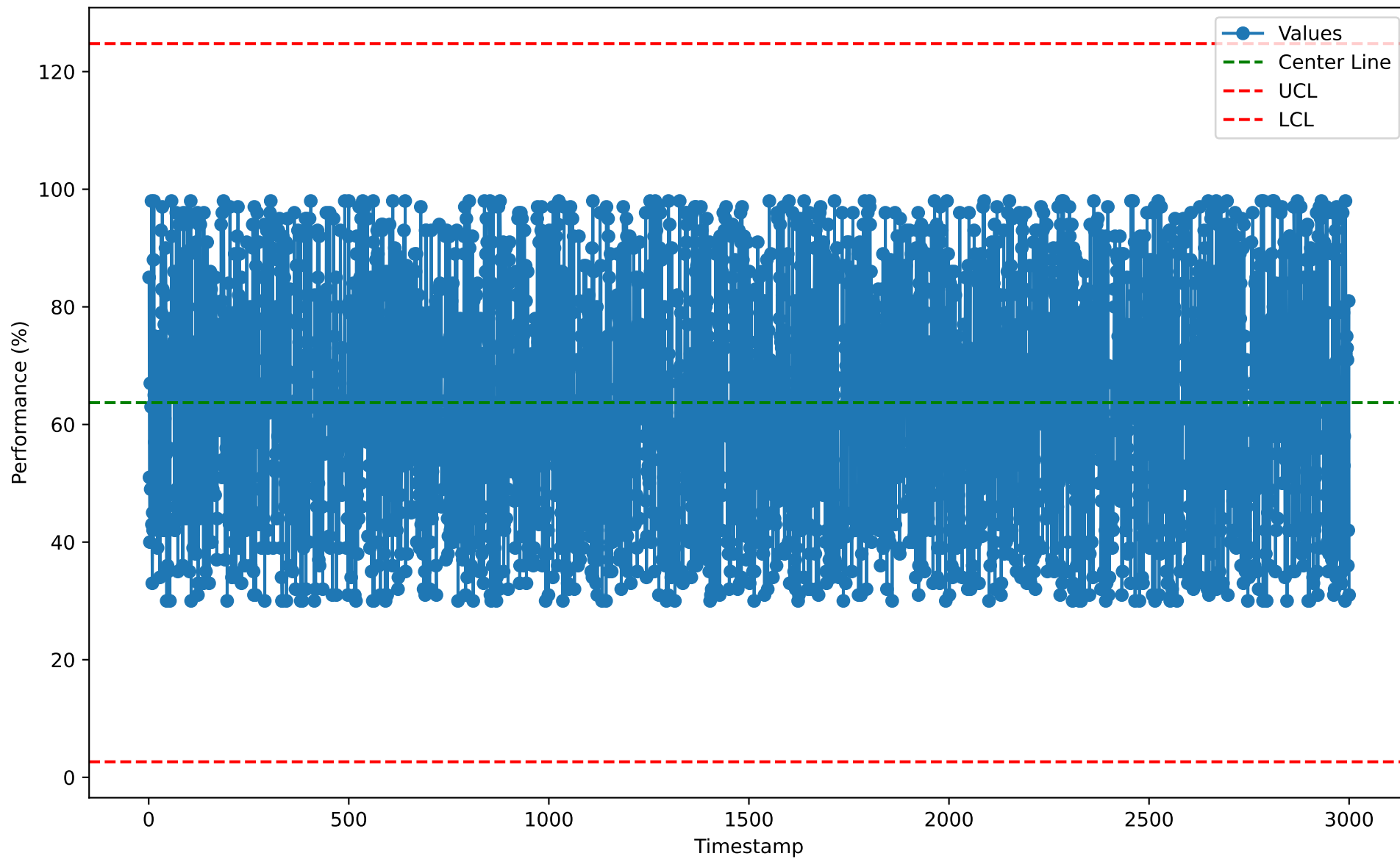
Individuals Chart for IDP10110 (2026-01-07)
