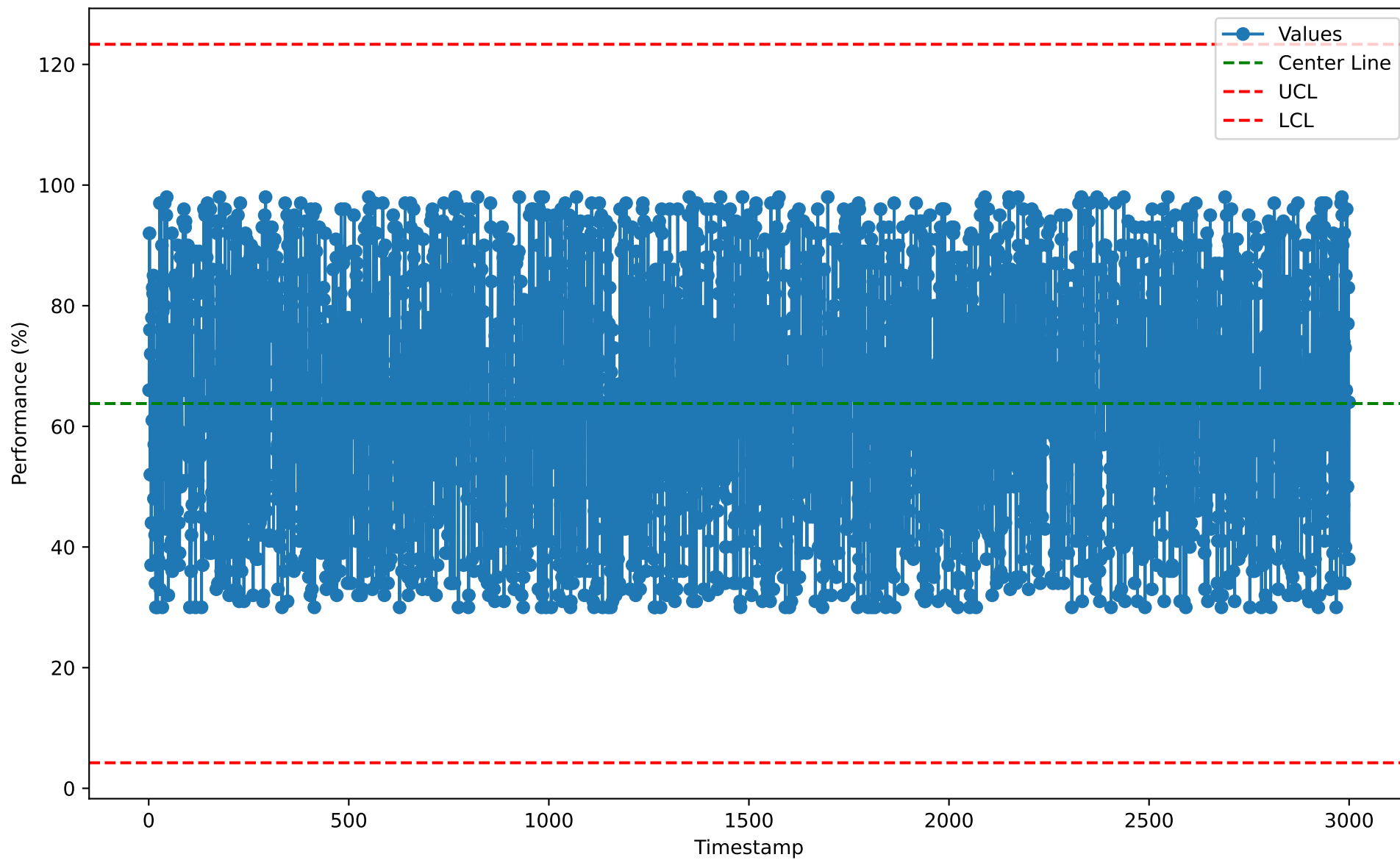
Individuals Chart for DLY10134 (2026-01-07)
