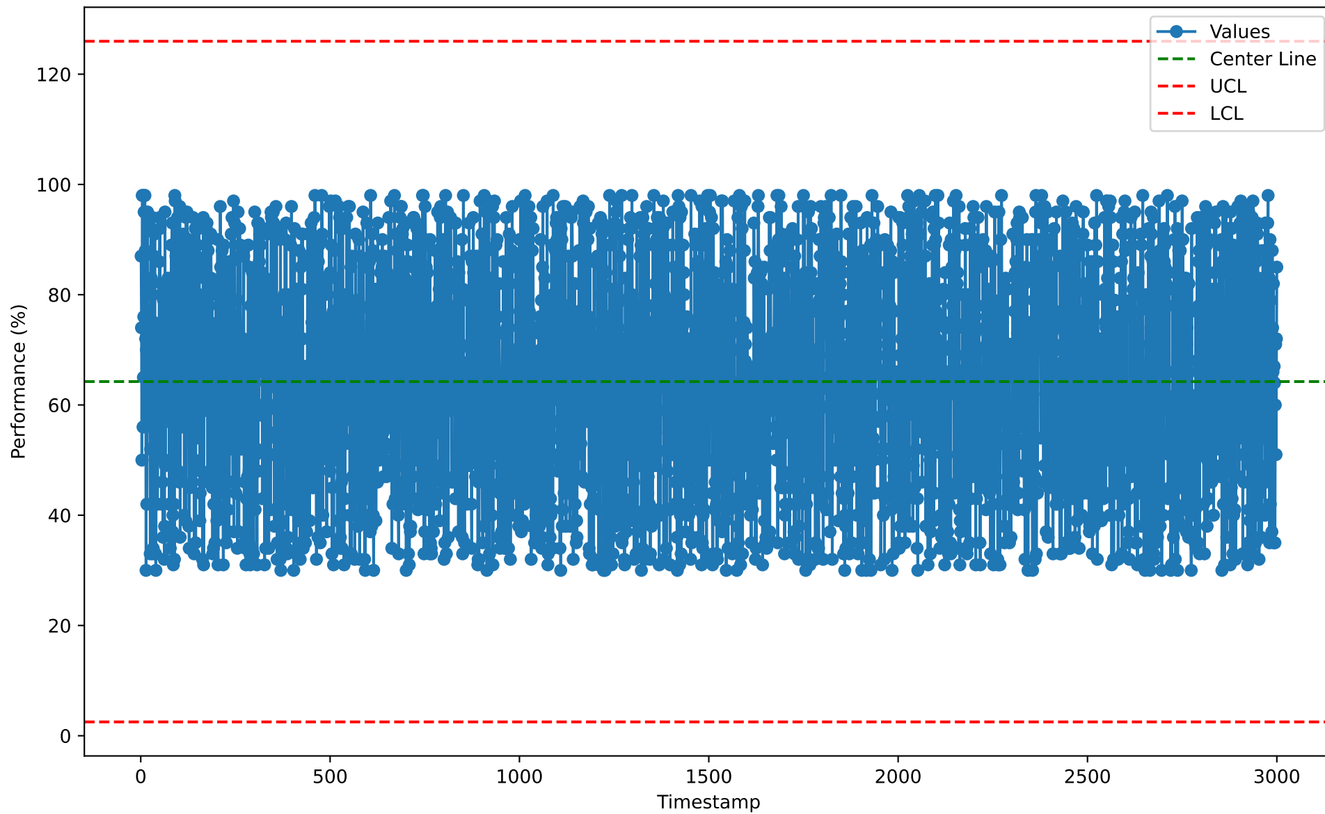
Individuals Chart for DLY10118 (2026-01-07)
