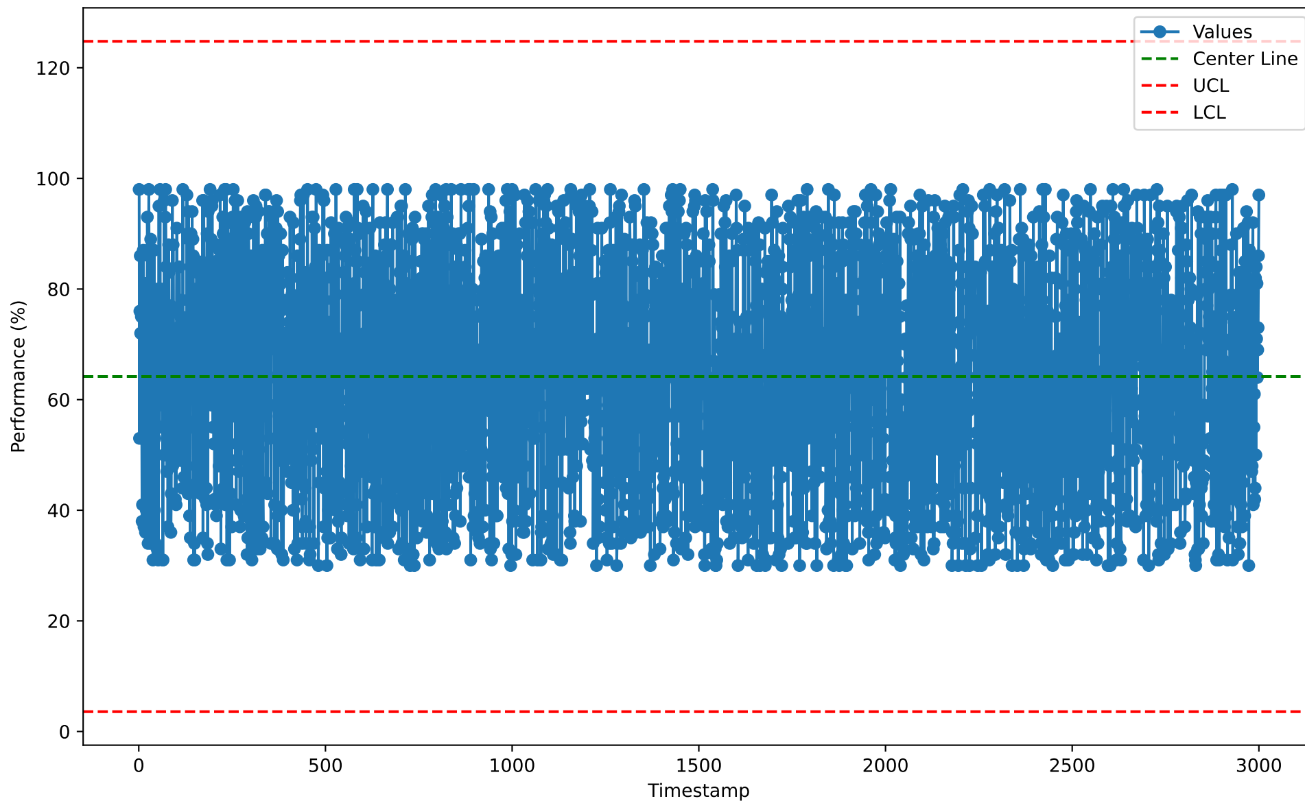
Individuals Chart for PTY10119 (2026-01-07)
