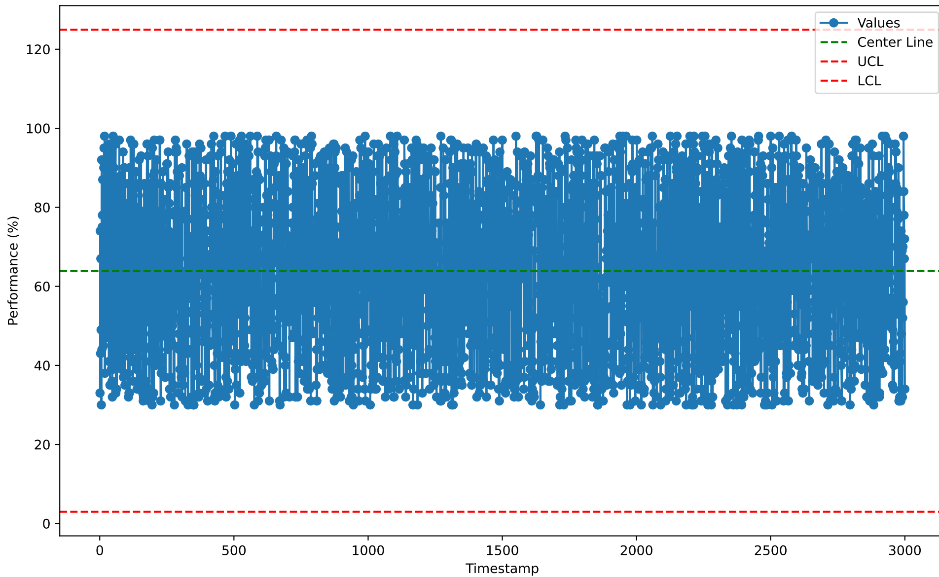
Individuals Chart for DLY10104 (2026-01-07)
