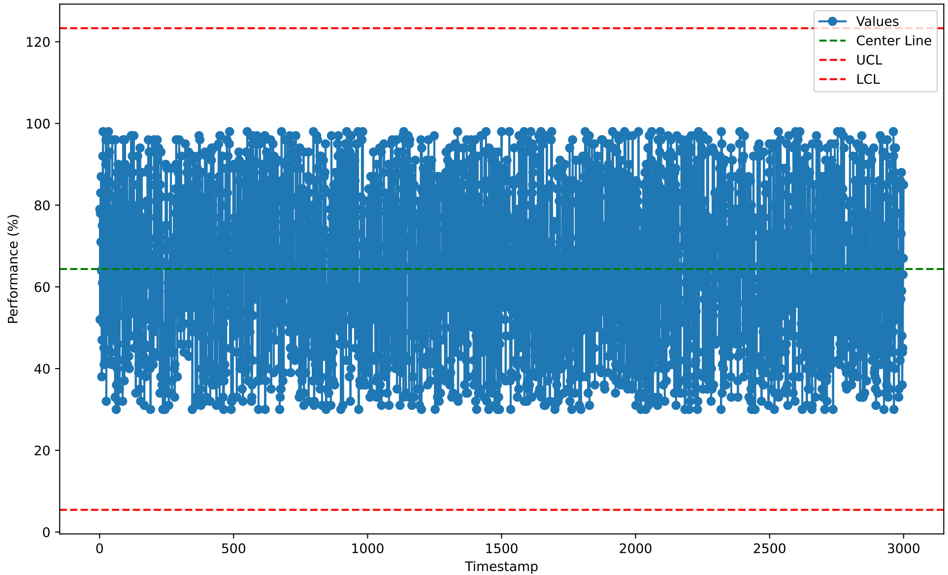
Individuals Chart for CMM10115 (2026-01-07)
