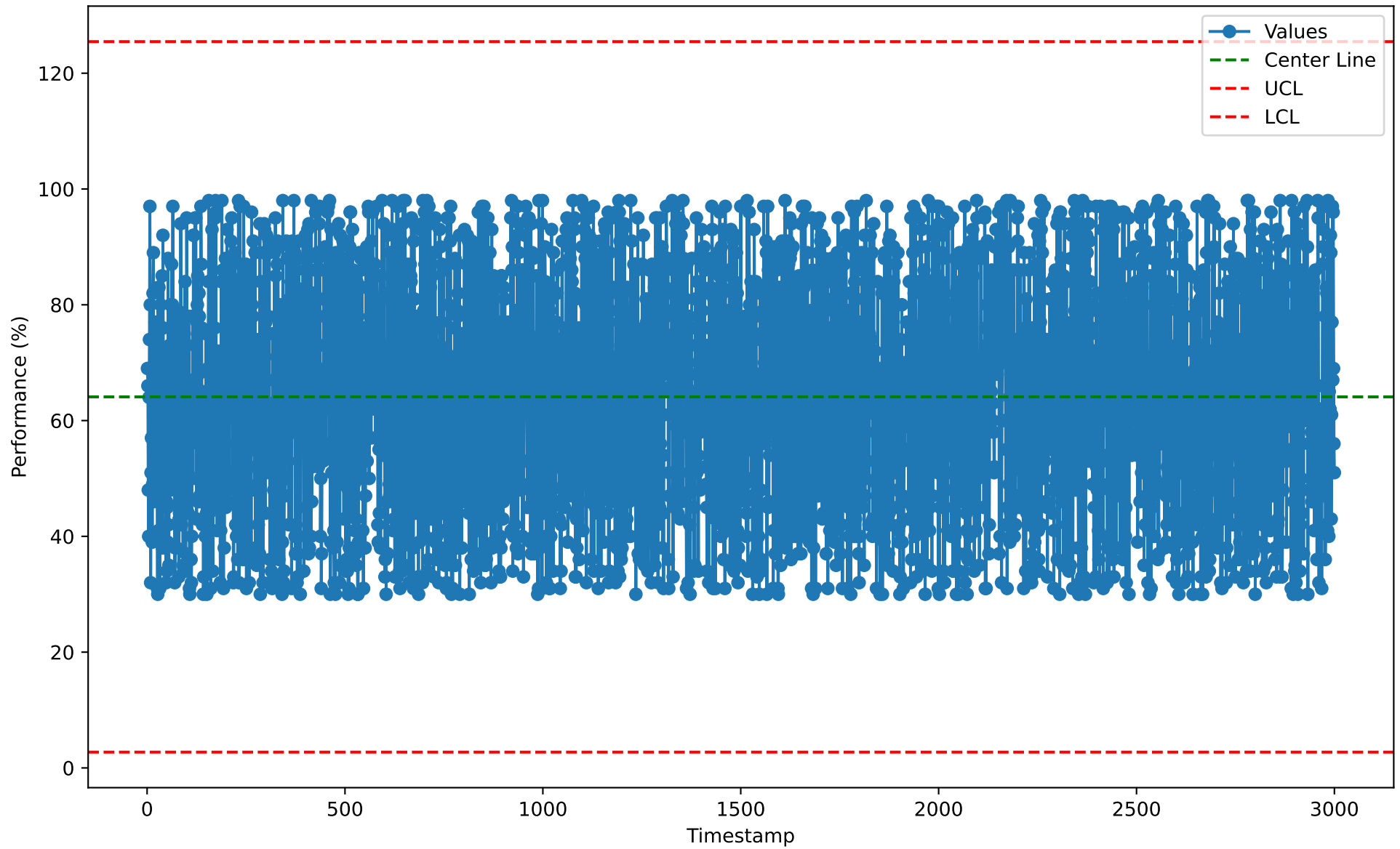
Individuals Chart for MDM10116 (2026-01-07)
