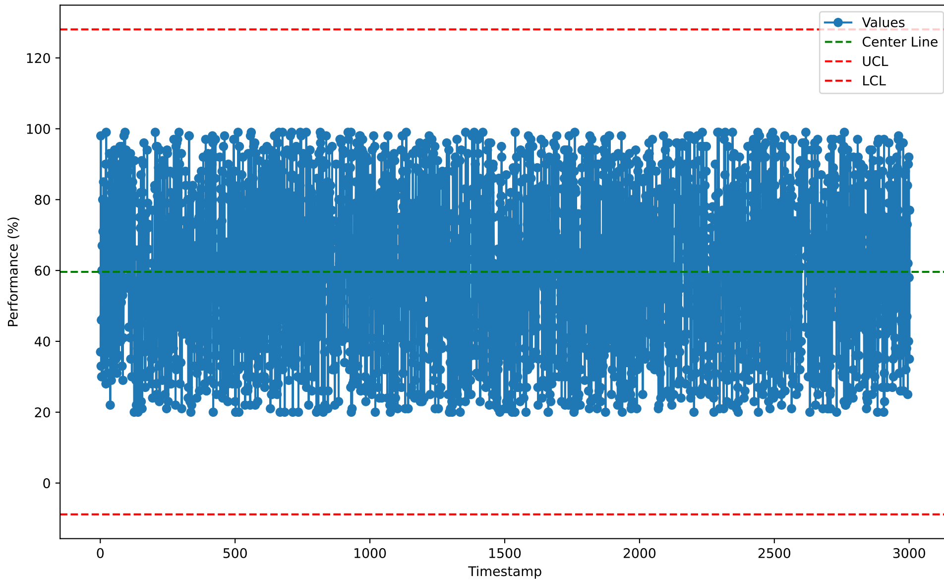
Individuals Chart for CFS10115 (2026-01-07)
