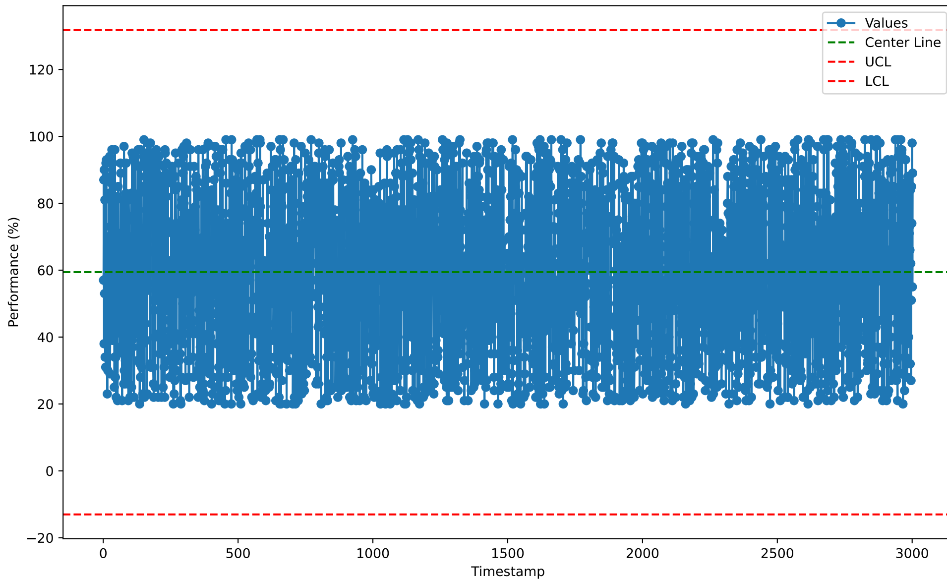
Individuals Chart for ITM10116 (2026-01-07)
