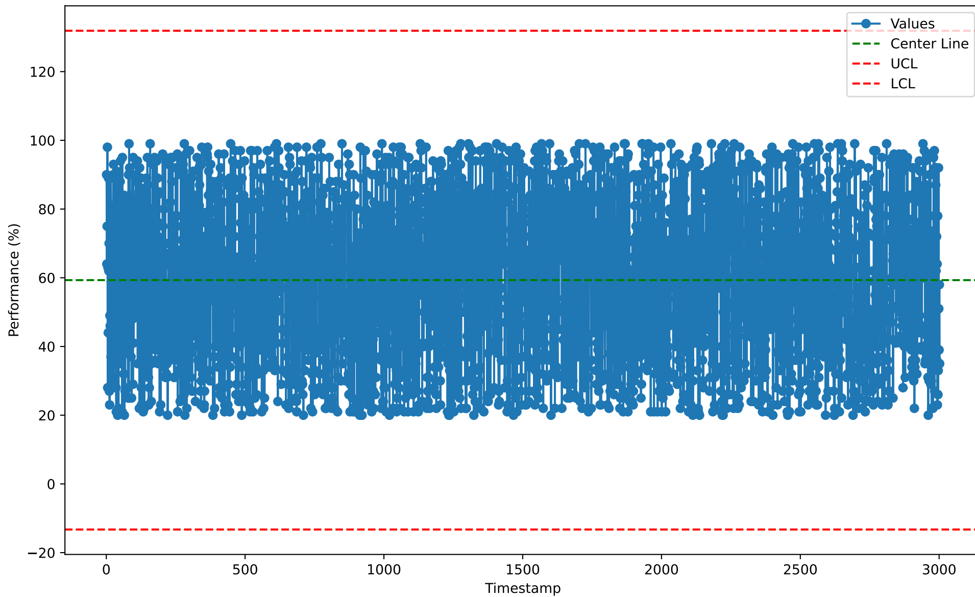
Individuals Chart for BIH10117 (2026-01-07)
