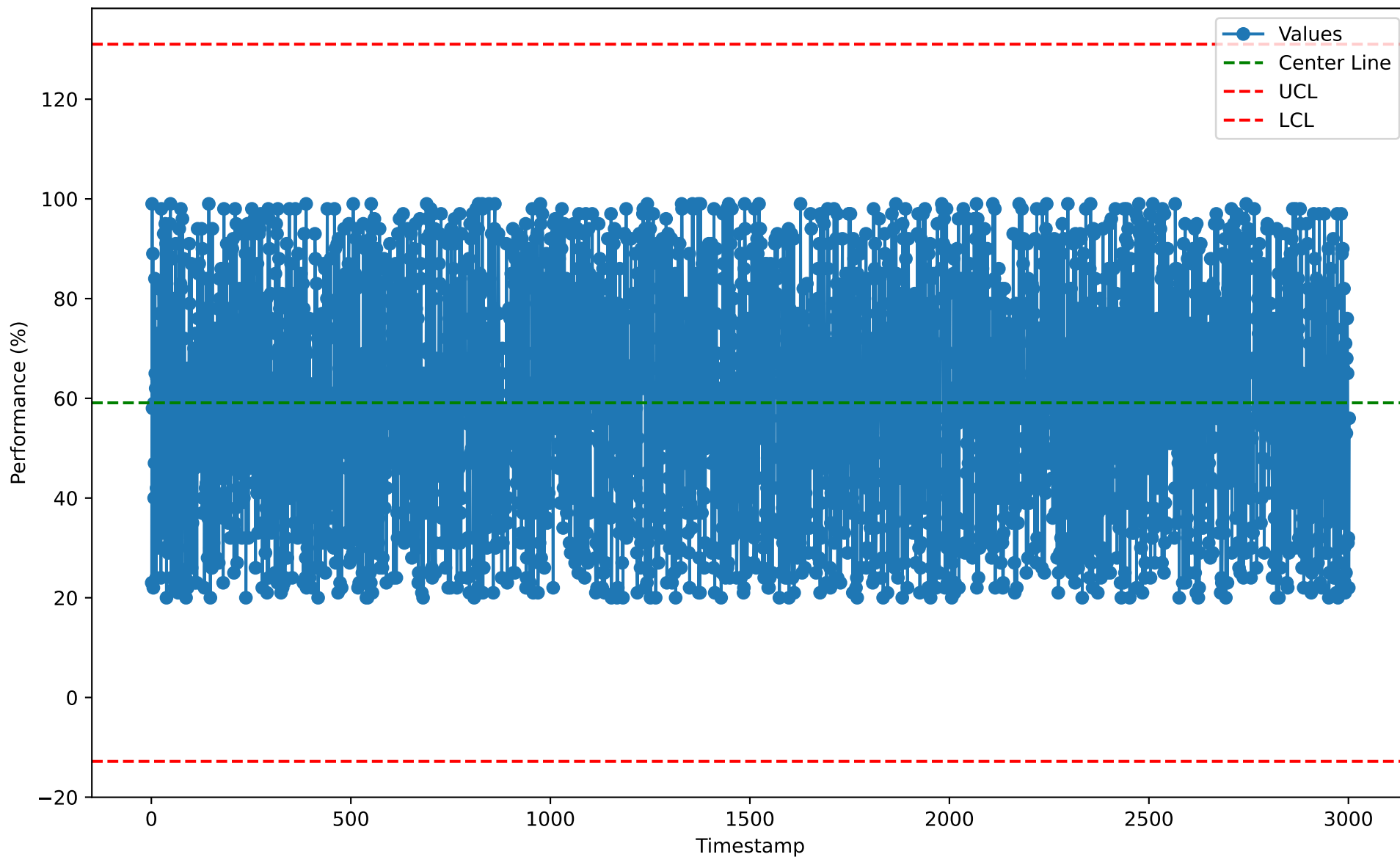
Individuals Chart for BIM10105 (2026-01-07)
