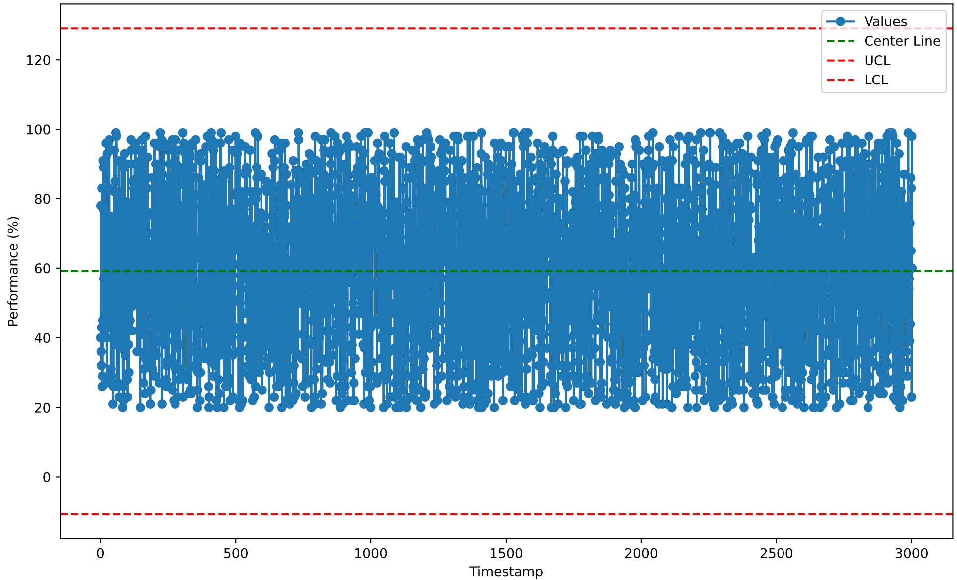
Individuals Chart for BIH10111 (2026-01-07)
