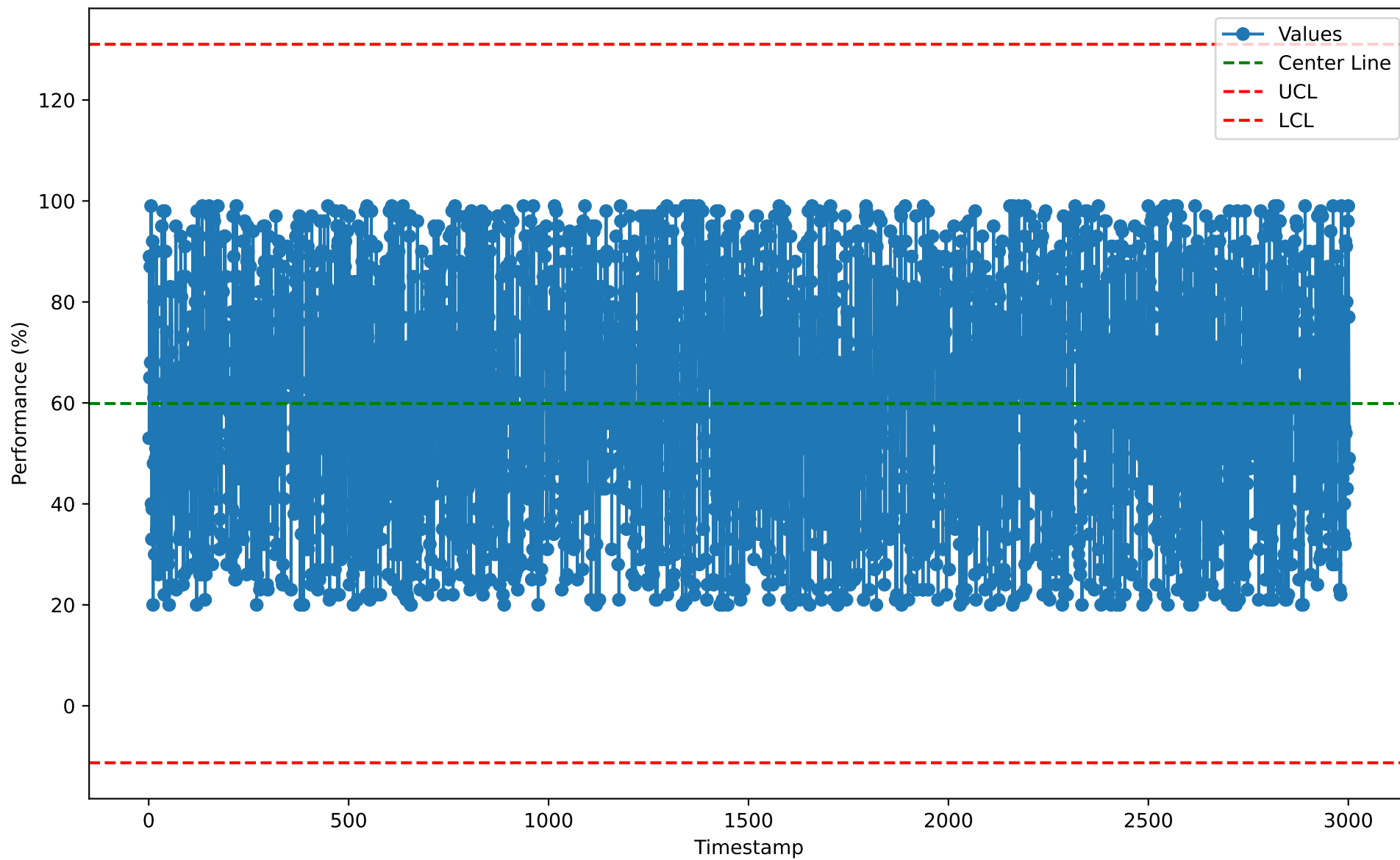
Individuals Chart for CFS10105 (2026-01-07)
