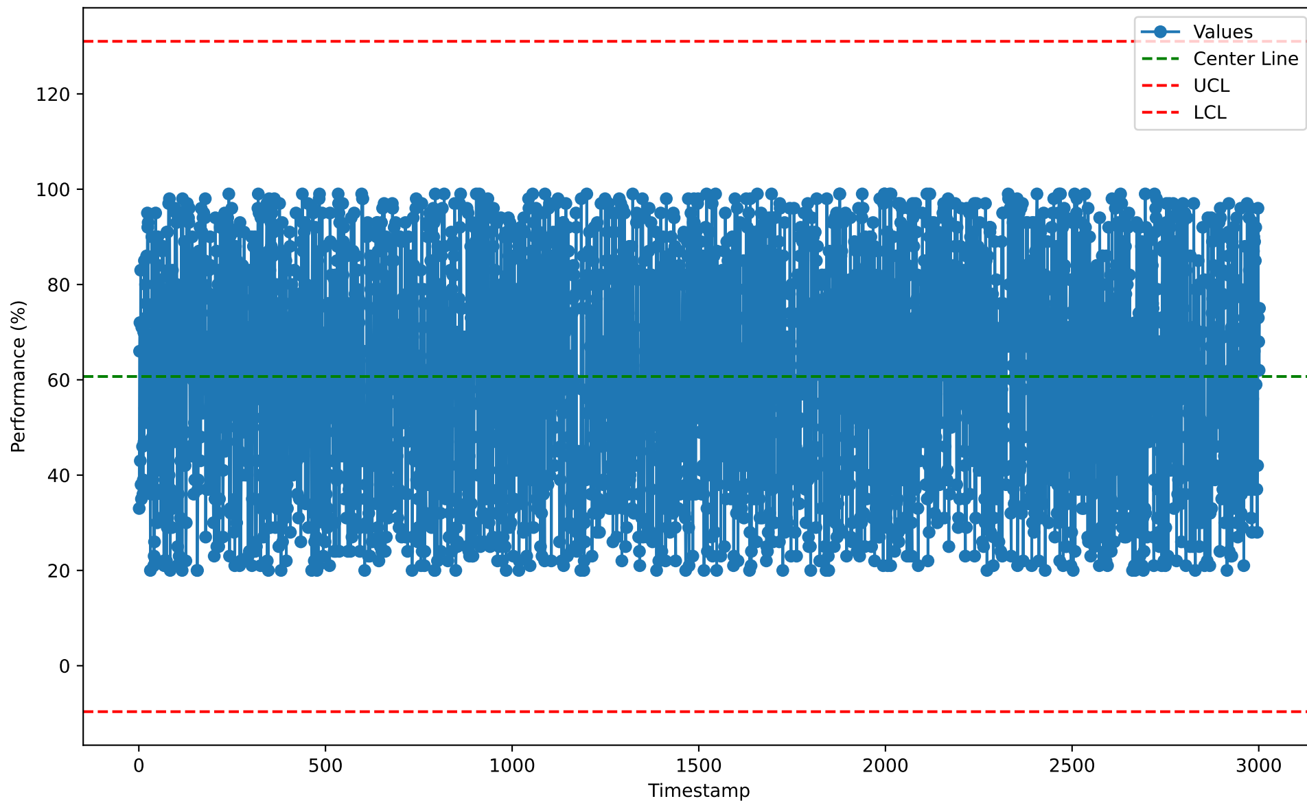
Individuals Chart for CIM10113 (2026-01-07)
