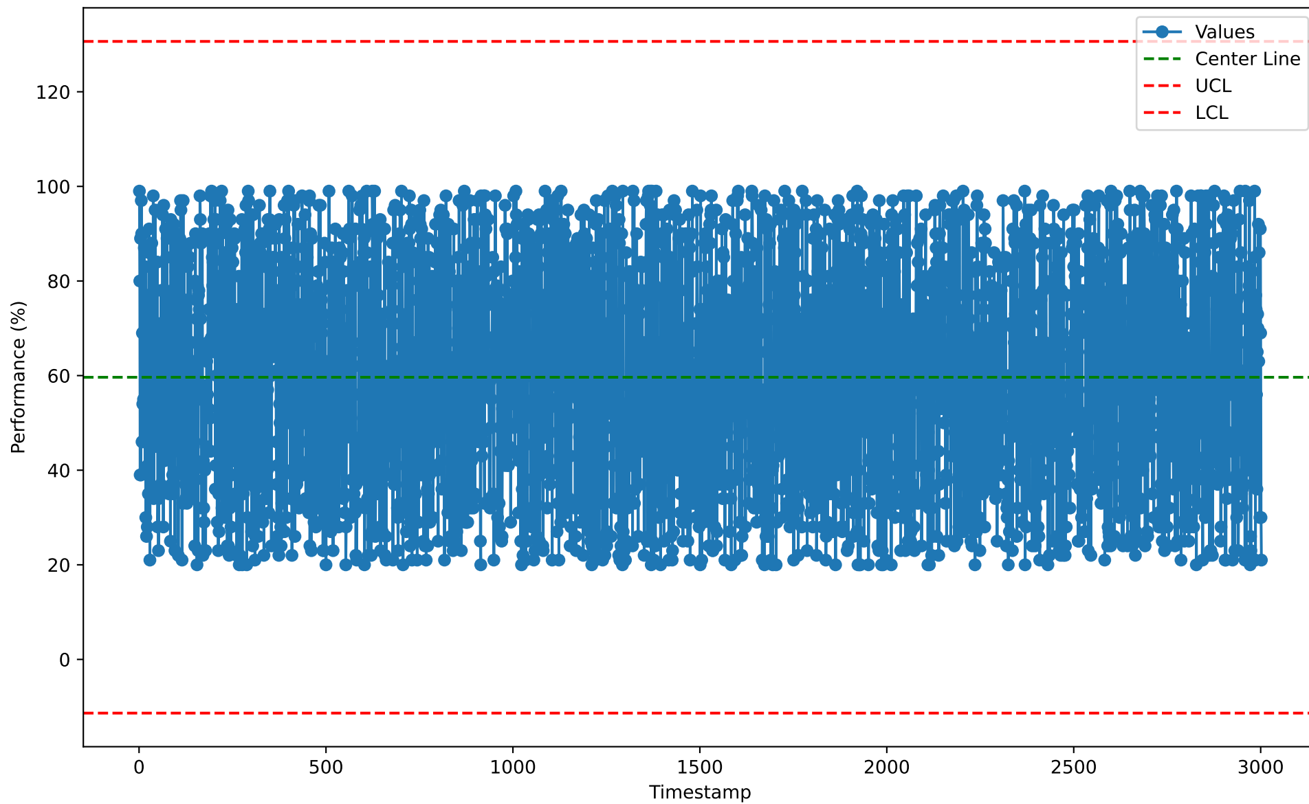
Individuals Chart for CFS10114 (2026-01-07)
