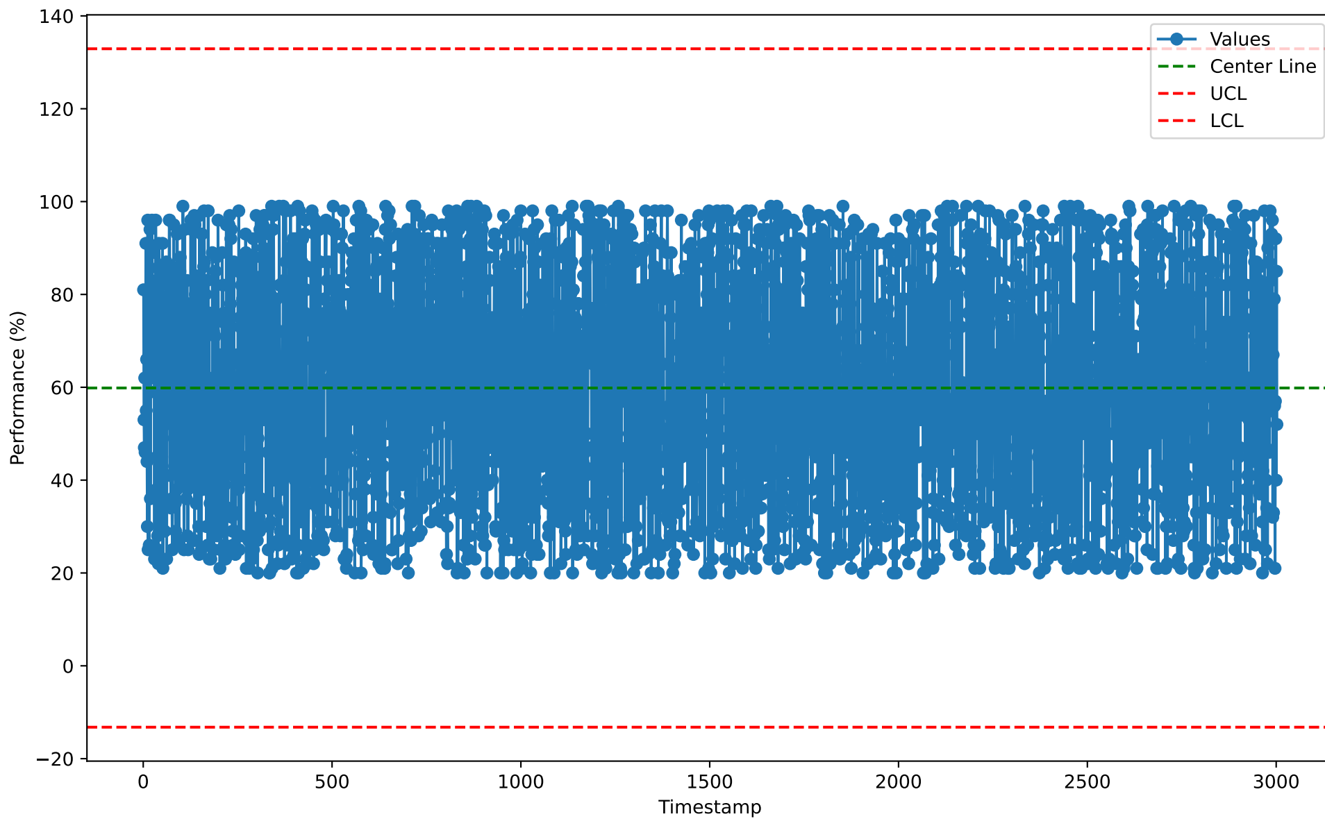
Individuals Chart for CIM10108 (2026-01-07)
