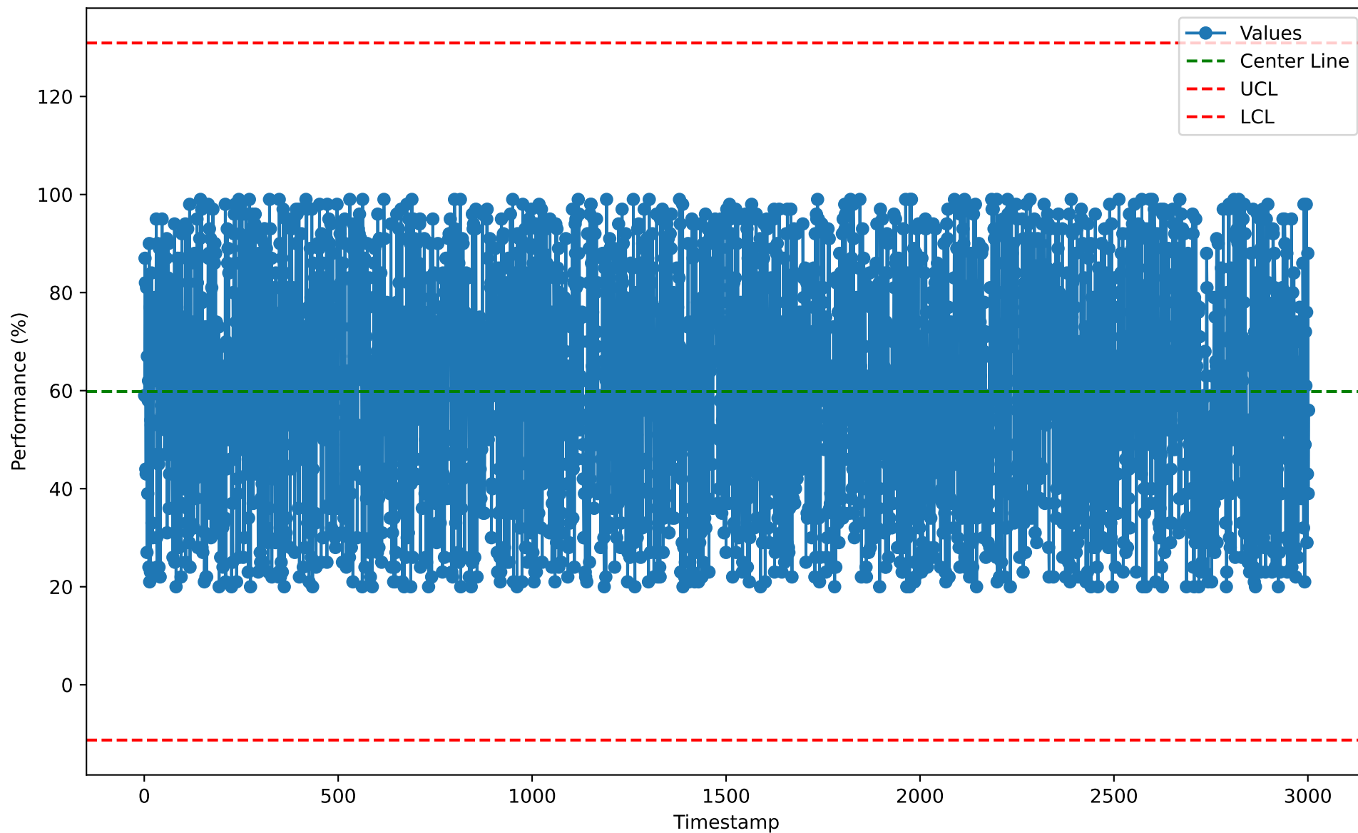
Individuals Chart for BIM10113 (2026-01-07)
