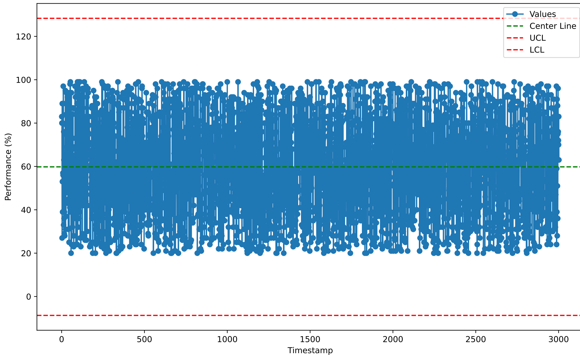
Individuals Chart for CFS10118 (2026-01-07)
