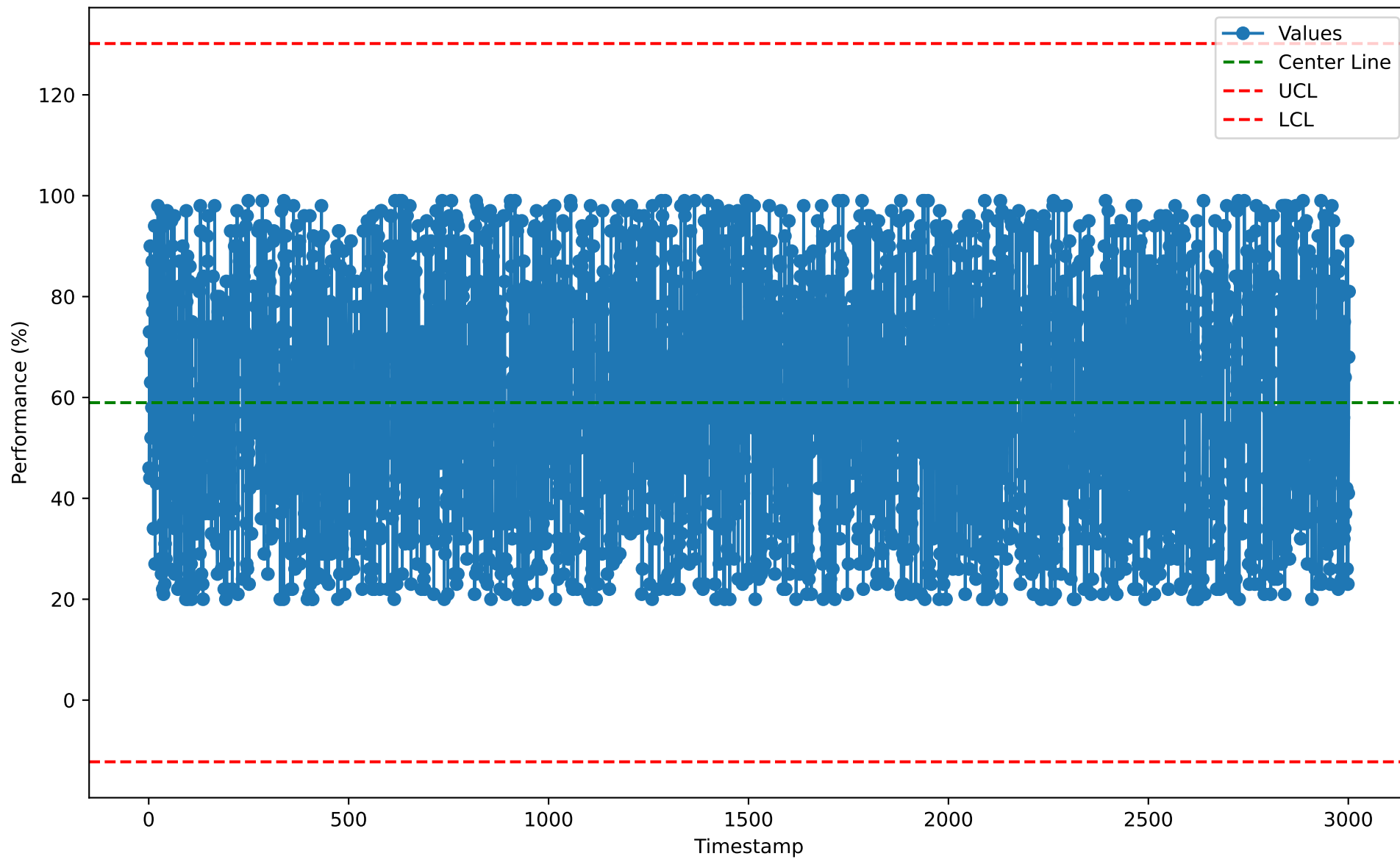
Individuals Chart for BIH10101 (2026-01-07)
