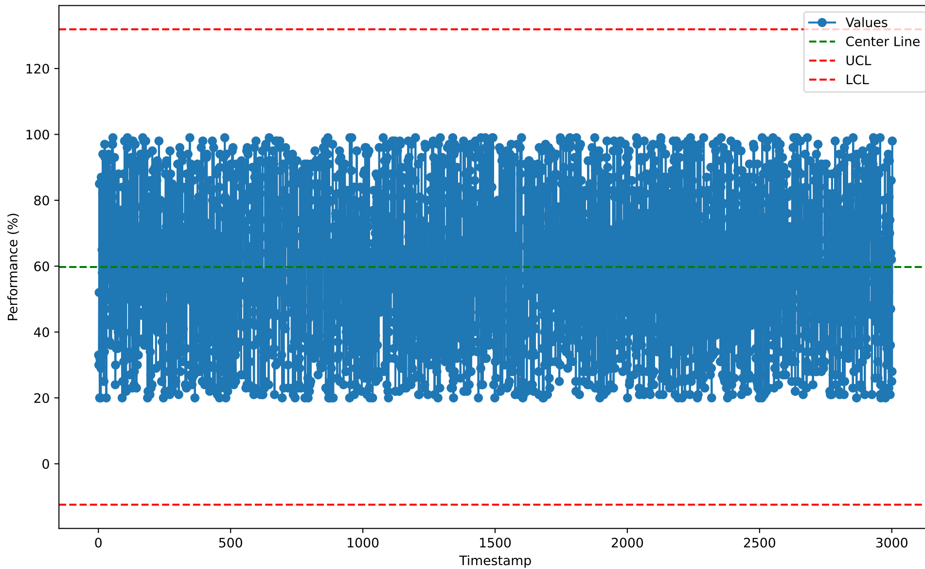
Individuals Chart for CIM10106 (2026-01-07)
