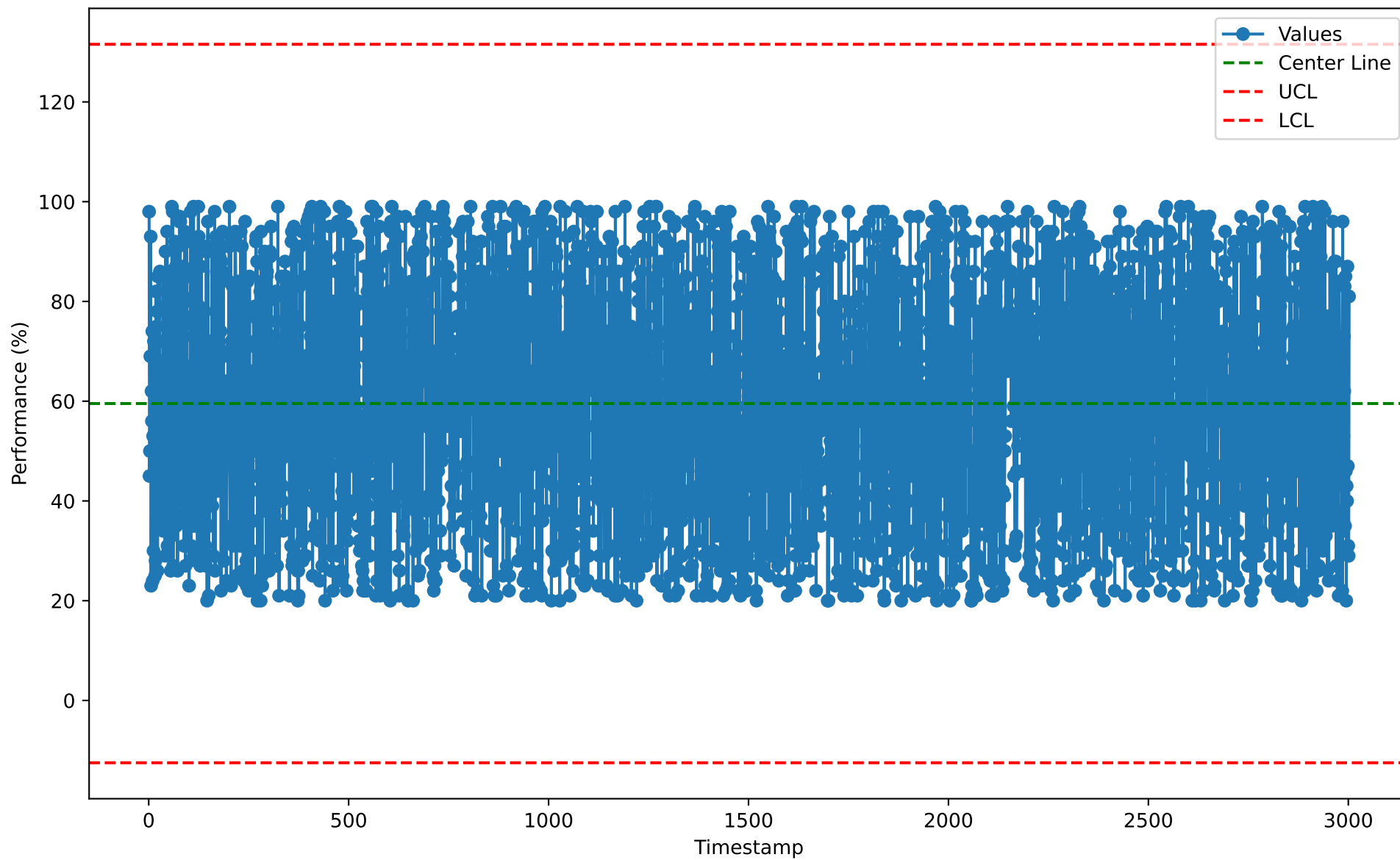
Individuals Chart for CIM10118 (2026-01-07)
