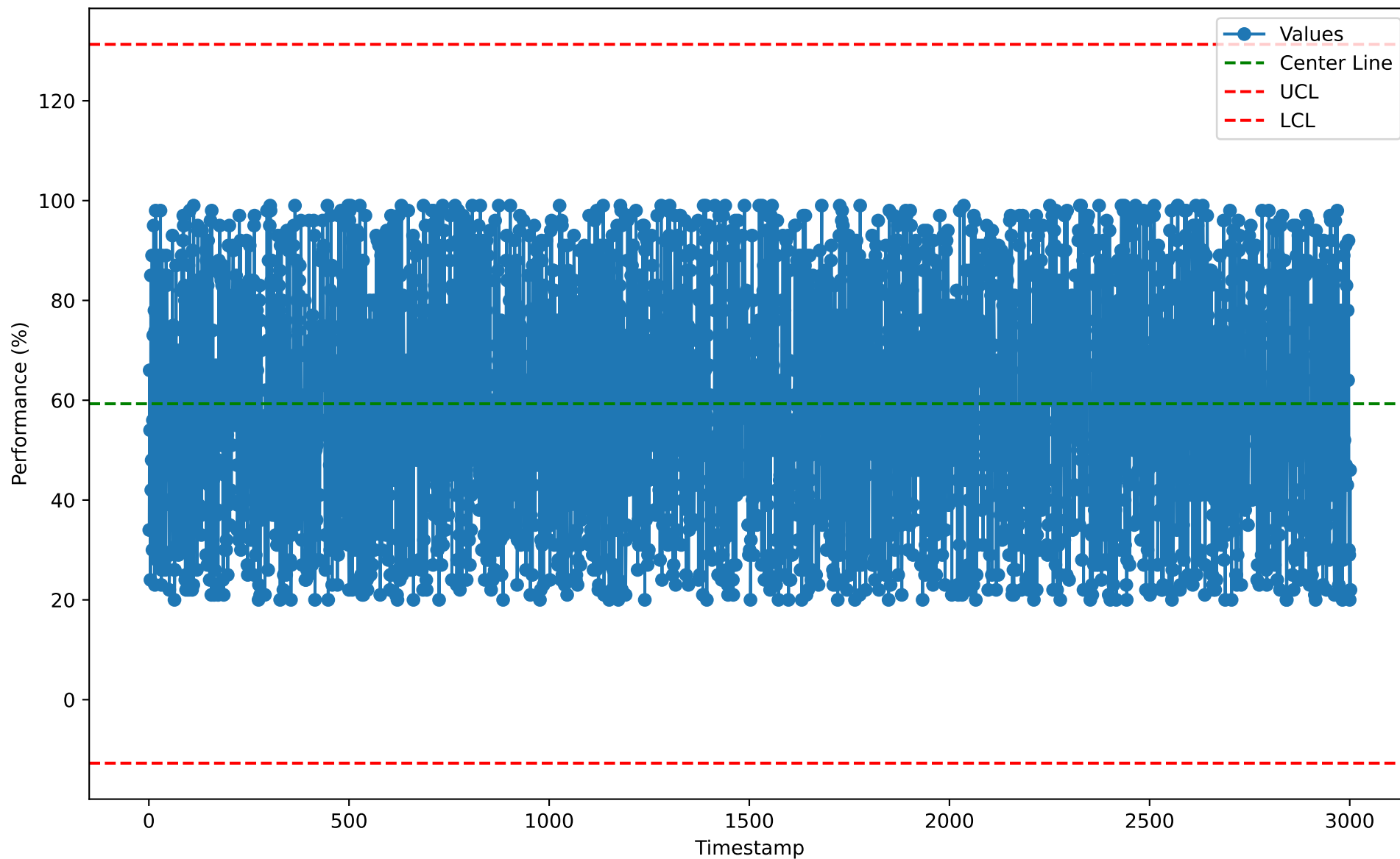
Individuals Chart for ITM10110 (2026-01-07)
