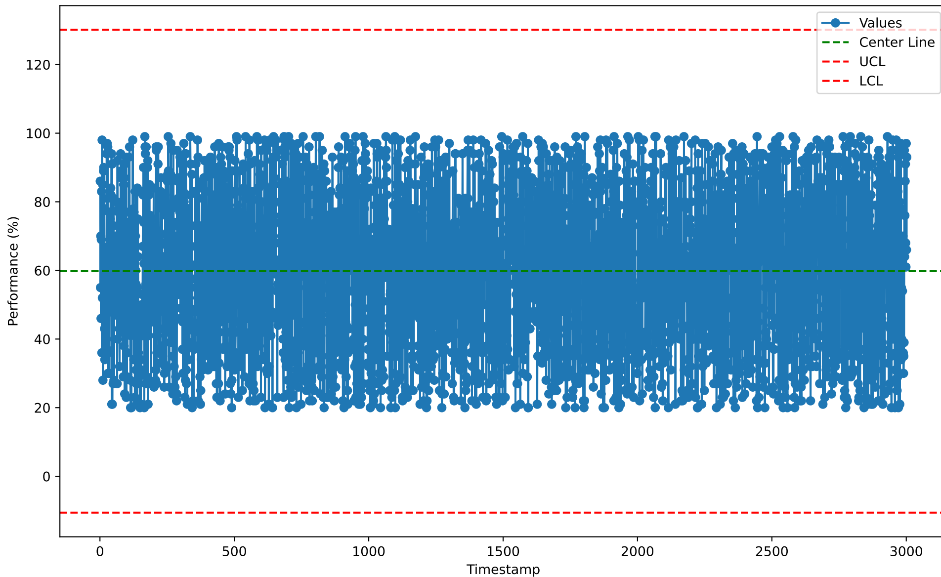
Individuals Chart for BIM10116 (2026-01-07)
