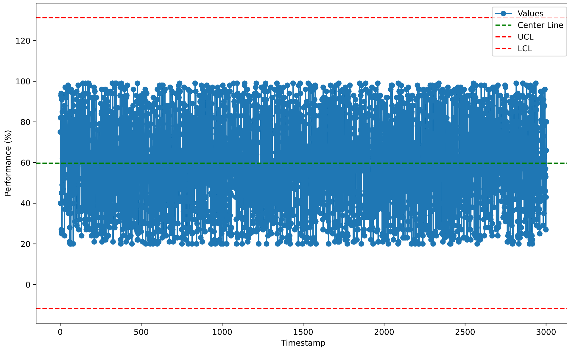
Individuals Chart for CII10111 (2026-01-07)
