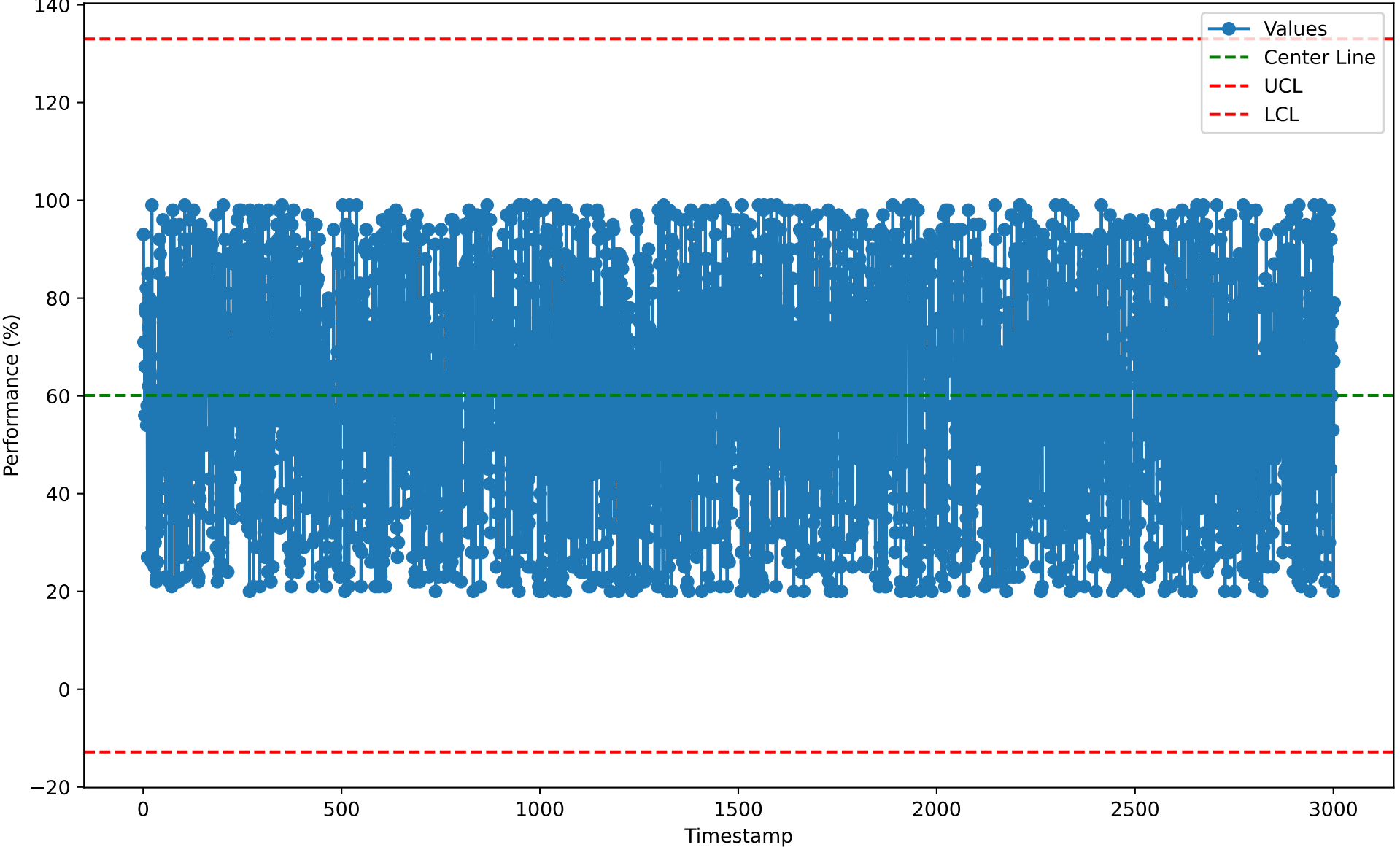
Individuals Chart for RTN10113 (2026-01-07)
