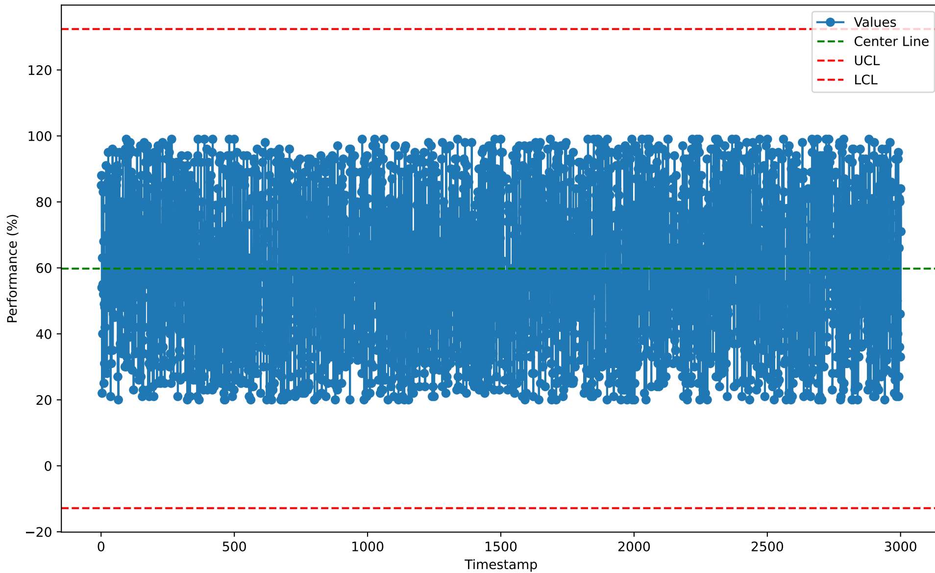
Individuals Chart for CIM10111 (2026-01-07)
