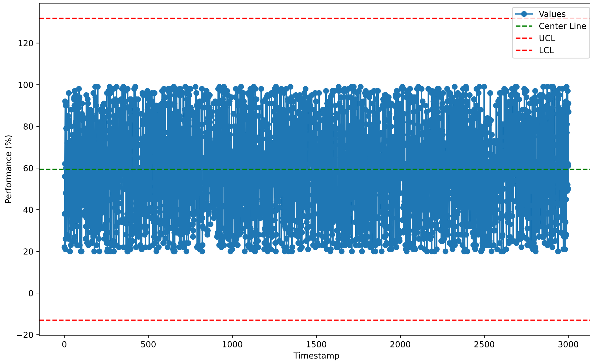
Individuals Chart for BIM10103 (2026-01-07)
