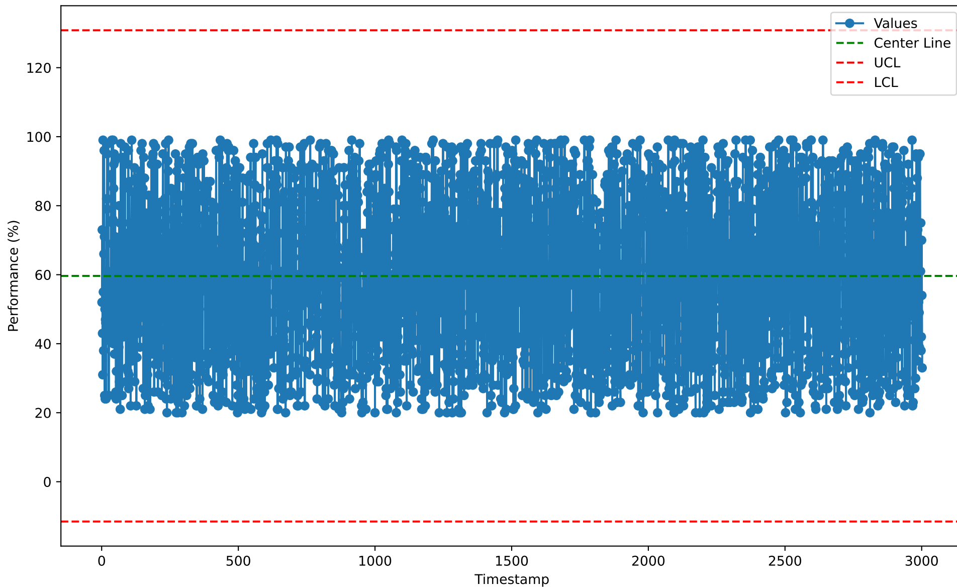
Individuals Chart for CIM10101 (2026-01-07)
