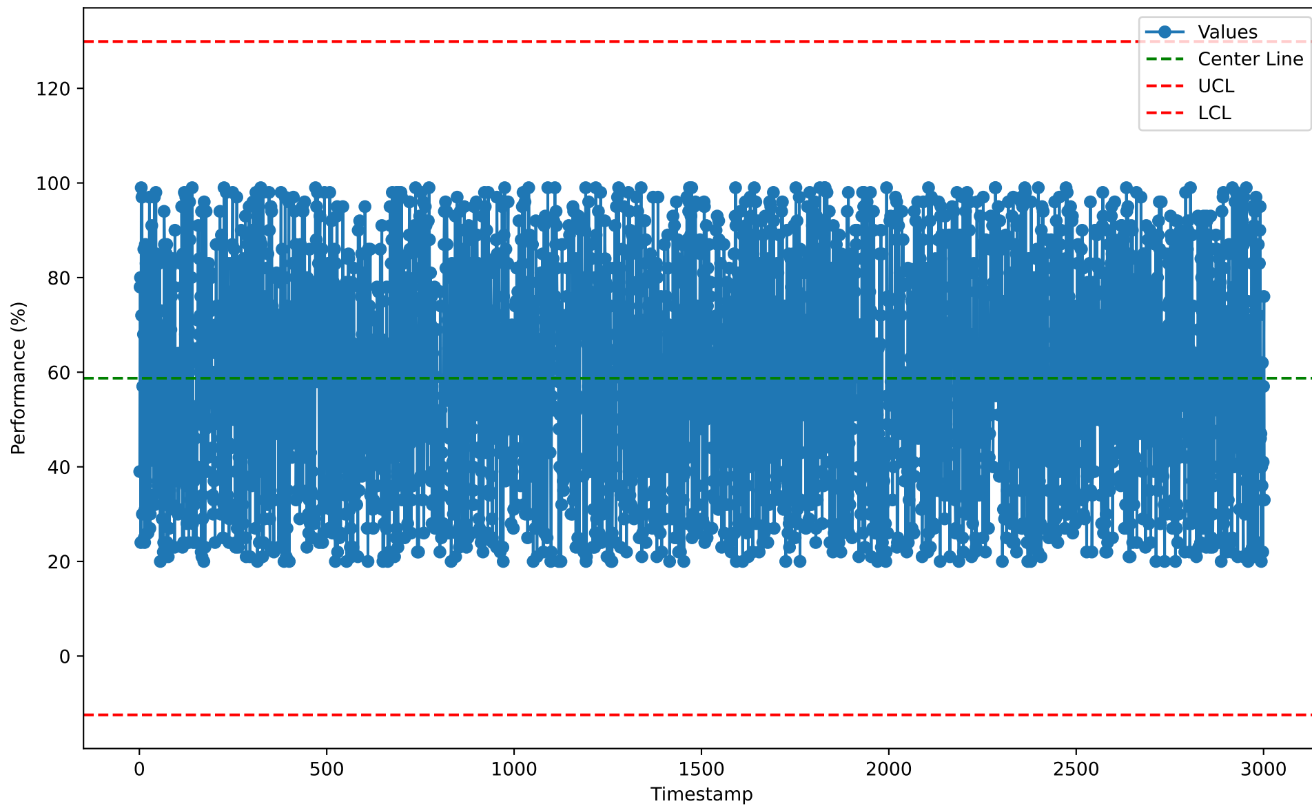
Individuals Chart for CIM10119 (2026-01-07)
