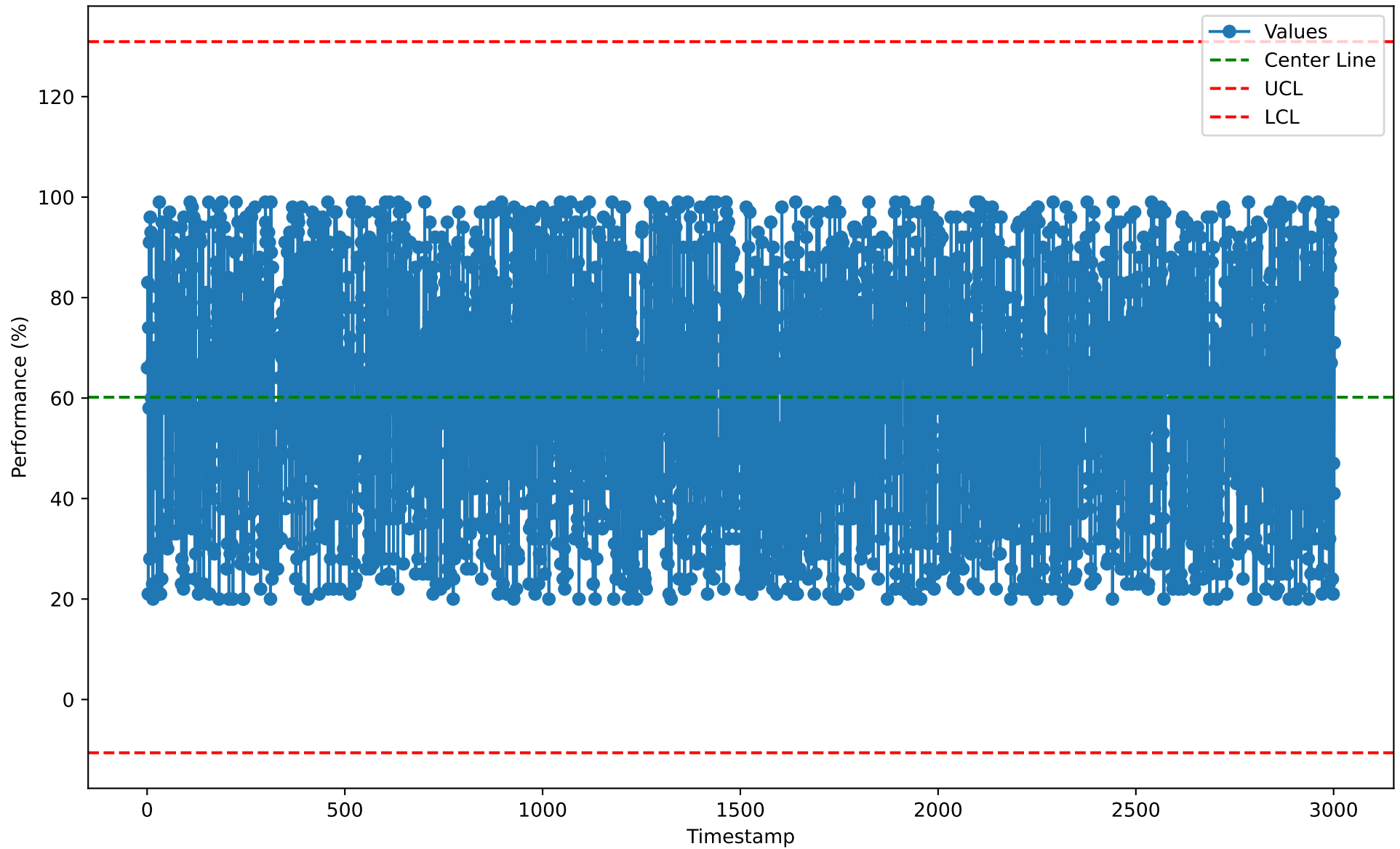
Individuals Chart for BIH10105 (2026-01-07)
