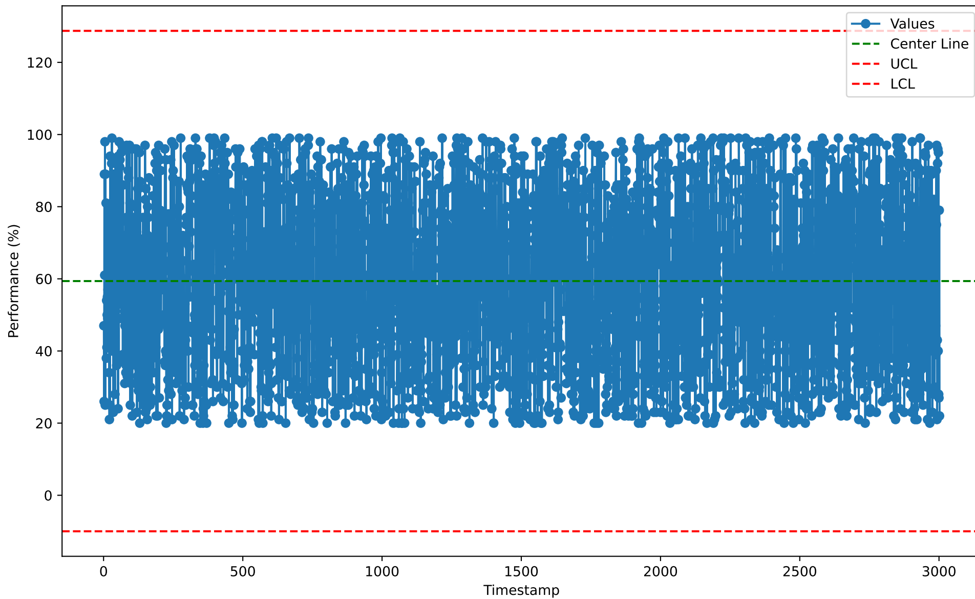
Individuals Chart for CIM10114 (2026-01-07)
