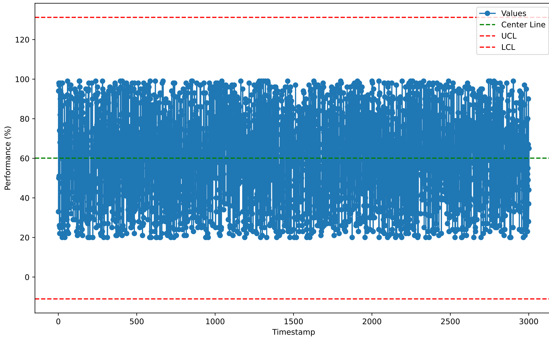
Individuals Chart for BIH10109 (2026-01-07)
