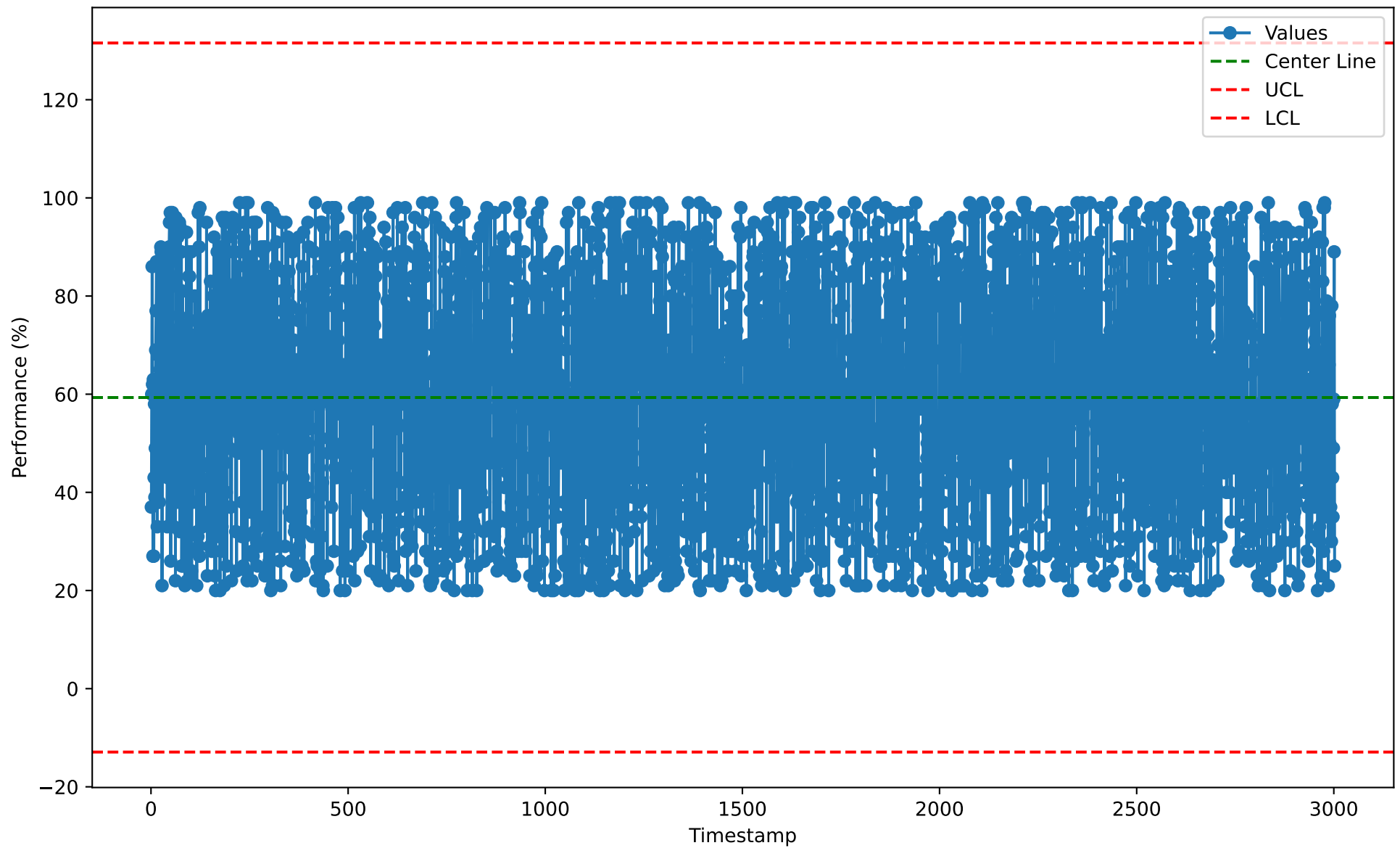
Individuals Chart for BIH10116 (2026-01-07)
