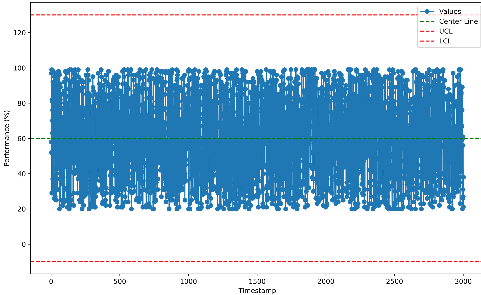
Individuals Chart for BIM10107 (2026-01-07)
