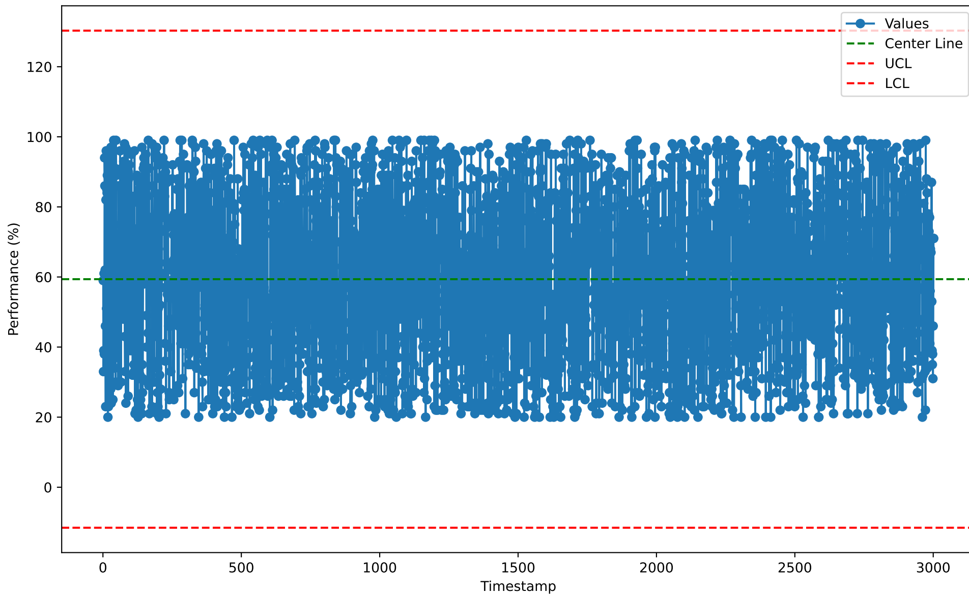
Individuals Chart for ITM10112 (2026-01-07)
