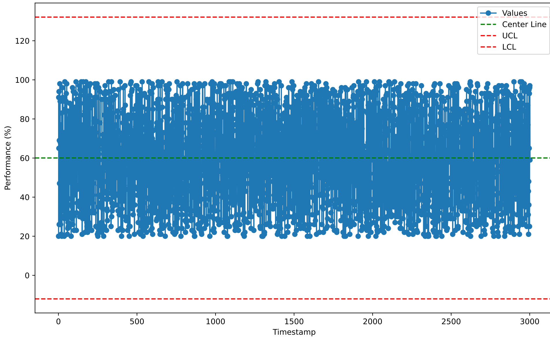
Individuals Chart for ITM10102 (2026-01-07)
