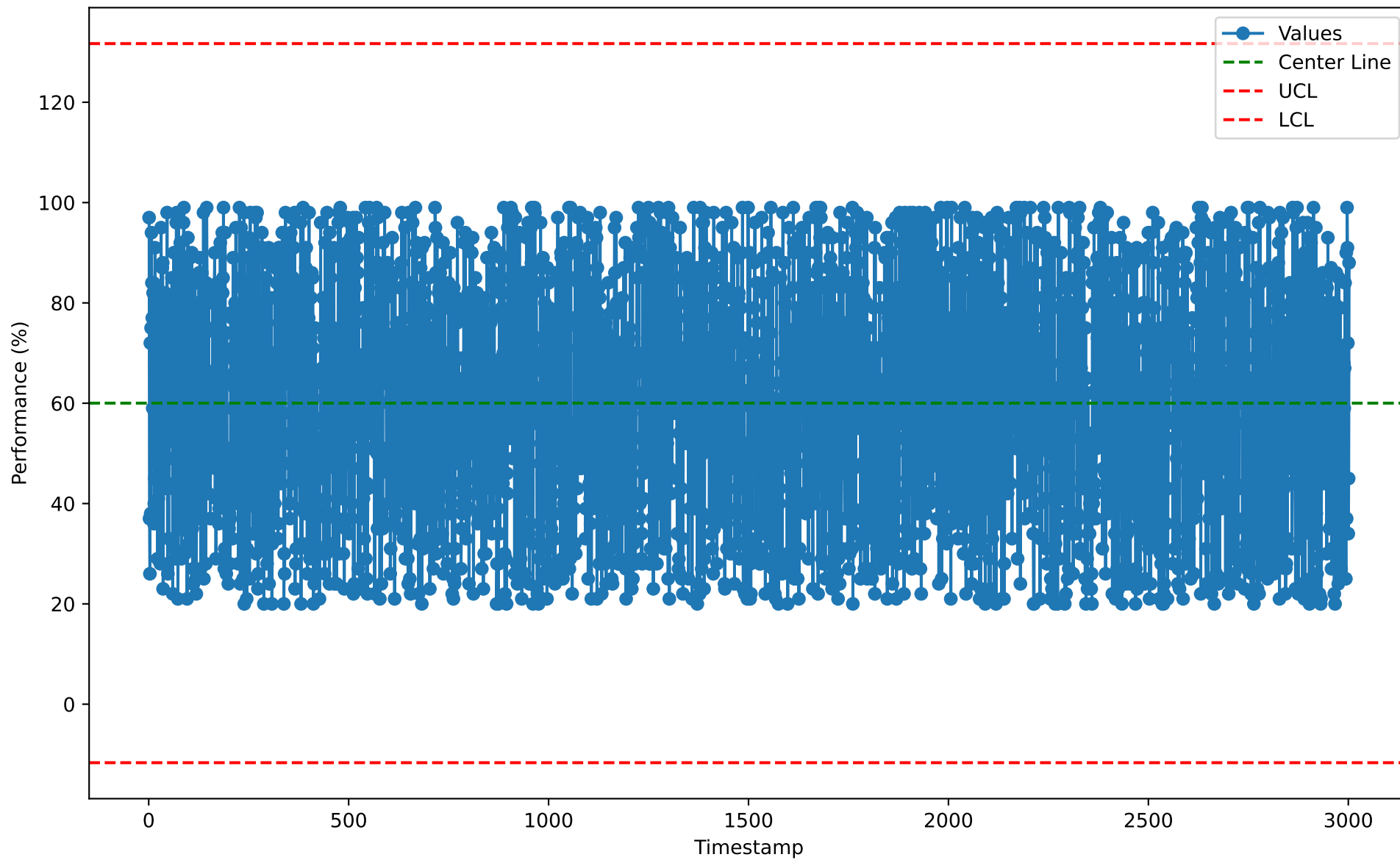
Individuals Chart for CII10114 (2026-01-07)
