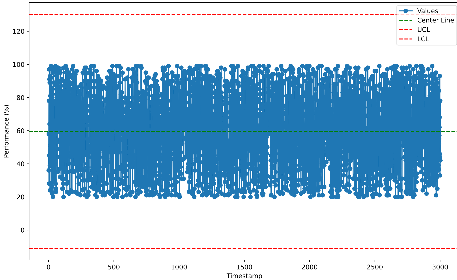
Individuals Chart for CFS10119 (2026-01-07)
