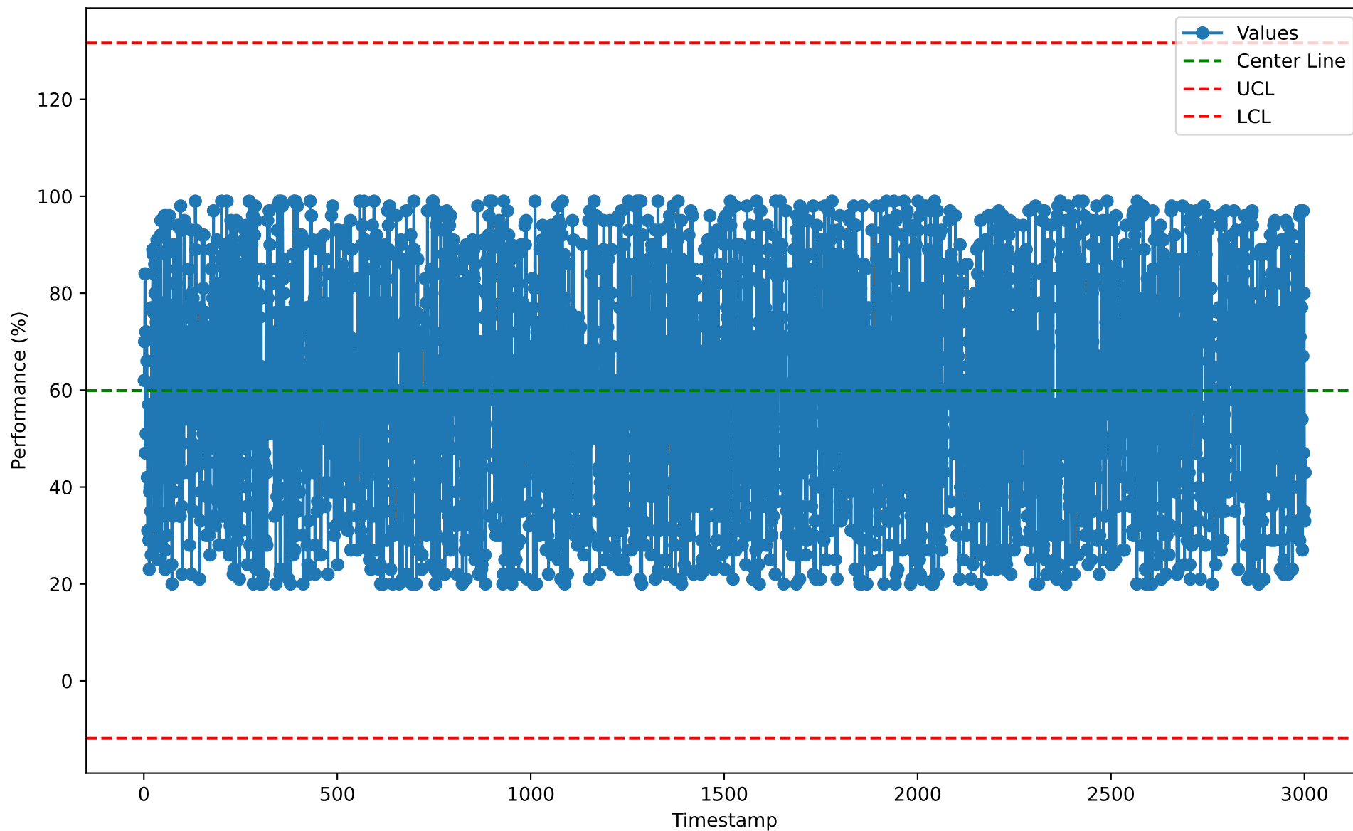
Individuals Chart for CIM10109 (2026-01-07)
