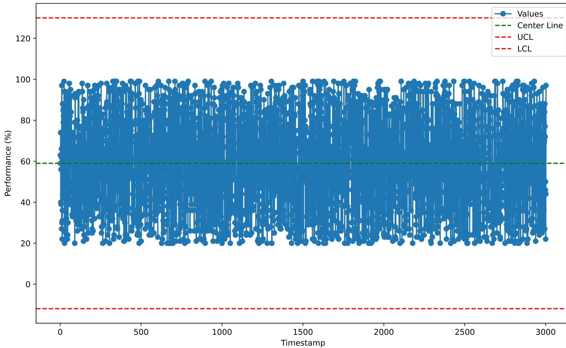
Individuals Chart for ITM10101 (2026-01-07)
