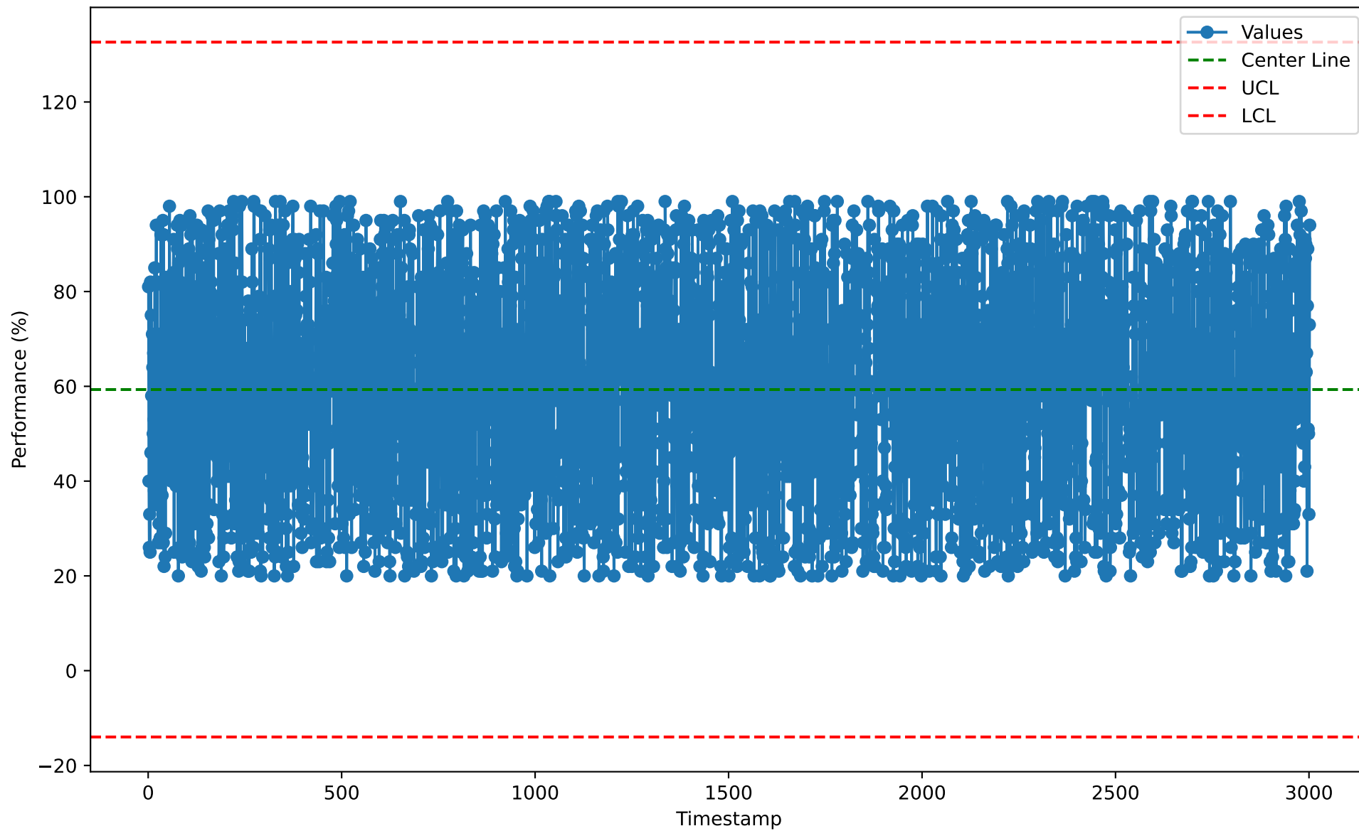
Individuals Chart for BIM10118 (2026-01-07)
