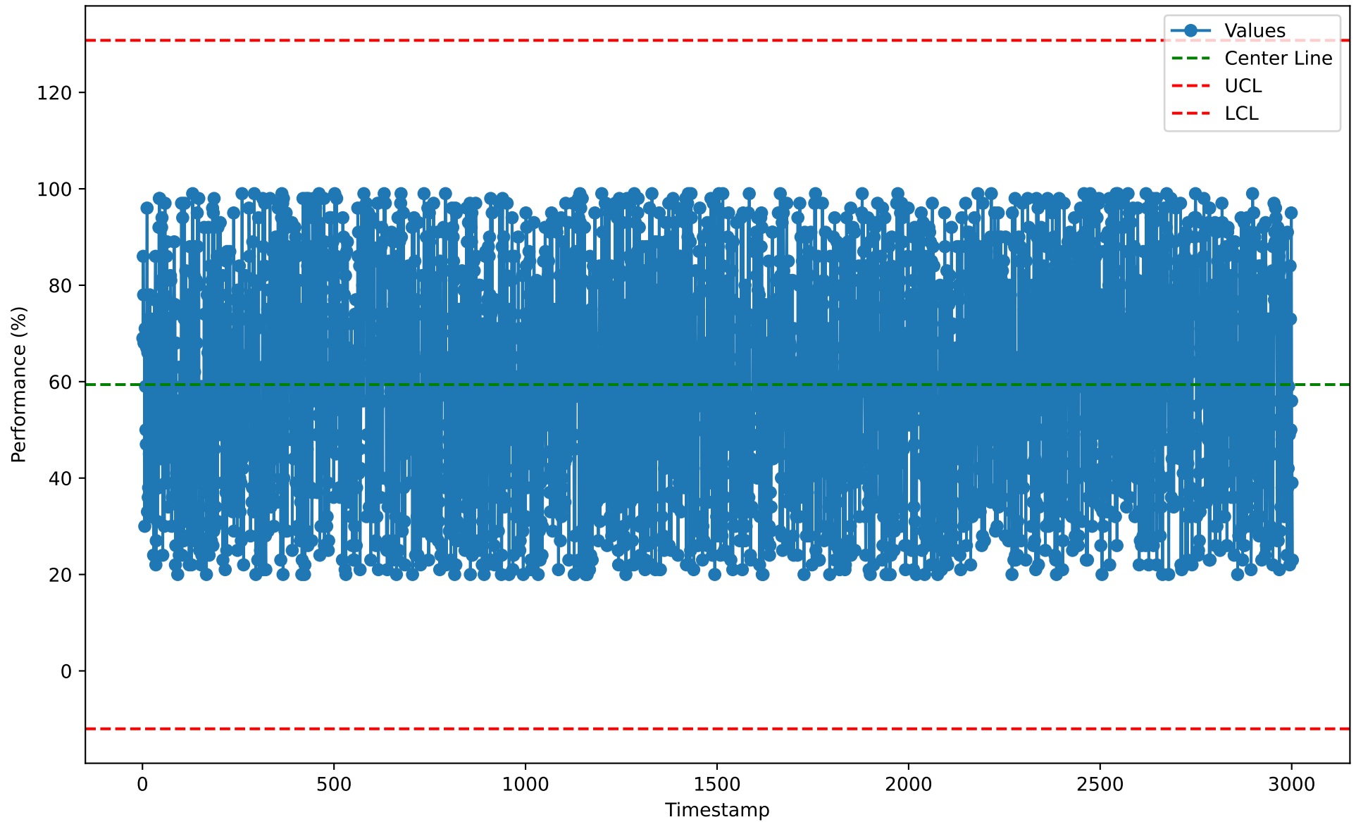
Individuals Chart for ITM10104 (2026-01-07)
