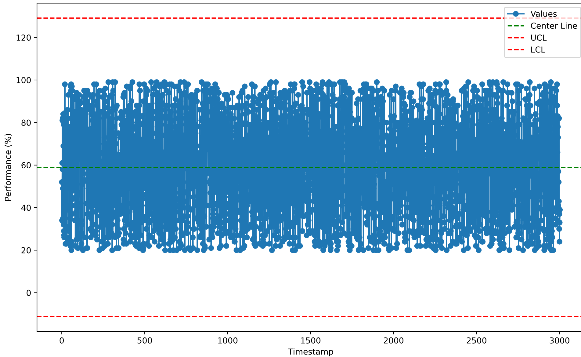
Individuals Chart for CII10110 (2026-01-07)
