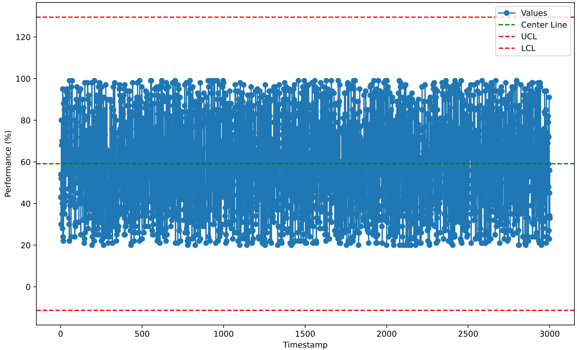
Individuals Chart for BIH10103 (2026-01-07)
