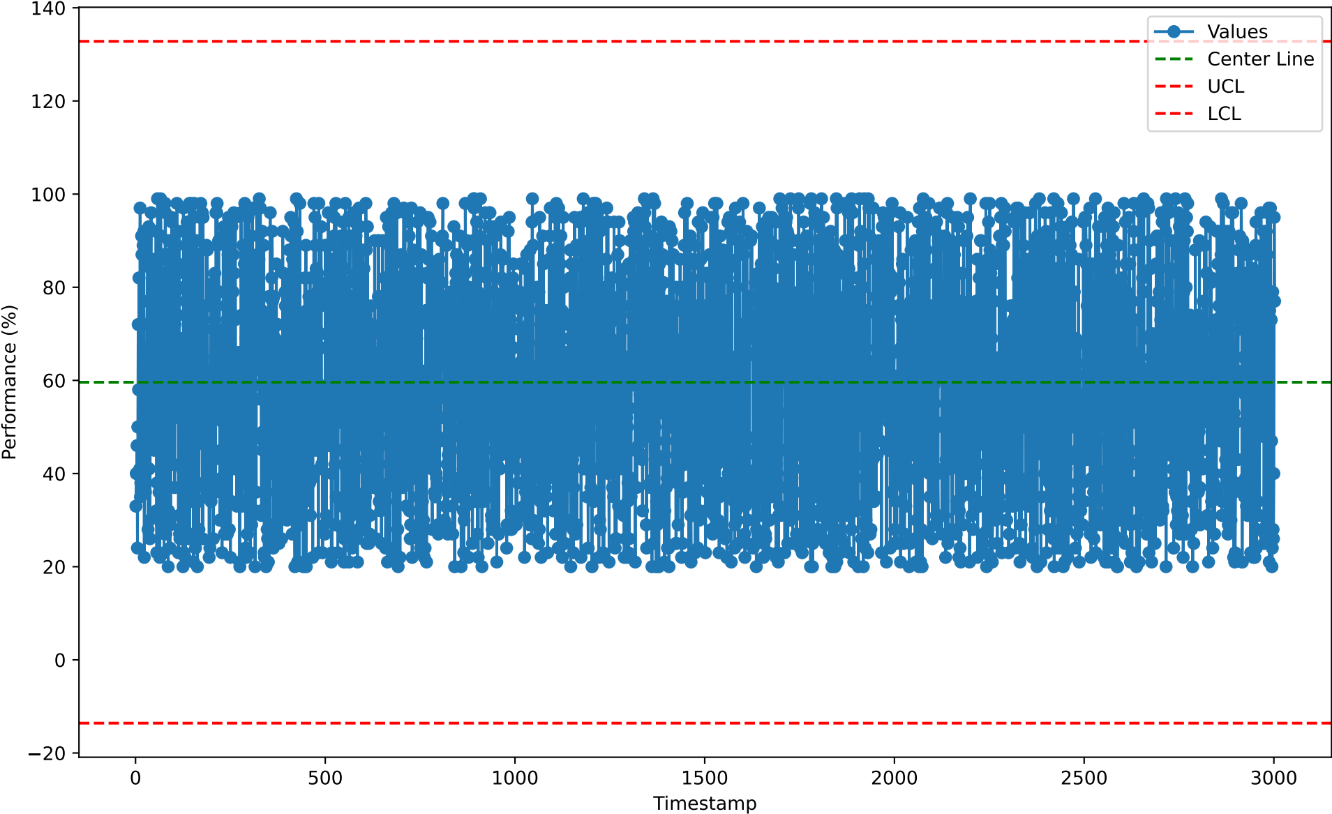
Individuals Chart for RTN10116 (2026-01-07)
