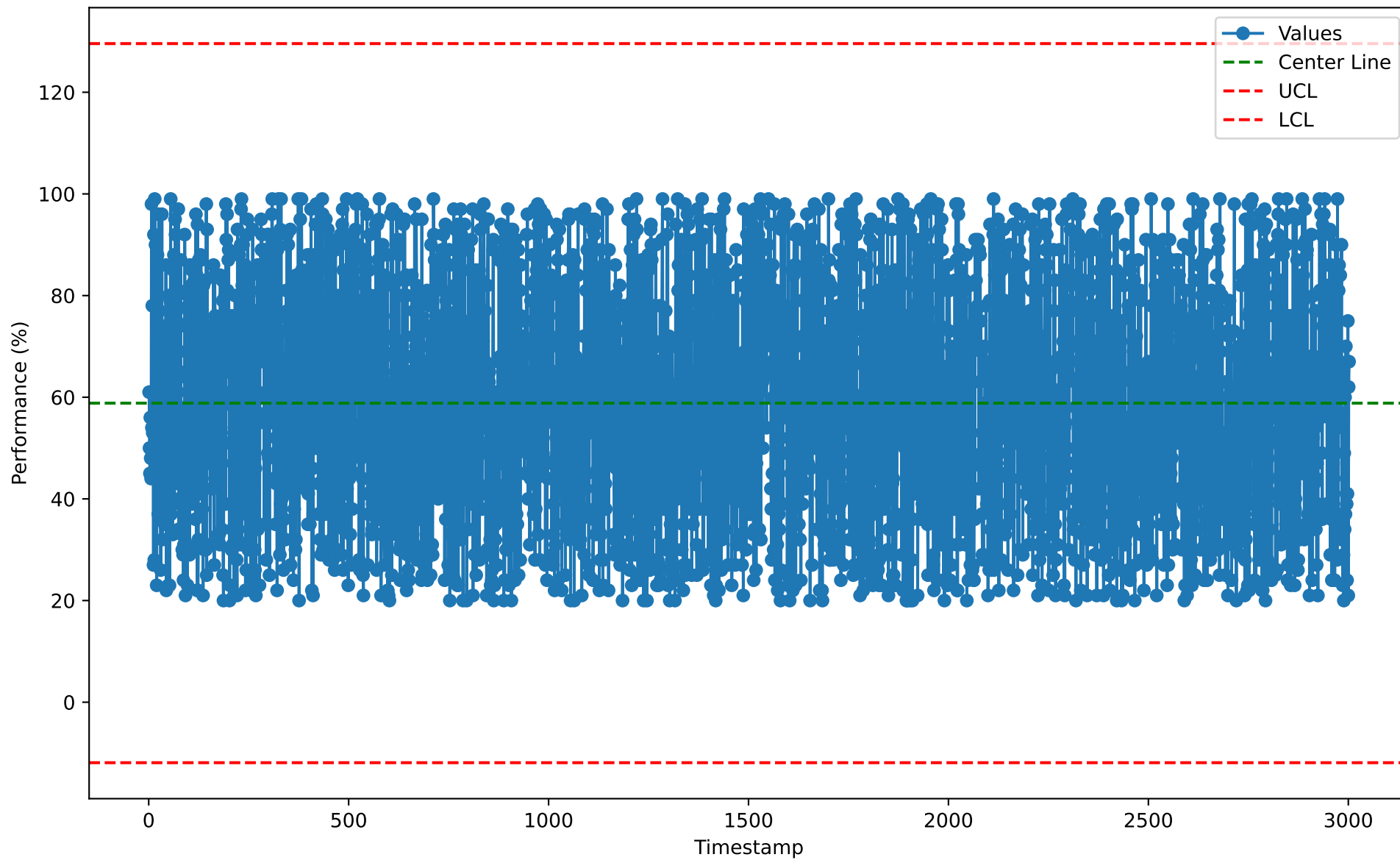
Individuals Chart for BIM10101 (2026-01-07)
