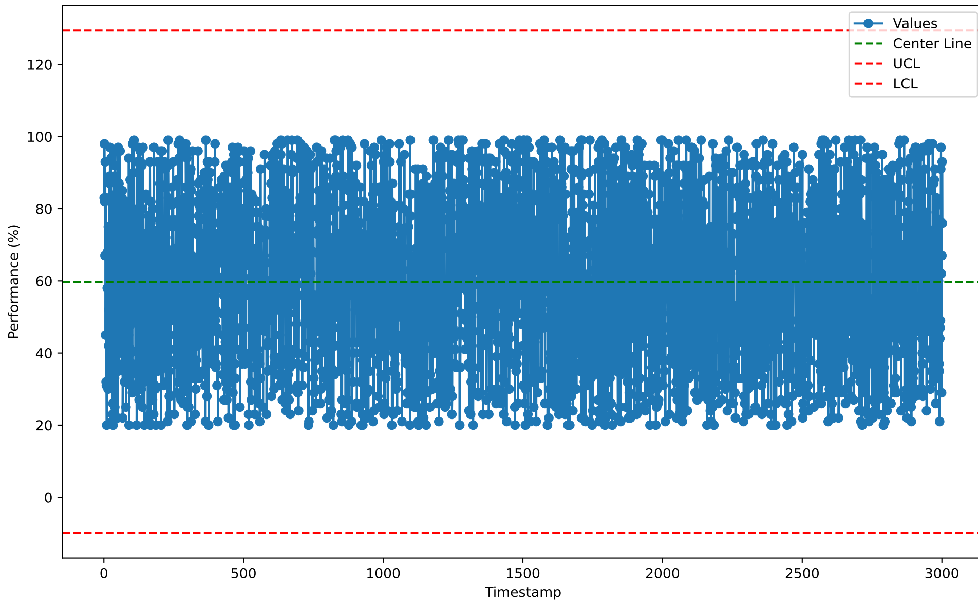
Individuals Chart for CII10102 (2026-01-07)
