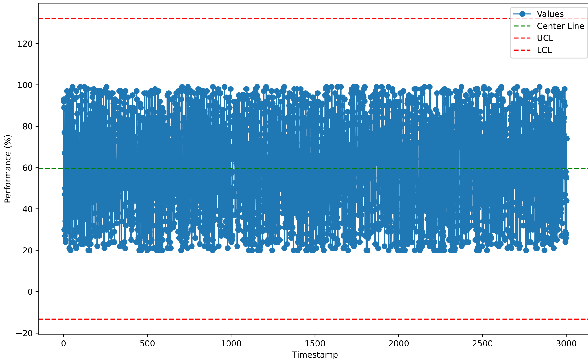
Individuals Chart for CIM10116 (2026-01-07)
