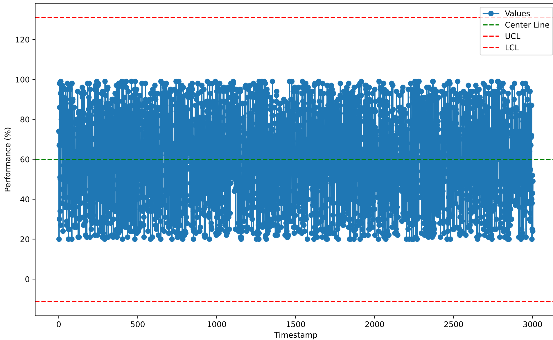
Individuals Chart for CIM10110 (2026-01-07)
