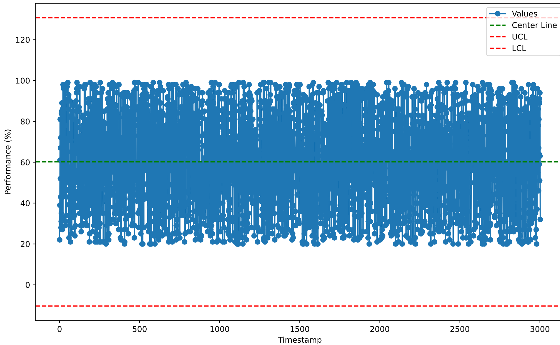
Individuals Chart for CII10112 (2026-01-07)
