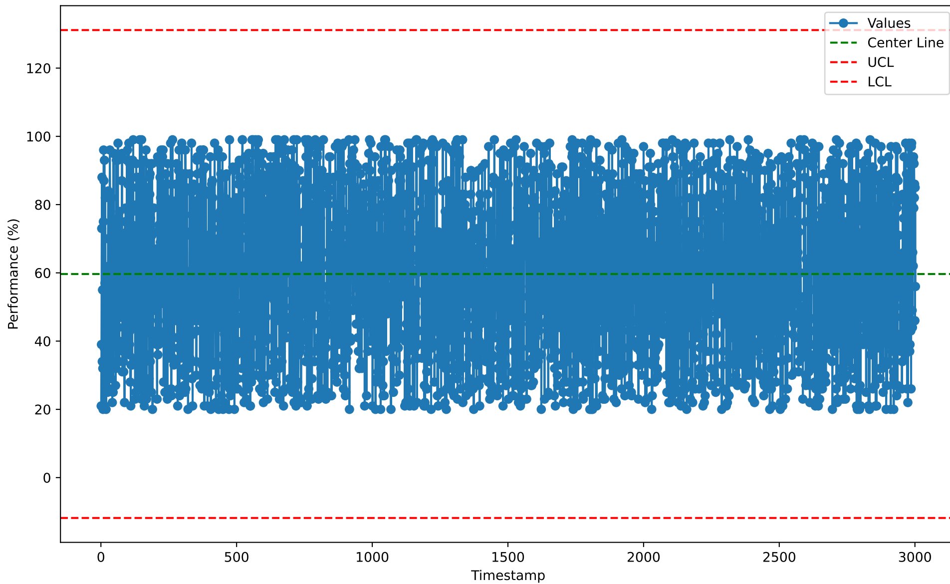
Individuals Chart for BIM10114 (2026-01-07)
