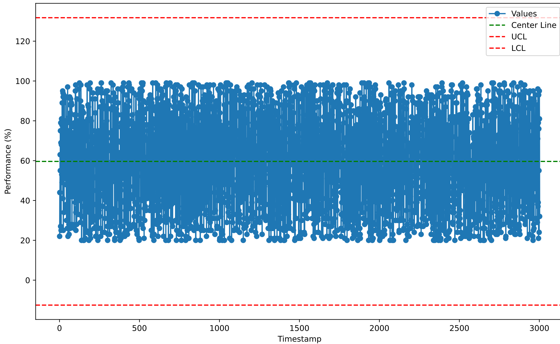
Individuals Chart for CII10104 (2026-01-07)
