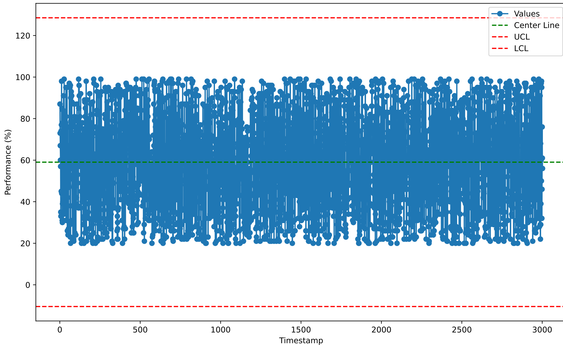
Individuals Chart for ITM10113 (2026-01-07)
