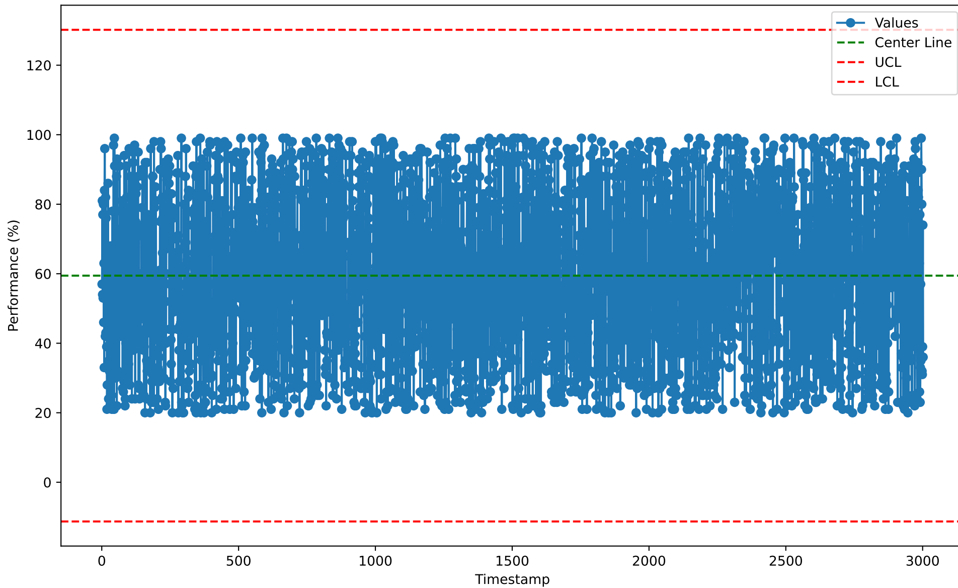
Individuals Chart for CFS10116 (2026-01-07)
