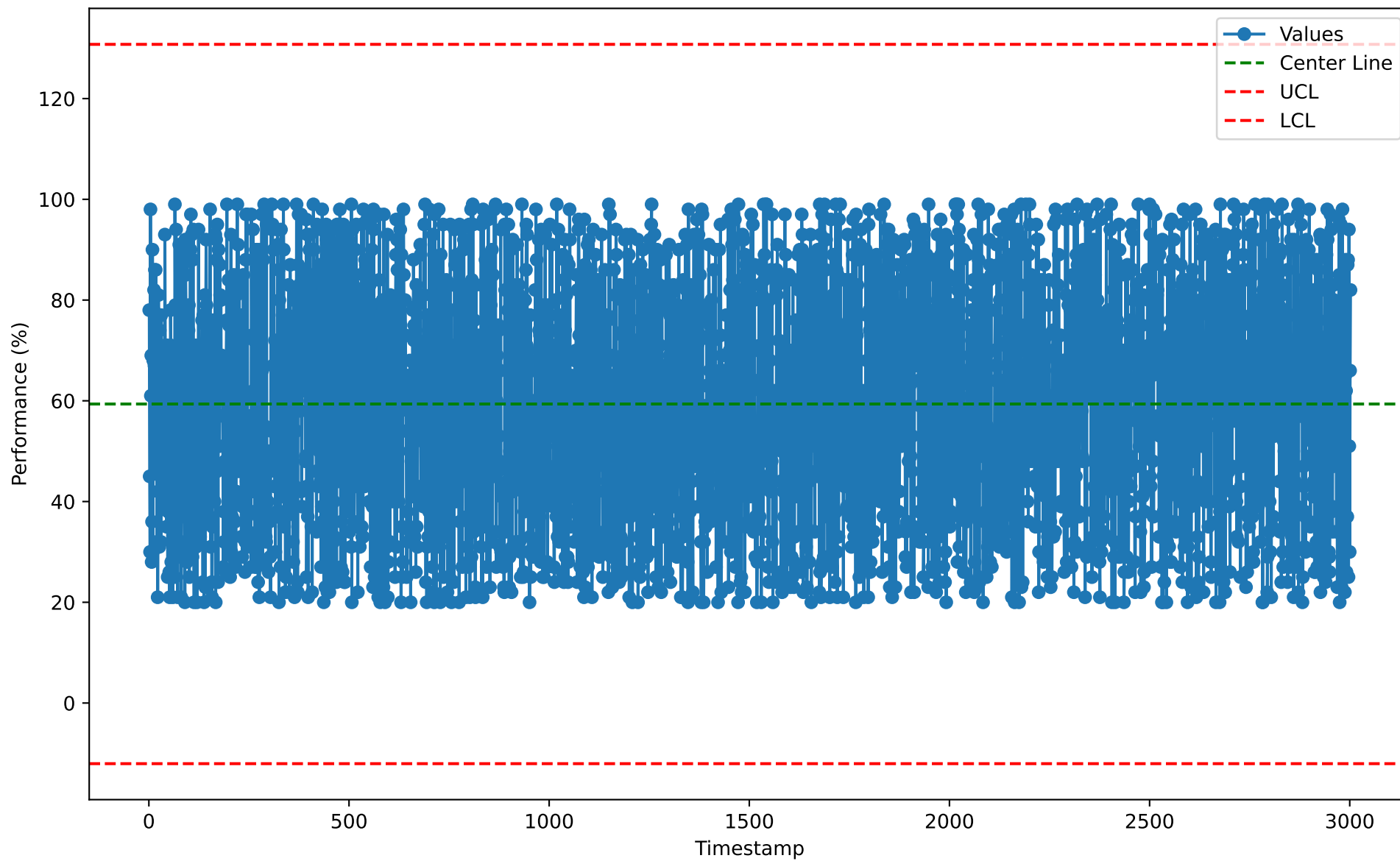
Individuals Chart for CII10119 (2026-01-07)
