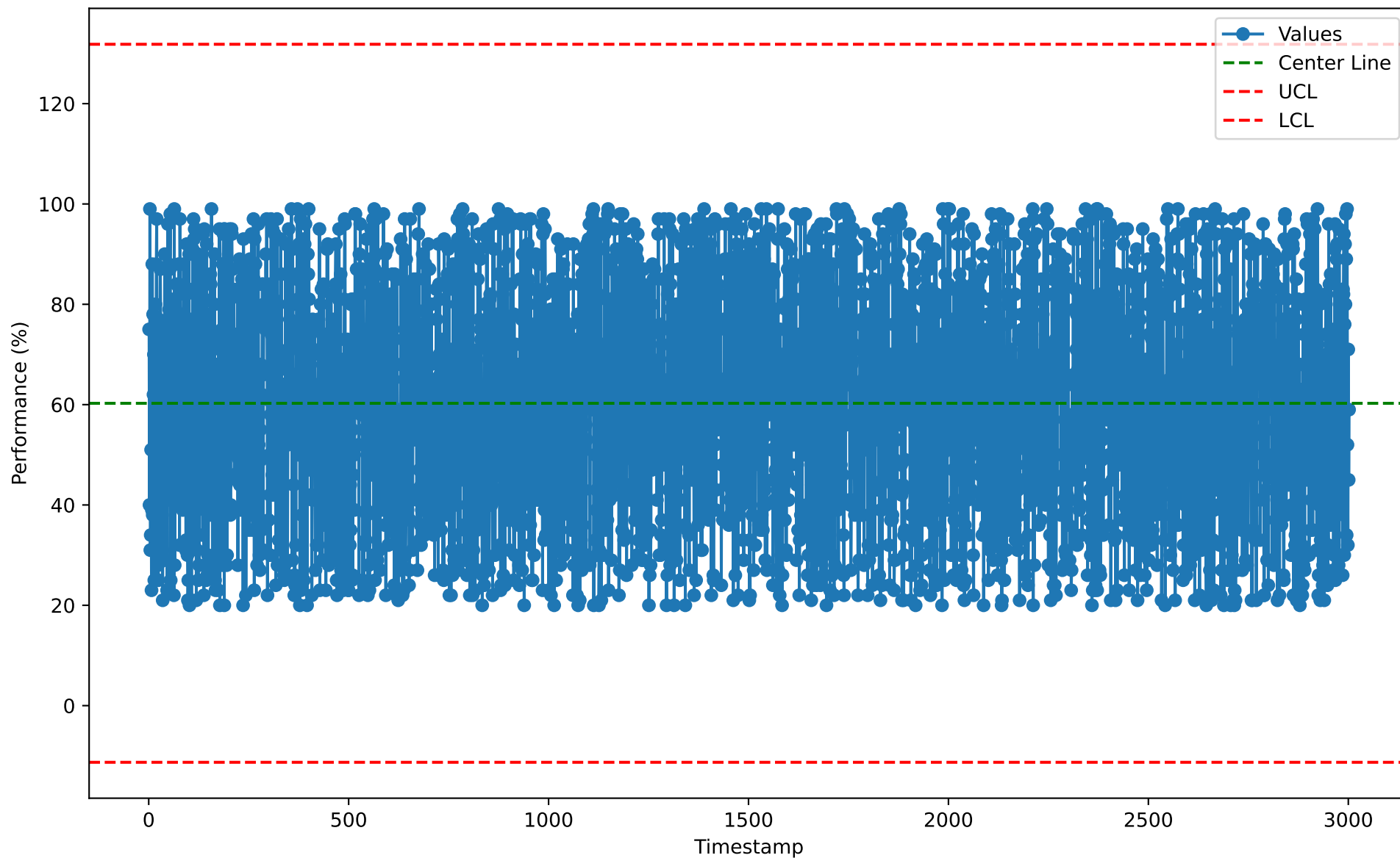
Individuals Chart for ITM10119 (2026-01-07)
