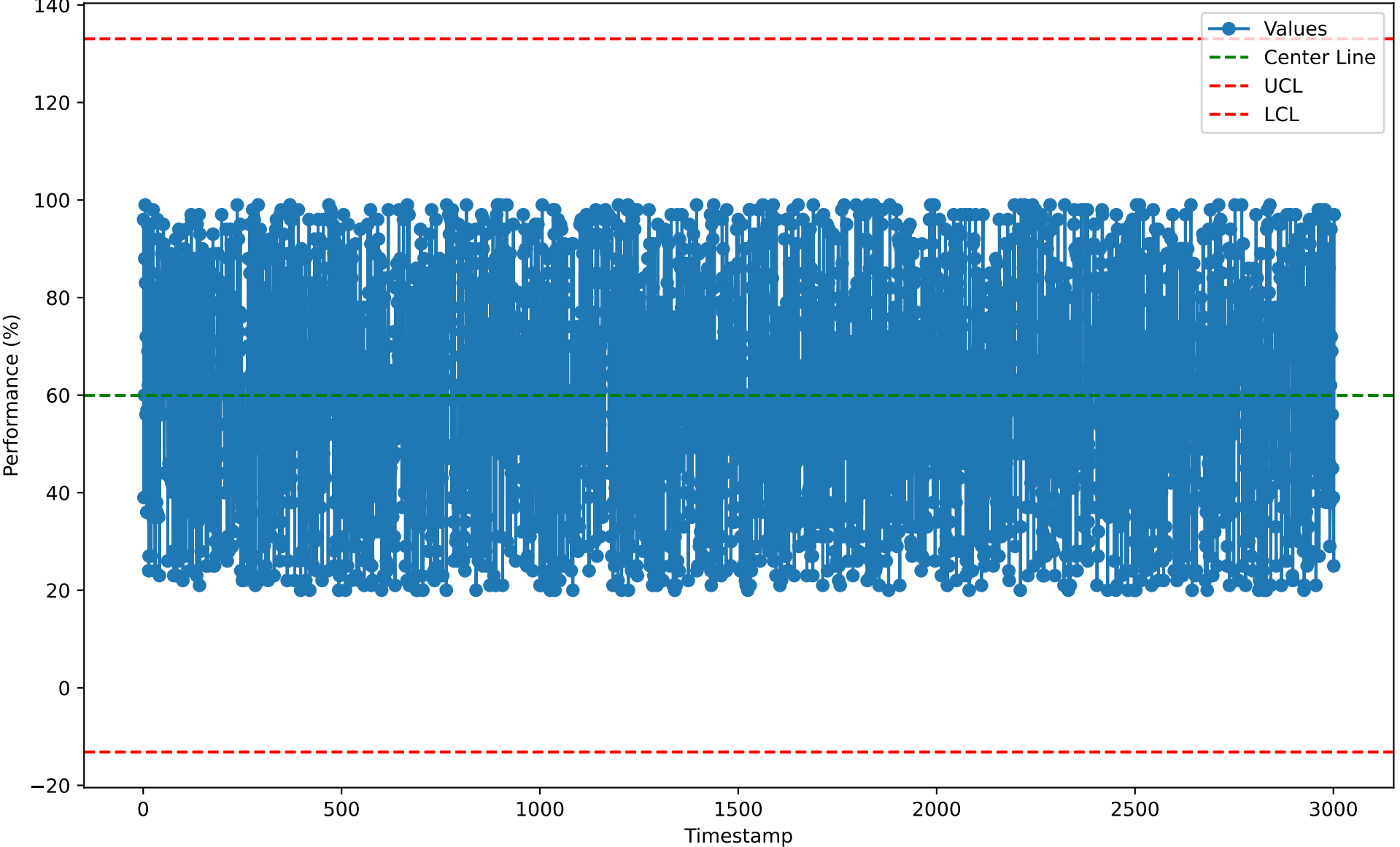
Individuals Chart for CHG10108 (2026-01-07)
