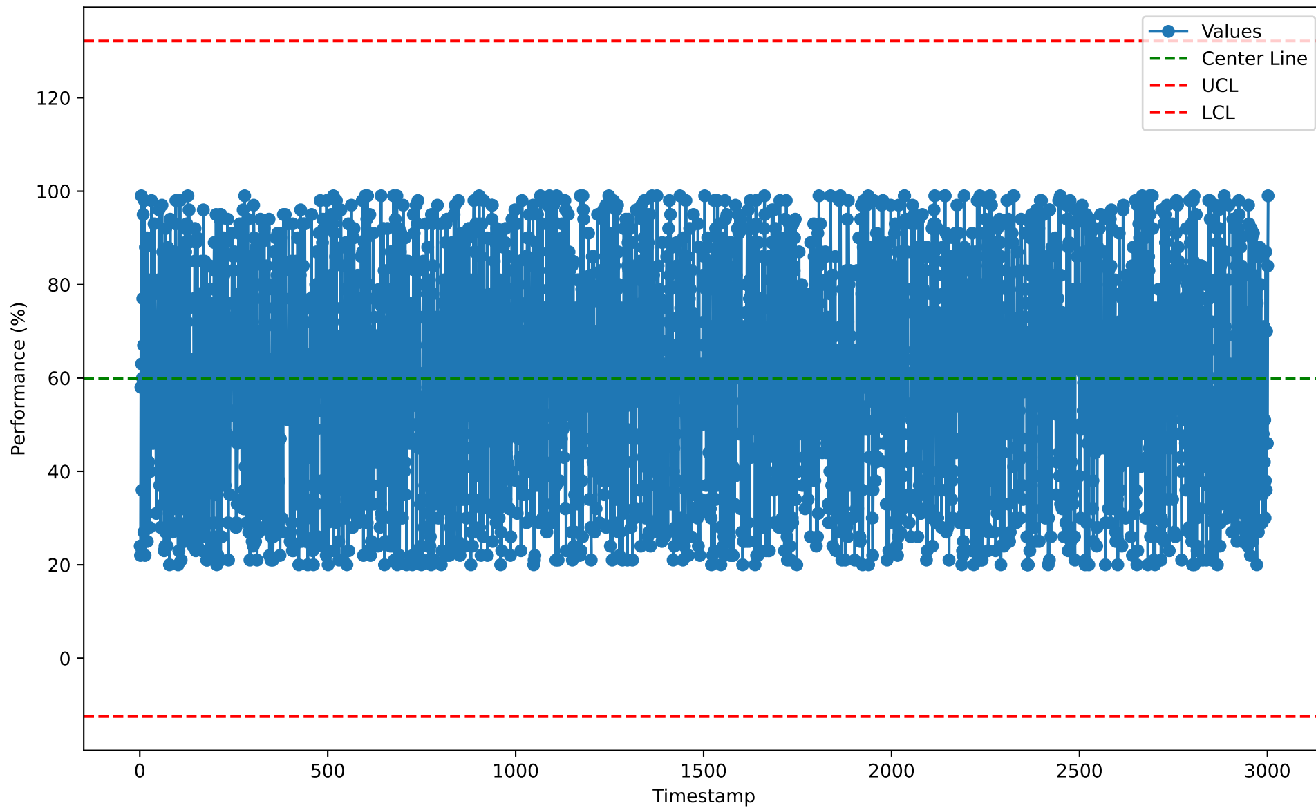
Individuals Chart for ITM10117 (2026-01-07)
