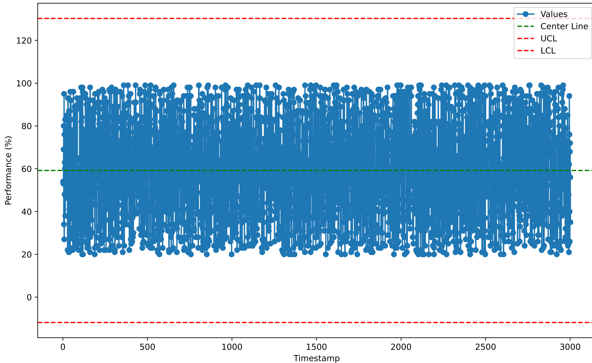
Individuals Chart for CII10117 (2026-01-07)
