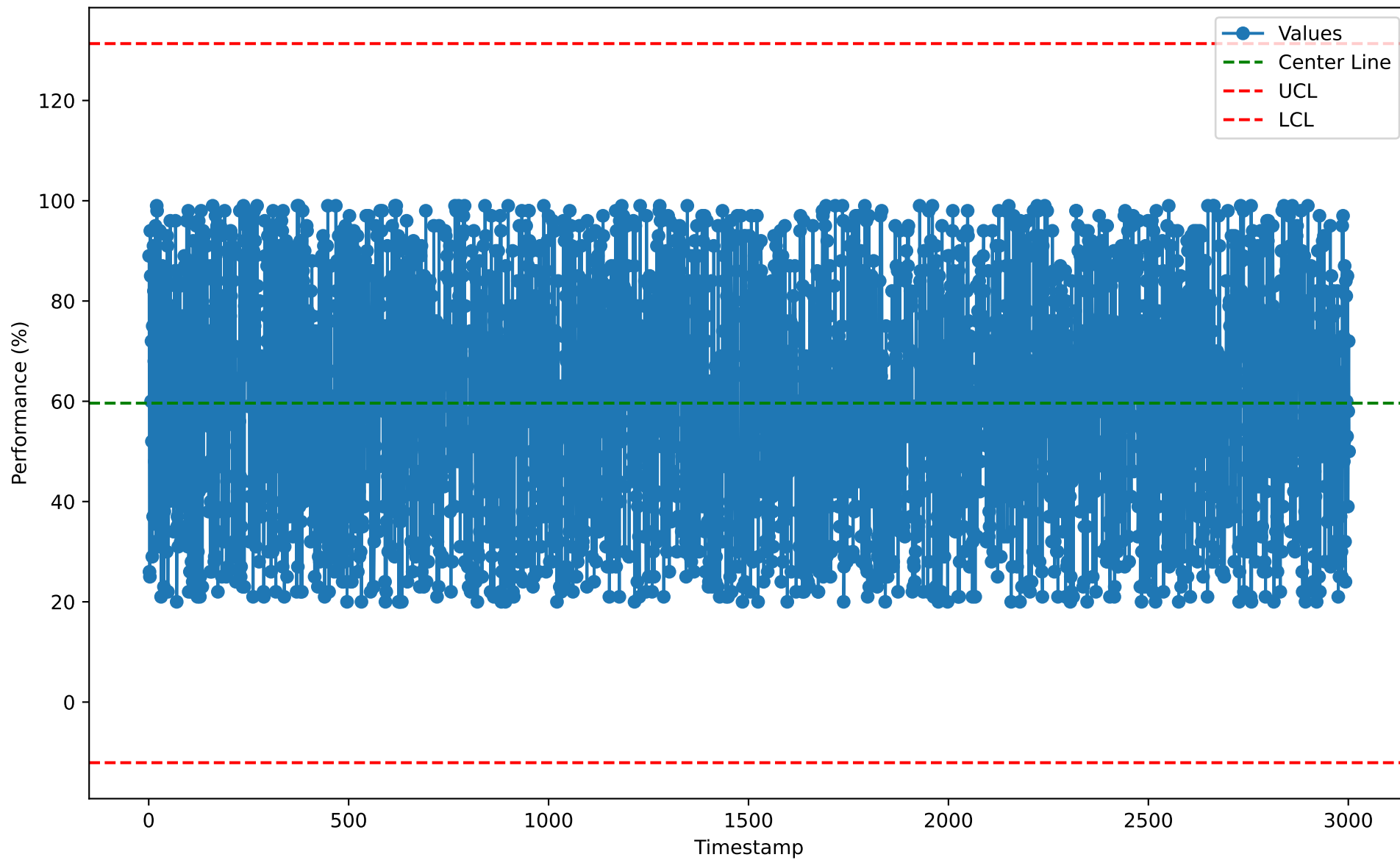
Individuals Chart for CII10115 (2026-01-07)
