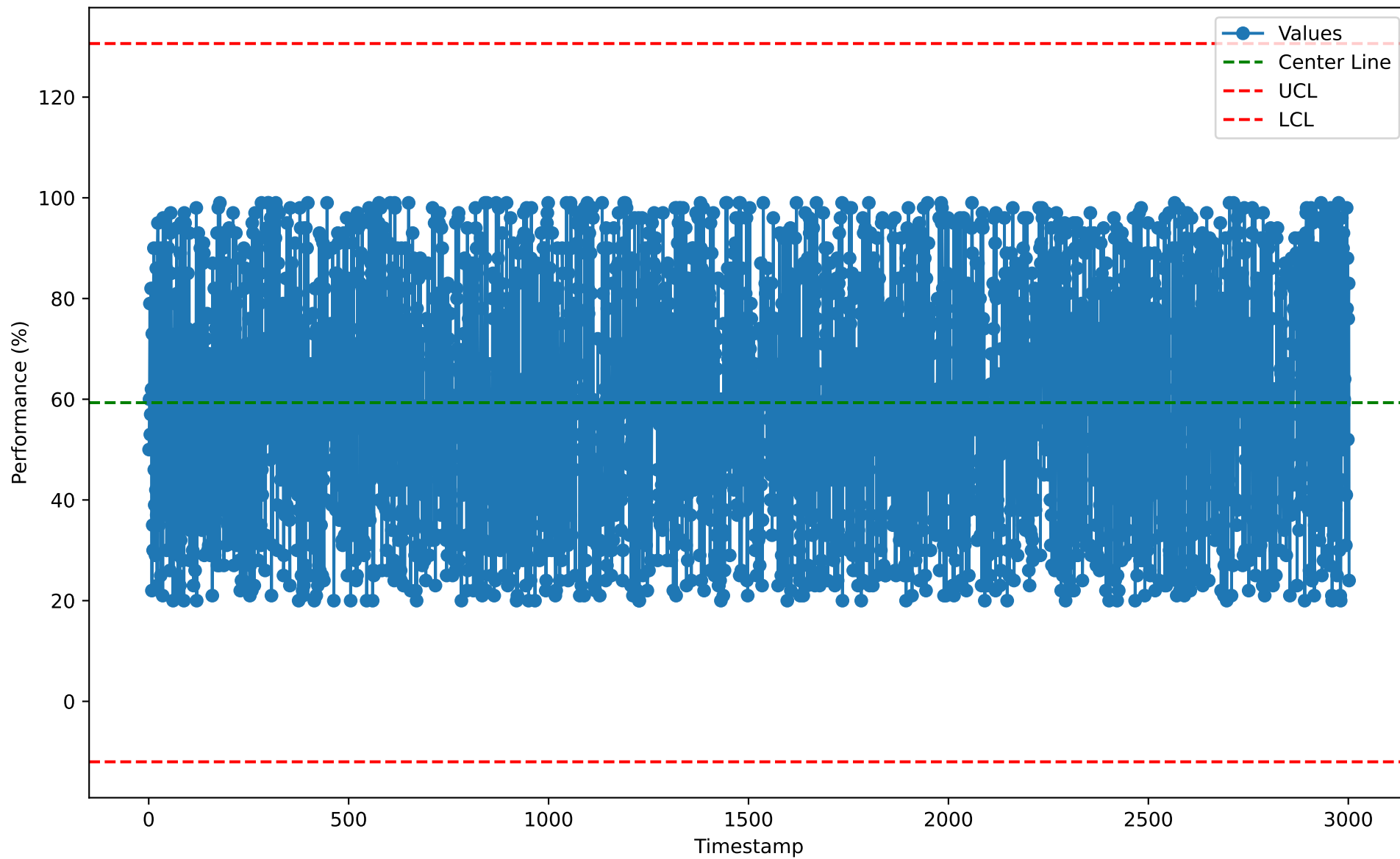
Individuals Chart for CFS10117 (2026-01-07)
