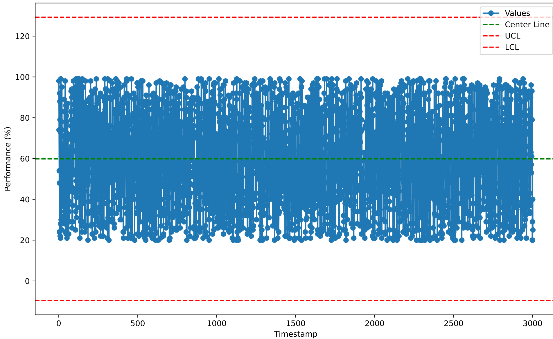
Individuals Chart for CFS10109 (2026-01-07)
