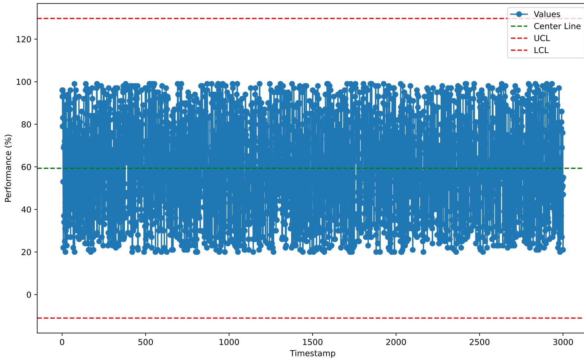
Individuals Chart for BIM10117 (2026-01-07)
