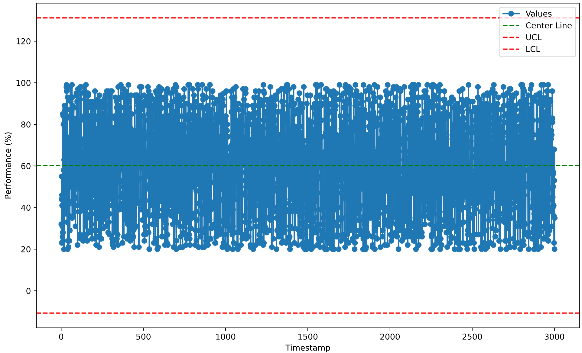
Individuals Chart for BIH10110 (2026-01-07)
