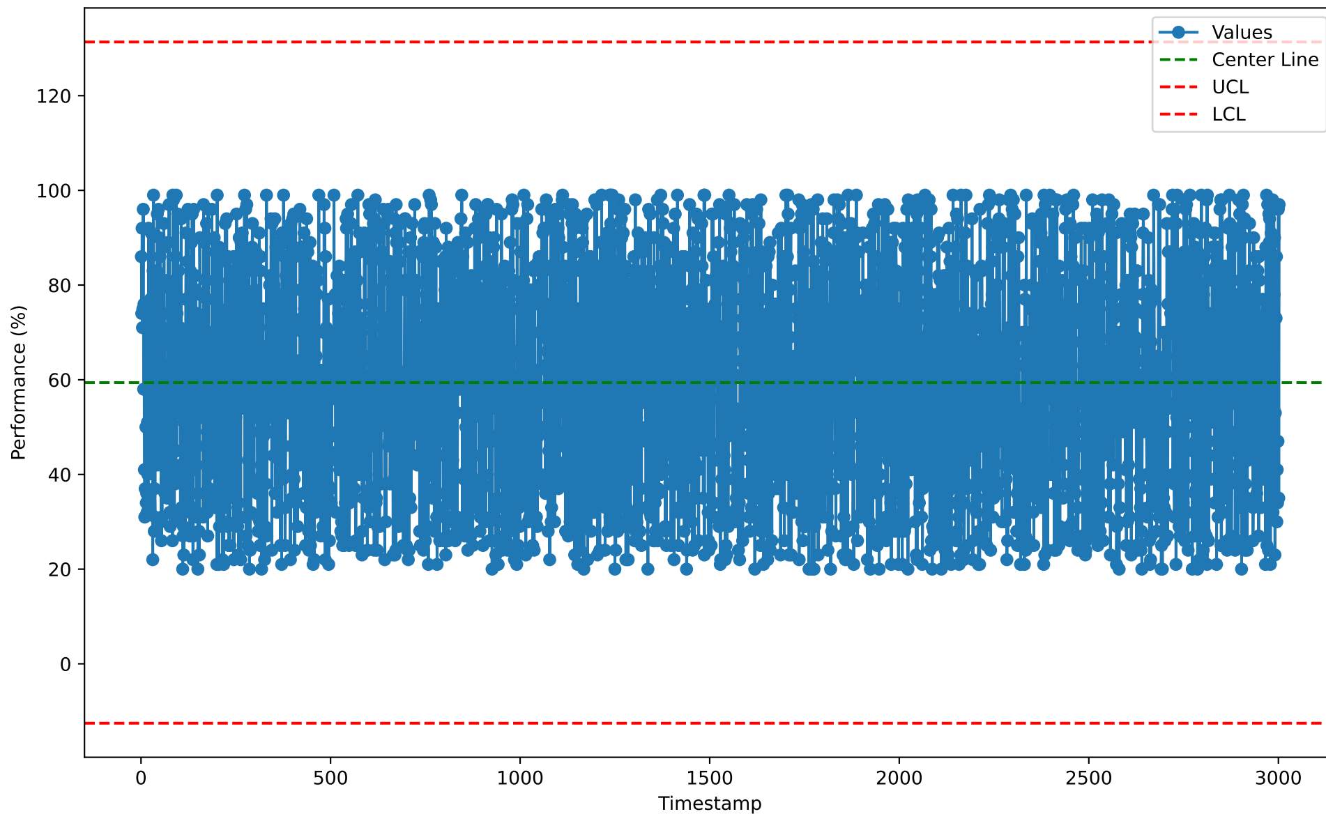
Individuals Chart for CFS10104 (2026-01-07)
