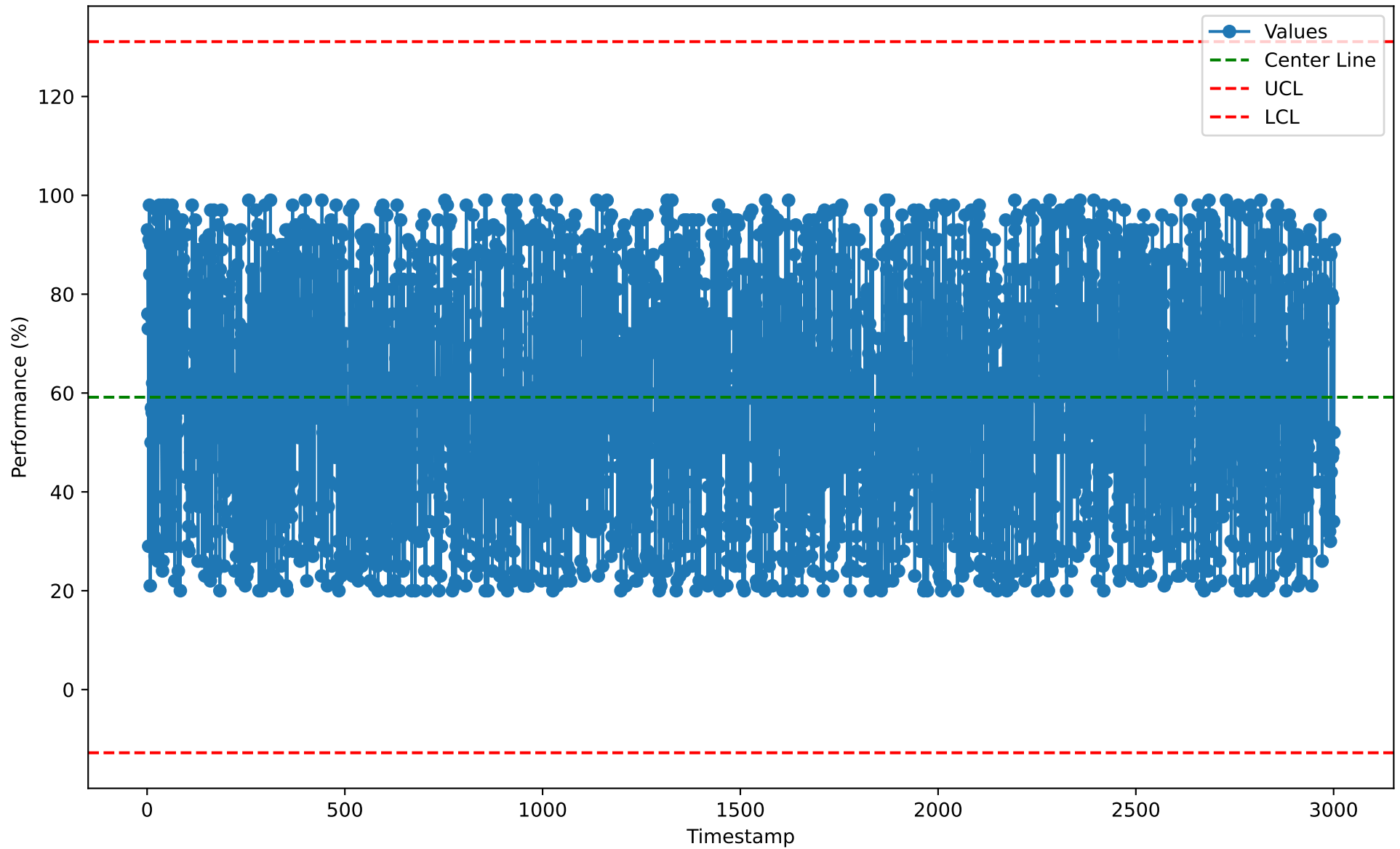
Individuals Chart for BIH10104 (2026-01-07)
