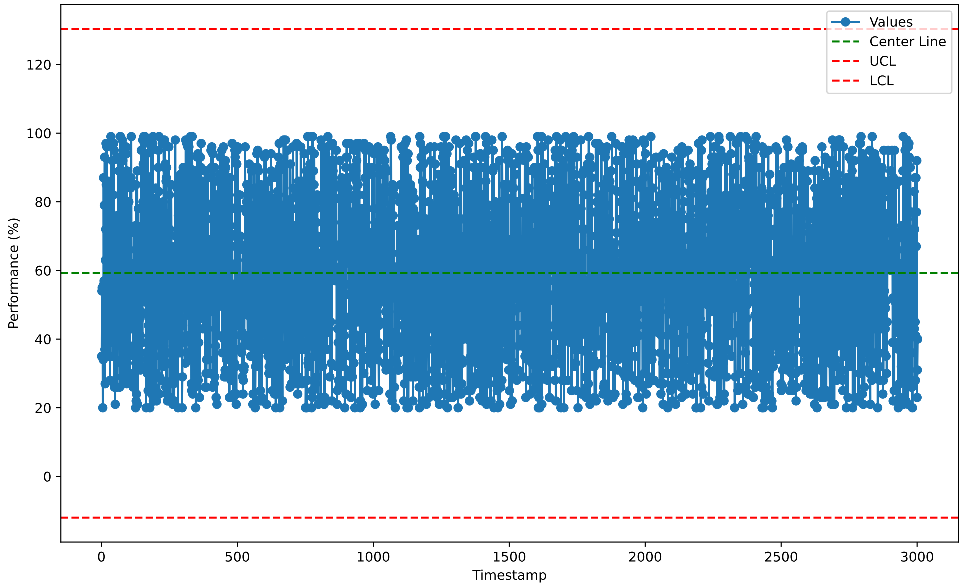
Individuals Chart for BIH10113 (2026-01-07)
