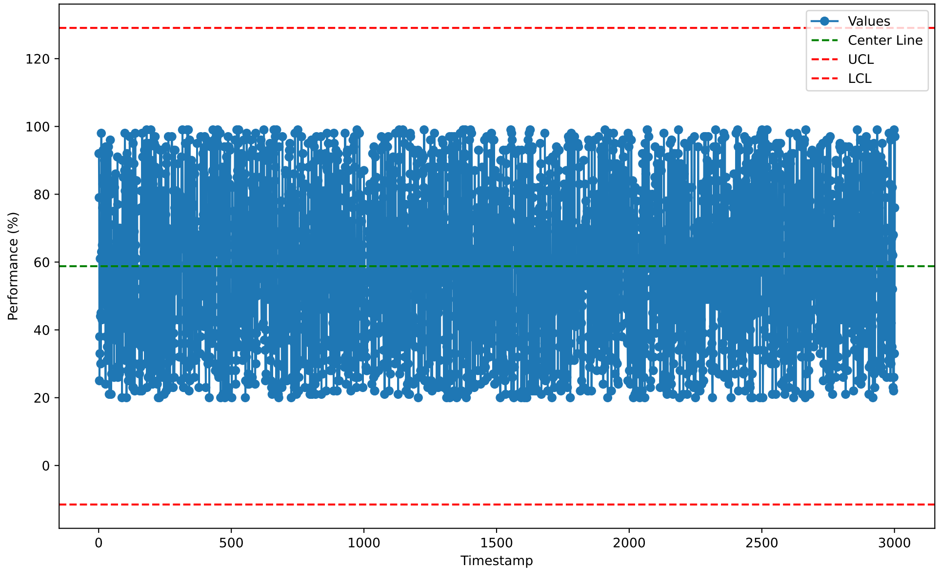
Individuals Chart for BIH10119 (2026-01-07)
