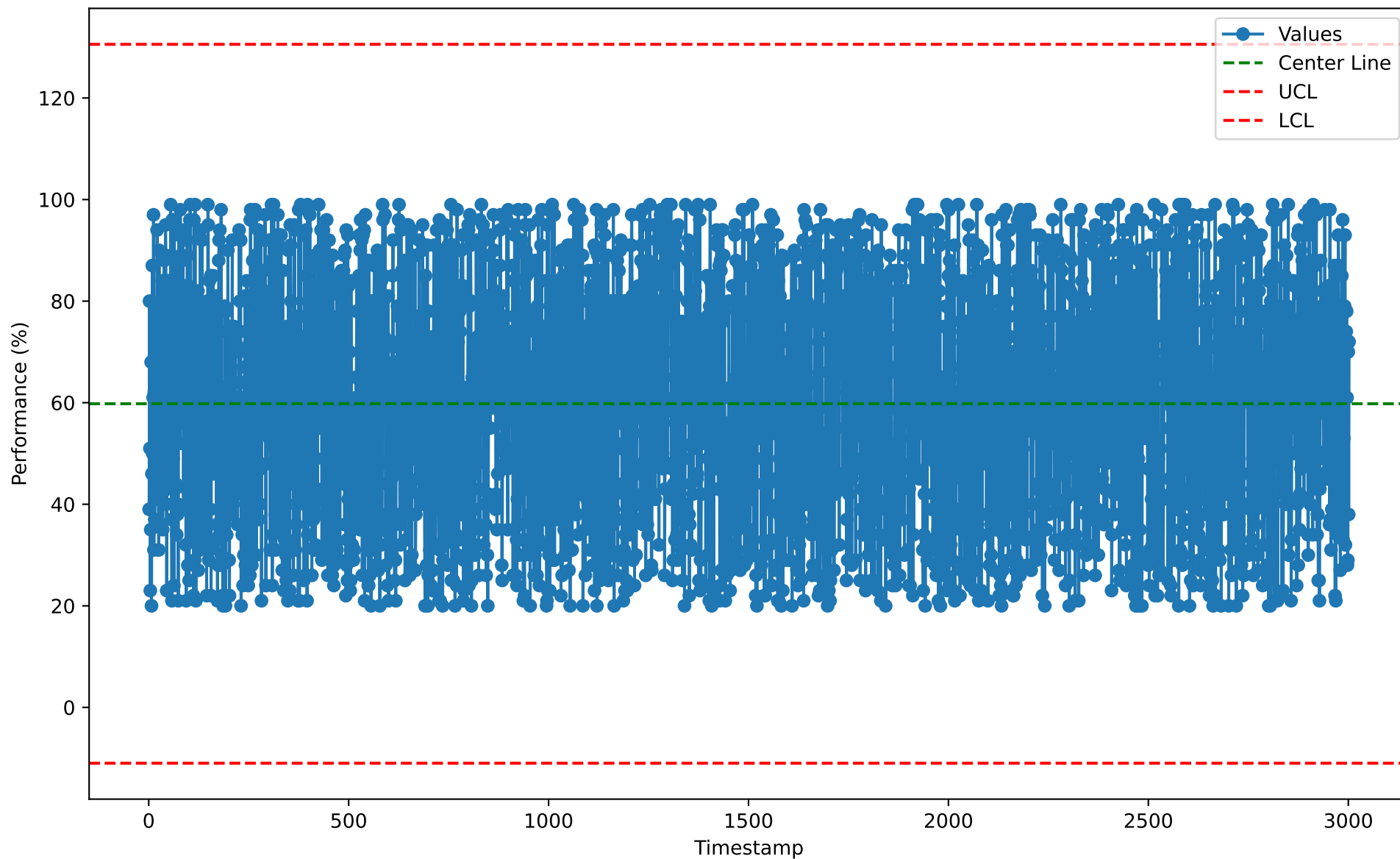
Individuals Chart for CIM10115 (2026-01-07)
