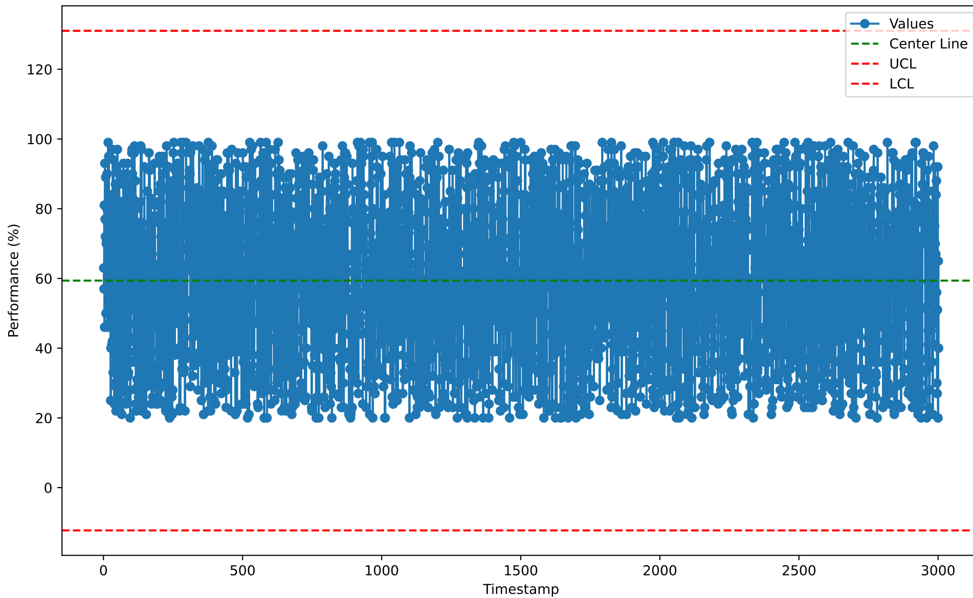
Individuals Chart for ITM10109 (2026-01-07)
