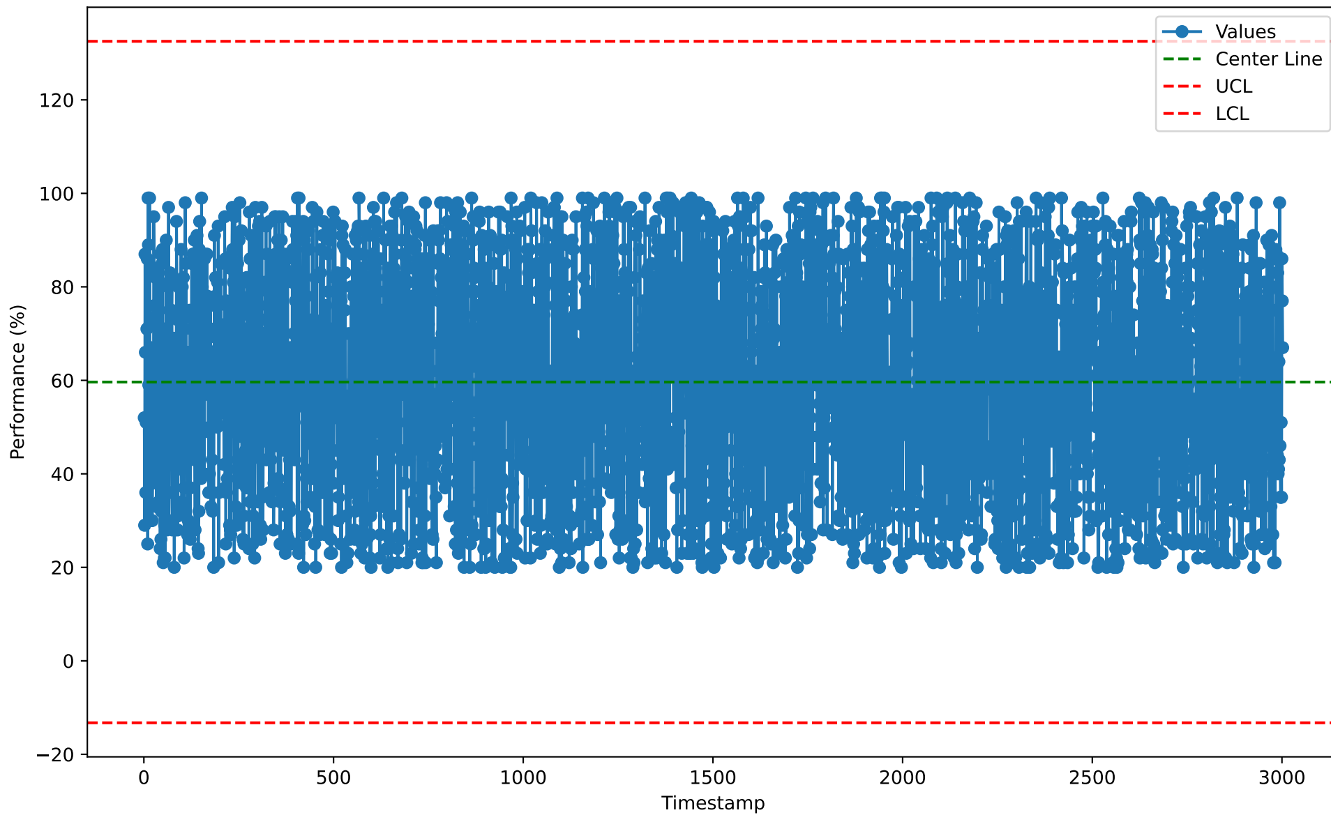
Individuals Chart for CFS10113 (2026-01-07)
