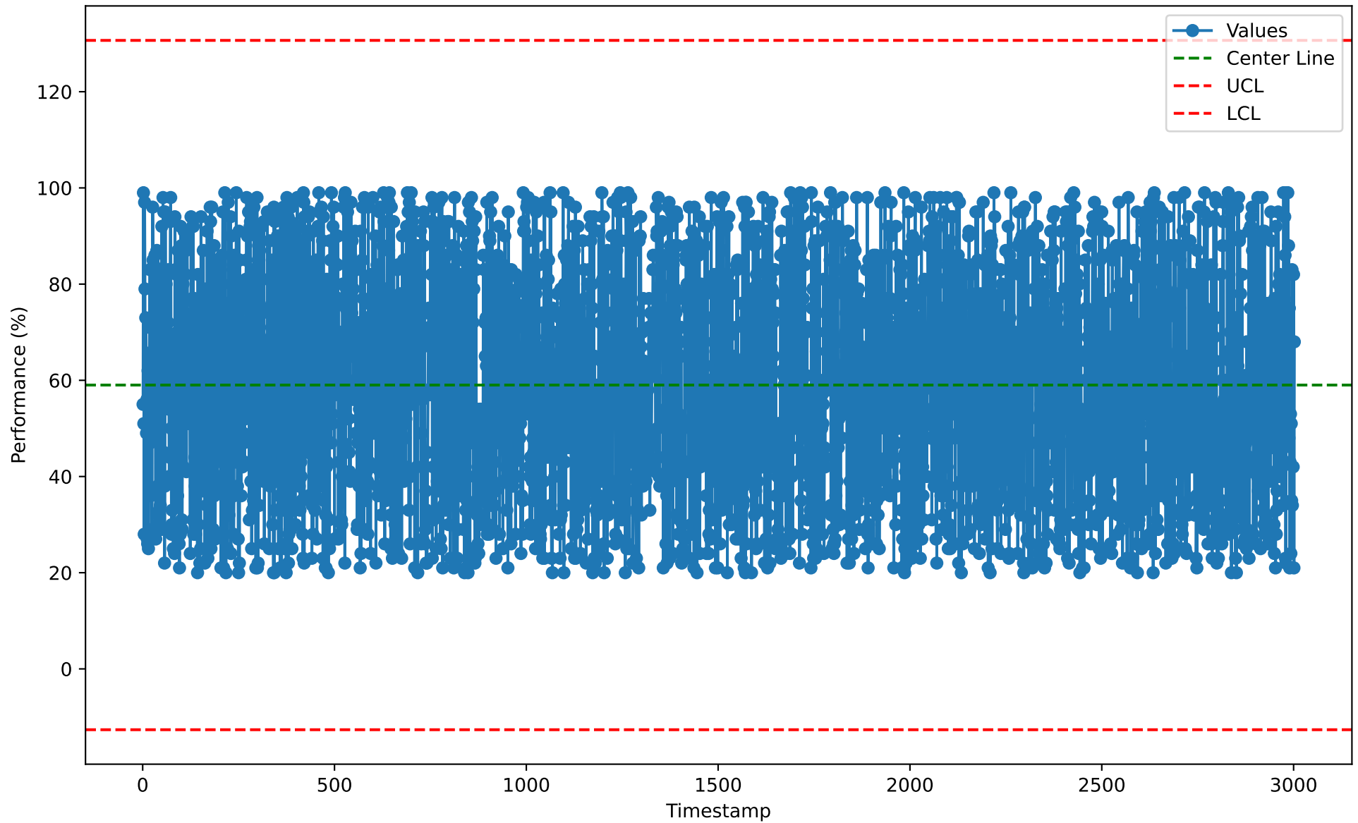
Individuals Chart for ITM10111 (2026-01-07)
