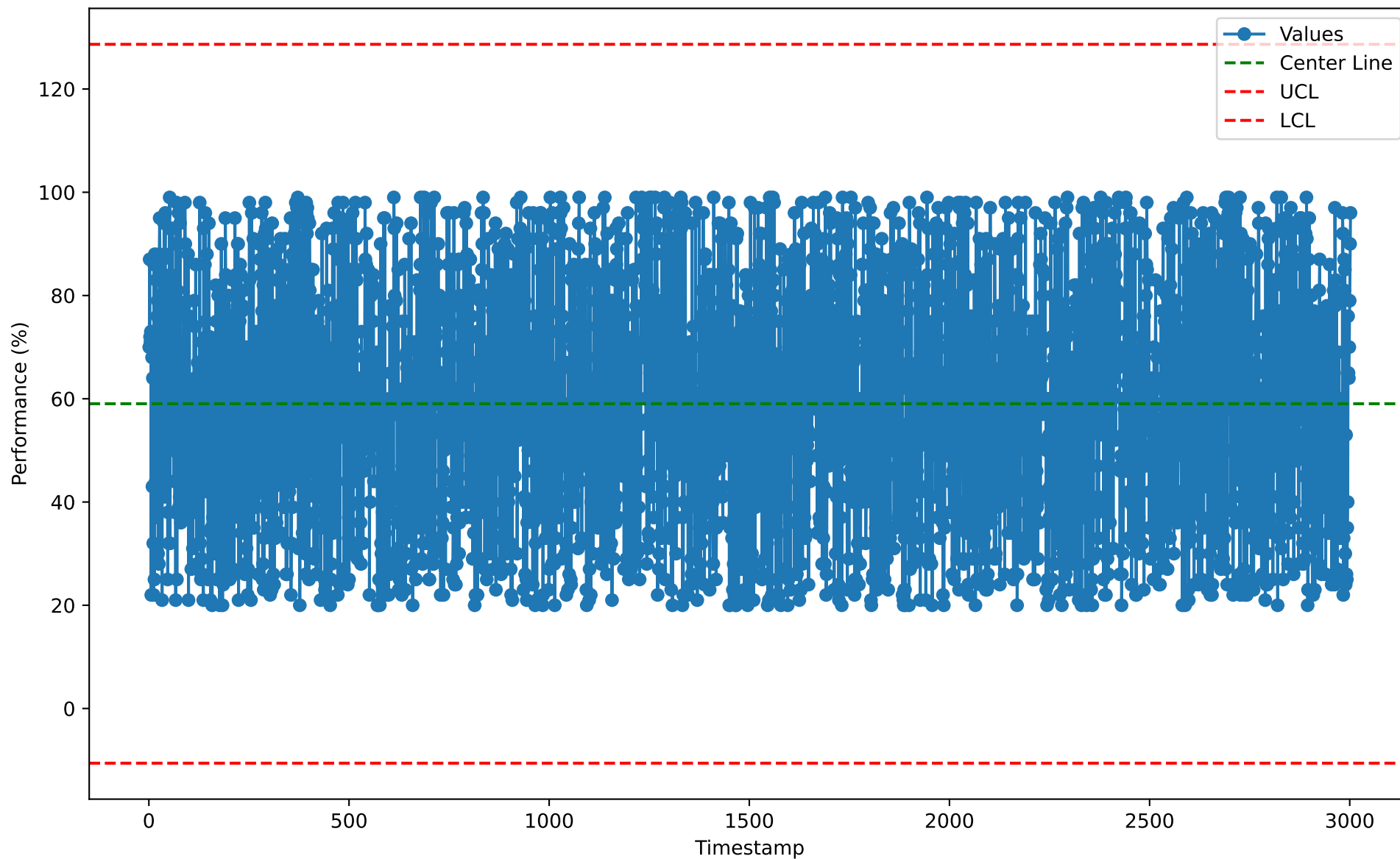
Individuals Chart for CFS10110 (2026-01-07)
