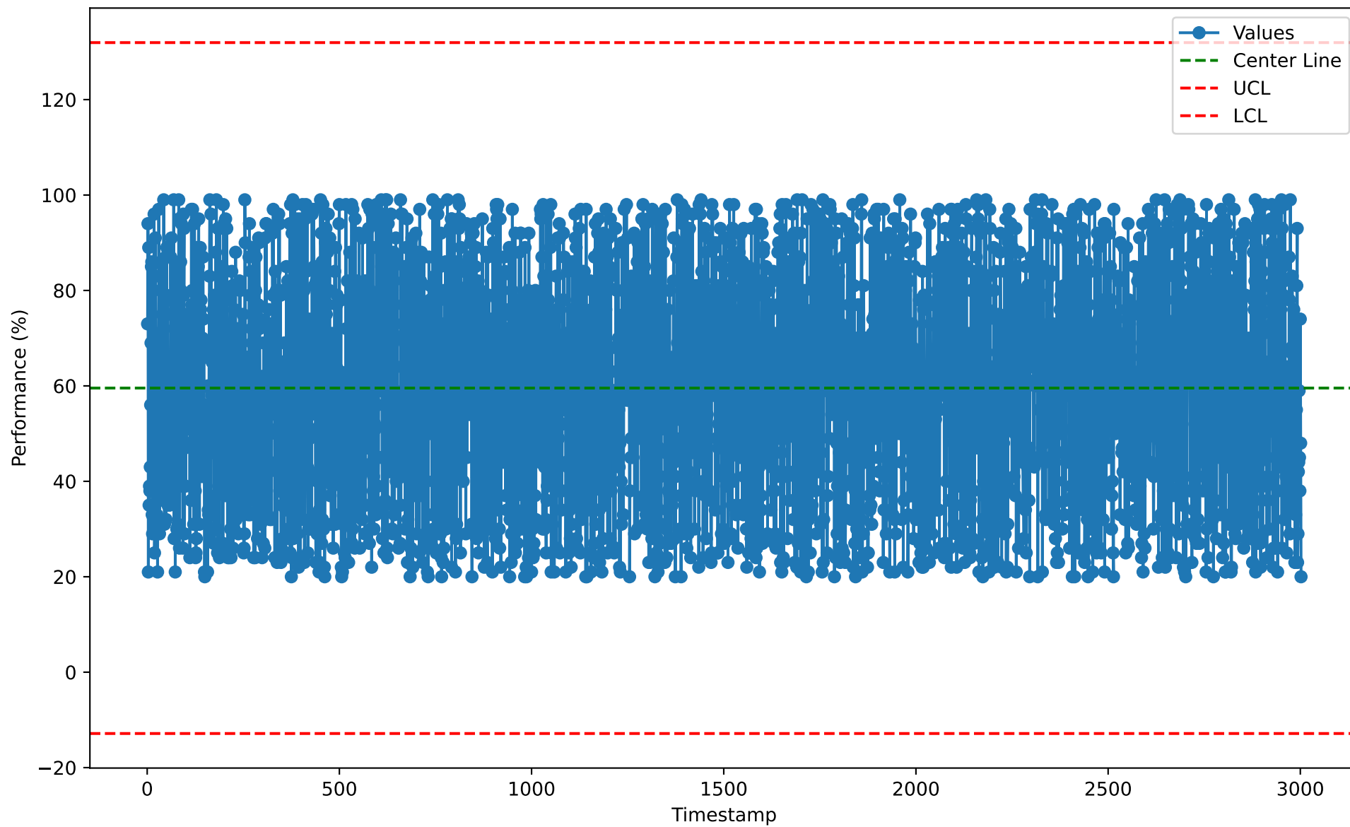
Individuals Chart for BIH10108 (2026-01-07)
