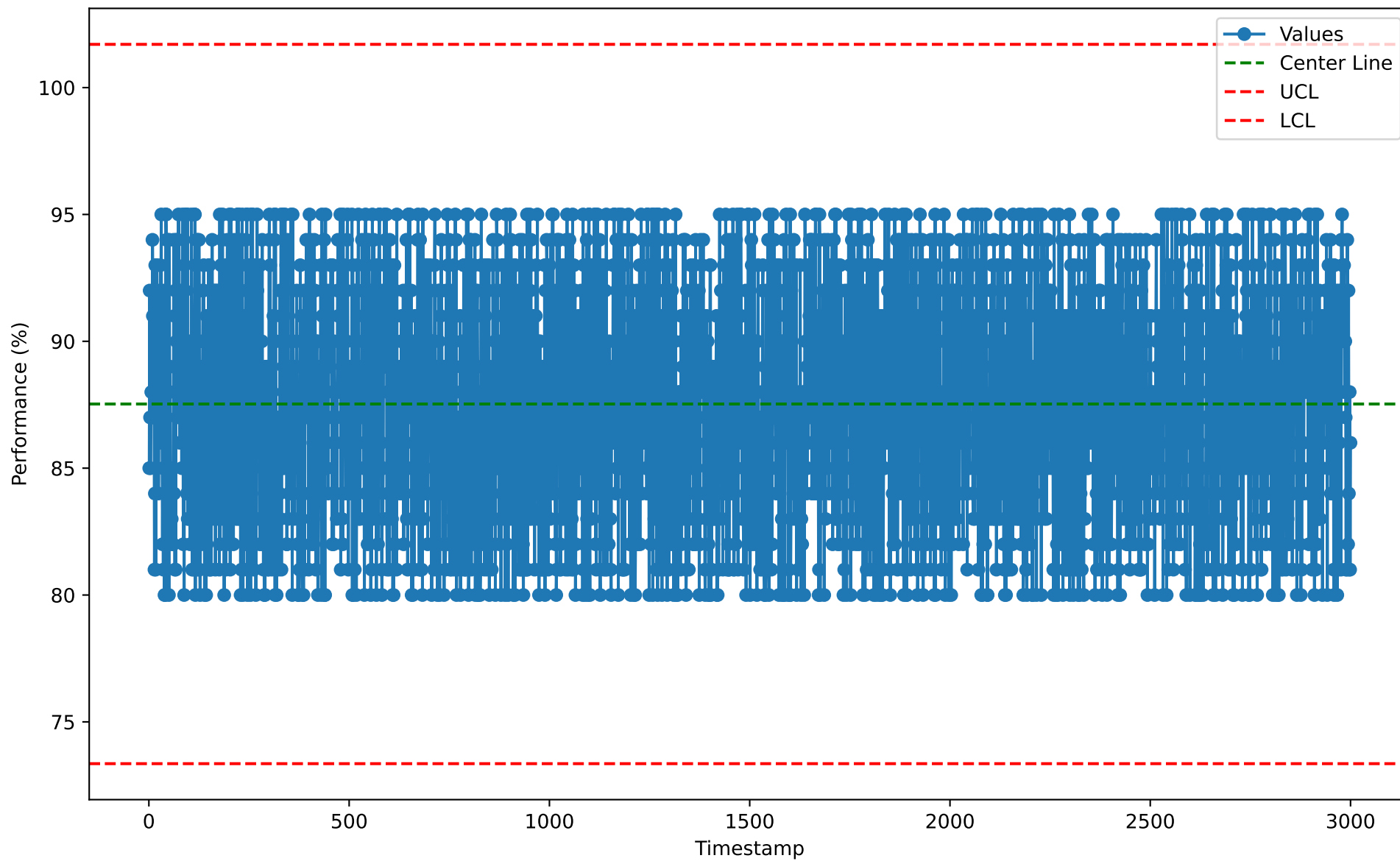
Individuals Chart for RTS10106 (2026-01-07)
