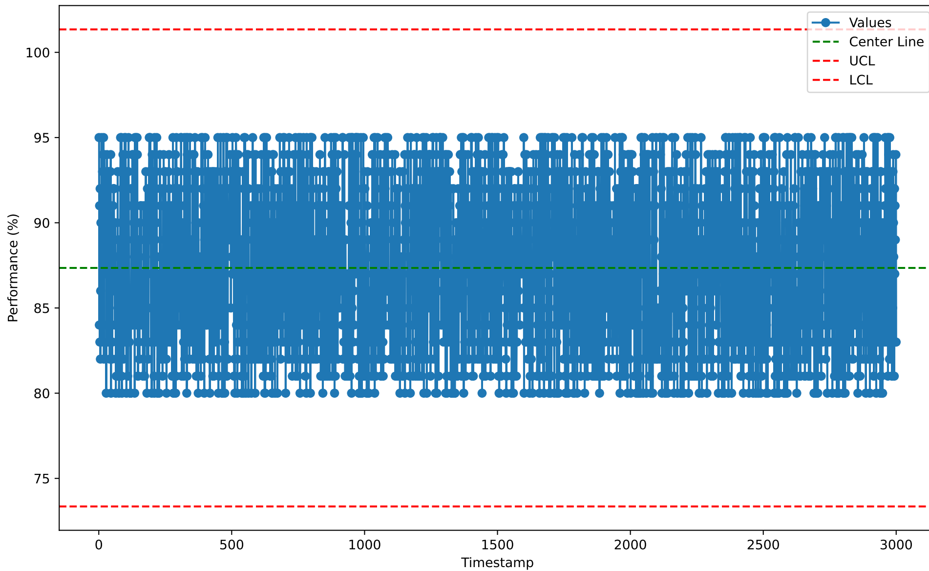
Individuals Chart for CIP10110 (2026-01-07)
