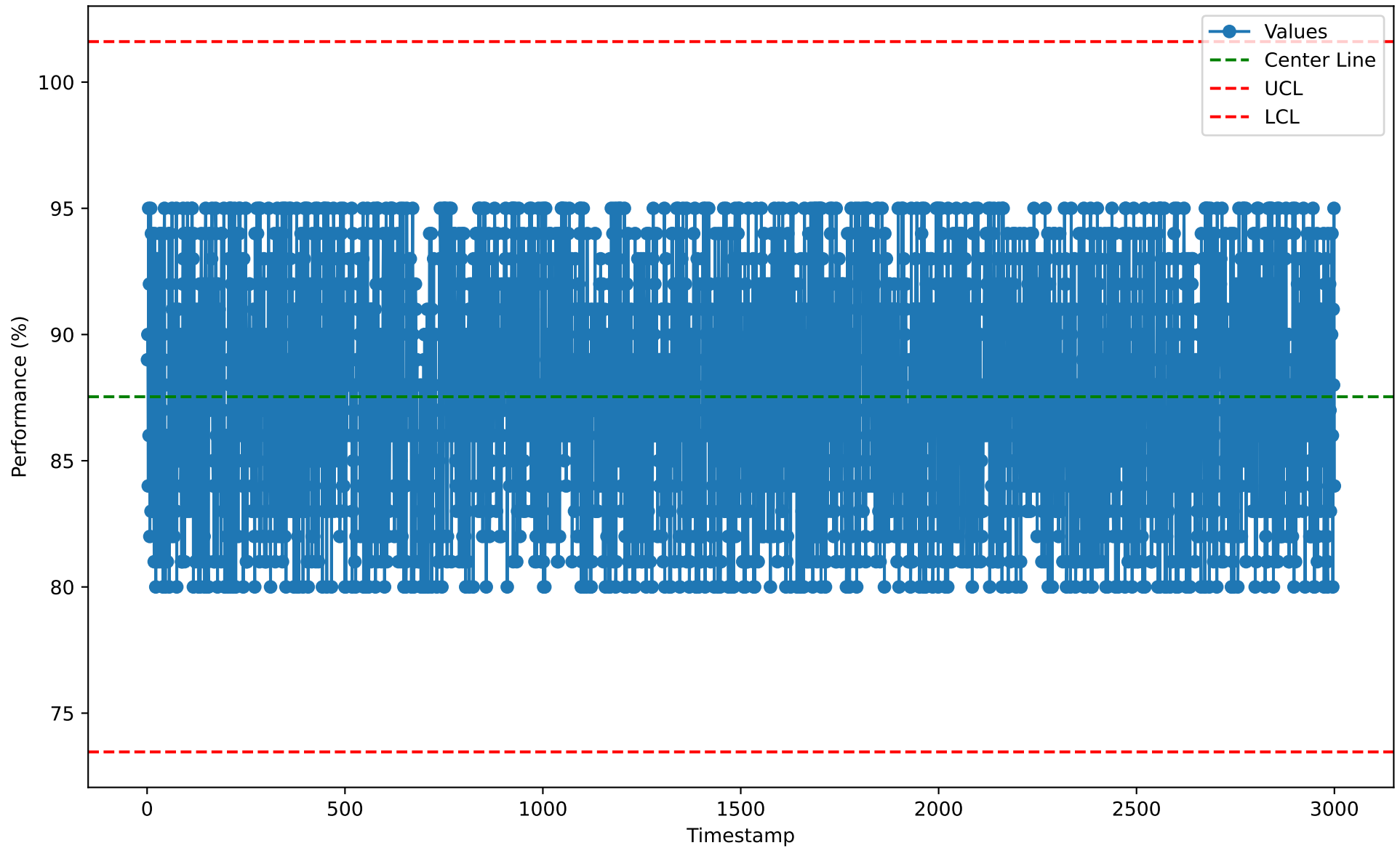
Individuals Chart for CIP10111 (2026-01-07)
