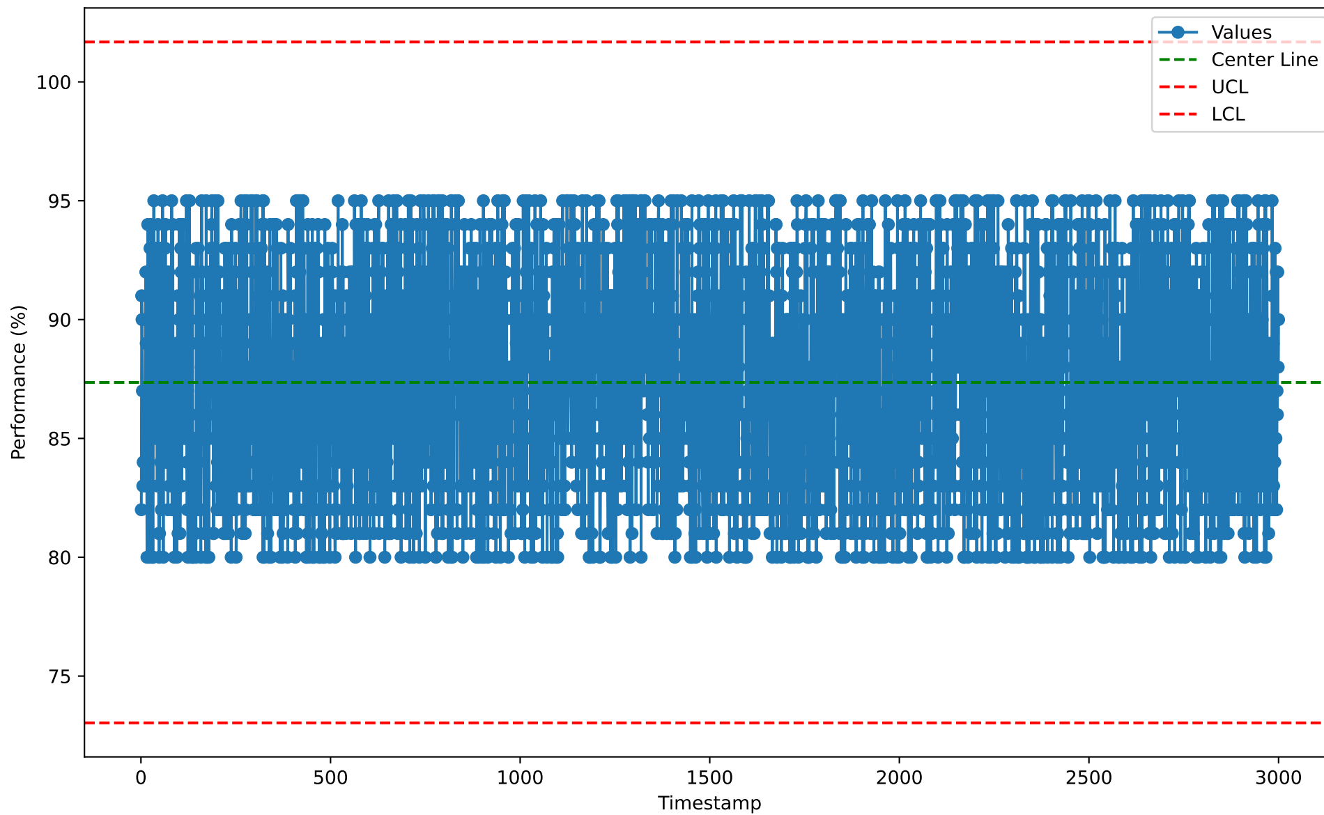
Individuals Chart for RTS10102 (2026-01-07)
