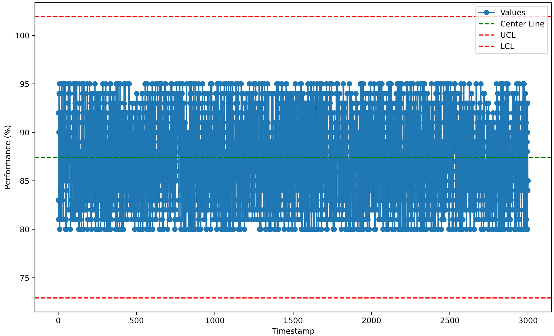
Individuals Chart for CIP10107 (2026-01-07)
