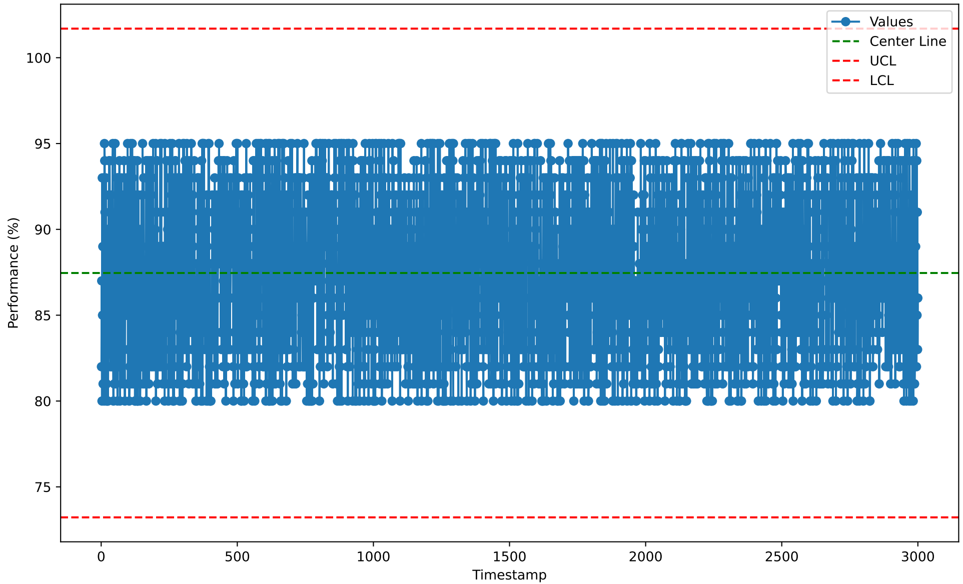
Individuals Chart for CIP10103 (2026-01-07)
