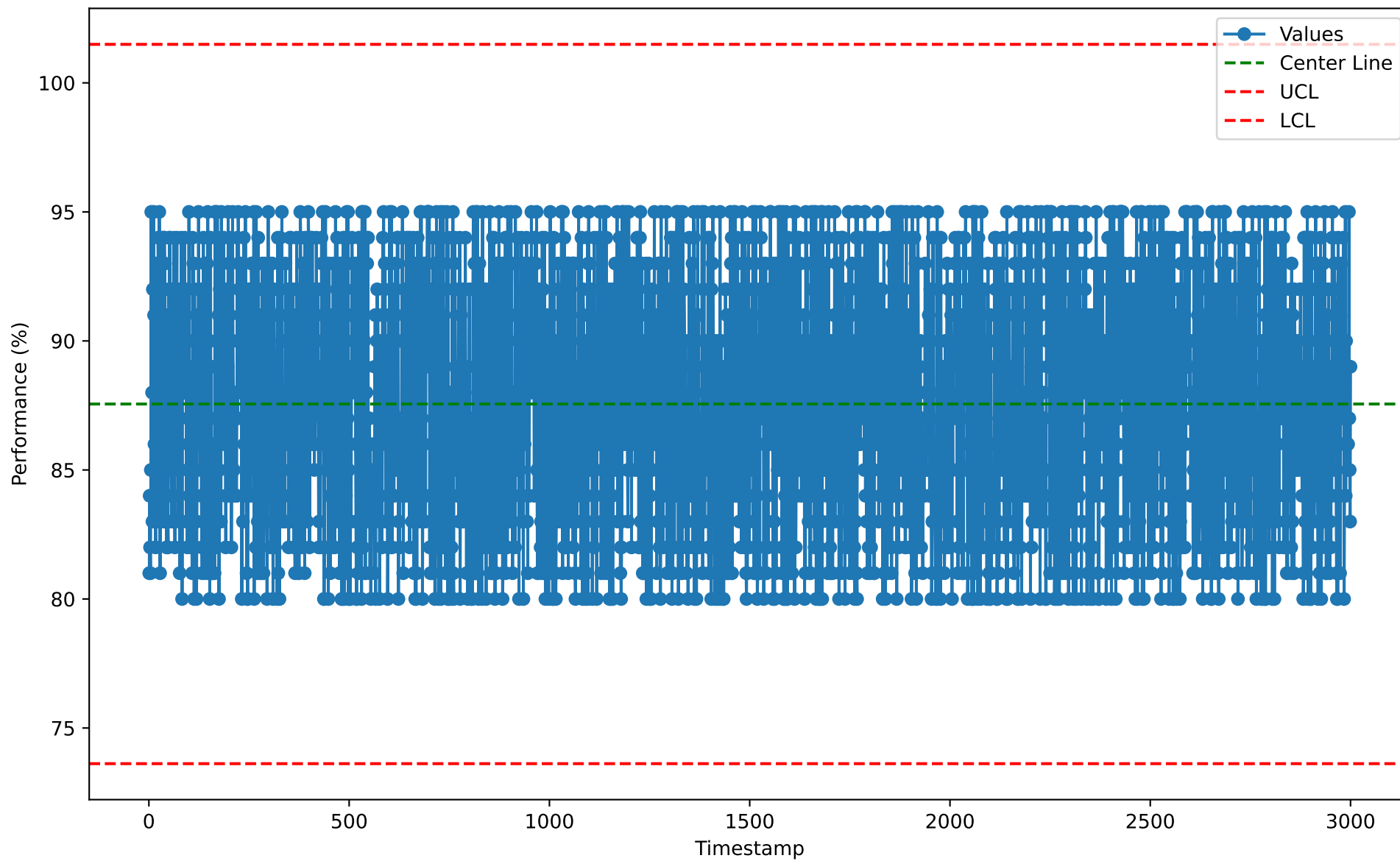
Individuals Chart for LCP10108 (2026-01-07)
