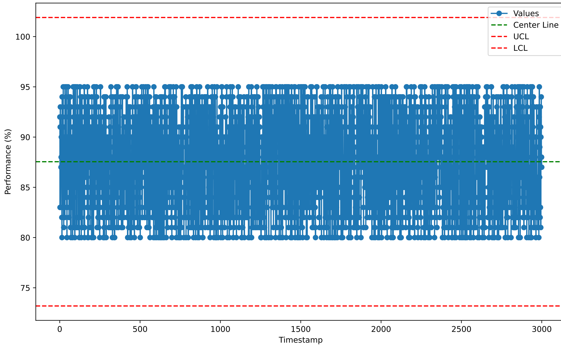
Individuals Chart for LCP10107 (2026-01-07)
