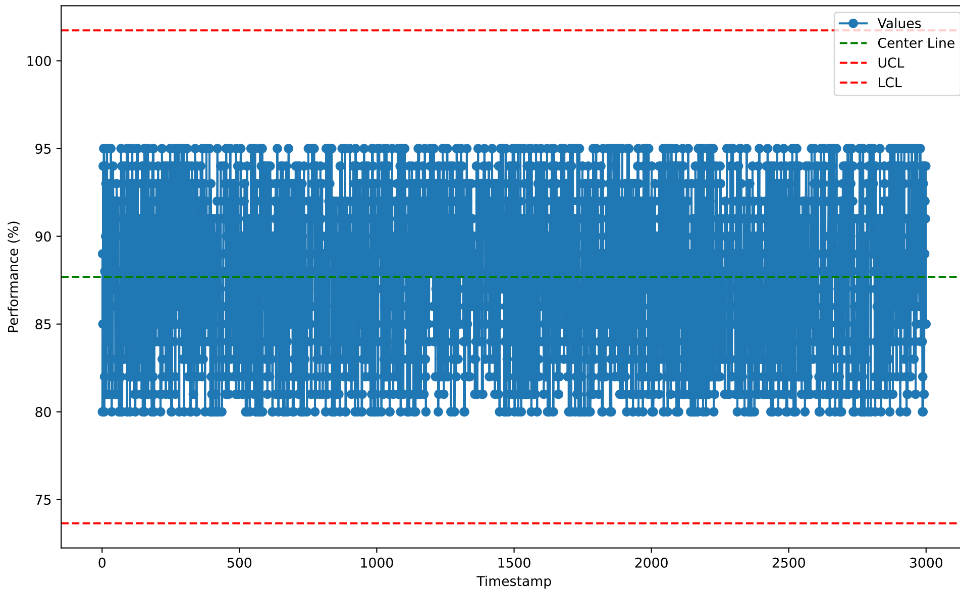
Individuals Chart for RTS10104 (2026-01-07)
