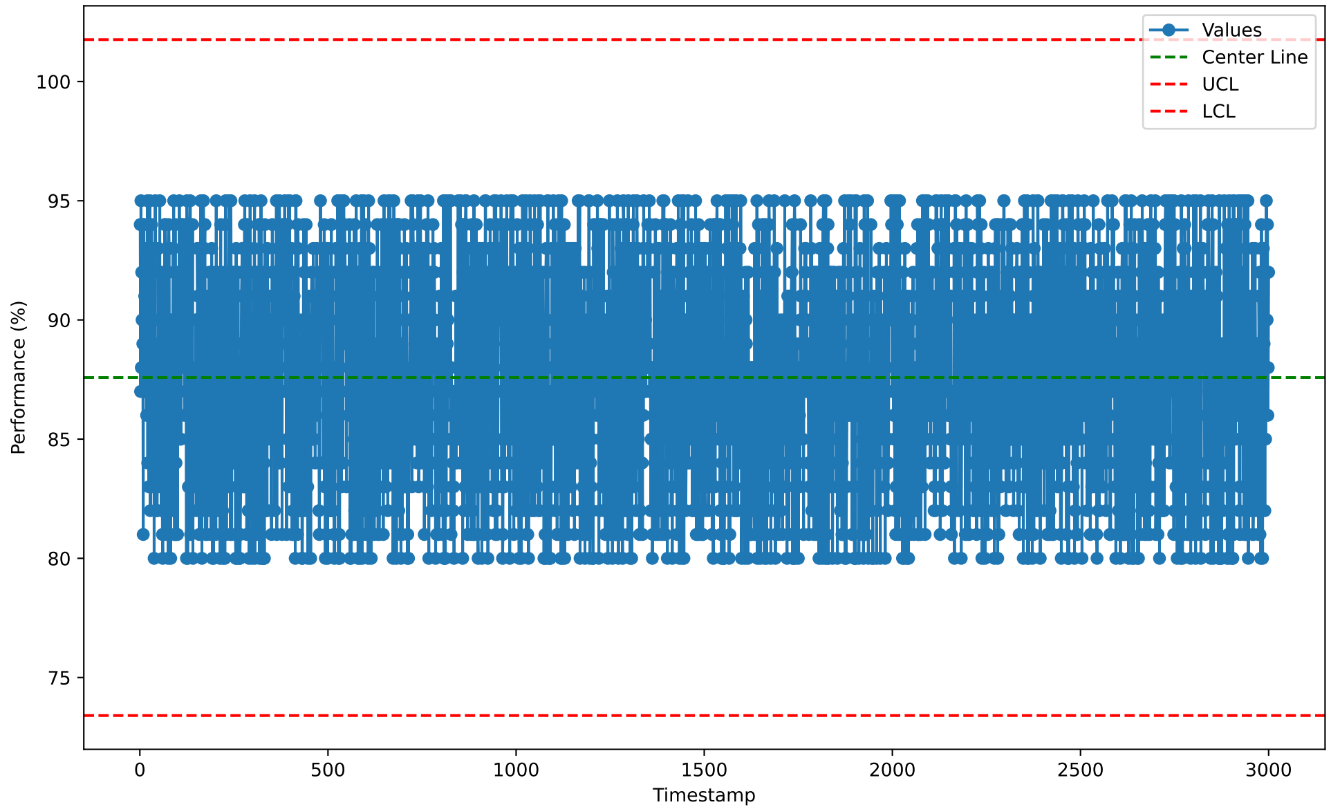
Individuals Chart for CIP10114 (2026-01-07)
