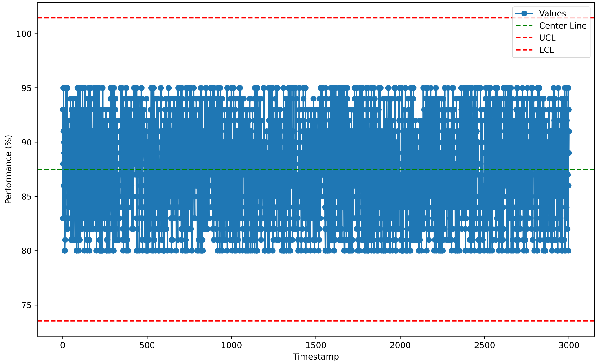
Individuals Chart for CIP10112 (2026-01-07)
