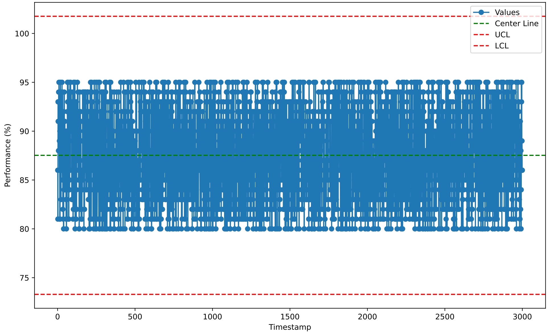
Individuals Chart for CIP10108 (2026-01-07)
