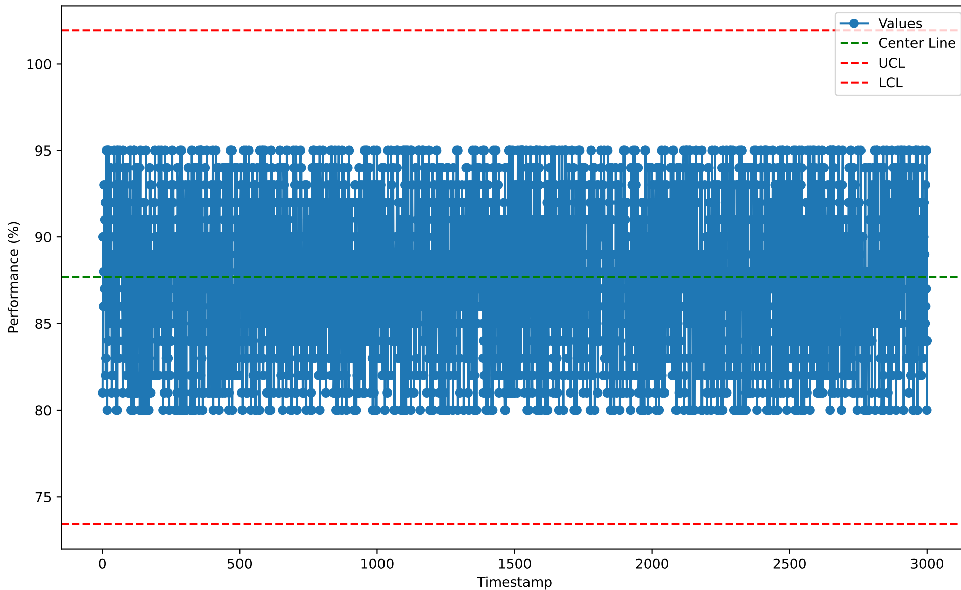
Individuals Chart for IOP10108 (2026-01-07)
