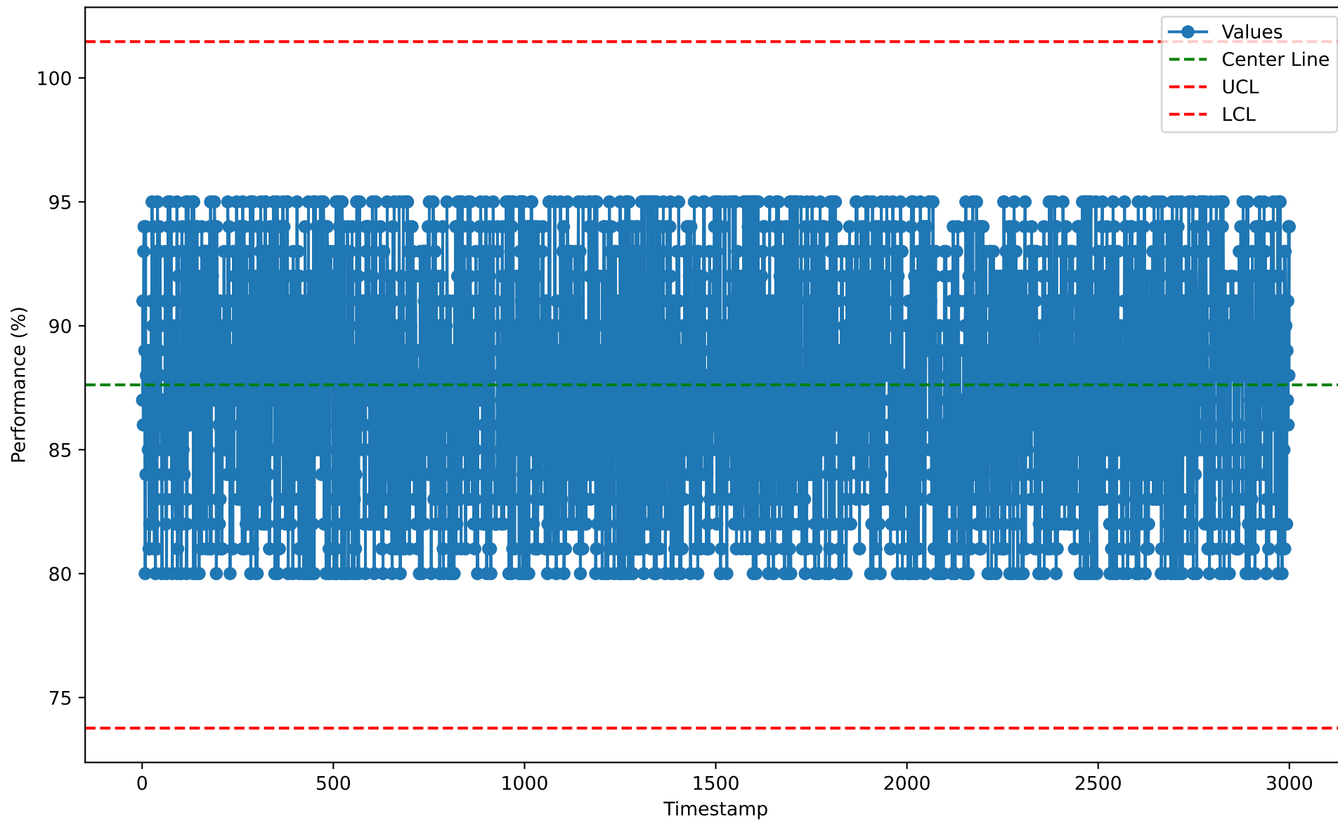
Individuals Chart for LCP10115 (2026-01-07)
