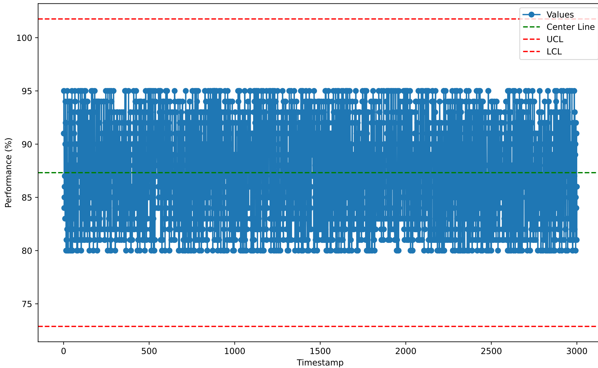
Individuals Chart for RTS10107 (2026-01-07)
