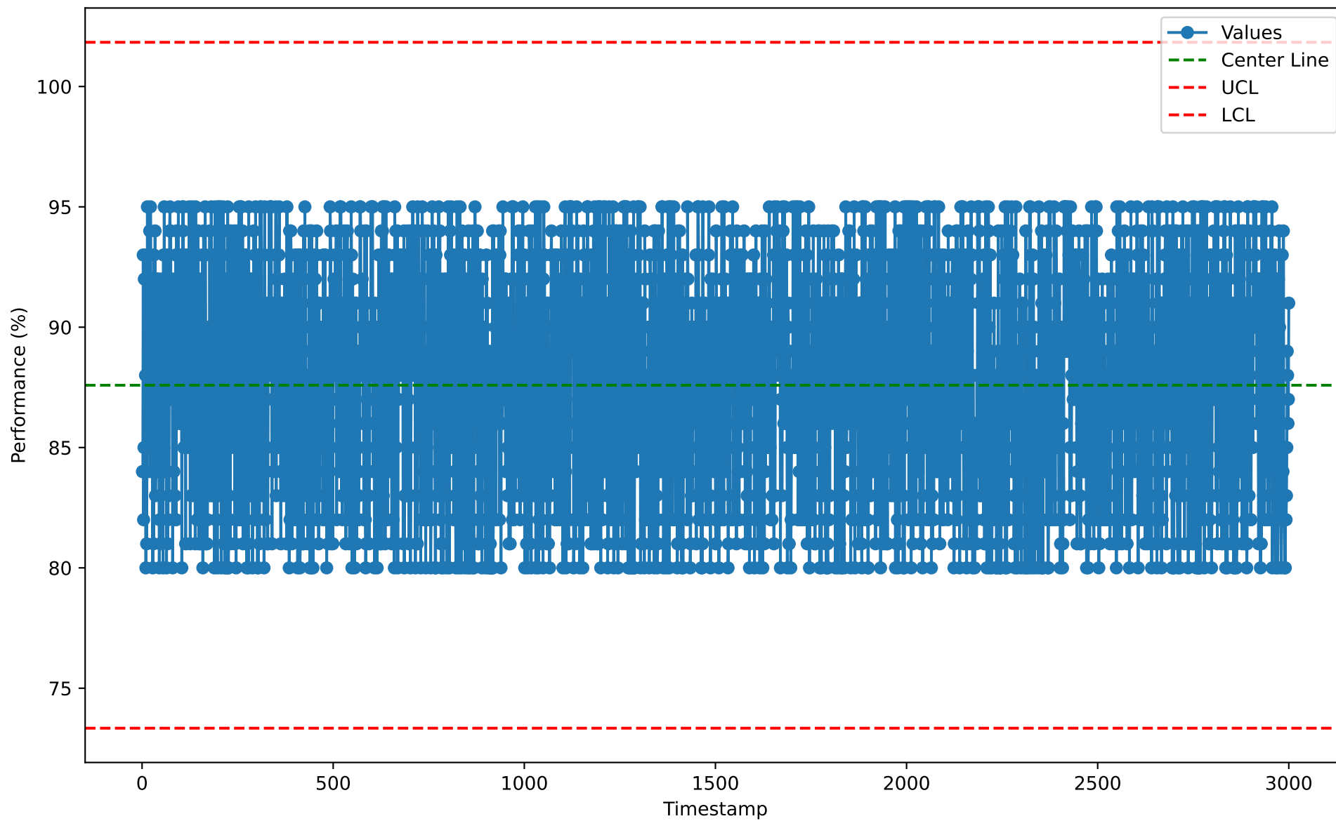
Individuals Chart for IOP10109 (2026-01-07)
