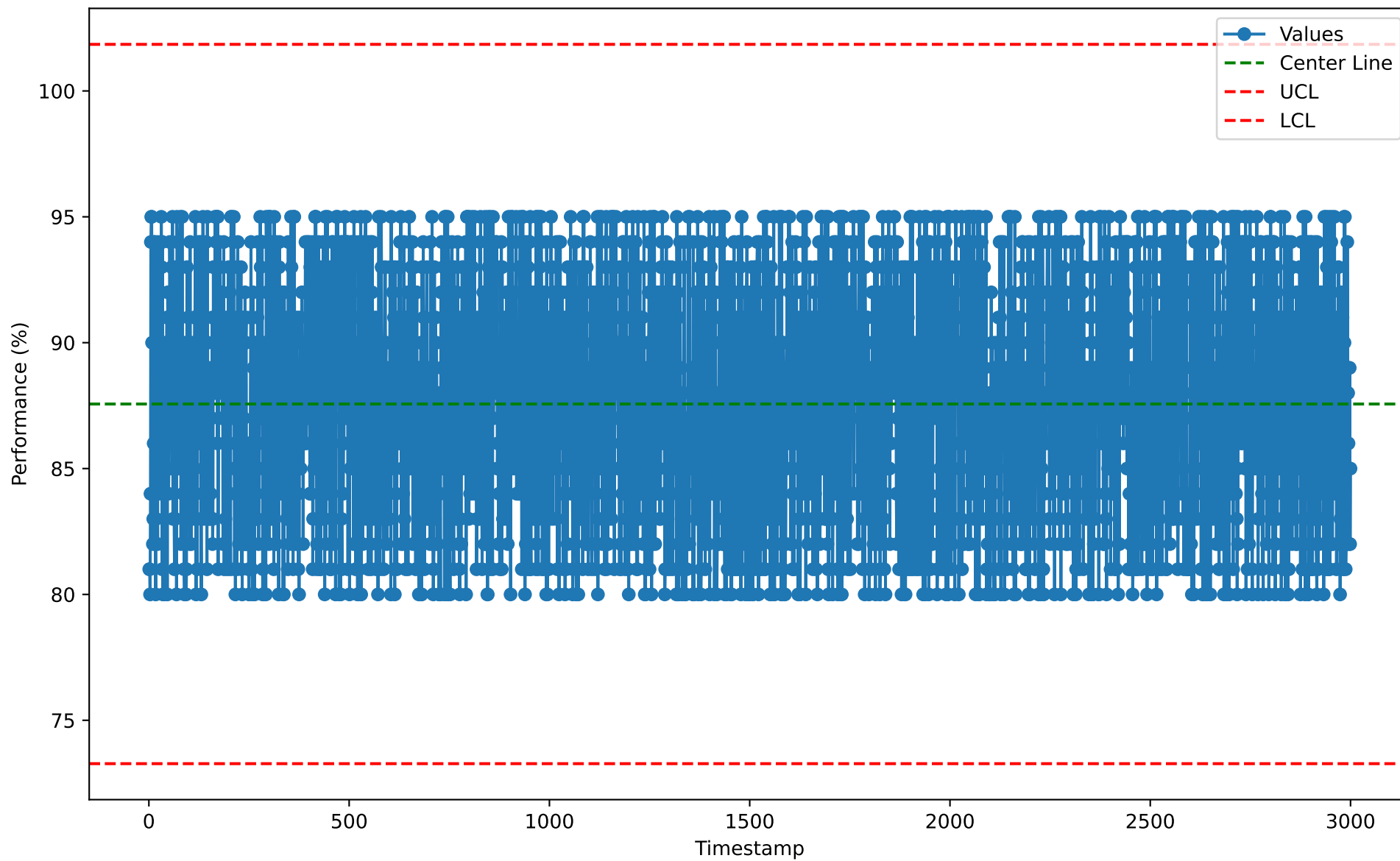
Individuals Chart for LCP10103 (2026-01-07)
