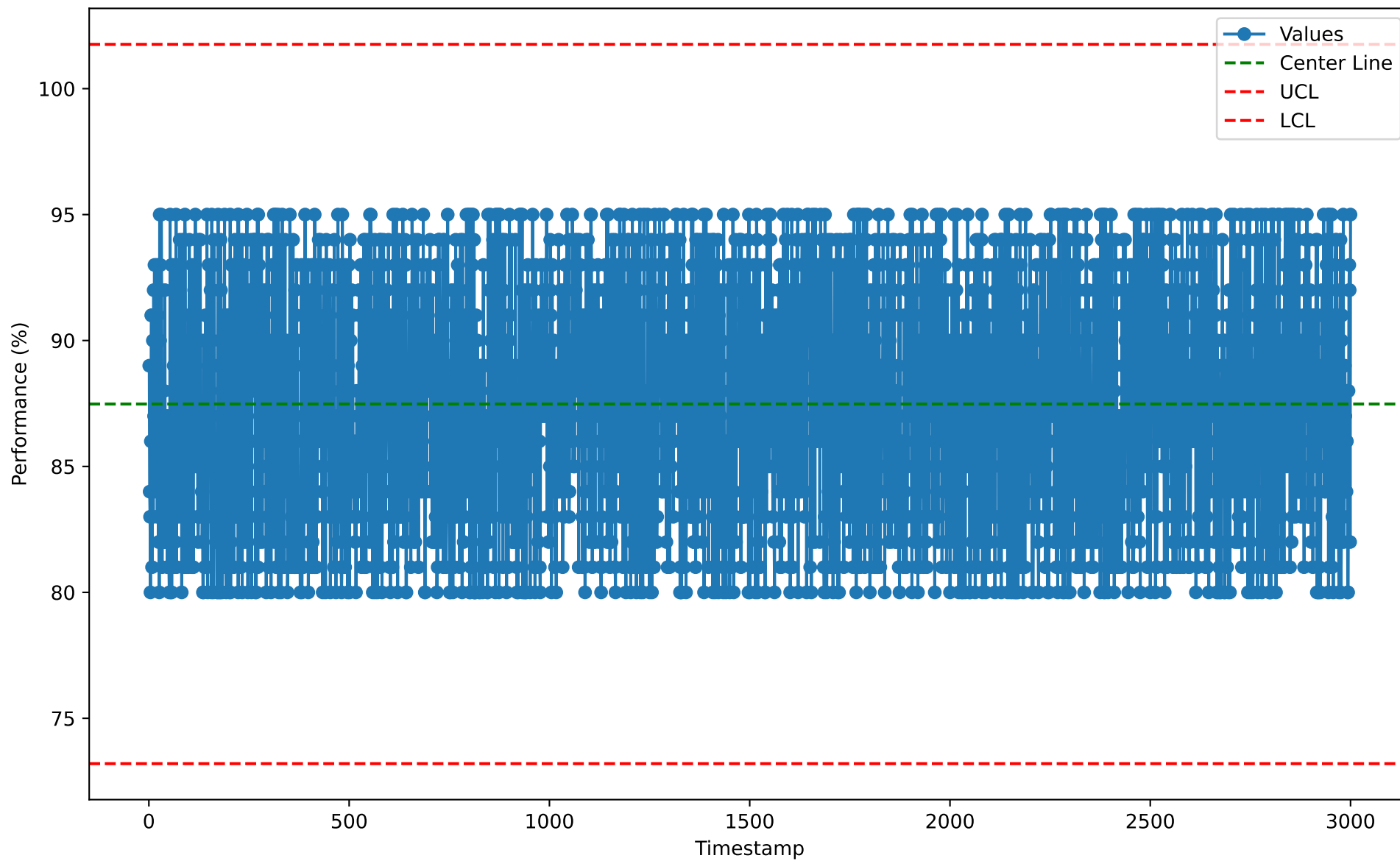
Individuals Chart for IOP10103 (2026-01-07)
