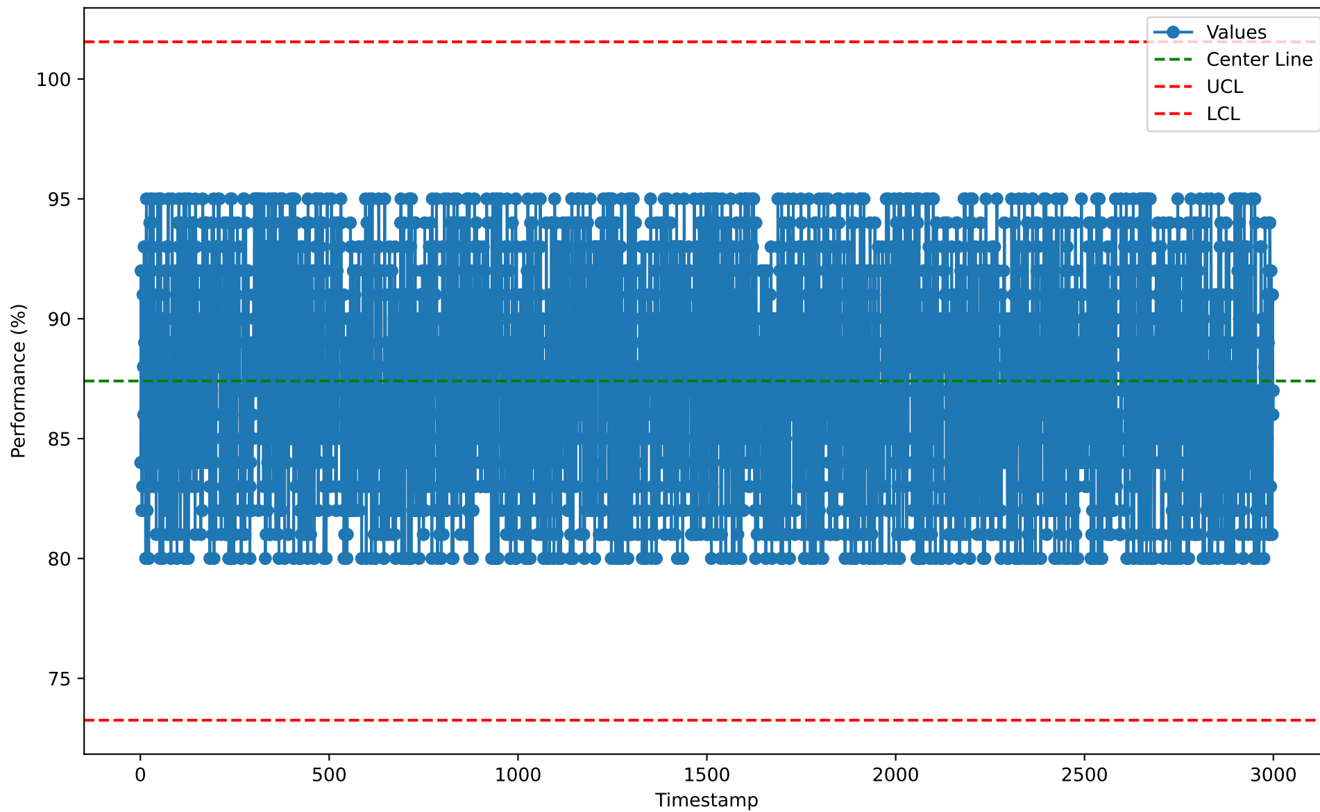
Individuals Chart for LCP10106 (2026-01-07)
