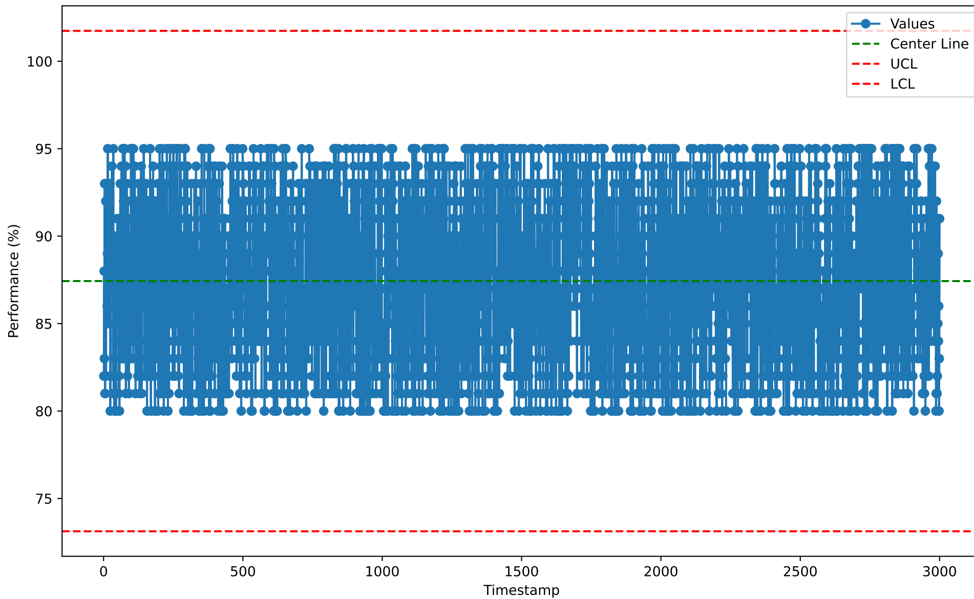
Individuals Chart for LCP10110 (2026-01-07)
