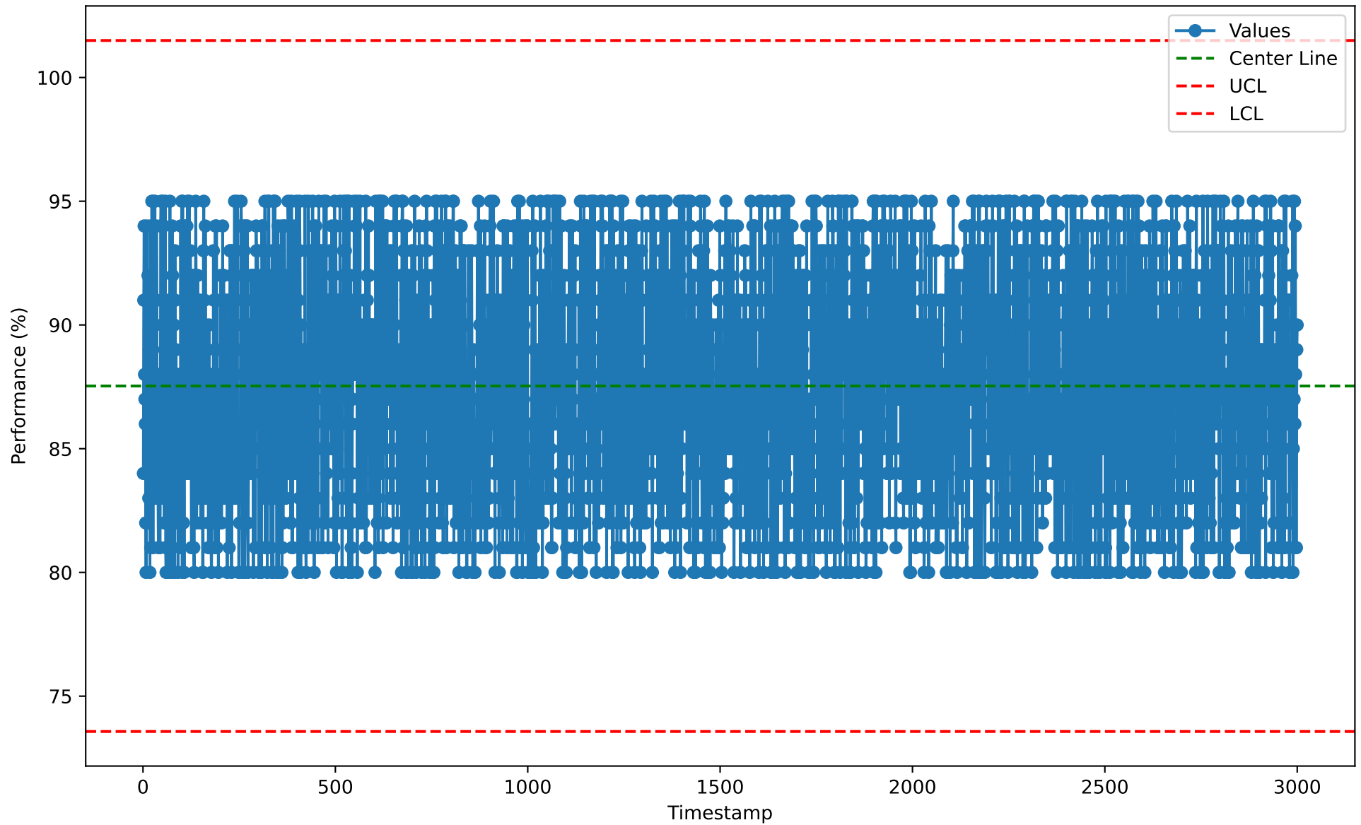
Individuals Chart for CIP10102 (2026-01-07)
