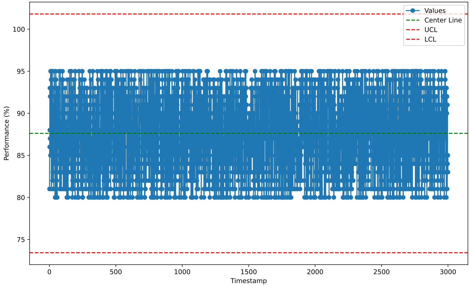
Individuals Chart for CIP10113 (2026-01-07)
