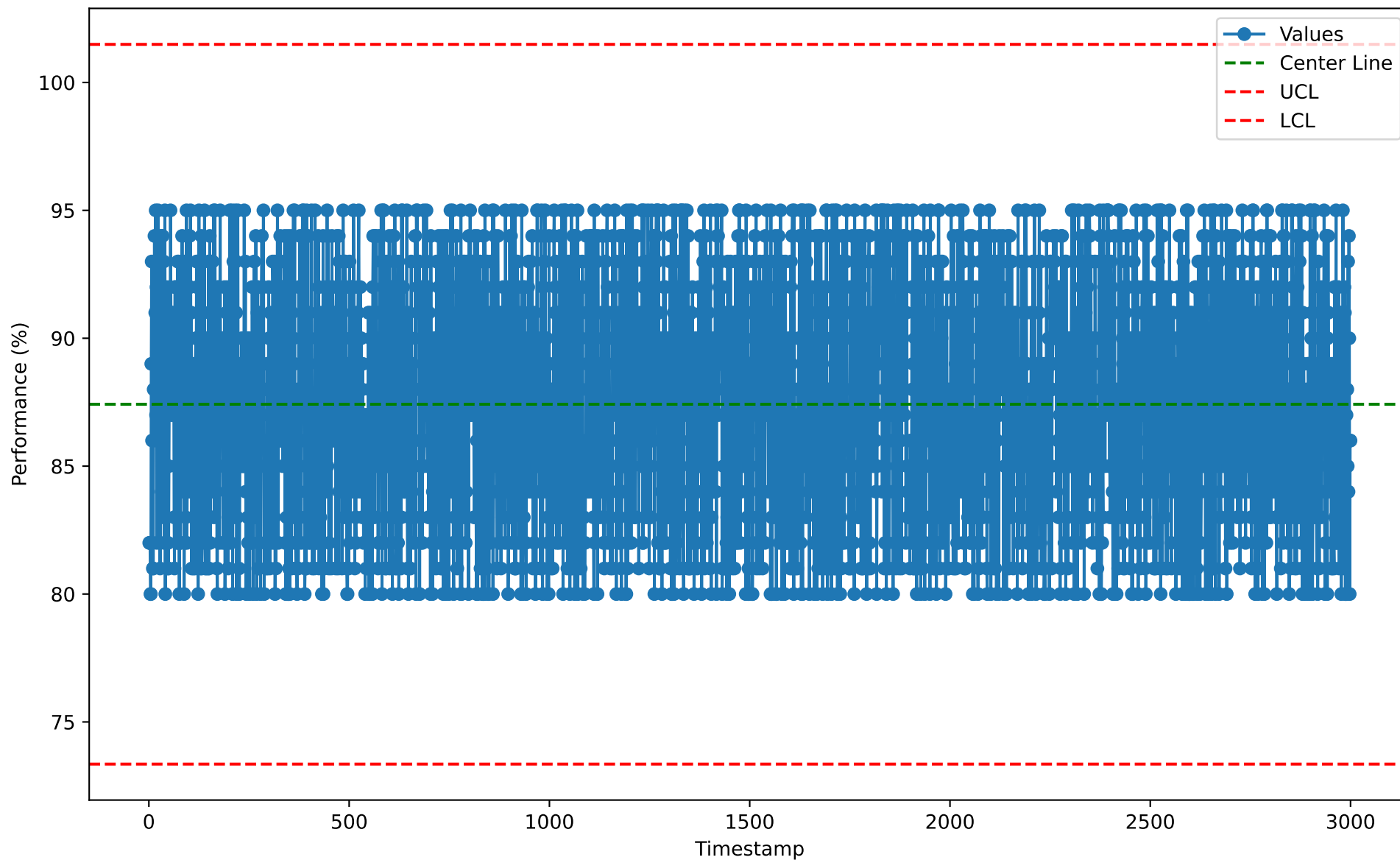
Individuals Chart for RTS10103 (2026-01-07)
