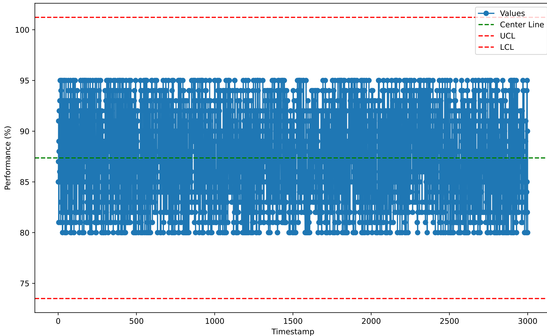
Individuals Chart for RTS10108 (2026-01-07)
