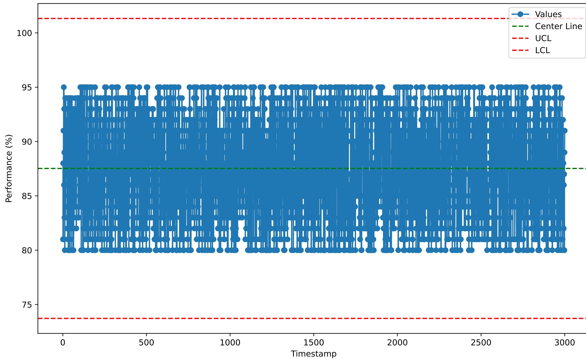
Individuals Chart for IOP10102 (2026-01-07)
