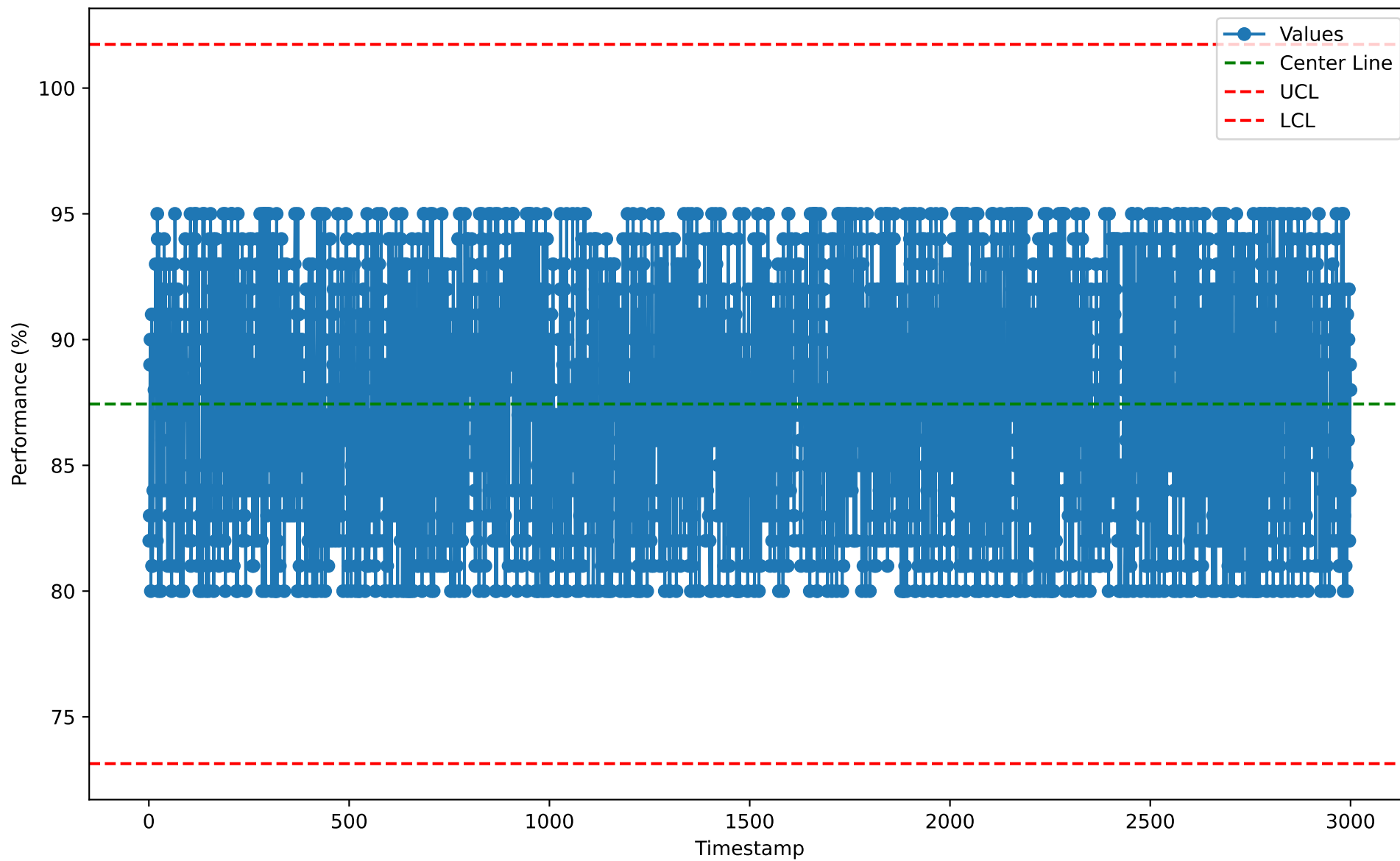
Individuals Chart for CIP10106 (2026-01-07)
