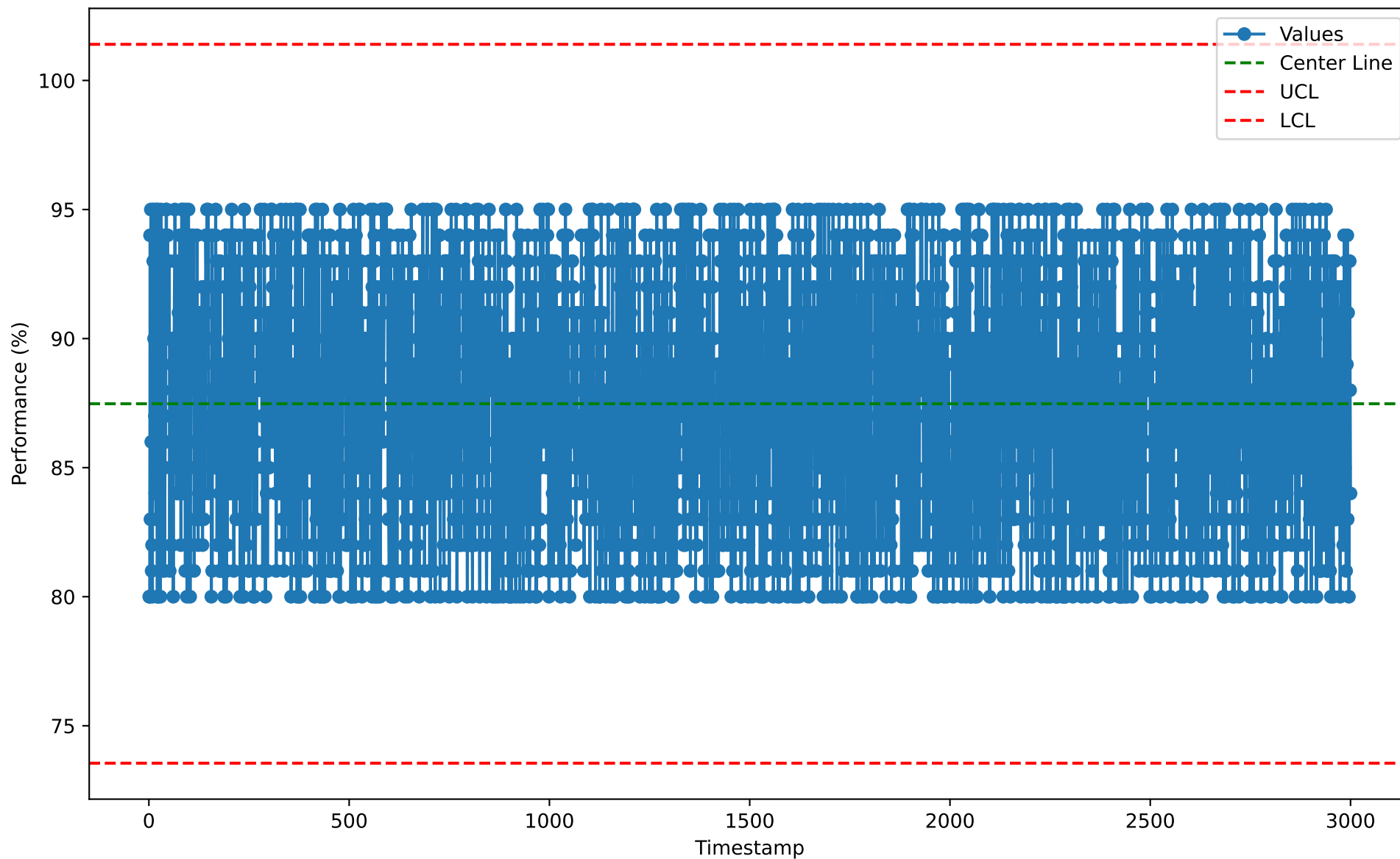
Individuals Chart for LCP10112 (2026-01-07)
