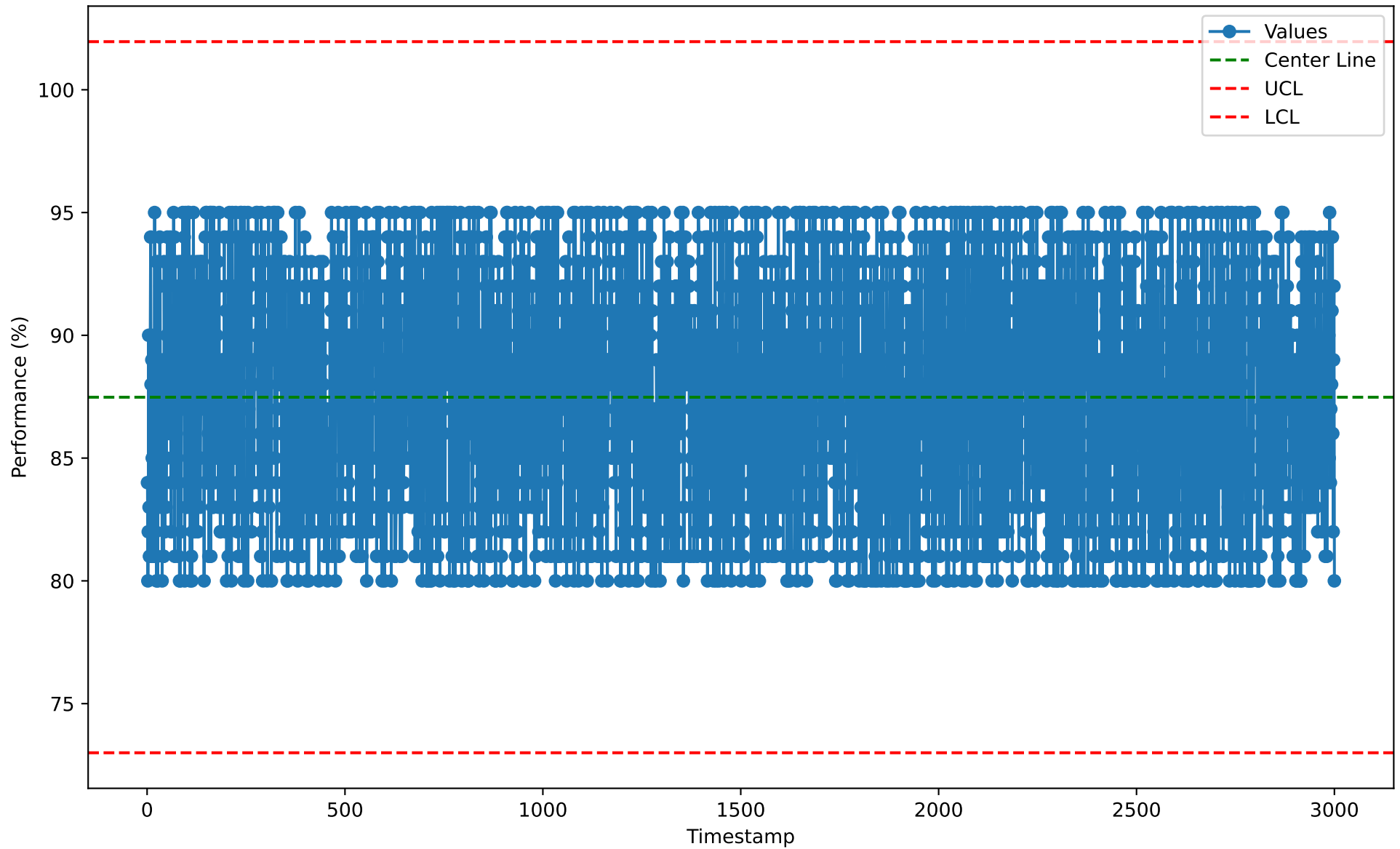
Individuals Chart for IOP10105 (2026-01-07)
