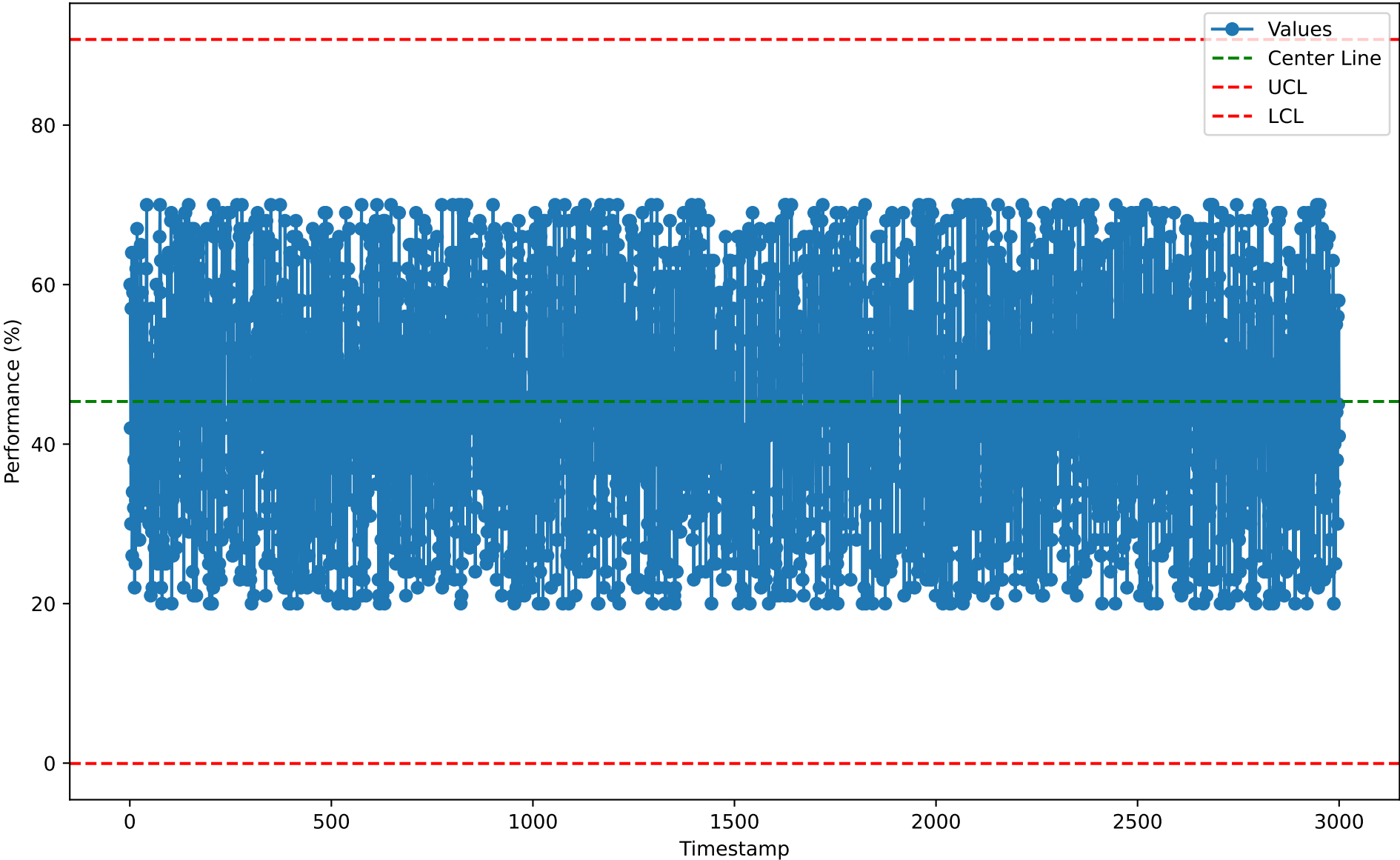
Individuals Chart for BRM10115 (2026-01-07)
