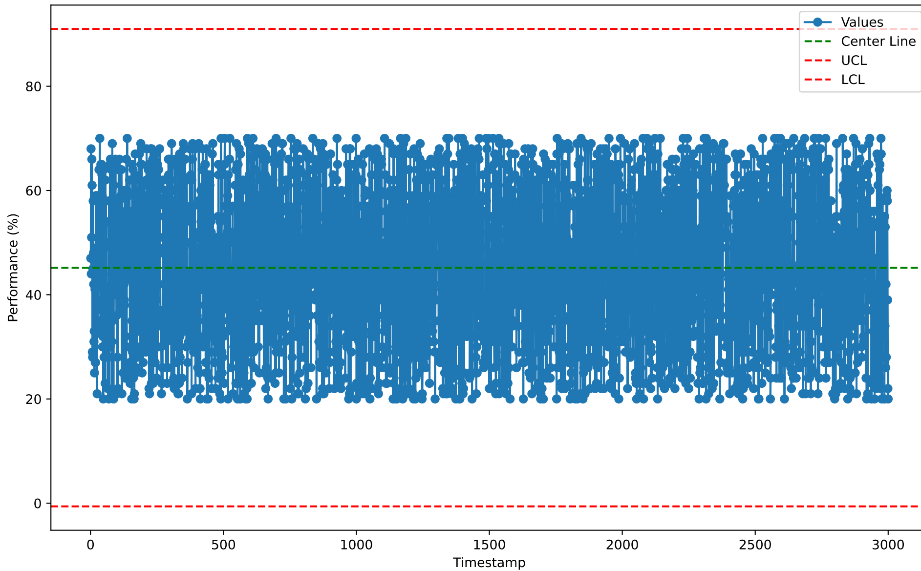
Individuals Chart for LYP10103 (2026-01-07)
