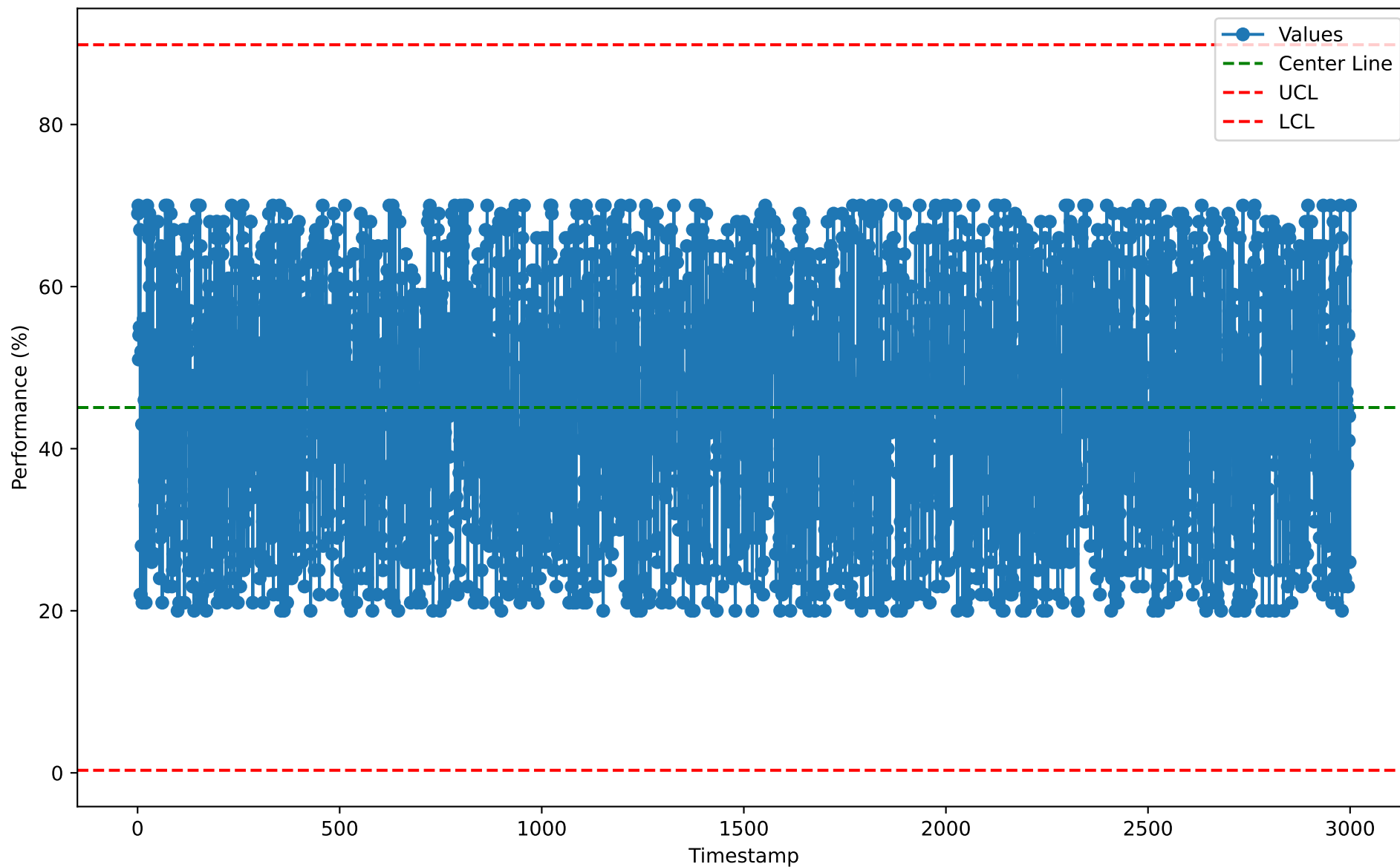
Individuals Chart for LYP10106 (2026-01-07)
