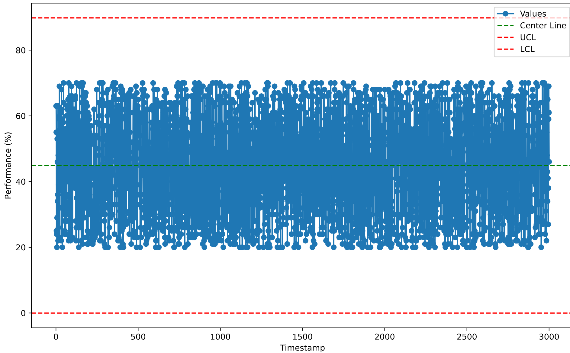
Individuals Chart for SSP10103 (2026-01-07)
