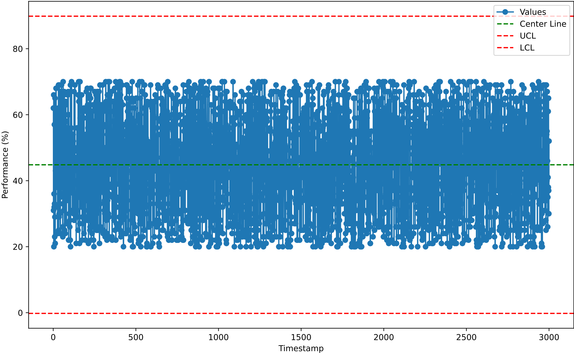
Individuals Chart for SFO10106 (2026-01-07)
