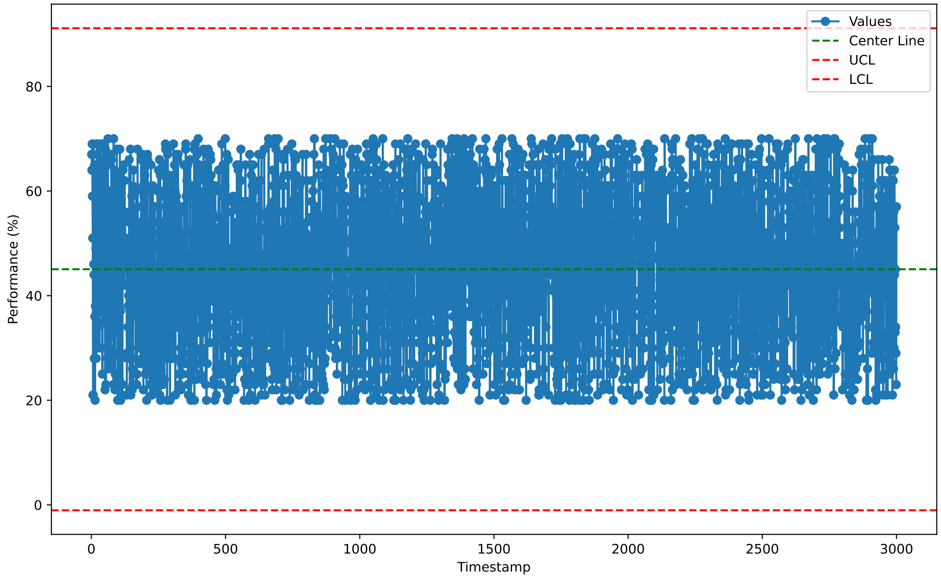
Individuals Chart for LYP10105 (2026-01-07)
