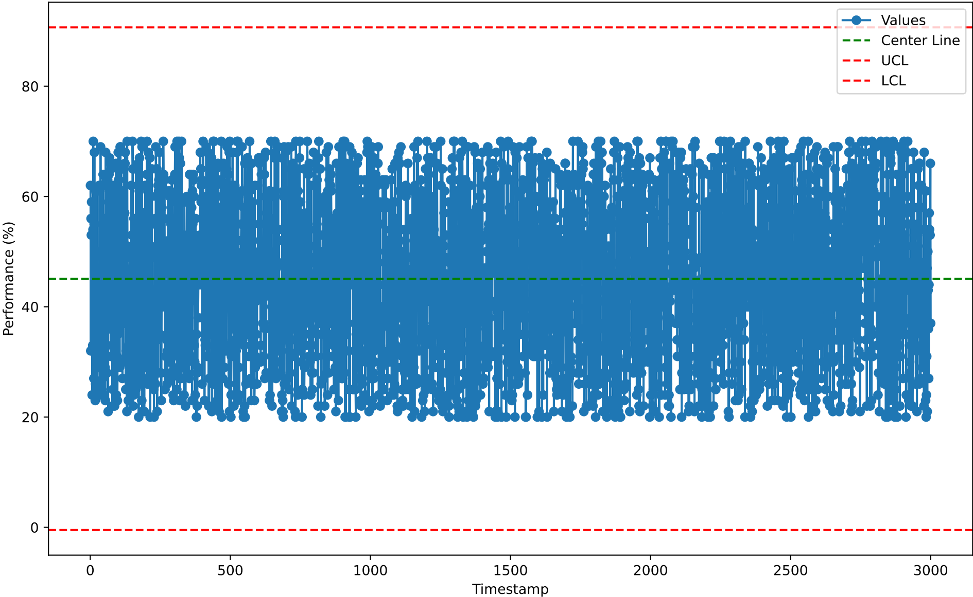
Individuals Chart for MKC10111 (2026-01-07)
