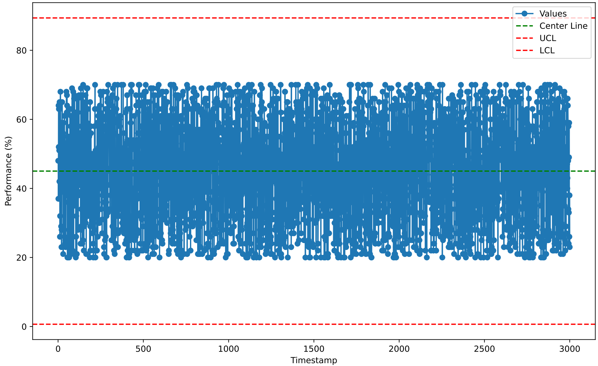
Individuals Chart for LYP10117 (2026-01-07)
