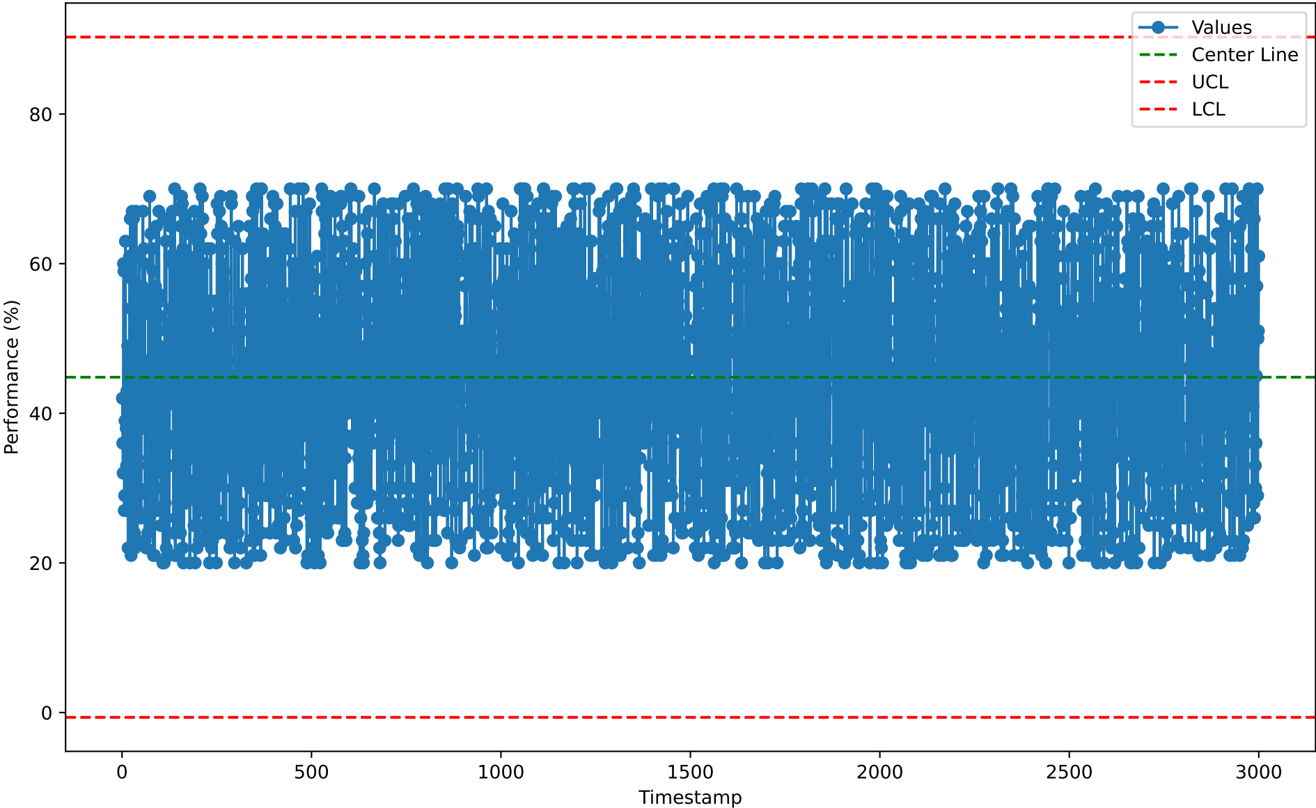
Individuals Chart for BRM10101 (2026-01-07)
