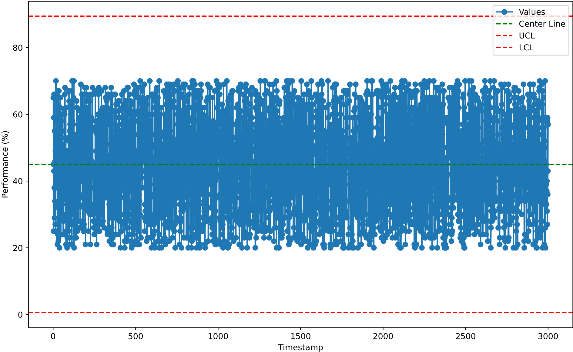
Individuals Chart for MKC10112 (2026-01-07)
