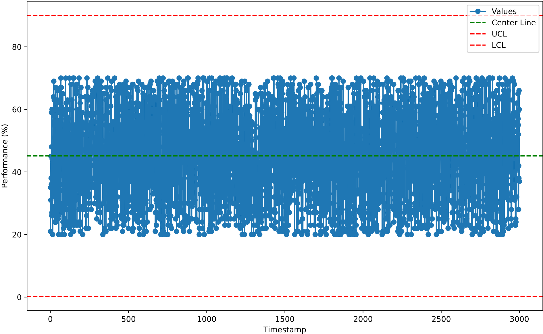
Individuals Chart for MKC10107 (2026-01-07)
