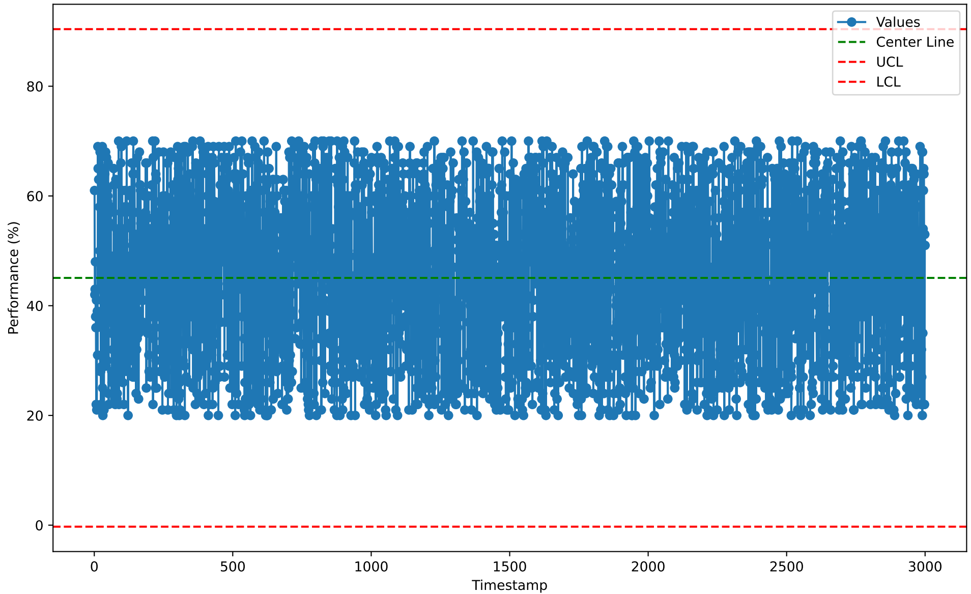
Individuals Chart for LYP10101 (2026-01-07)
