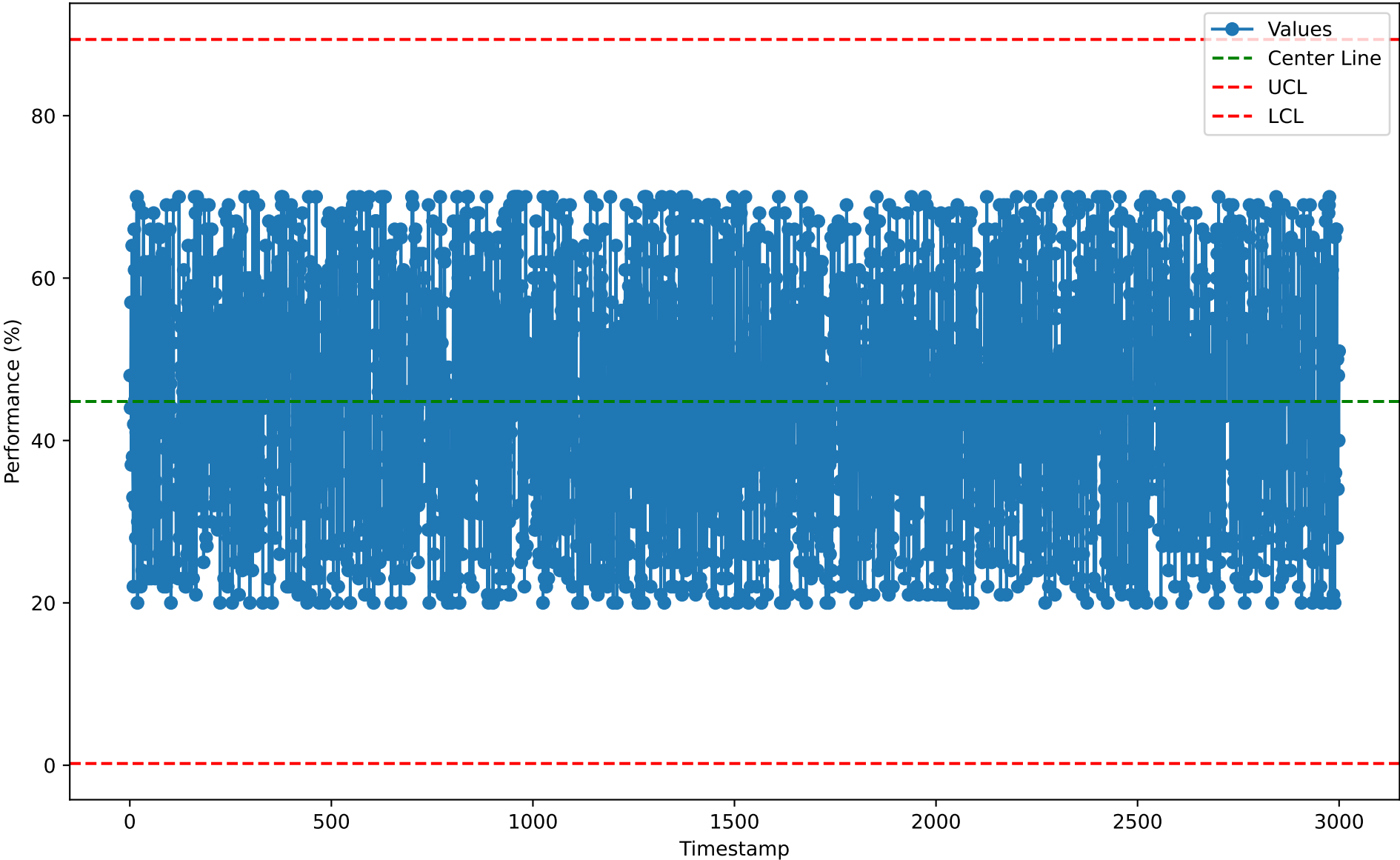
Individuals Chart for SFO10101 (2026-01-07)
