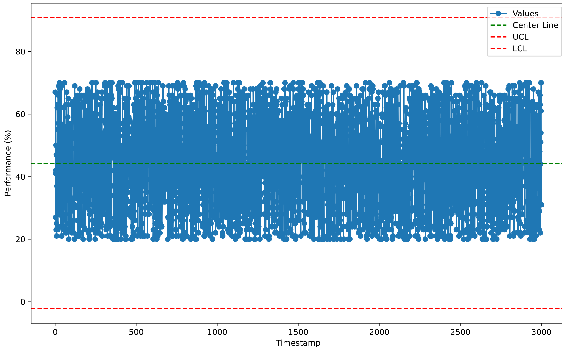
Individuals Chart for LYP10114 (2026-01-07)
