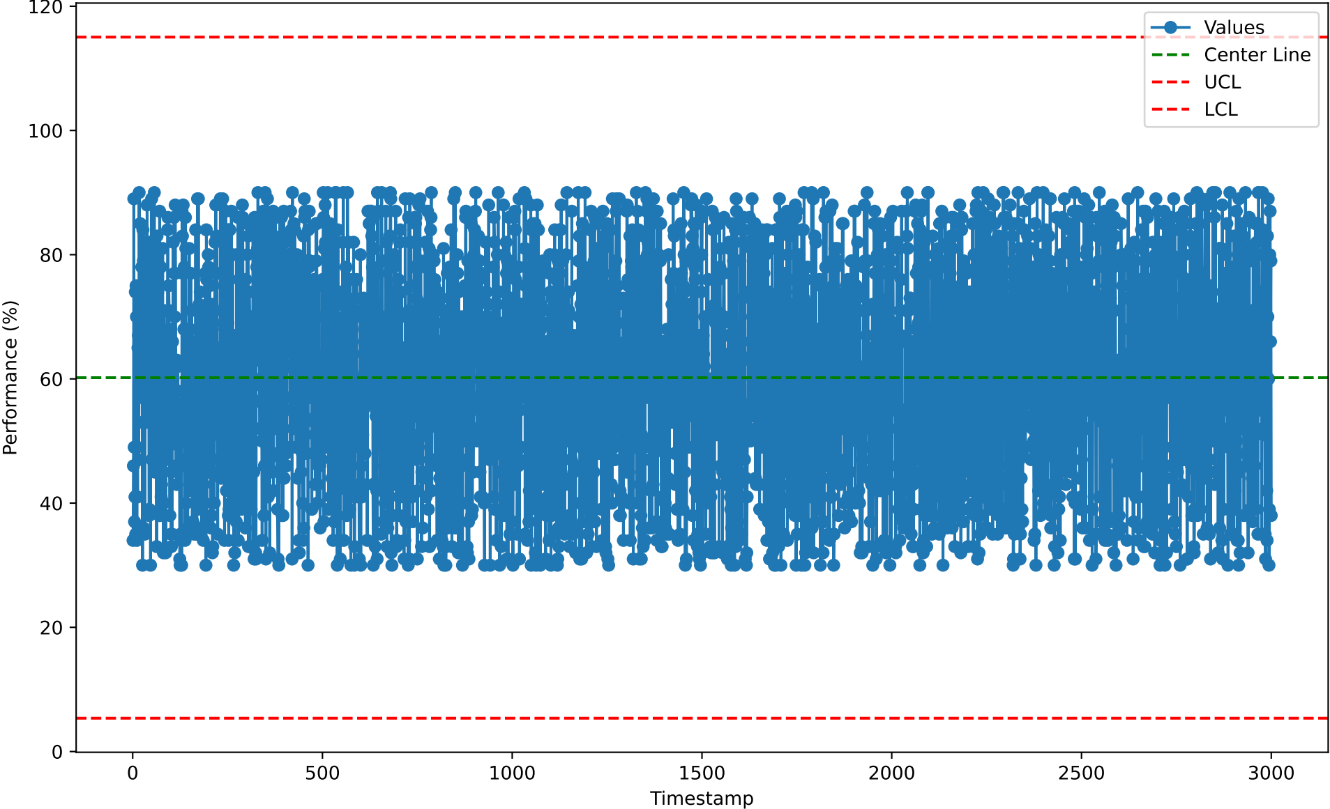
Individuals Chart for RTR10119 (2026-01-07)
