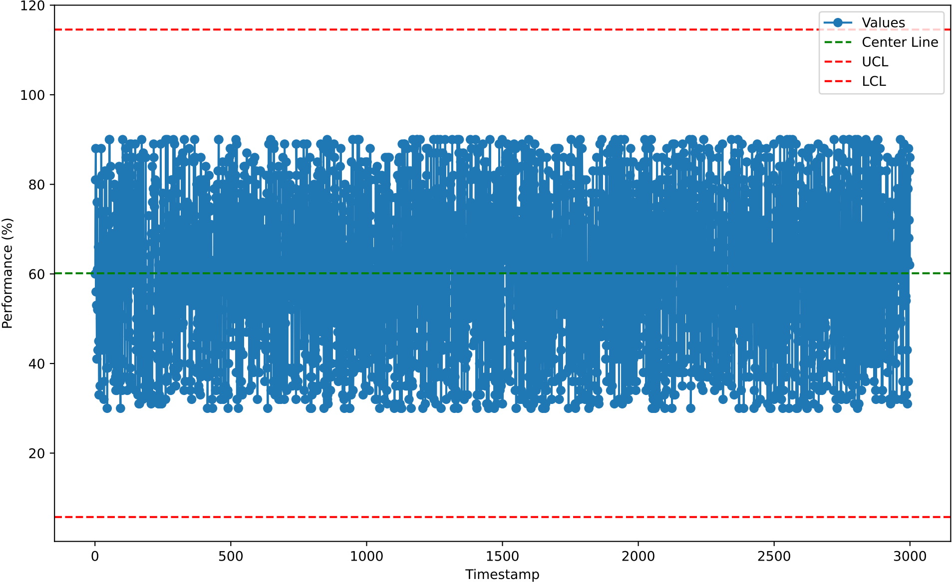
Individuals Chart for RST10111 (2026-01-07)
