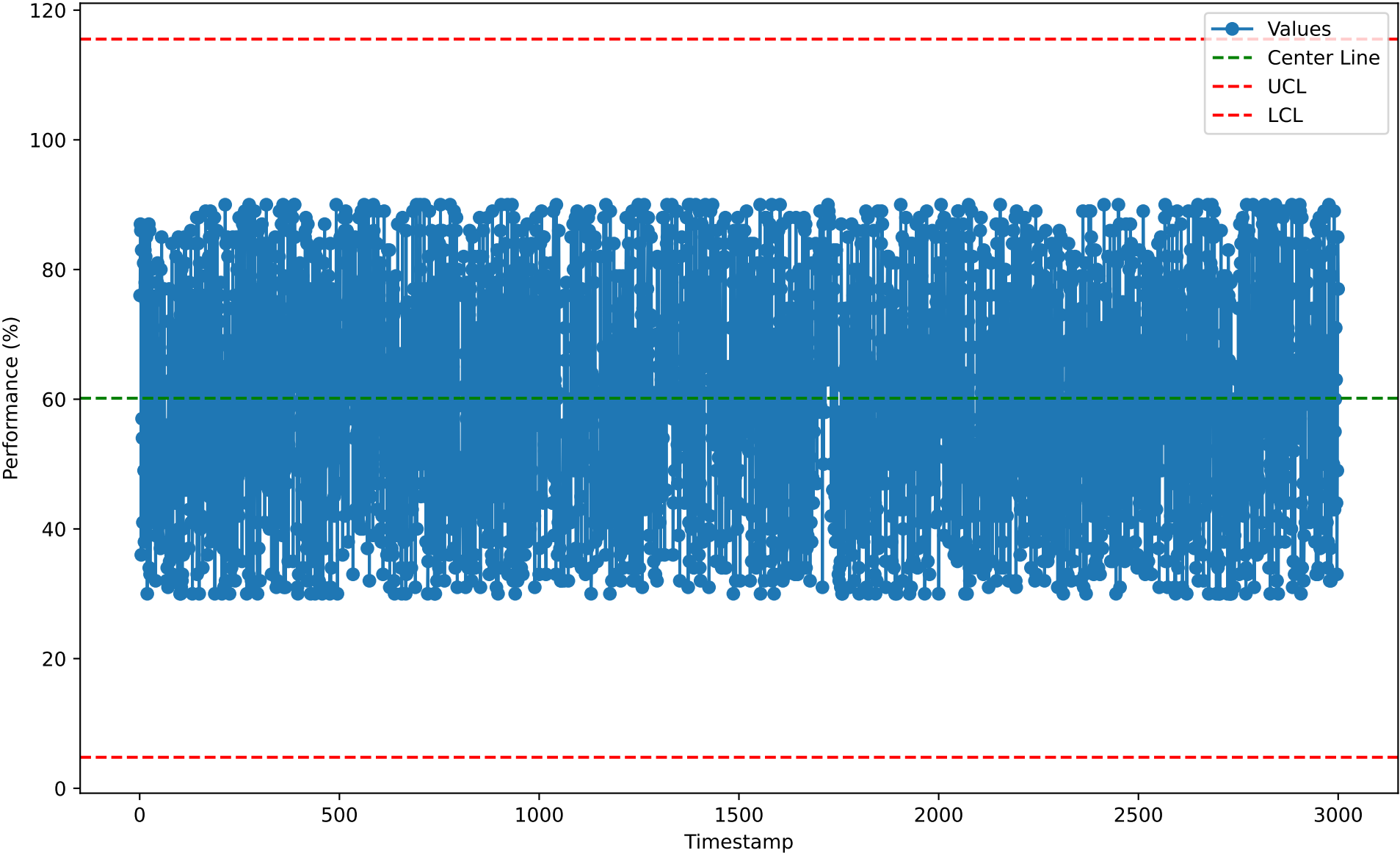
Individuals Chart for RDA10115 (2026-01-07)
