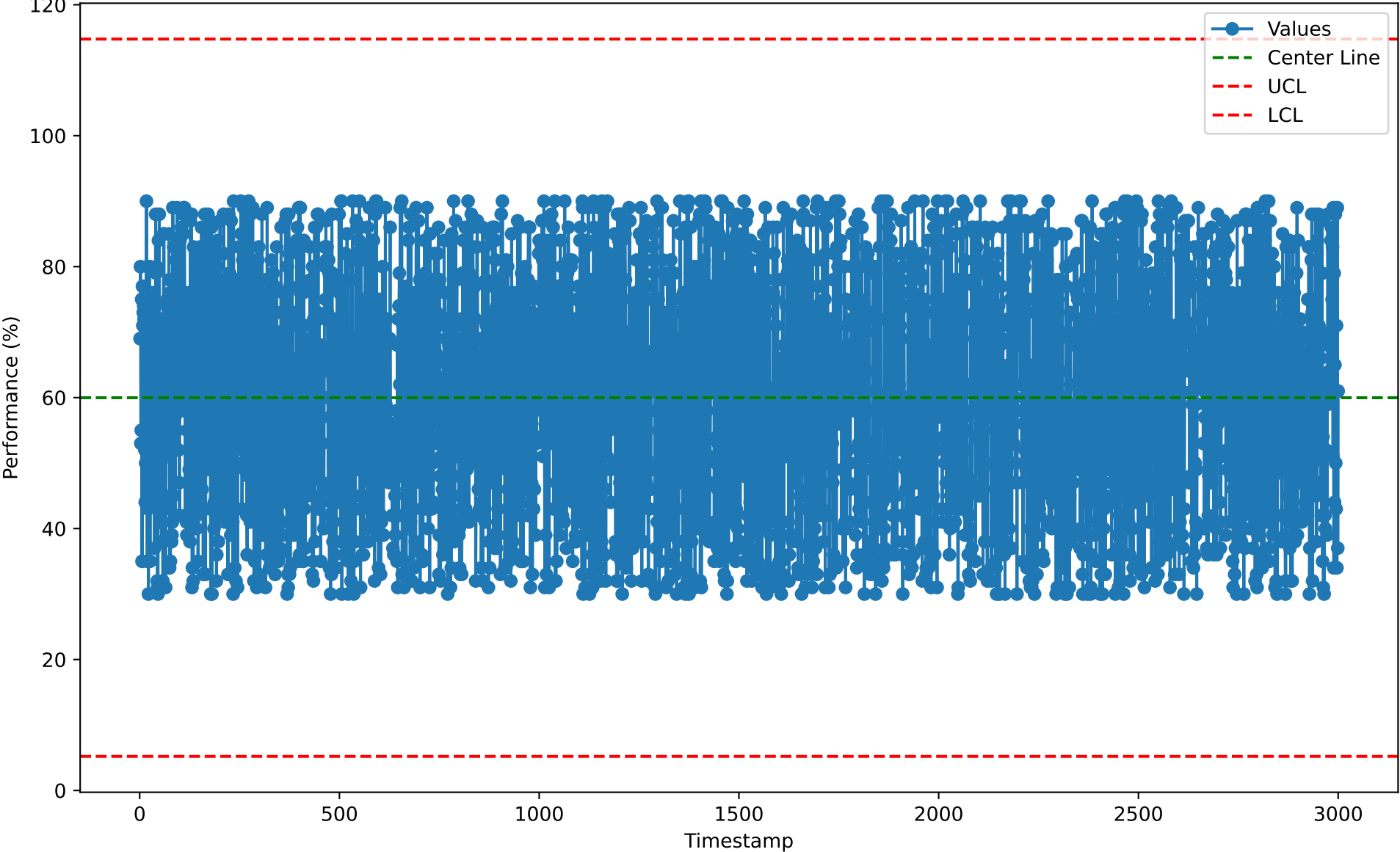
Individuals Chart for RSU10109 (2026-01-07)
