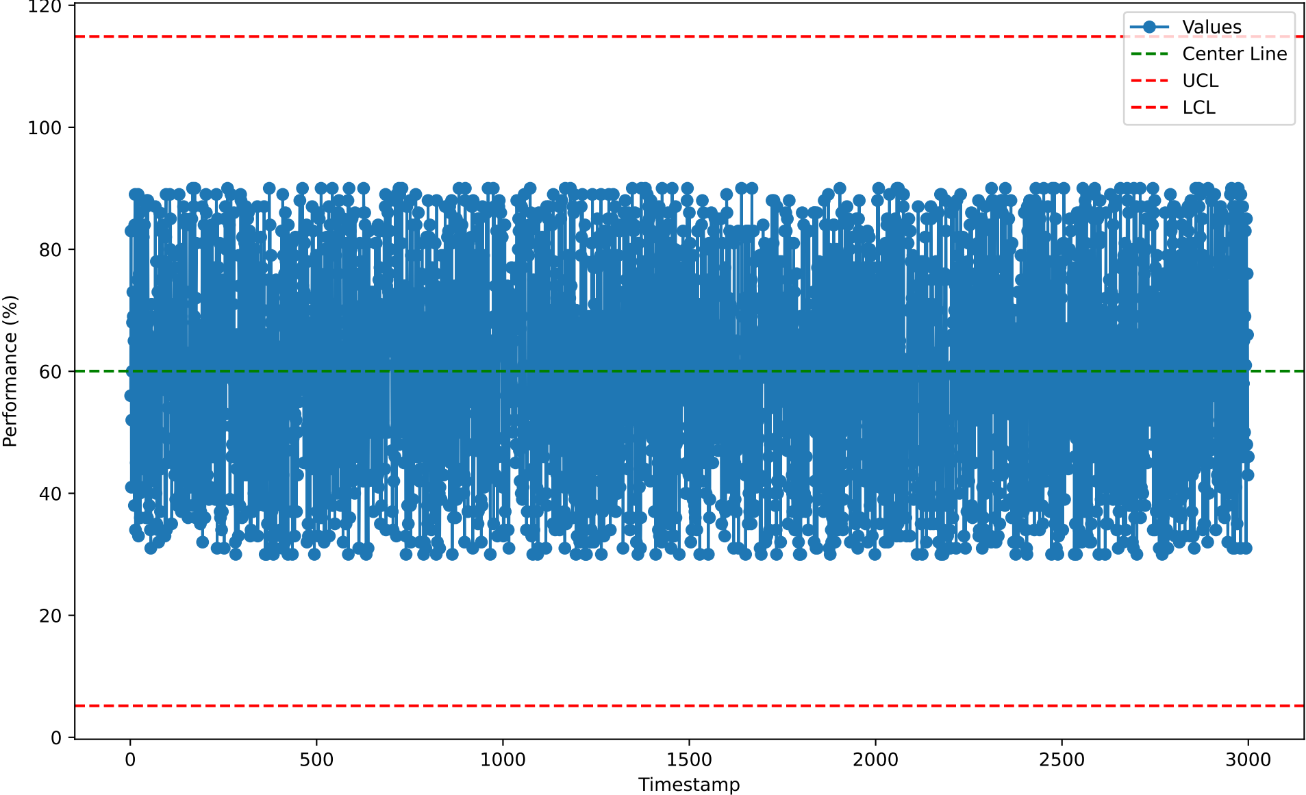
Individuals Chart for RTR10104 (2026-01-07)
