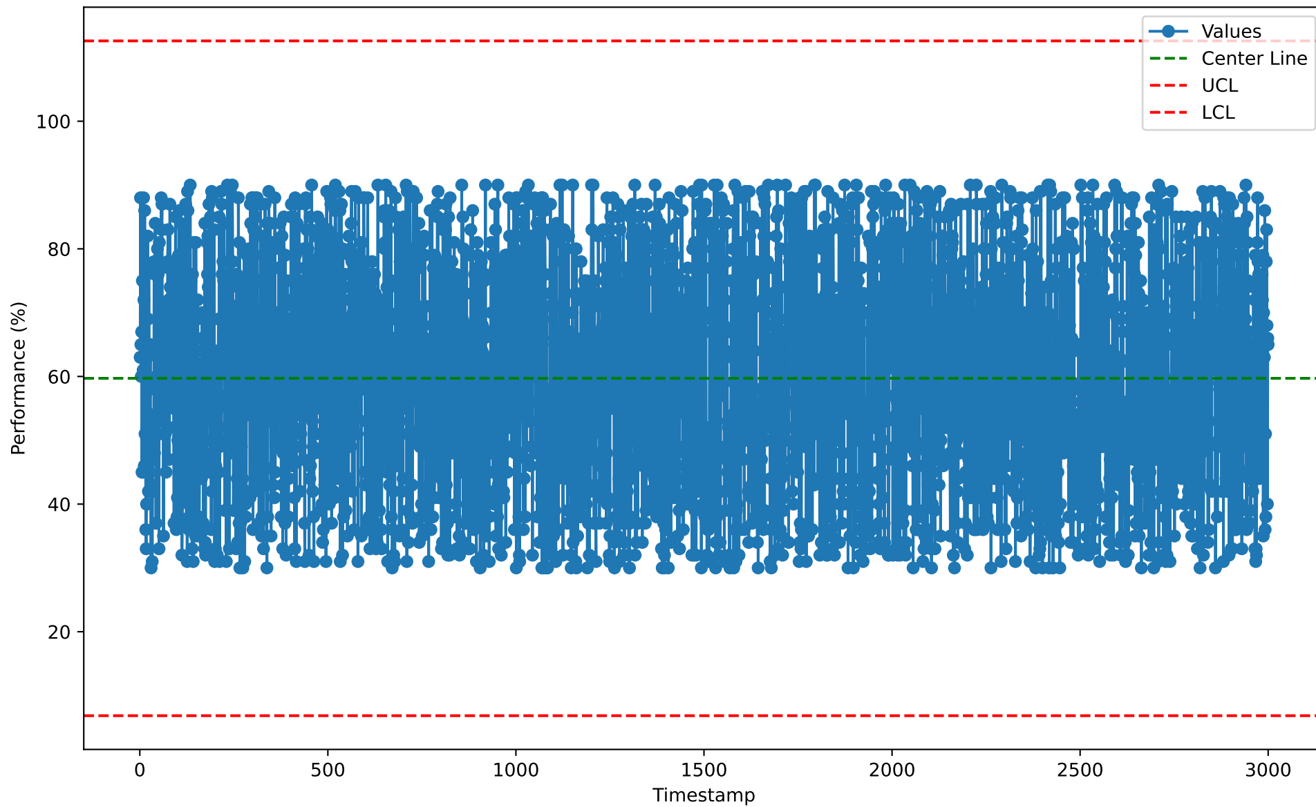
Individuals Chart for RSL10107 (2026-01-07)
