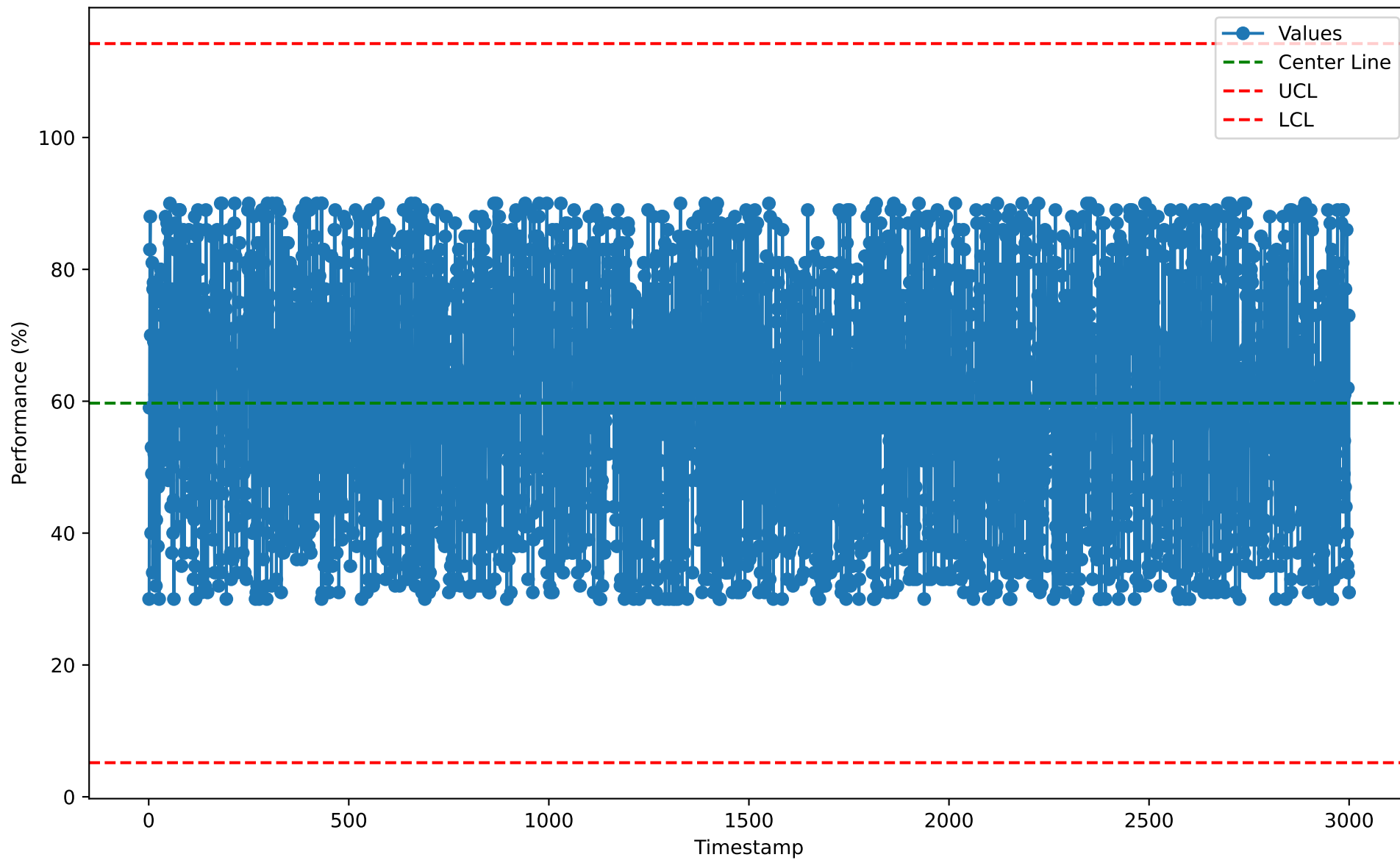
Individuals Chart for RSL10114 (2026-01-07)
