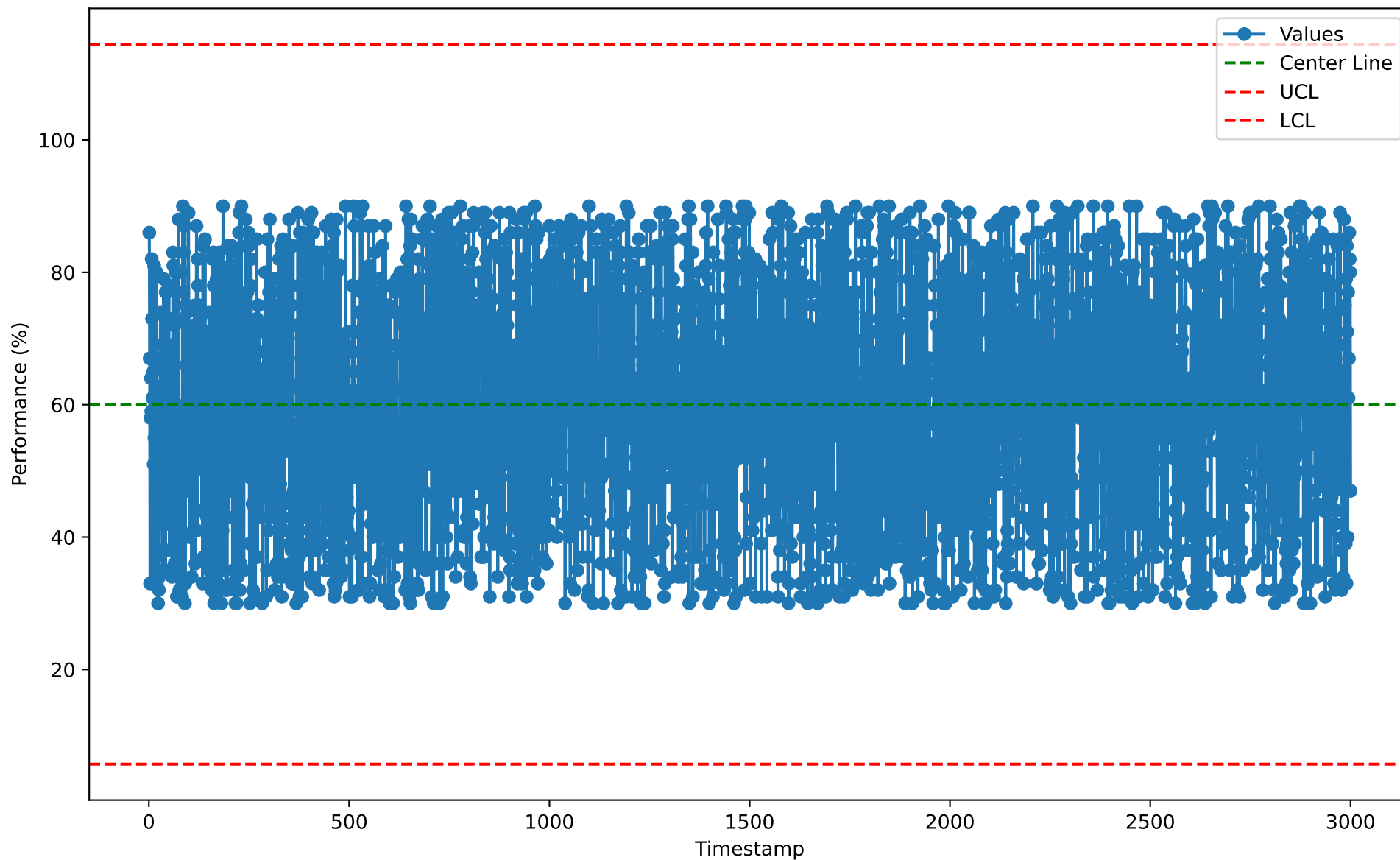
Individuals Chart for RCM10110 (2026-01-07)
