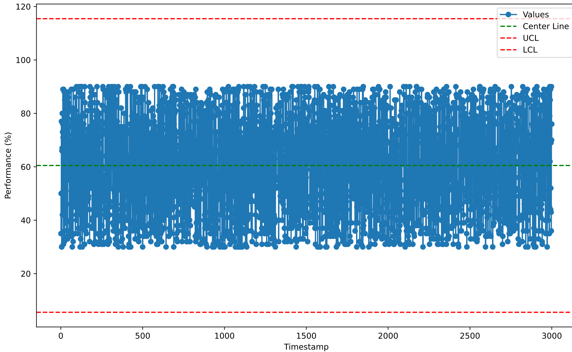
Individuals Chart for RSL10118 (2026-01-07)
