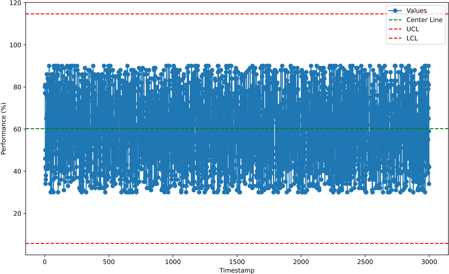
Individuals Chart for RPR10118 (2026-01-07)
