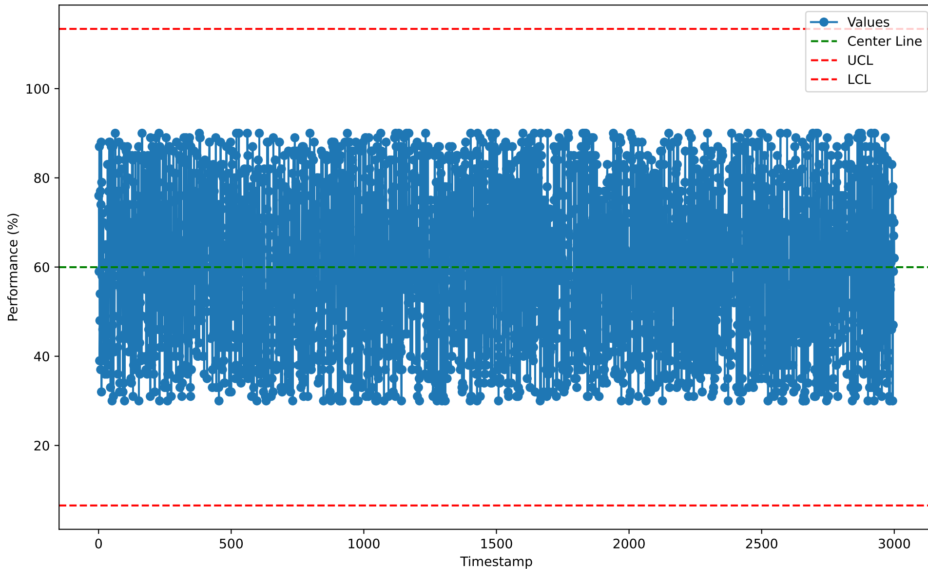
Individuals Chart for RSL10117 (2026-01-07)
