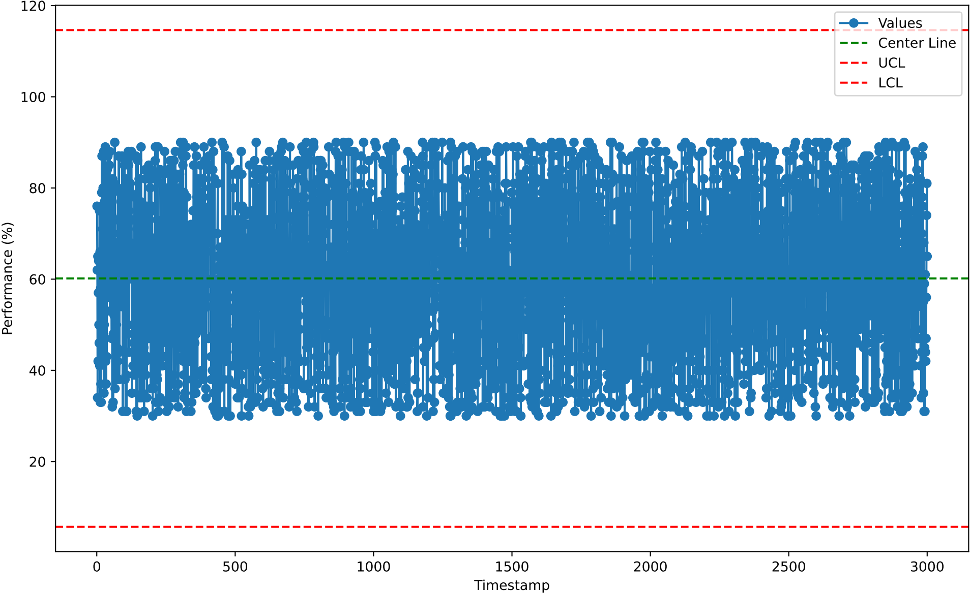
Individuals Chart for RDA10119 (2026-01-07)
