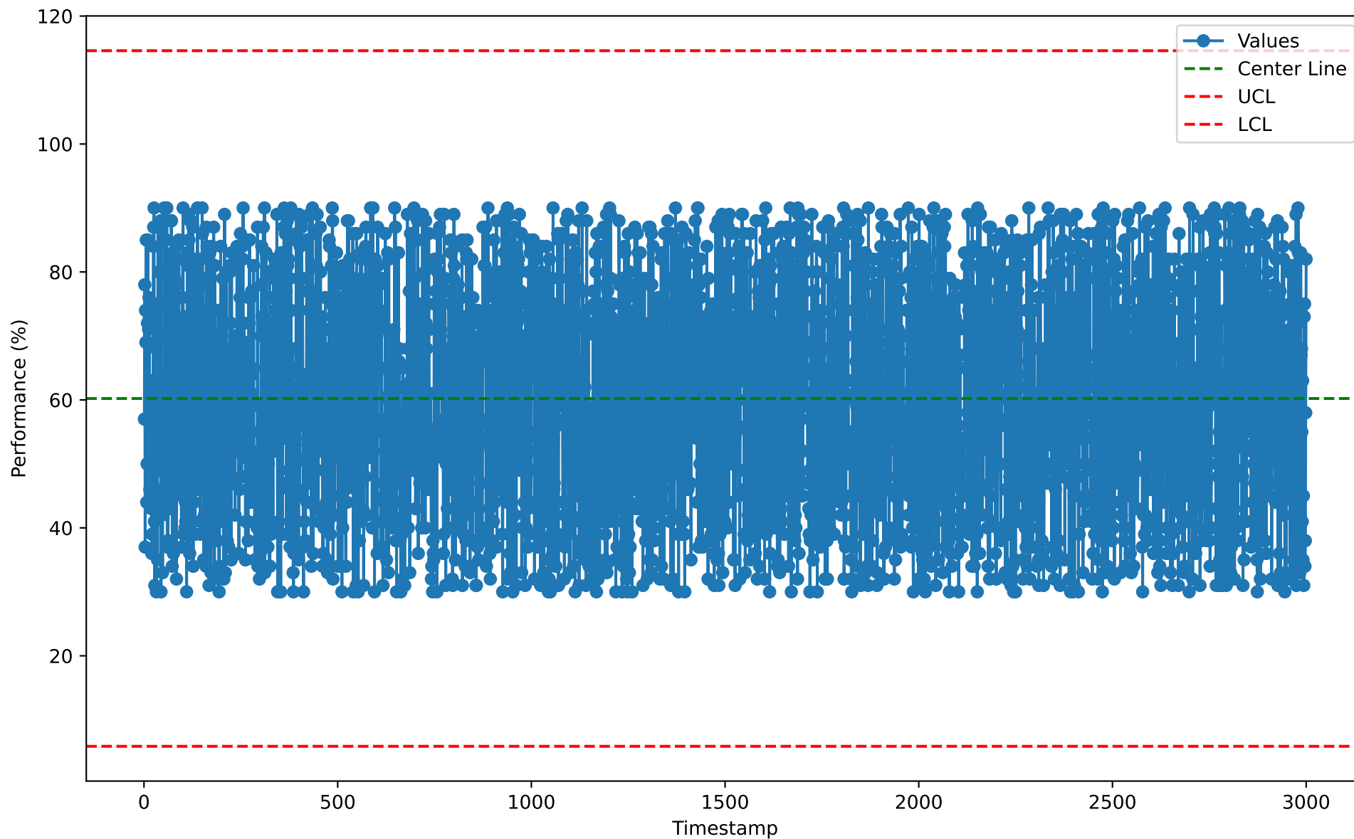
Individuals Chart for RSL10119 (2026-01-07)
