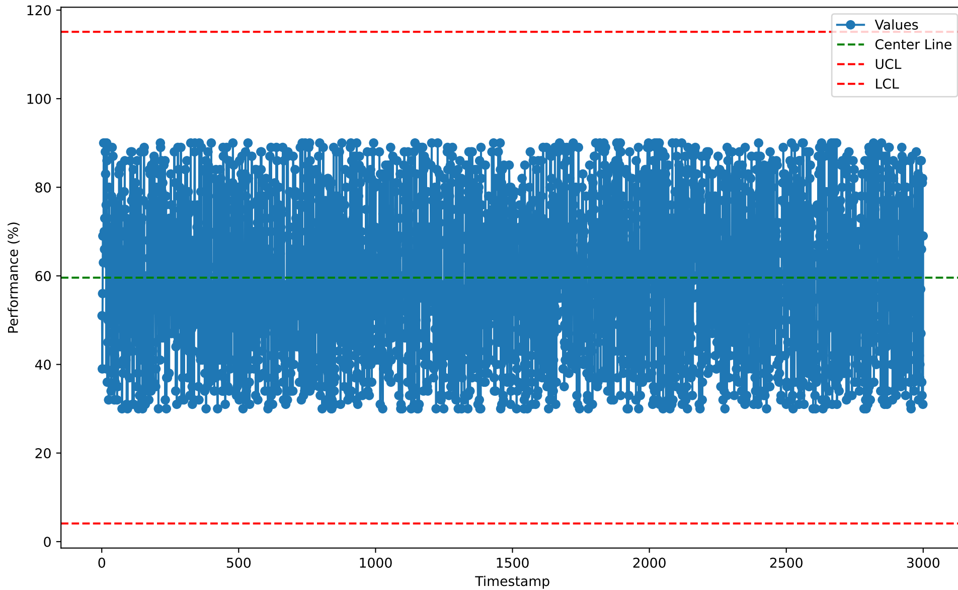
Individuals Chart for RSL10109 (2026-01-07)
