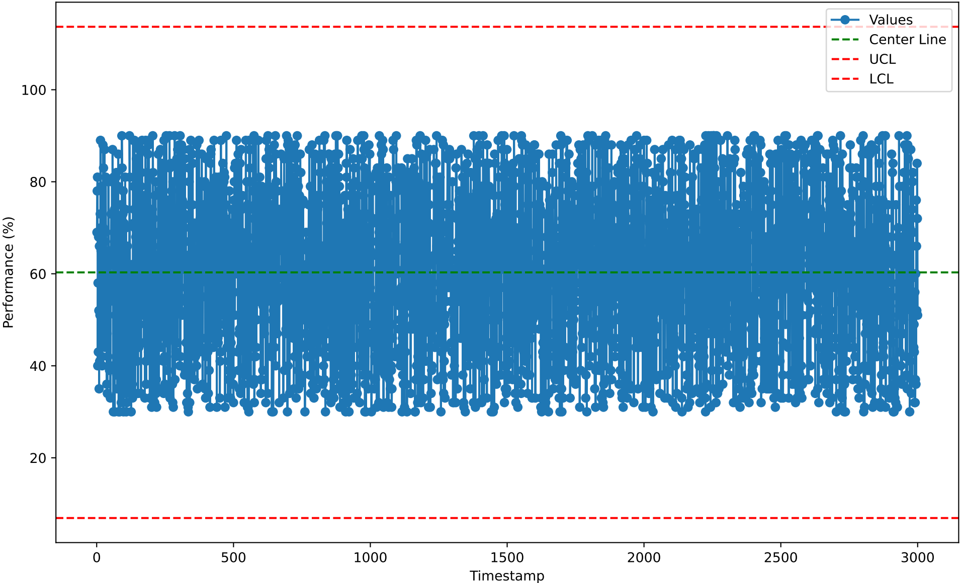
Individuals Chart for RST10102 (2026-01-07)
