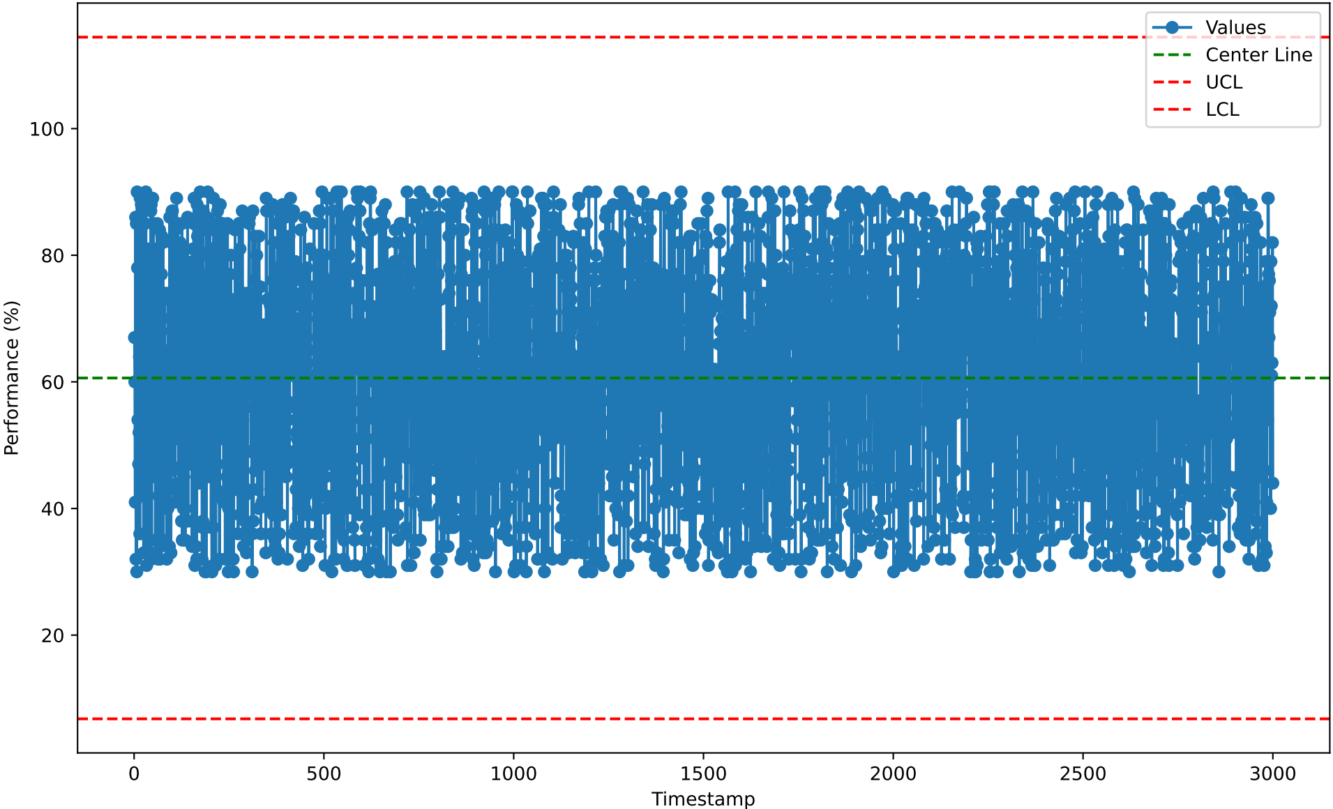
Individuals Chart for RMR10105 (2026-01-07)
