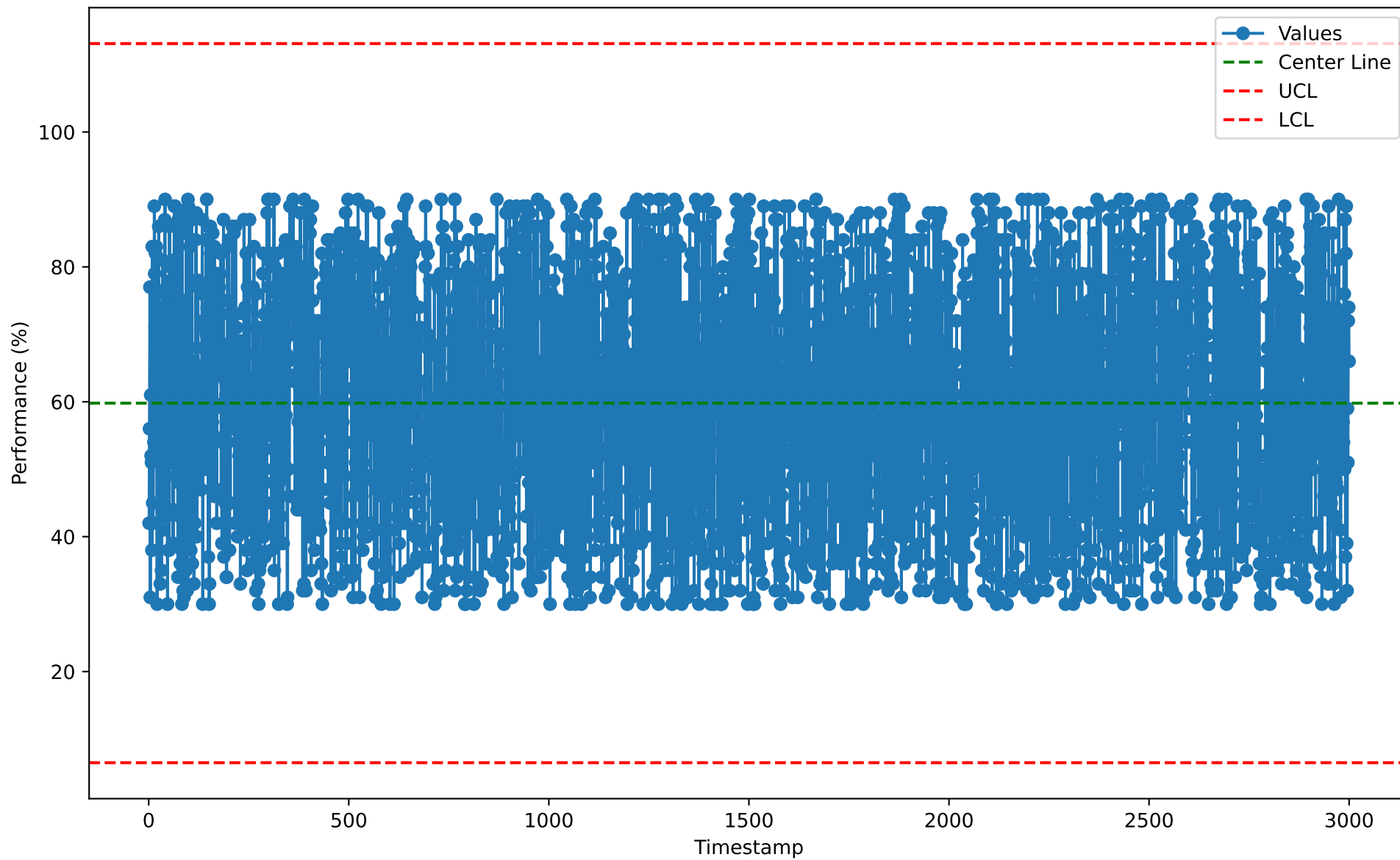
Individuals Chart for RCM10112 (2026-01-07)
