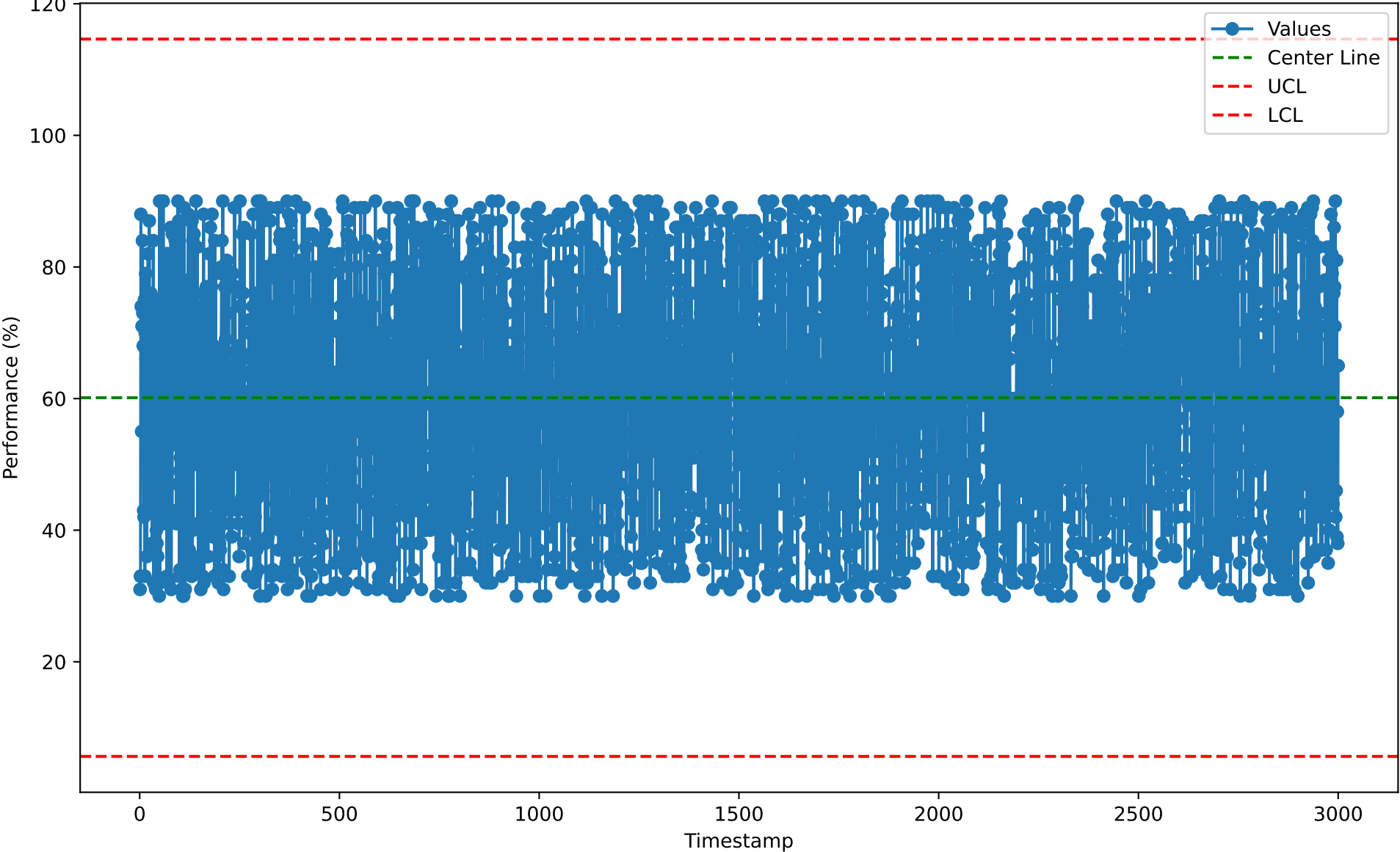
Individuals Chart for RDA10109 (2026-01-07)
