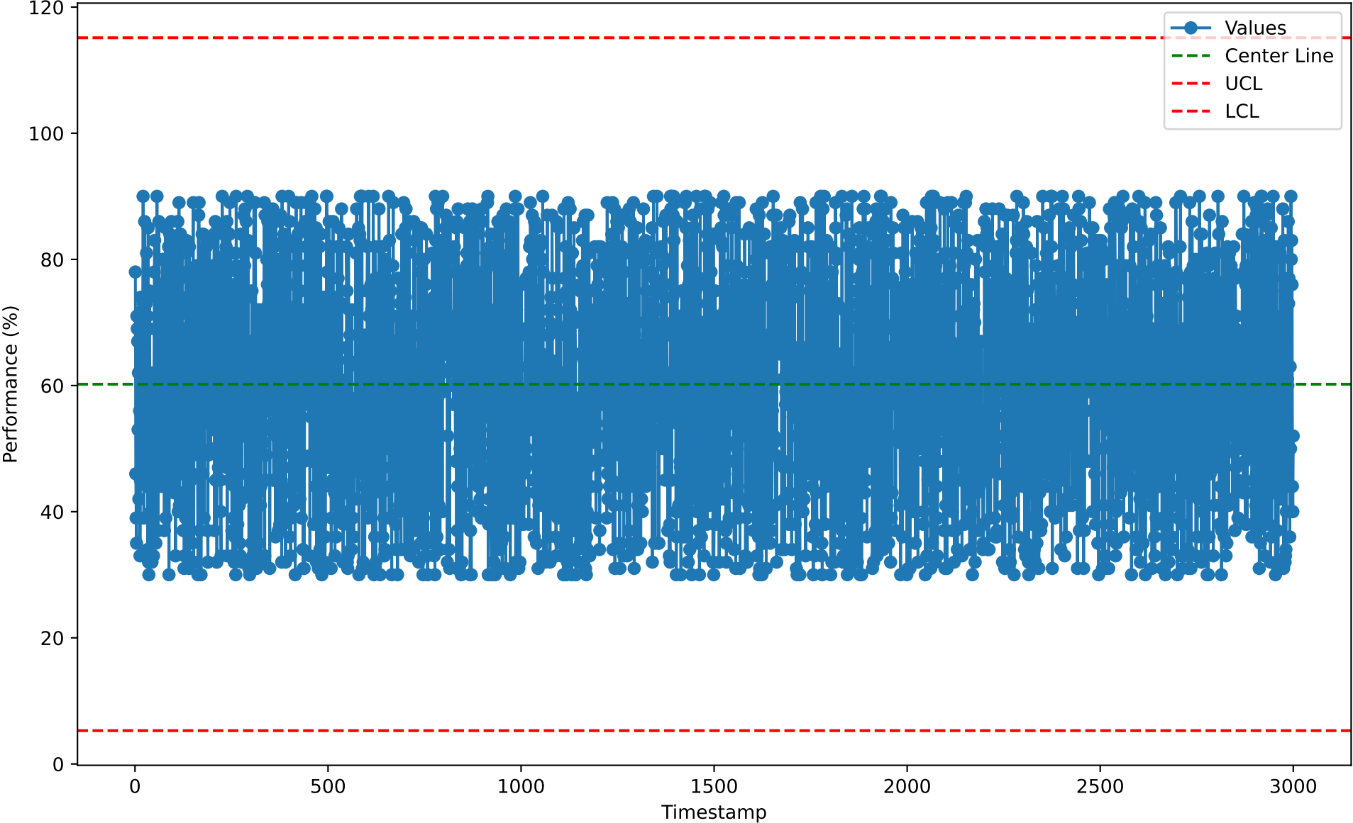
Individuals Chart for RSU10104 (2026-01-07)
