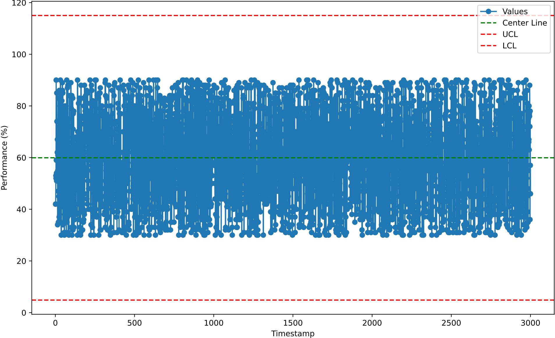
Individuals Chart for RMR10109 (2026-01-07)
