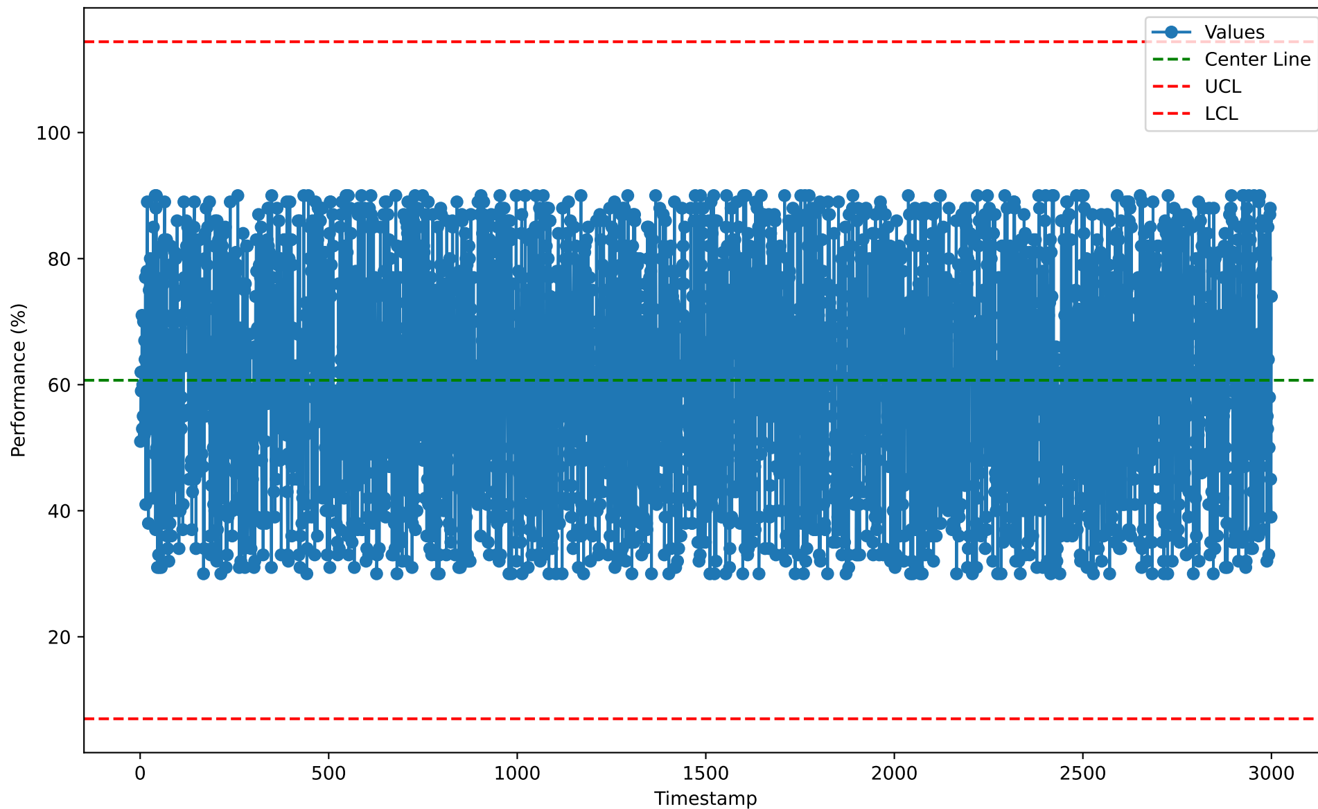
Individuals Chart for RSL10105 (2026-01-07)
