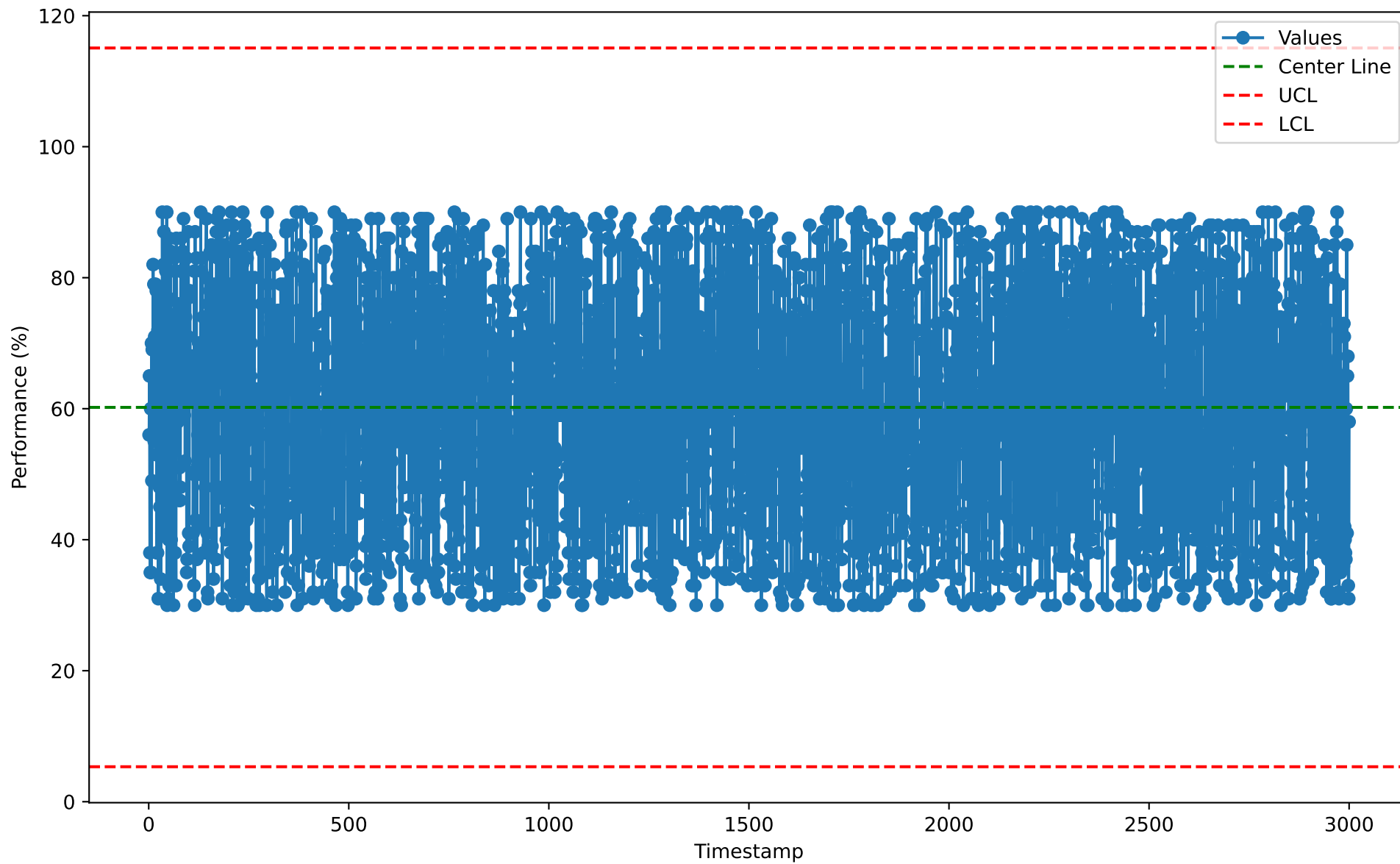
Individuals Chart for RCM10107 (2026-01-07)
