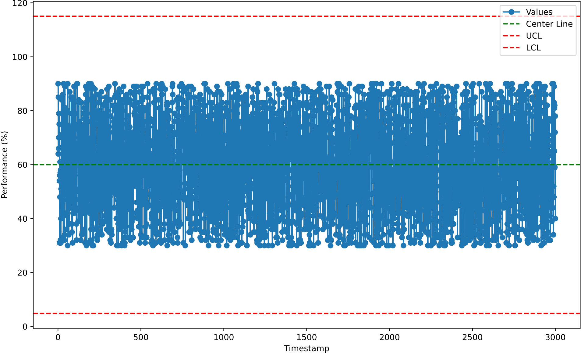
Individuals Chart for RSU10112 (2026-01-07)
