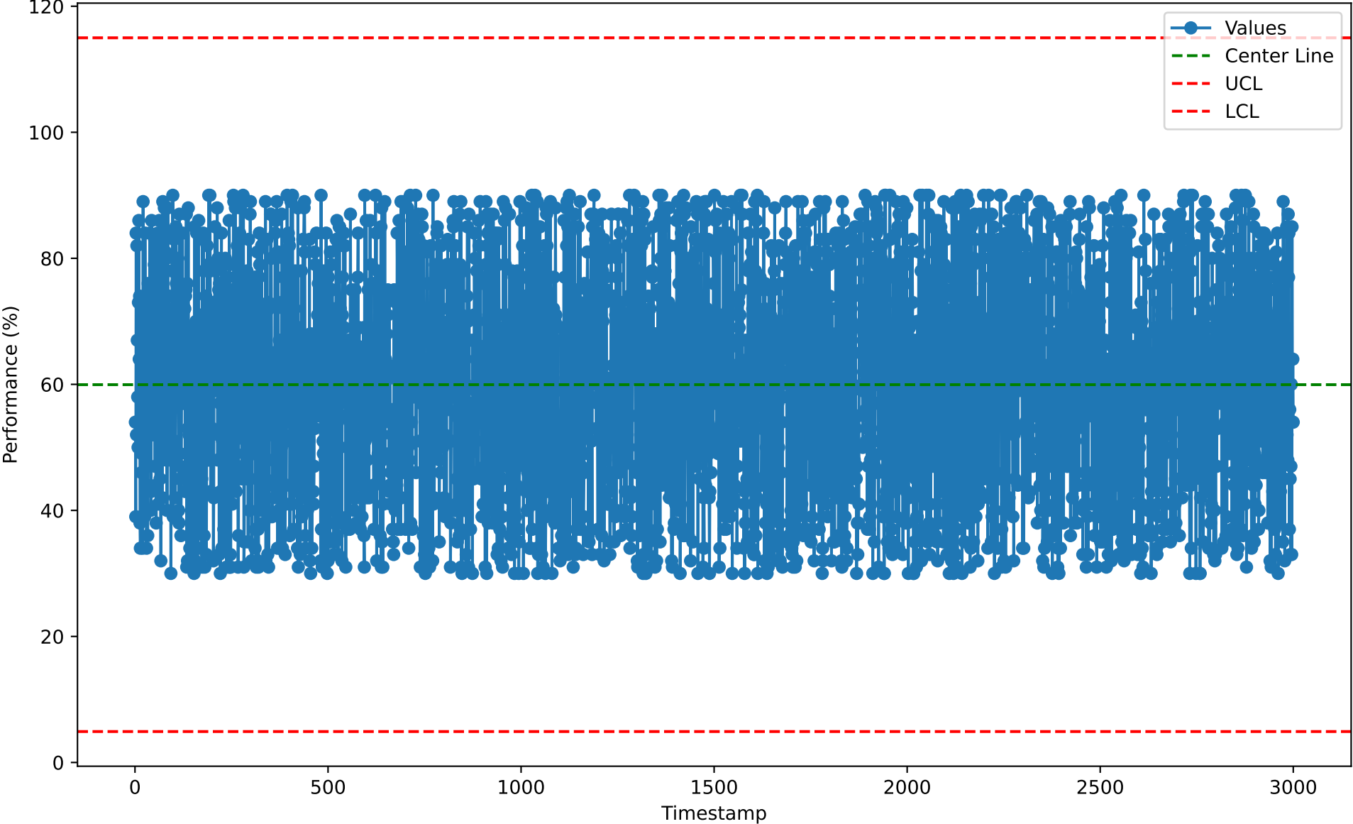
Individuals Chart for RSU10108 (2026-01-07)
