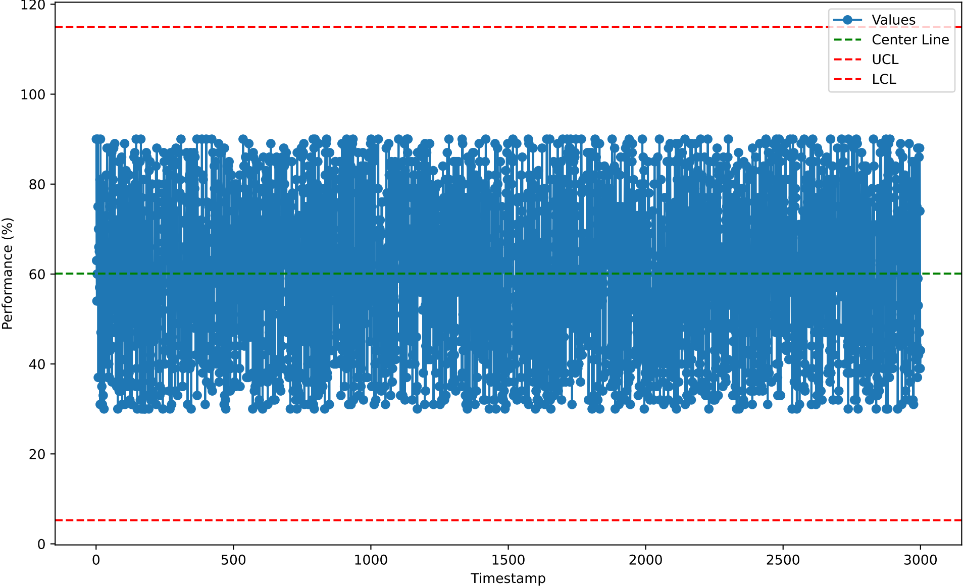
Individuals Chart for ROR10112 (2026-01-07)
