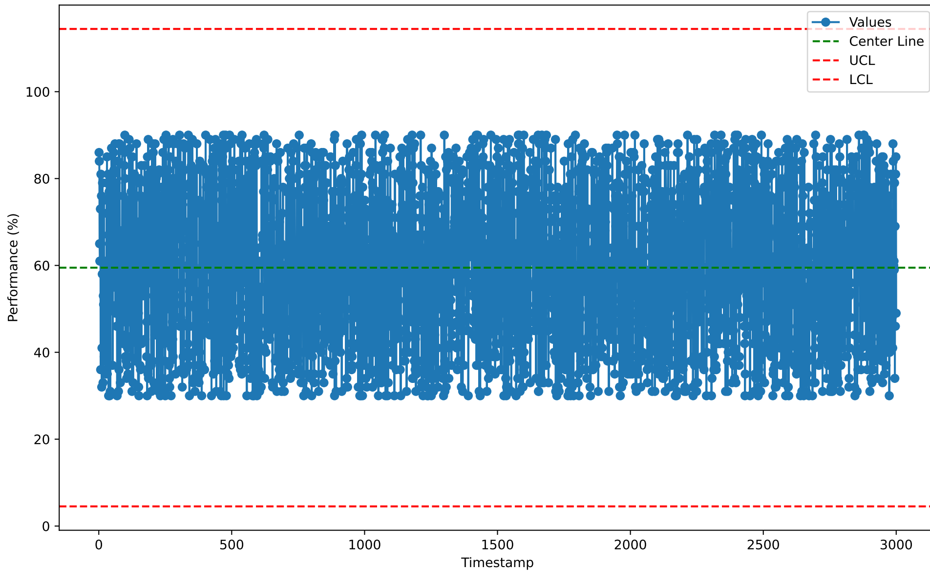
Individuals Chart for RSL10115 (2026-01-07)
