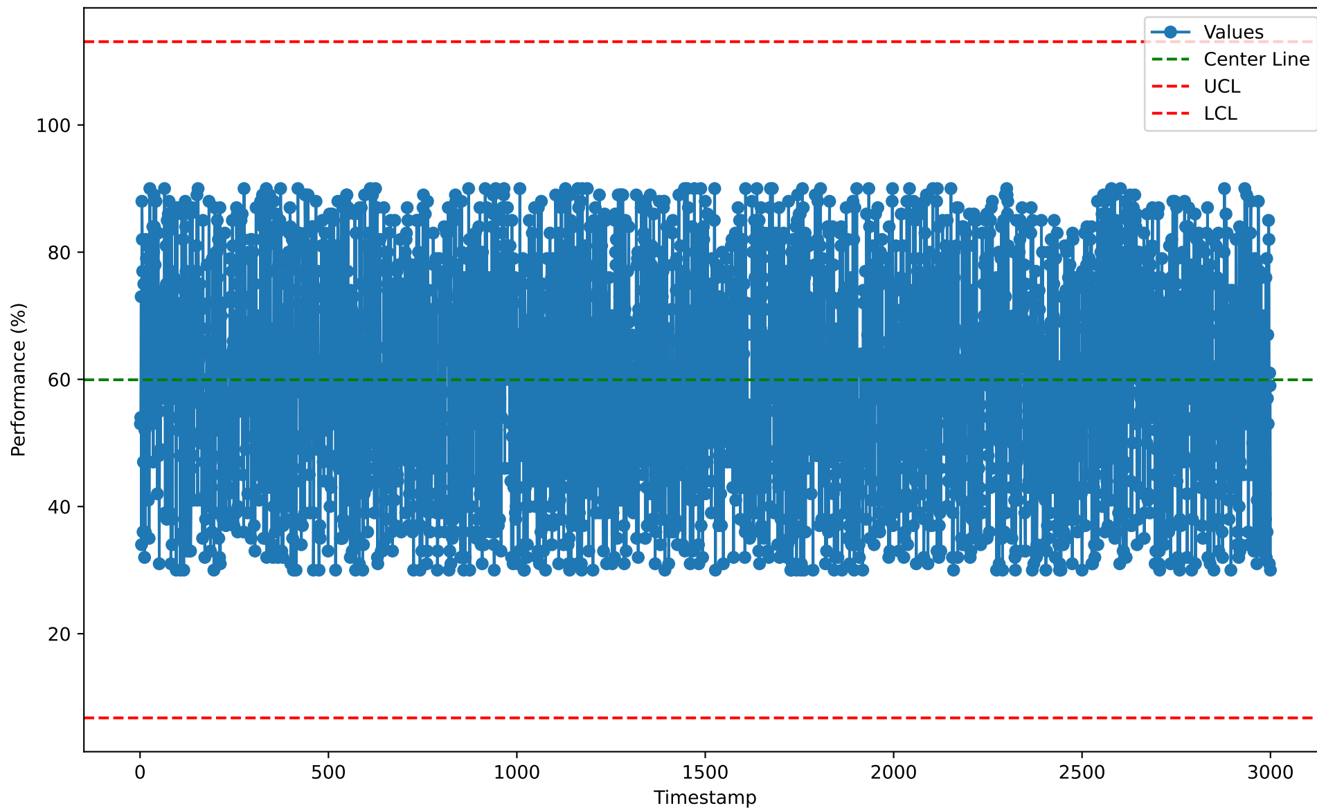
Individuals Chart for RCD10103 (2026-01-07)
