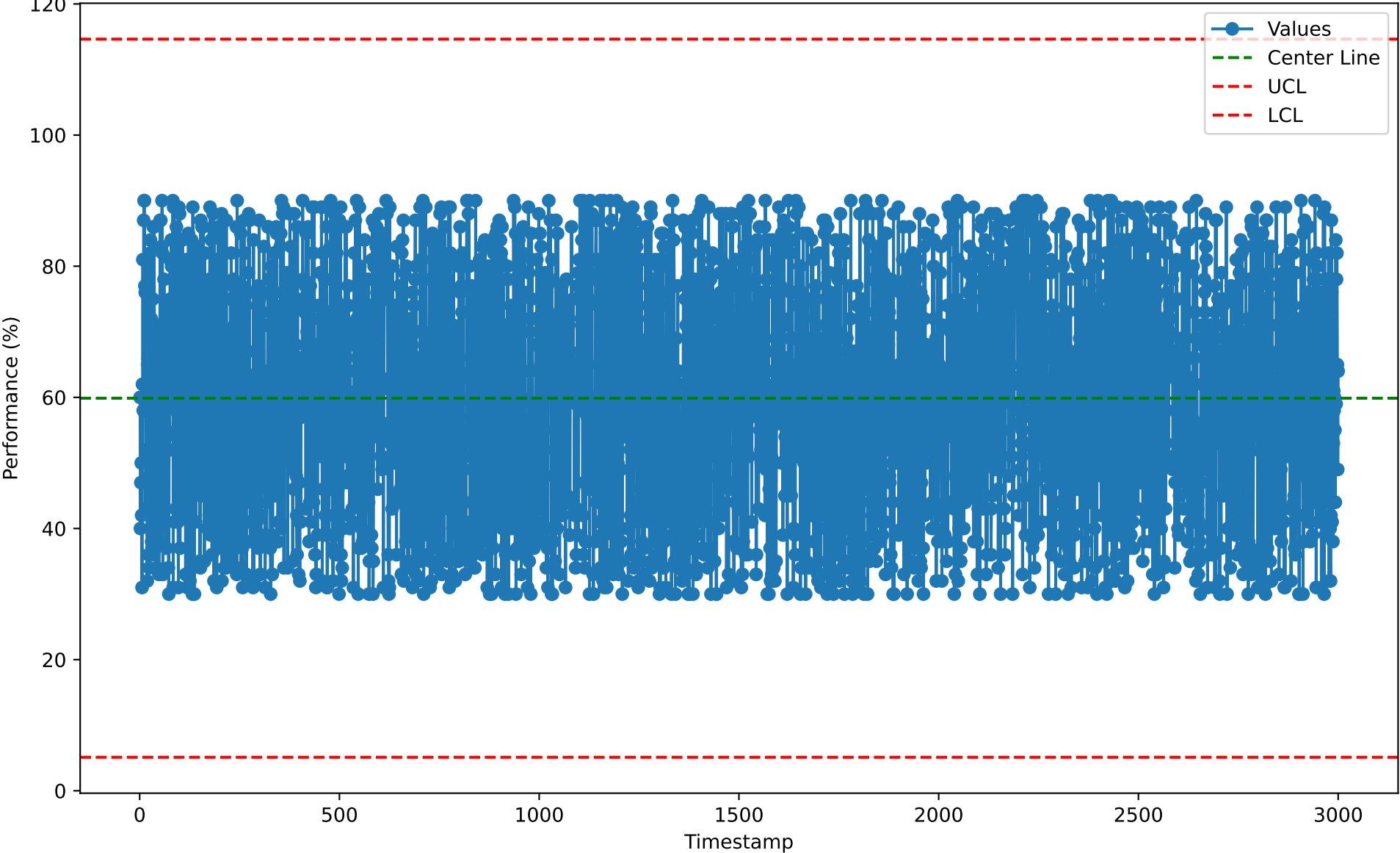
Individuals Chart for RMR10106 (2026-01-07)
