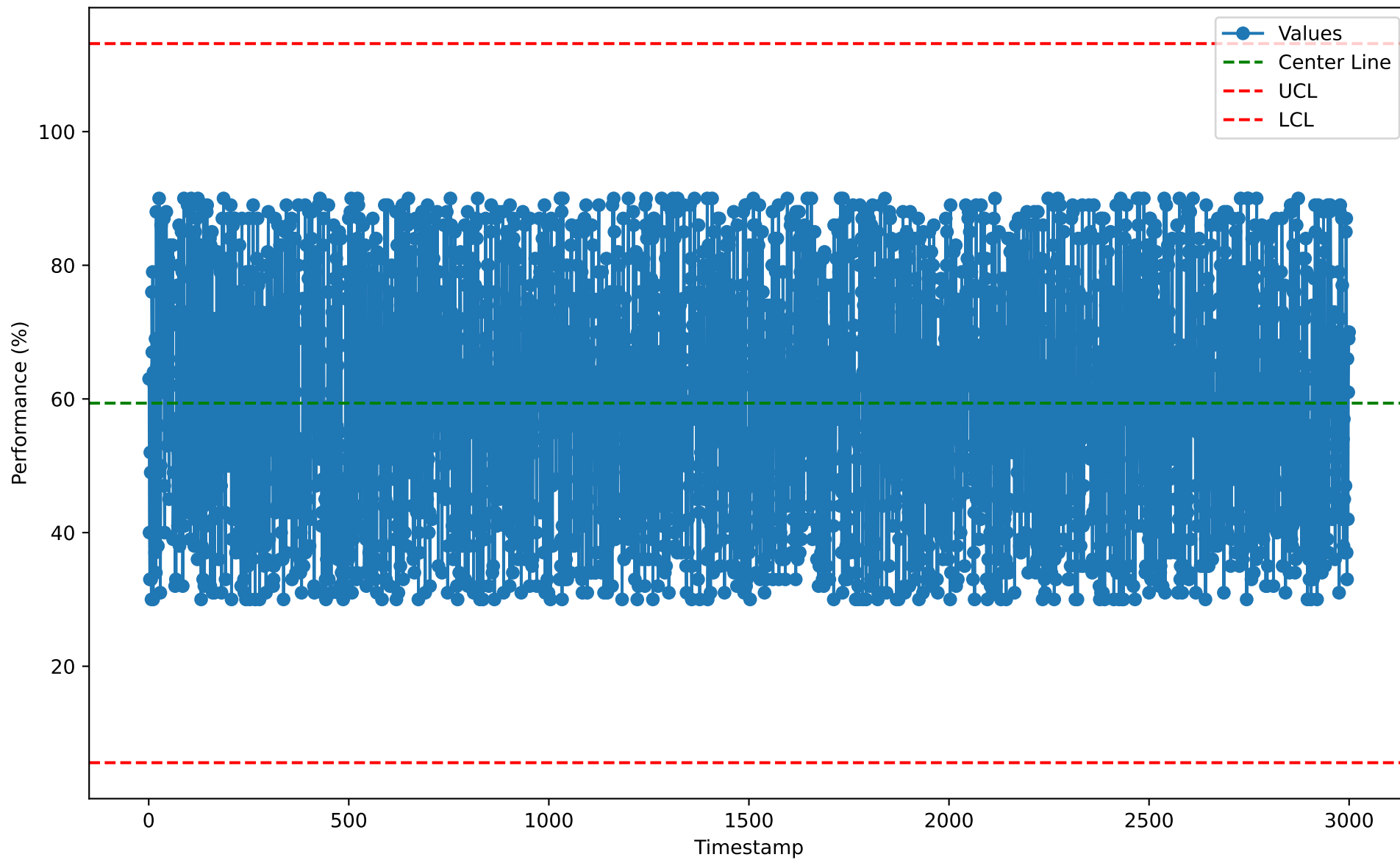
Individuals Chart for RSL10104 (2026-01-07)
