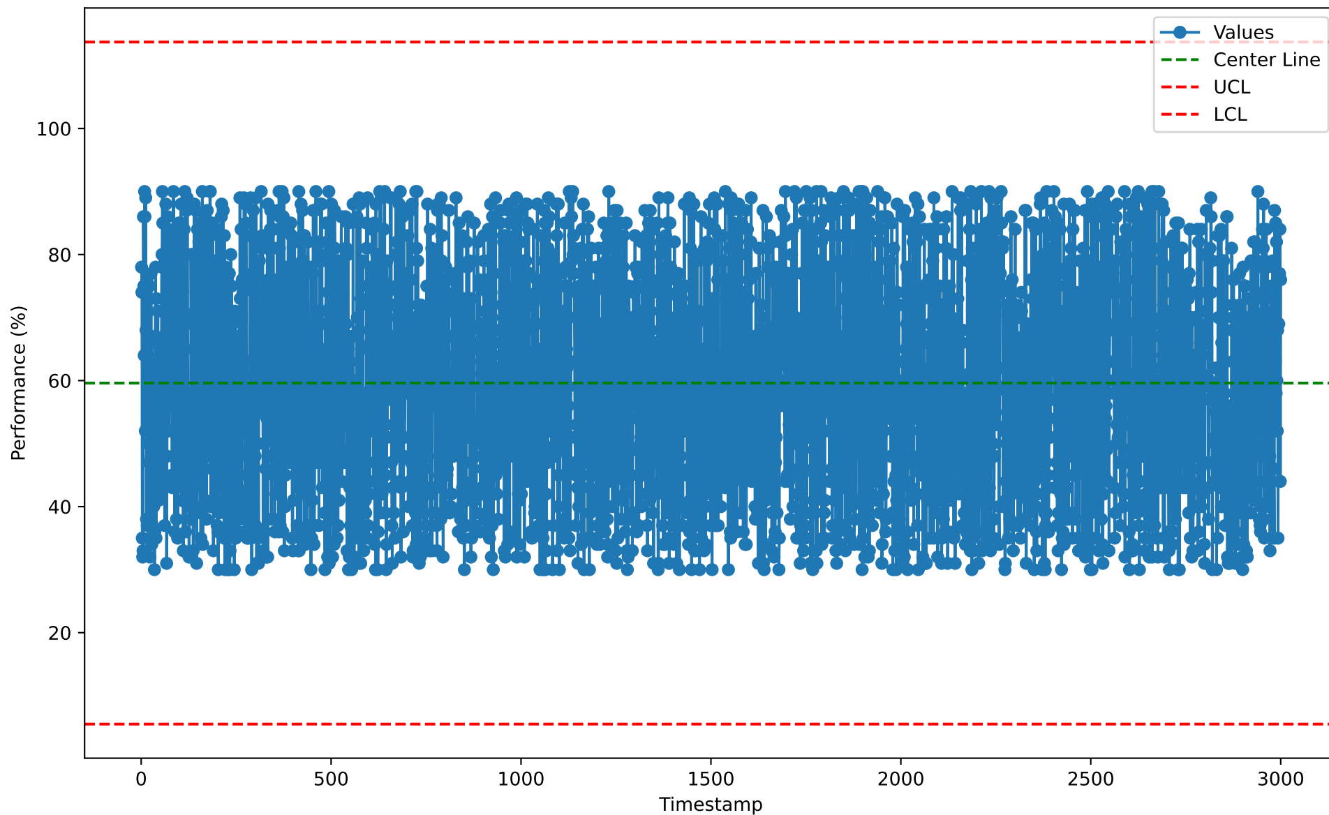
Individuals Chart for RSL10112 (2026-01-07)
