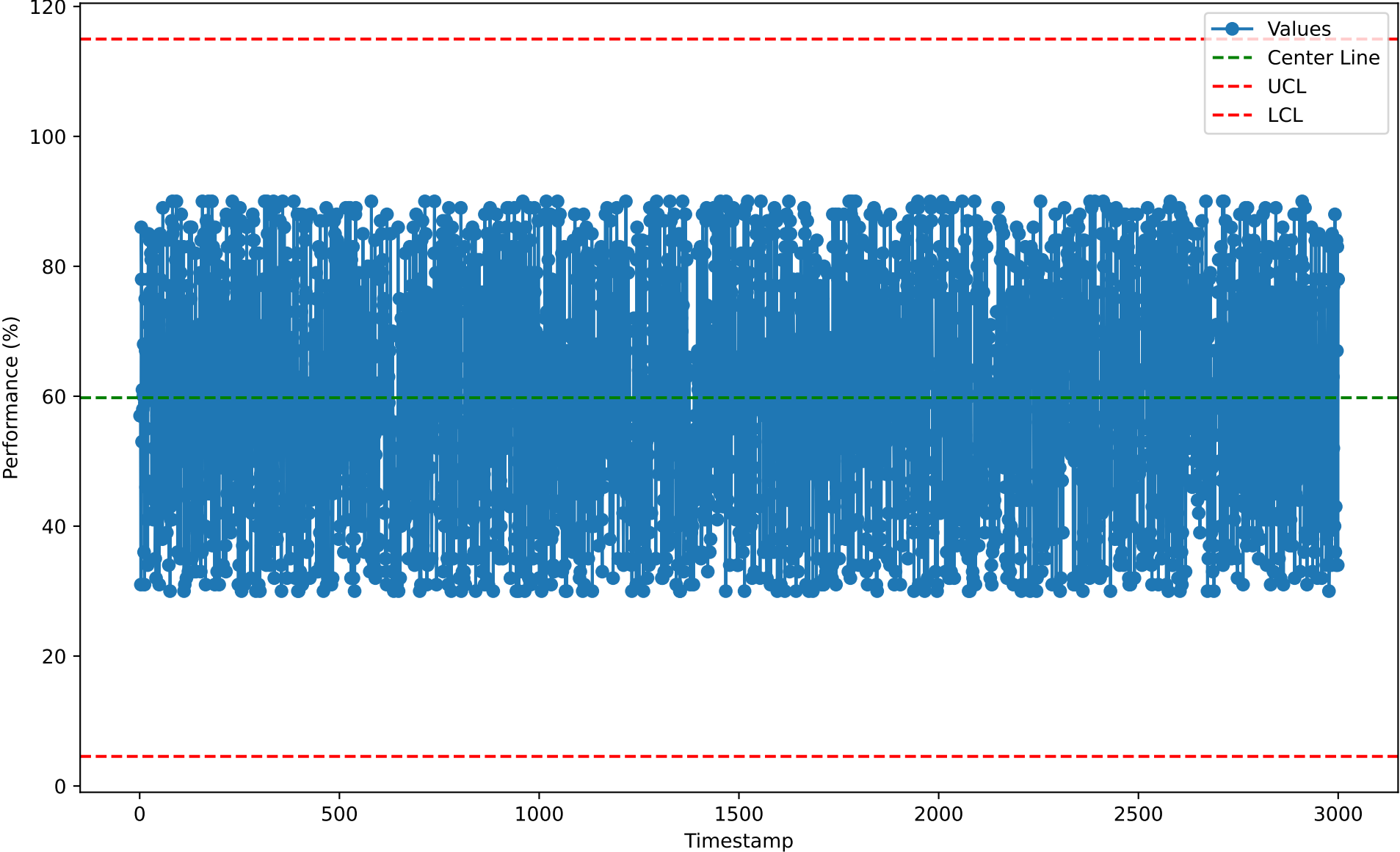
Individuals Chart for RPR10104 (2026-01-07)
