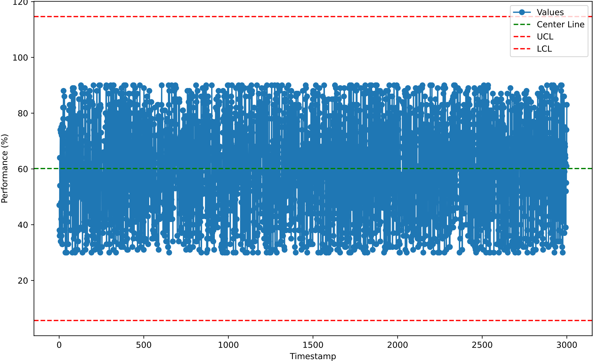
Individuals Chart for RCM10116 (2026-01-07)
