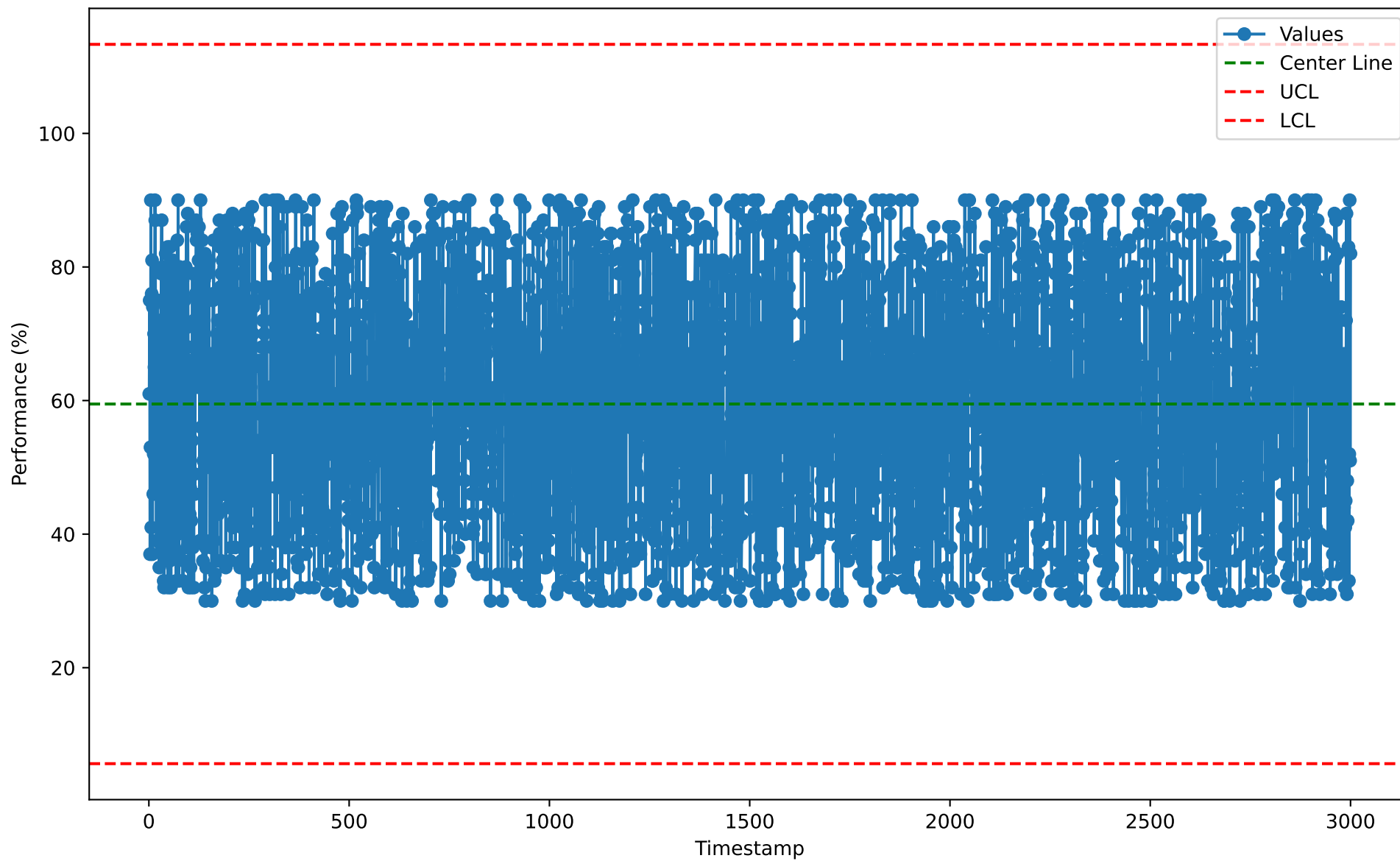
Individuals Chart for RCM10114 (2026-01-07)
