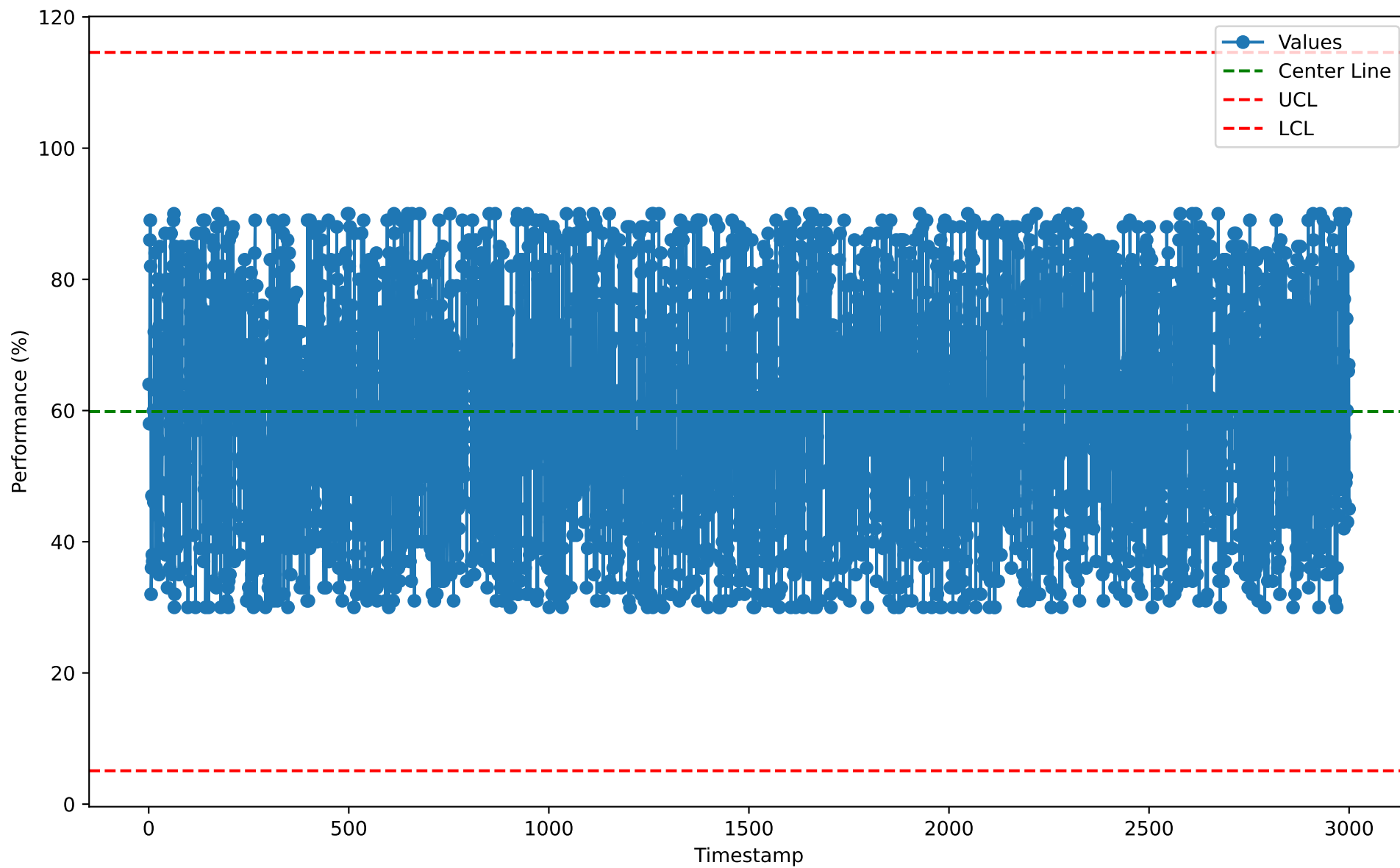
Individuals Chart for RSL10110 (2026-01-07)
