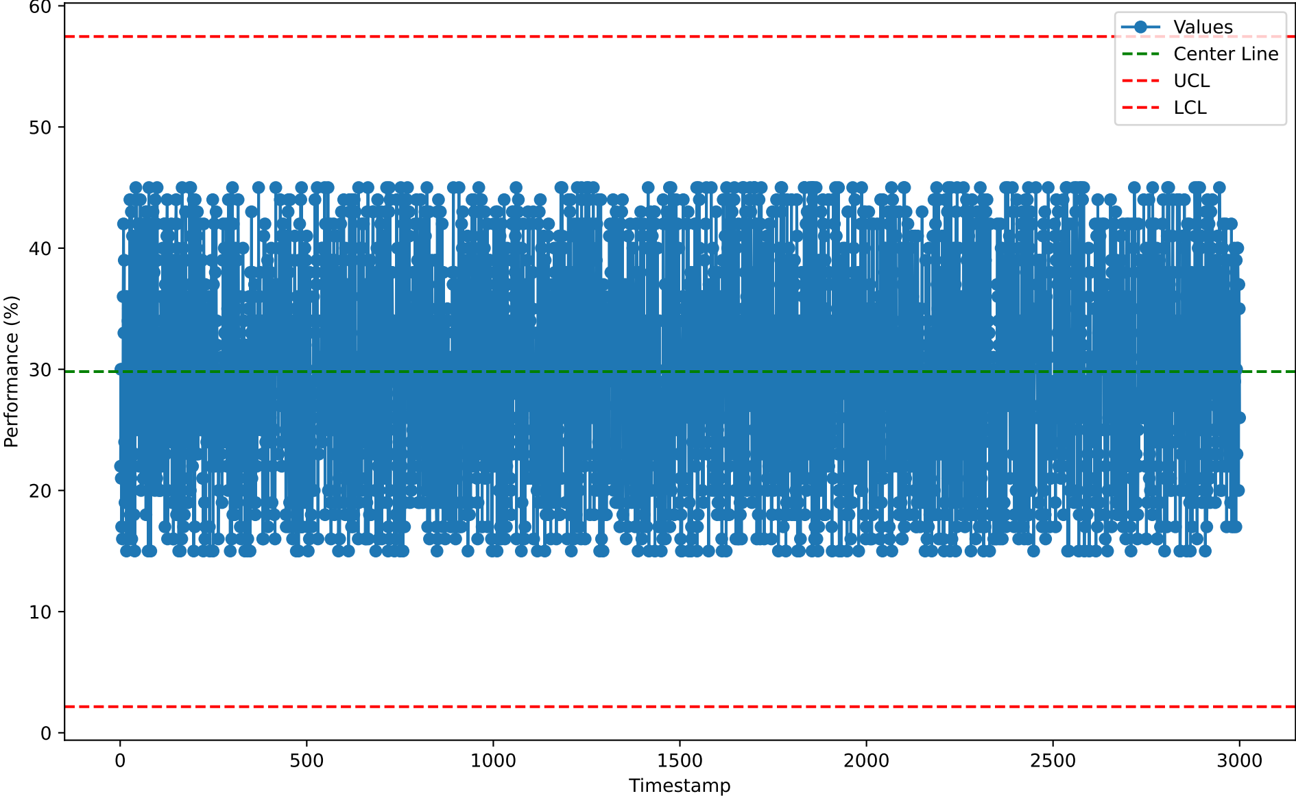
Individuals Chart for SCP10118 (2026-01-07)
