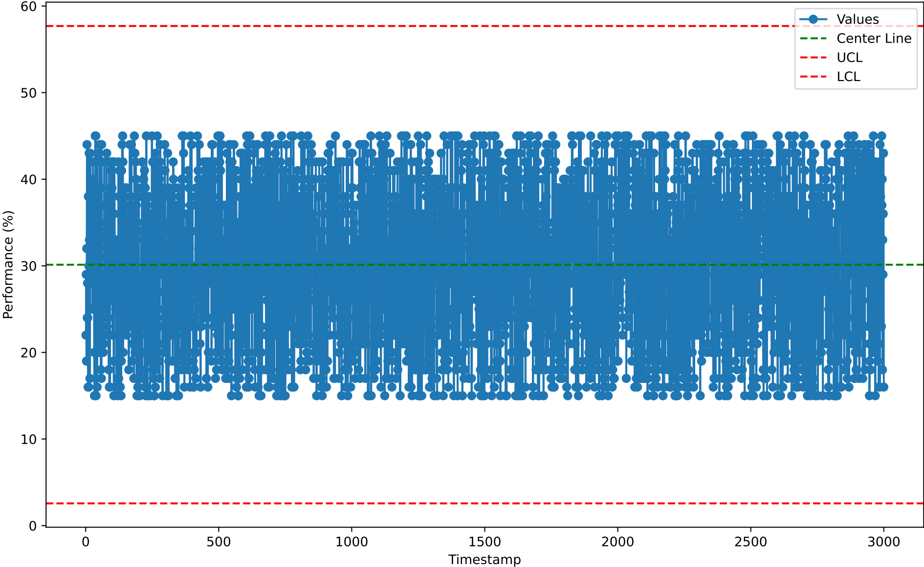
Individuals Chart for ACT10114 (2026-01-07)
