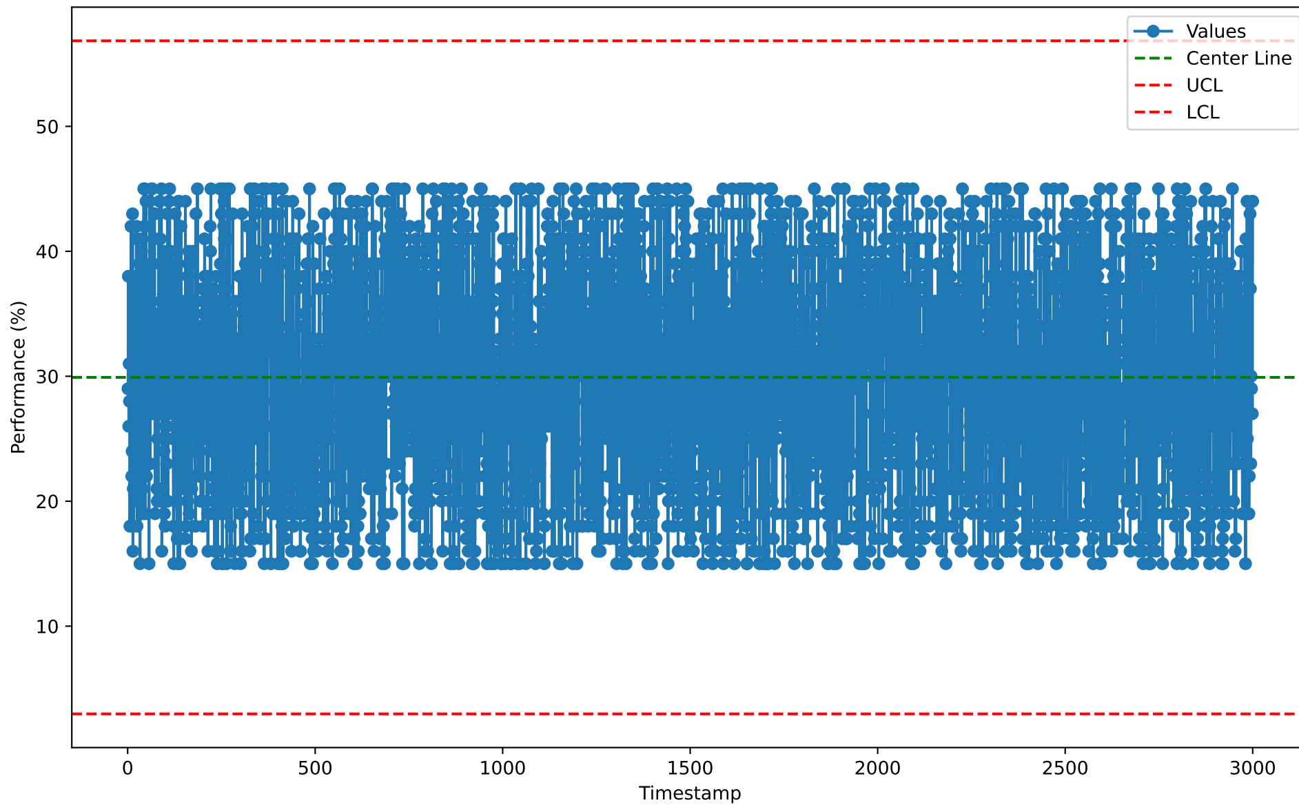
Individuals Chart for SST10117 (2026-01-07)
