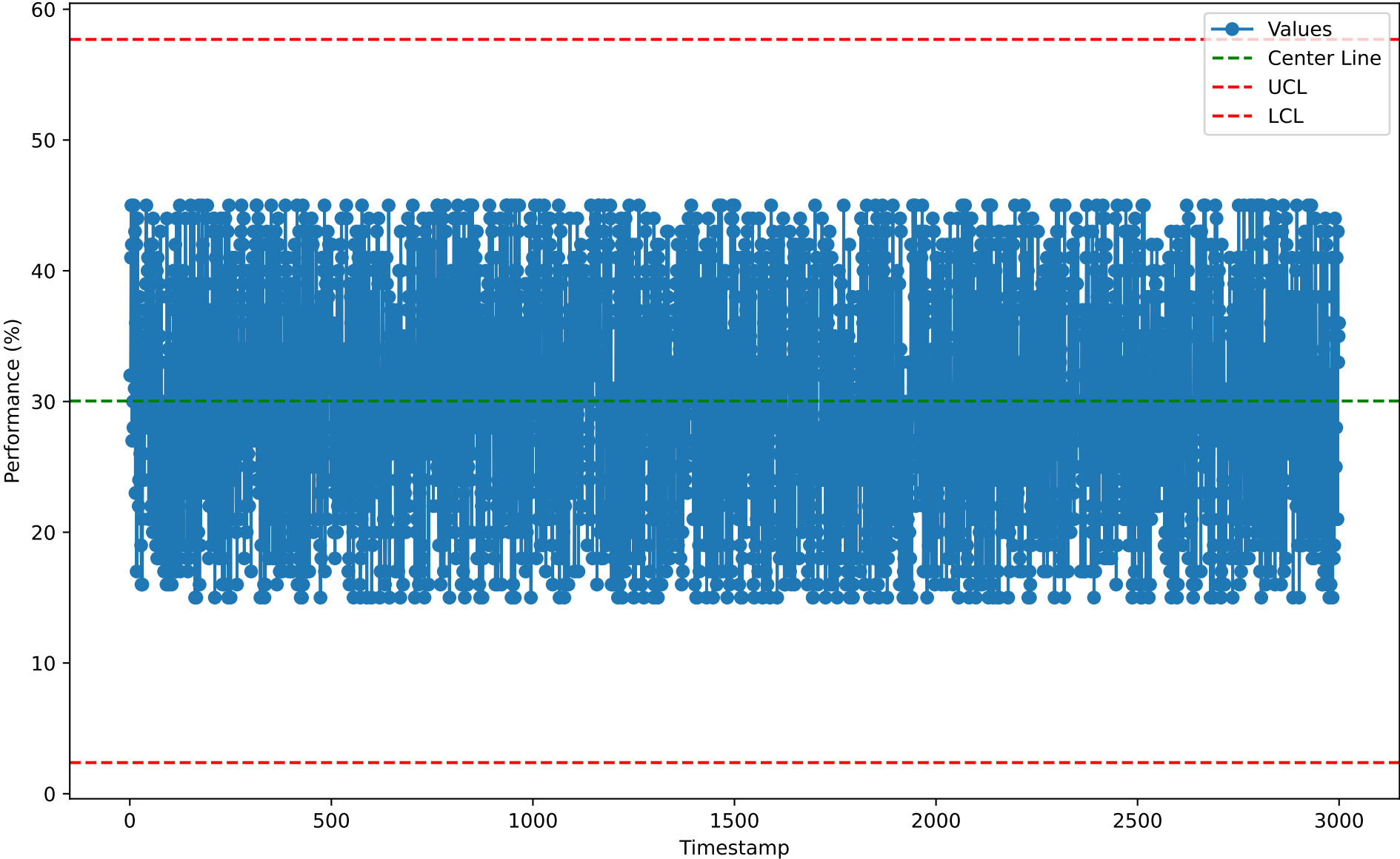
Individuals Chart for ORC10102 (2026-01-07)
