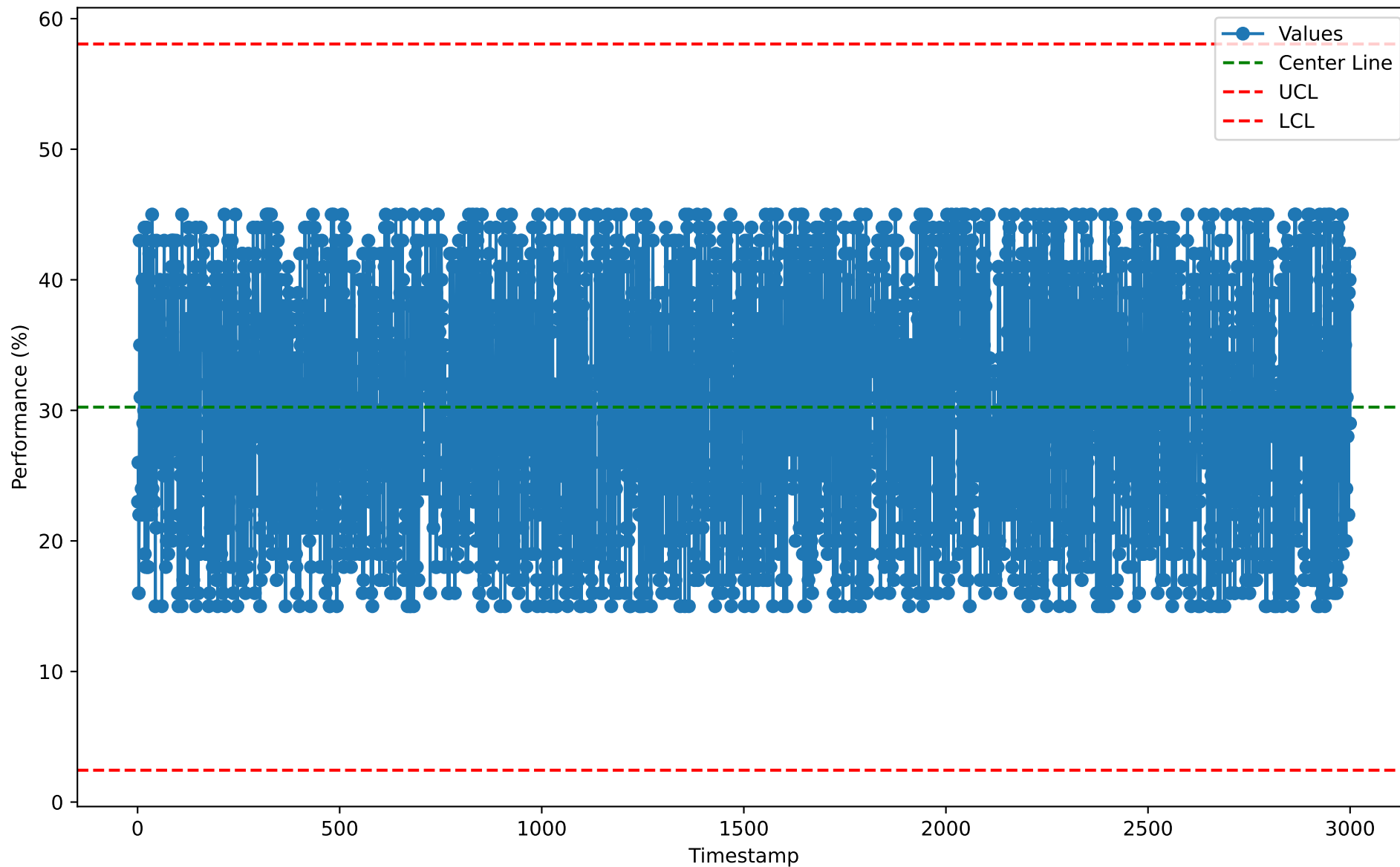
Individuals Chart for SST10110 (2026-01-07)
