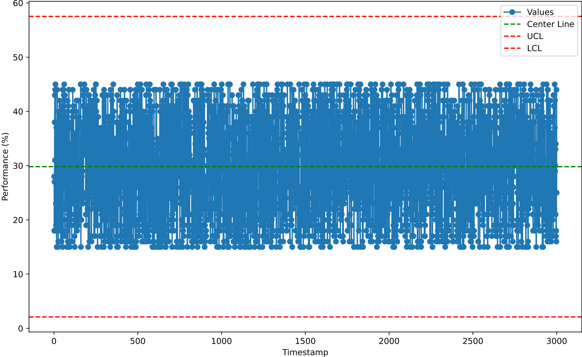
Individuals Chart for CPD10112 (2026-01-07)
