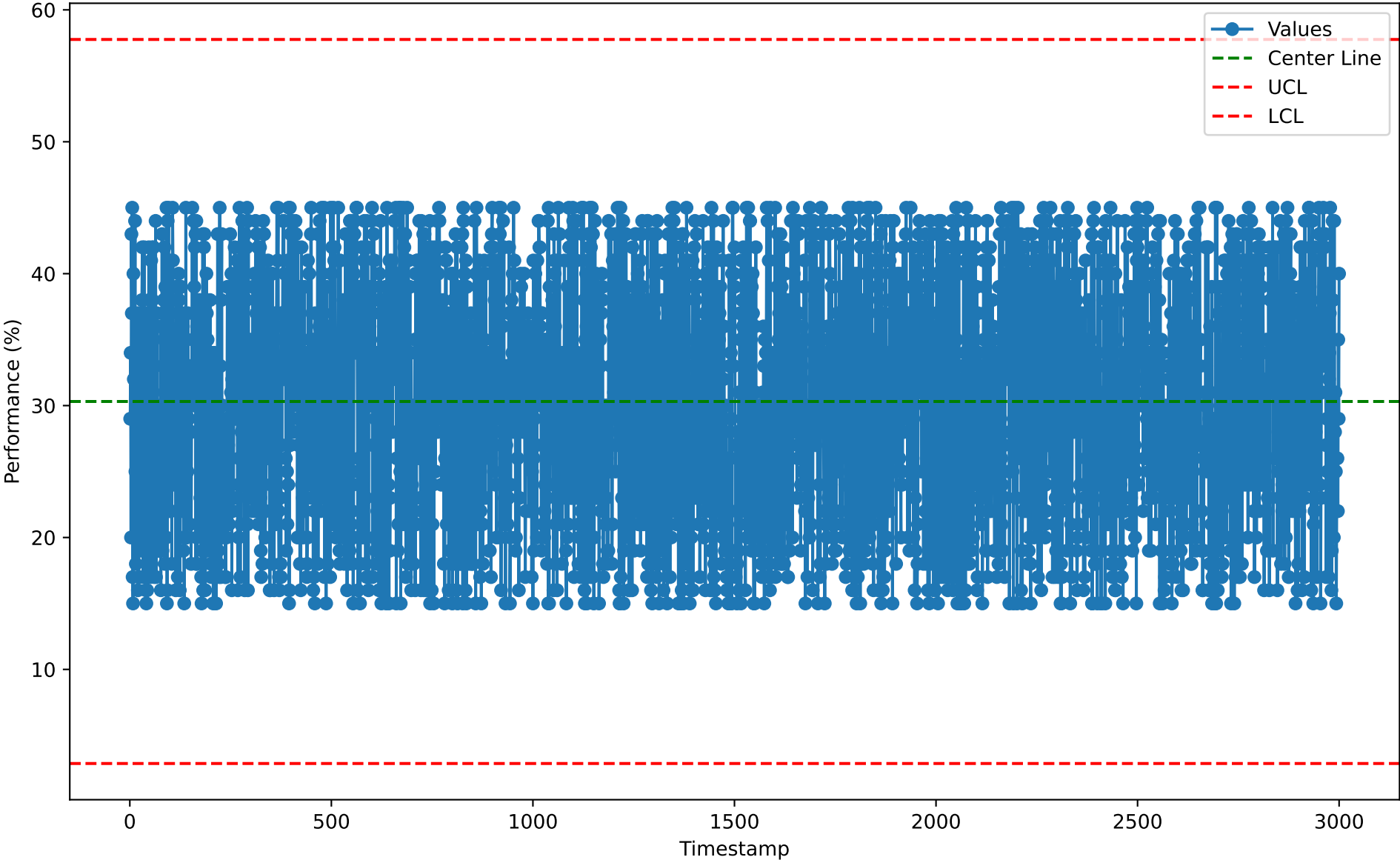
Individuals Chart for CLC10123 (2026-01-07)
