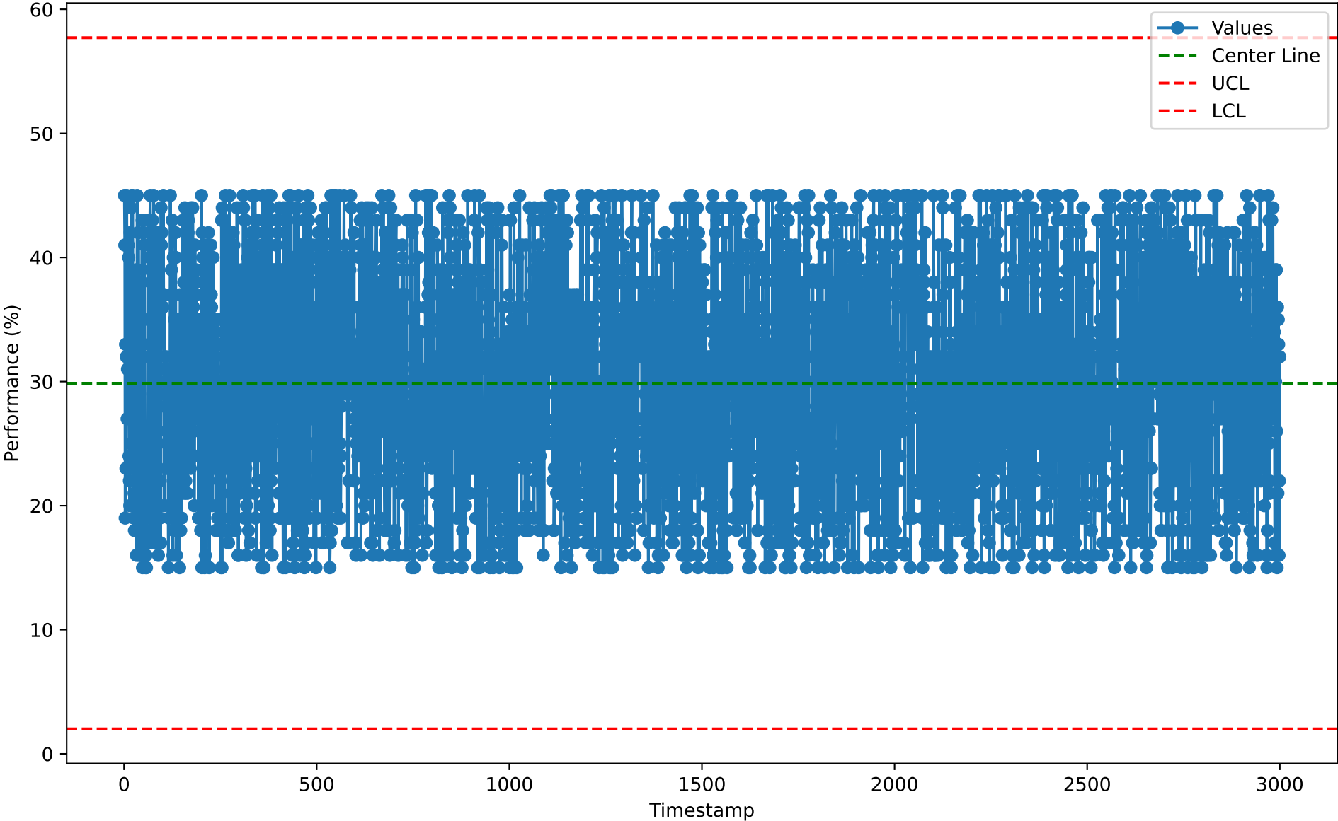
Individuals Chart for ALM10120 (2026-01-07)
