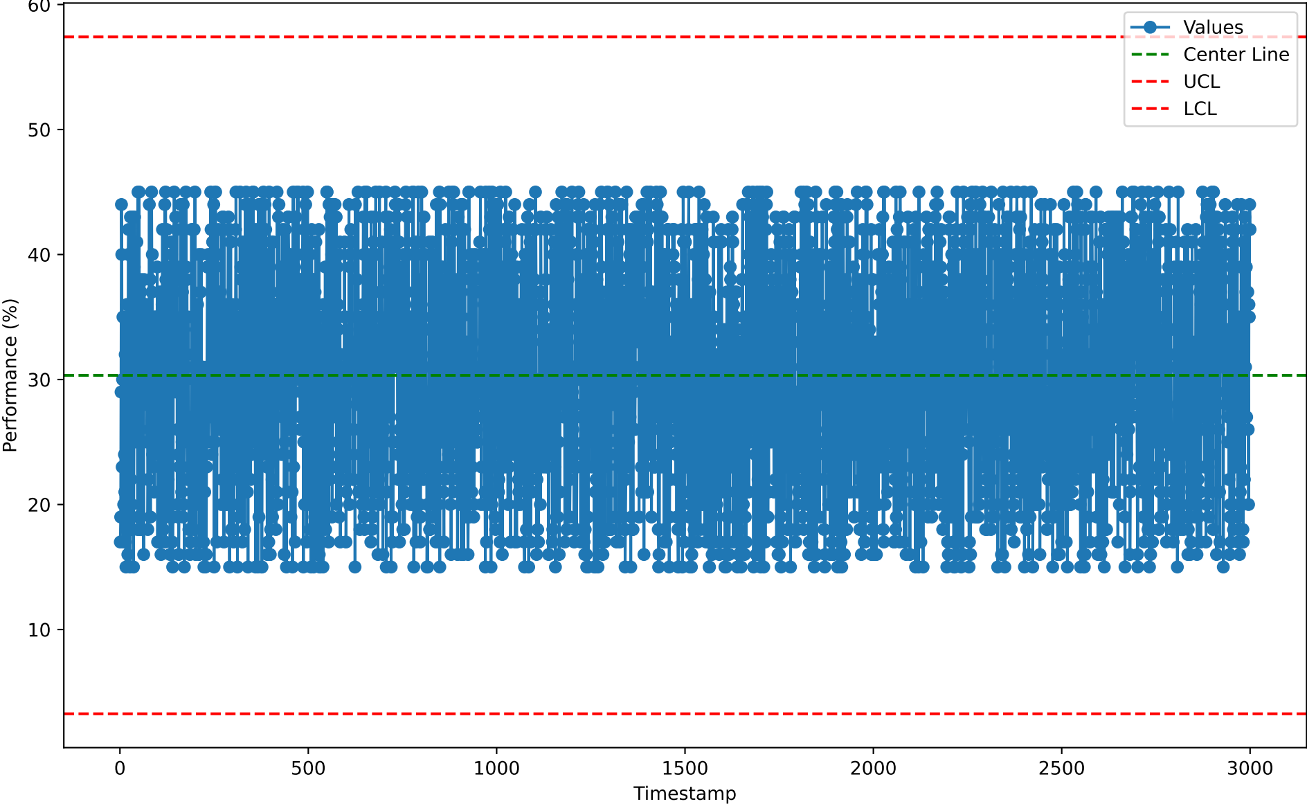
Individuals Chart for CPD10123 (2026-01-07)
