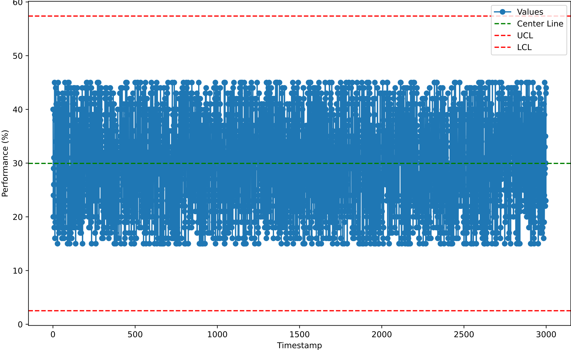
Individuals Chart for SCC10111 (2026-01-07)
