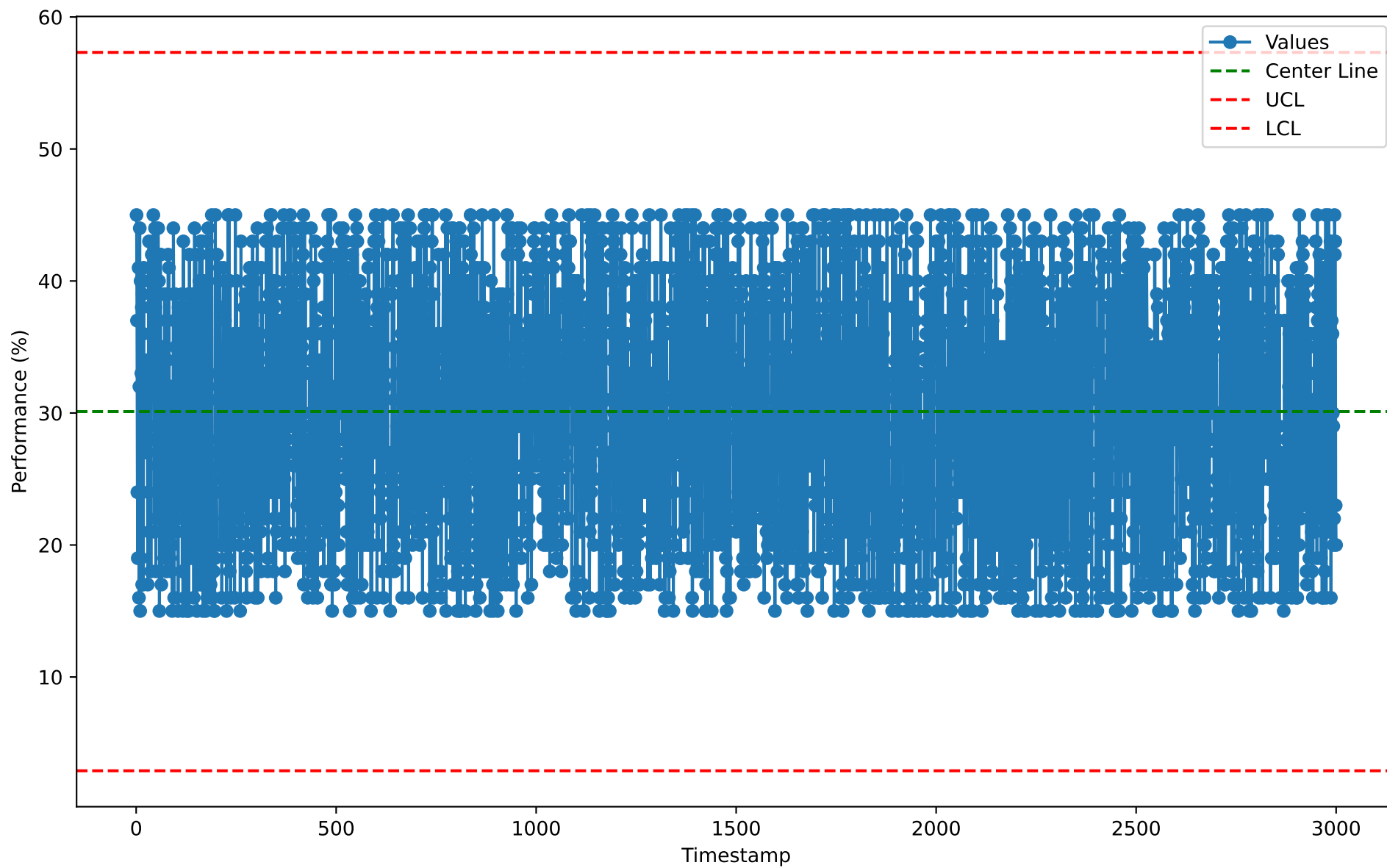
Individuals Chart for PFR10105 (2026-01-07)
