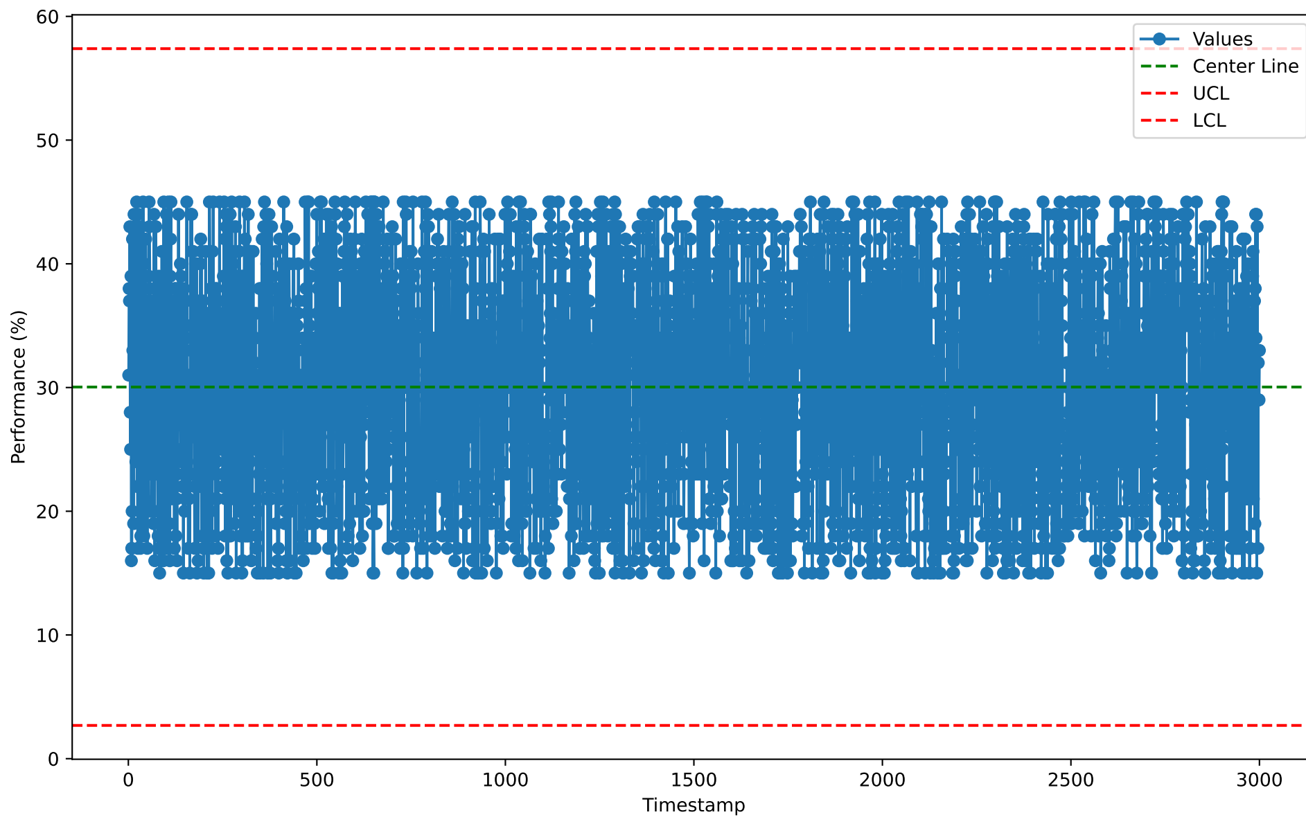
Individuals Chart for SST10111 (2026-01-07)
