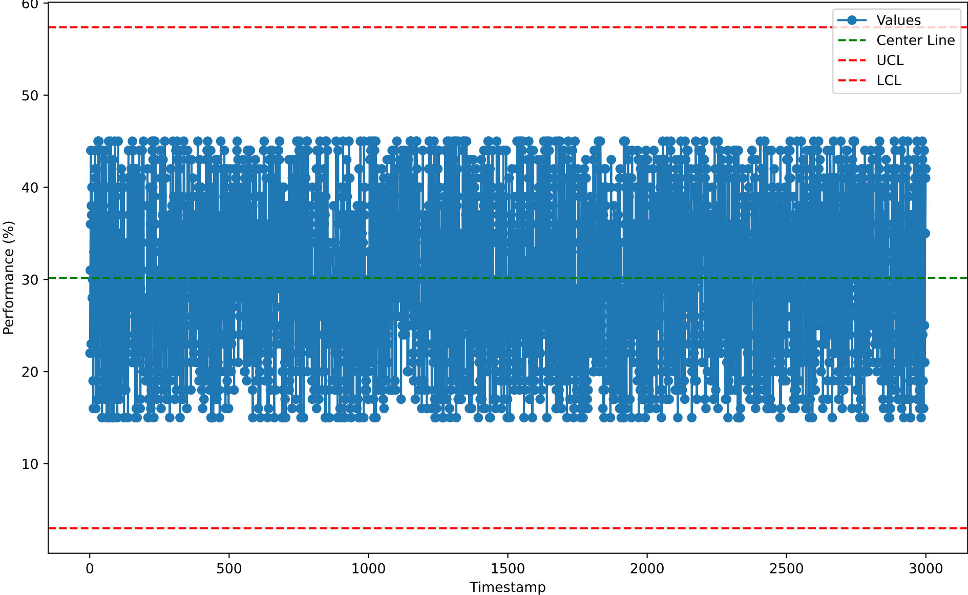
Individuals Chart for CPD10106 (2026-01-07)
