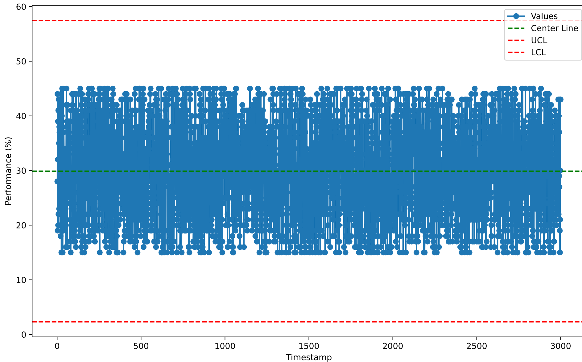
Individuals Chart for SST10102 (2026-01-07)
