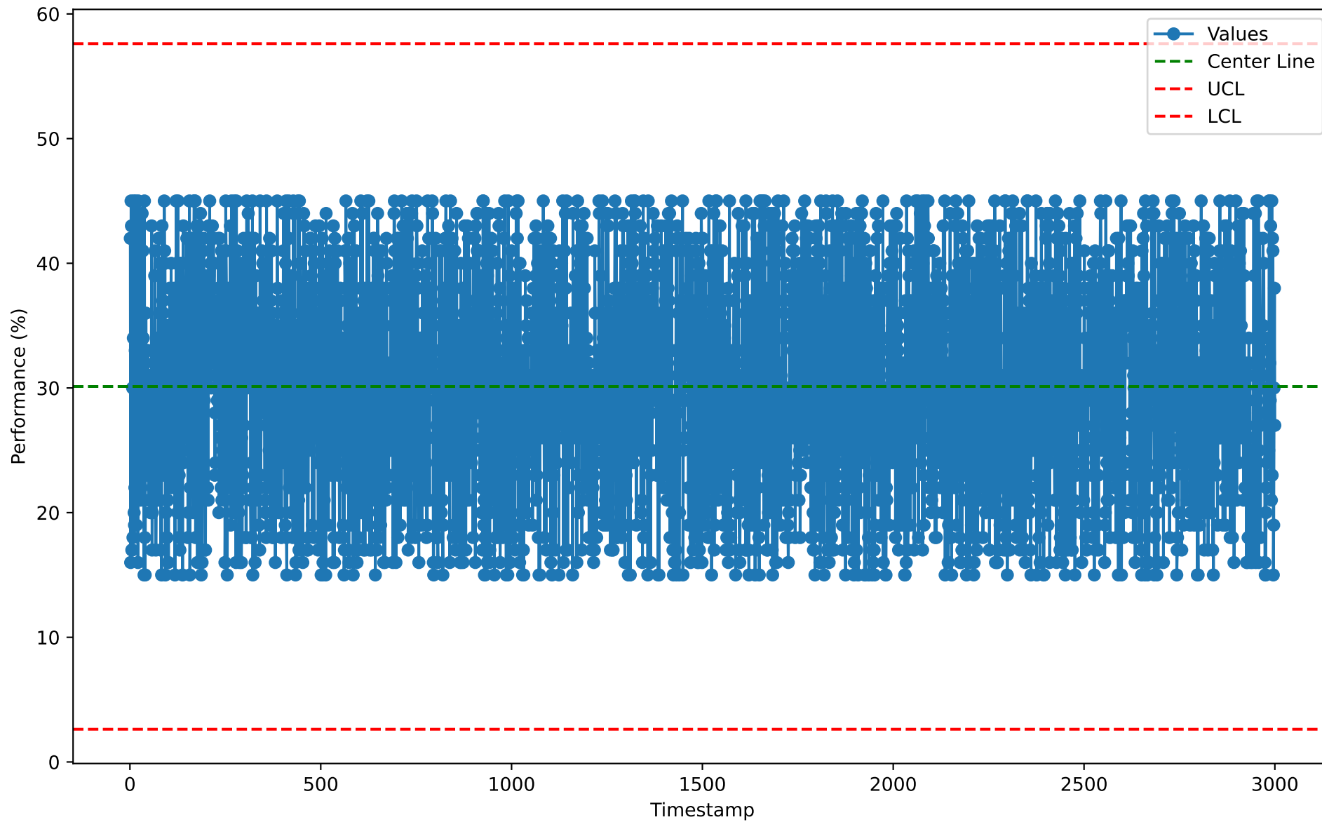
Individuals Chart for PFR10121 (2026-01-07)
