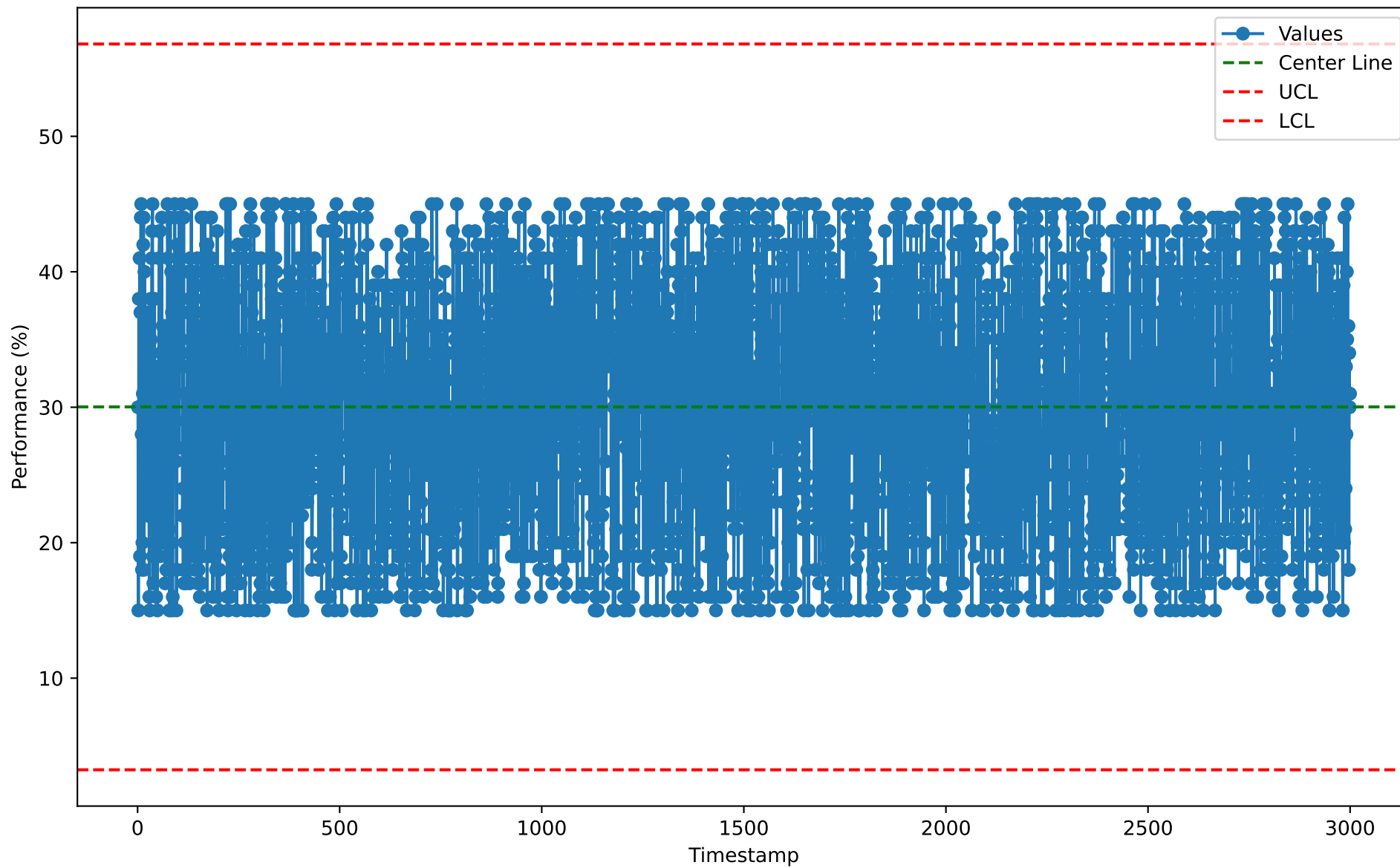
Individuals Chart for SPL10124 (2026-01-07)
