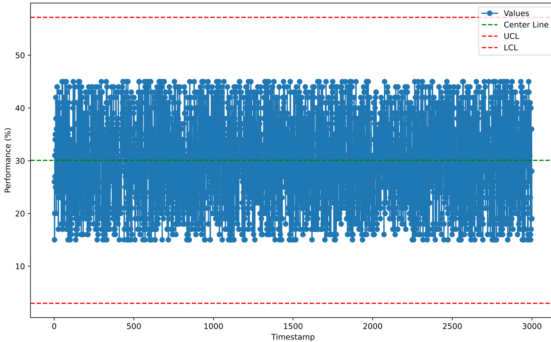
Individuals Chart for SST10104 (2026-01-07)
