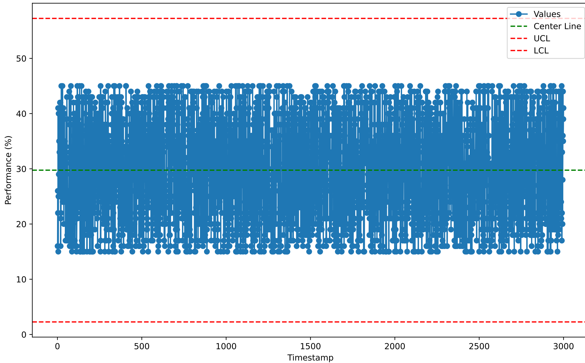
Individuals Chart for SPL10108 (2026-01-07)
