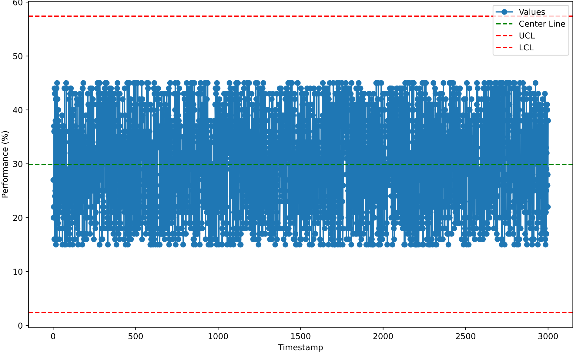
Individuals Chart for PRB10122 (2026-01-07)
