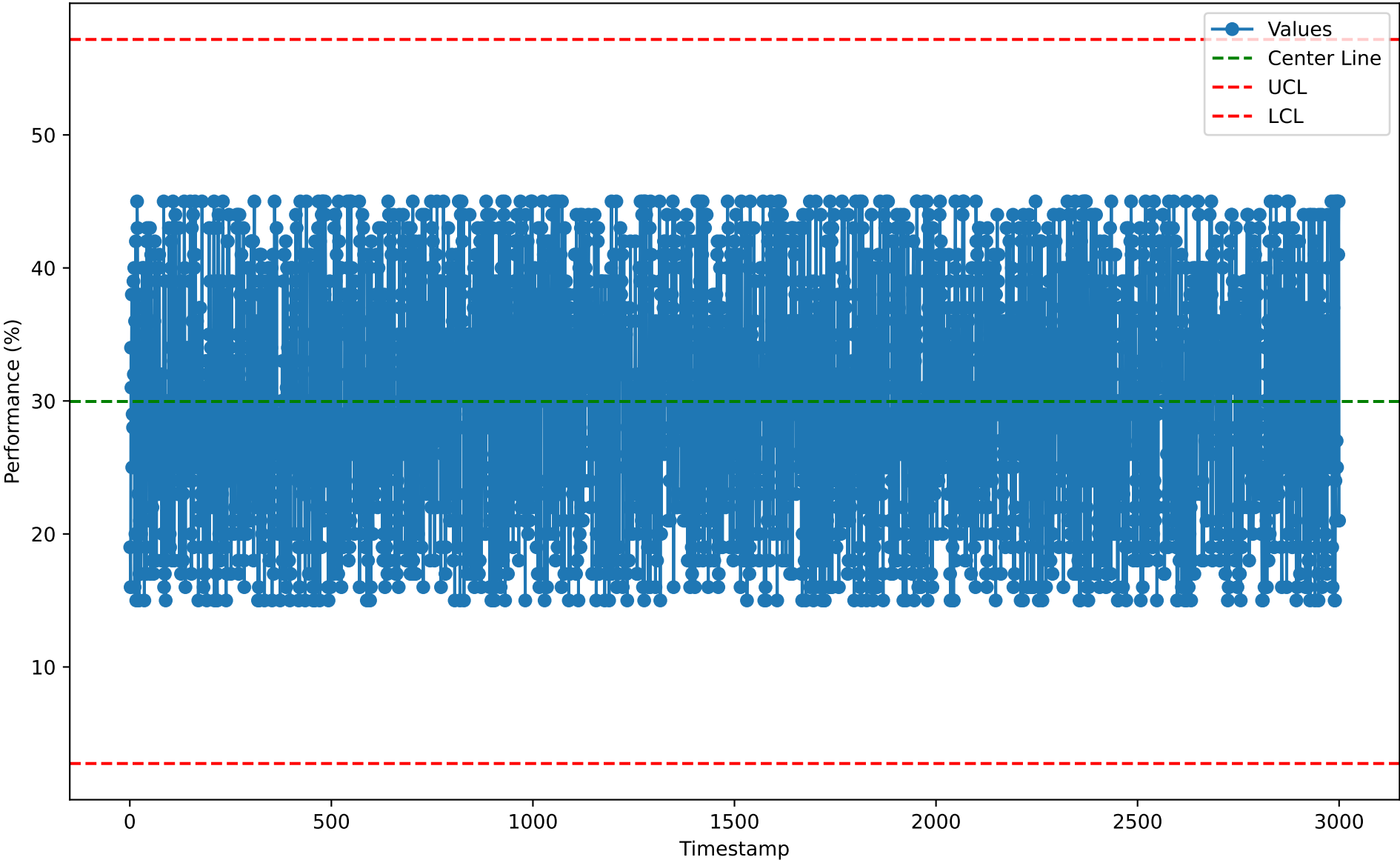
Individuals Chart for SSM10120 (2026-01-07)
