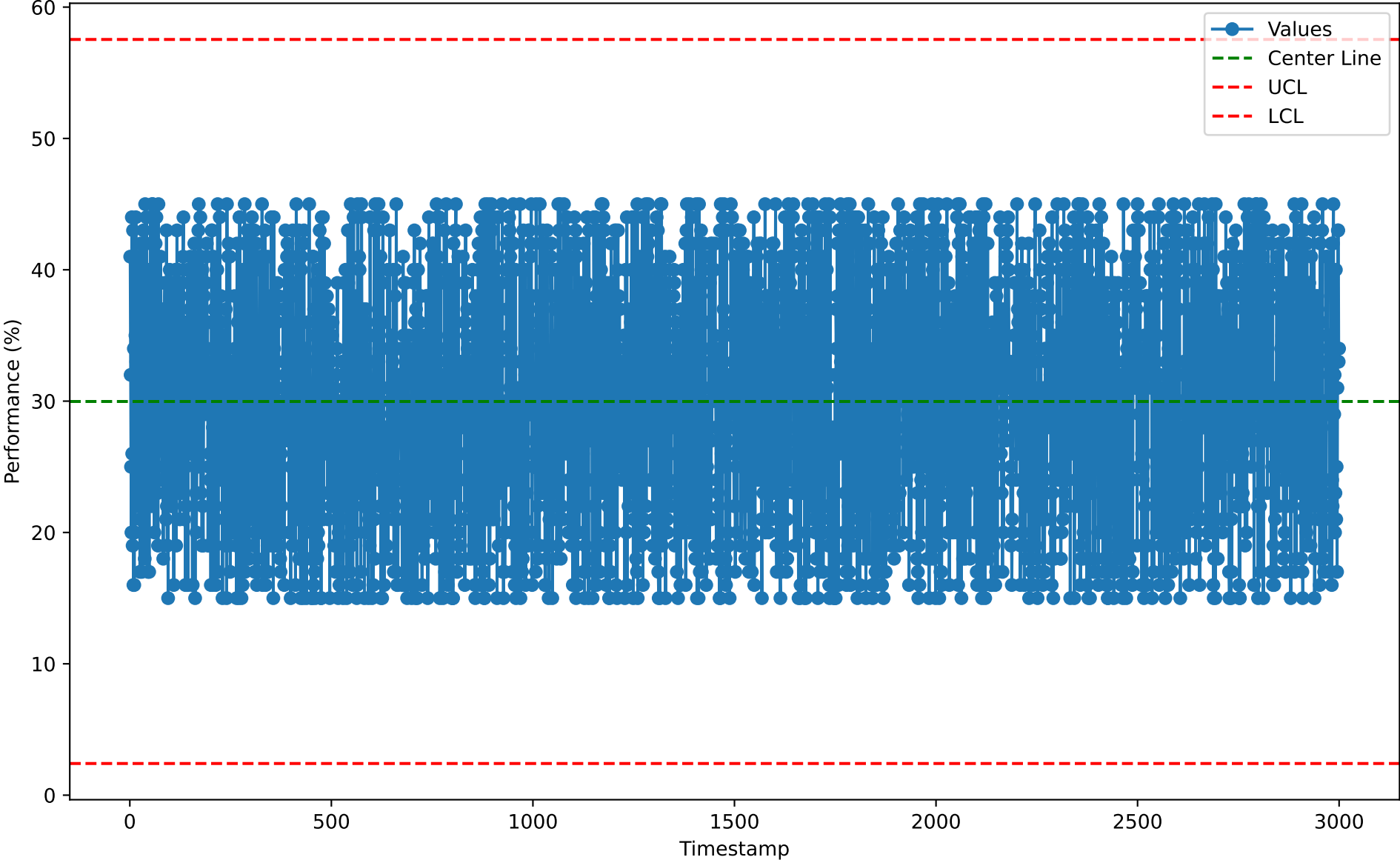
Individuals Chart for SUP10113 (2026-01-07)
