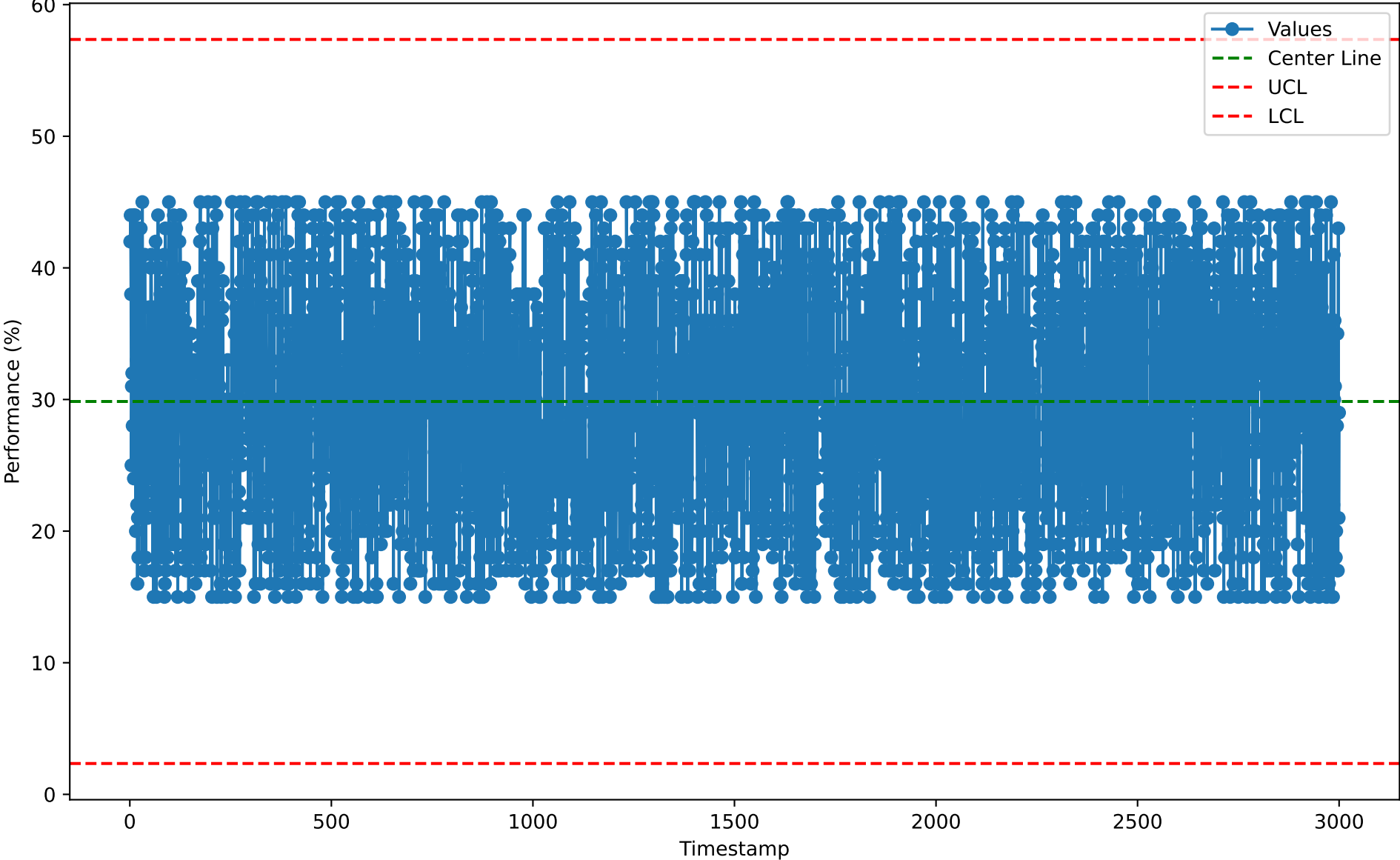
Individuals Chart for CPD10103 (2026-01-07)
