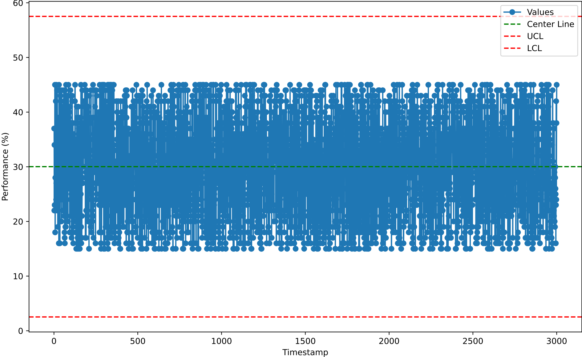
Individuals Chart for SCP10127 (2026-01-07)
