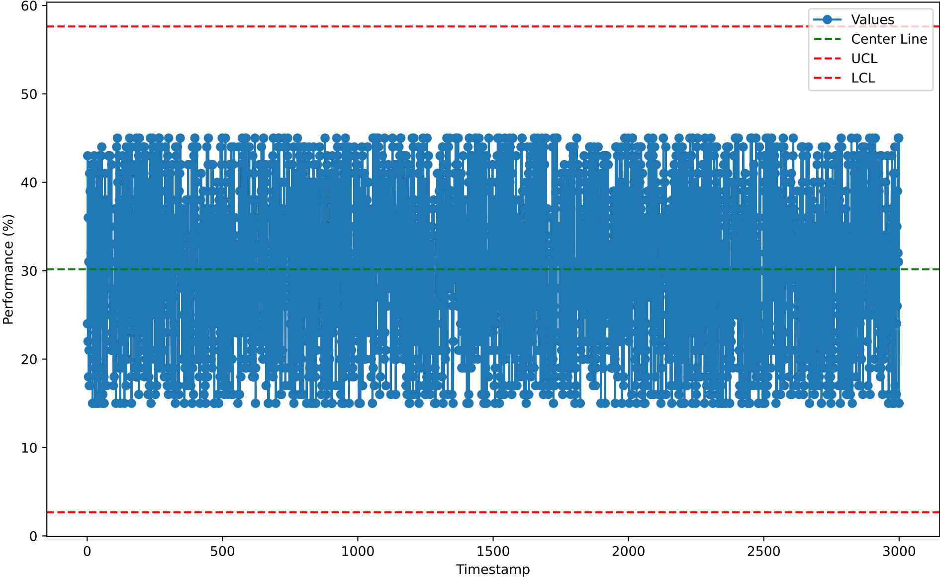
Individuals Chart for SSM10105 (2026-01-07)
