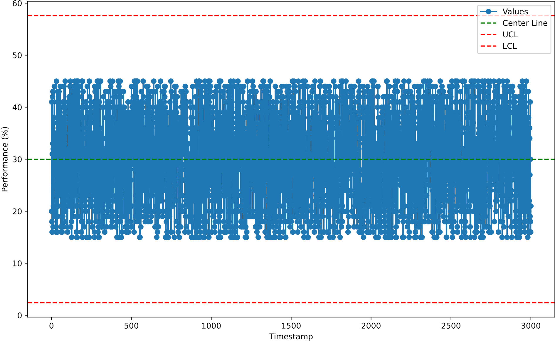
Individuals Chart for ORC10105 (2026-01-07)
