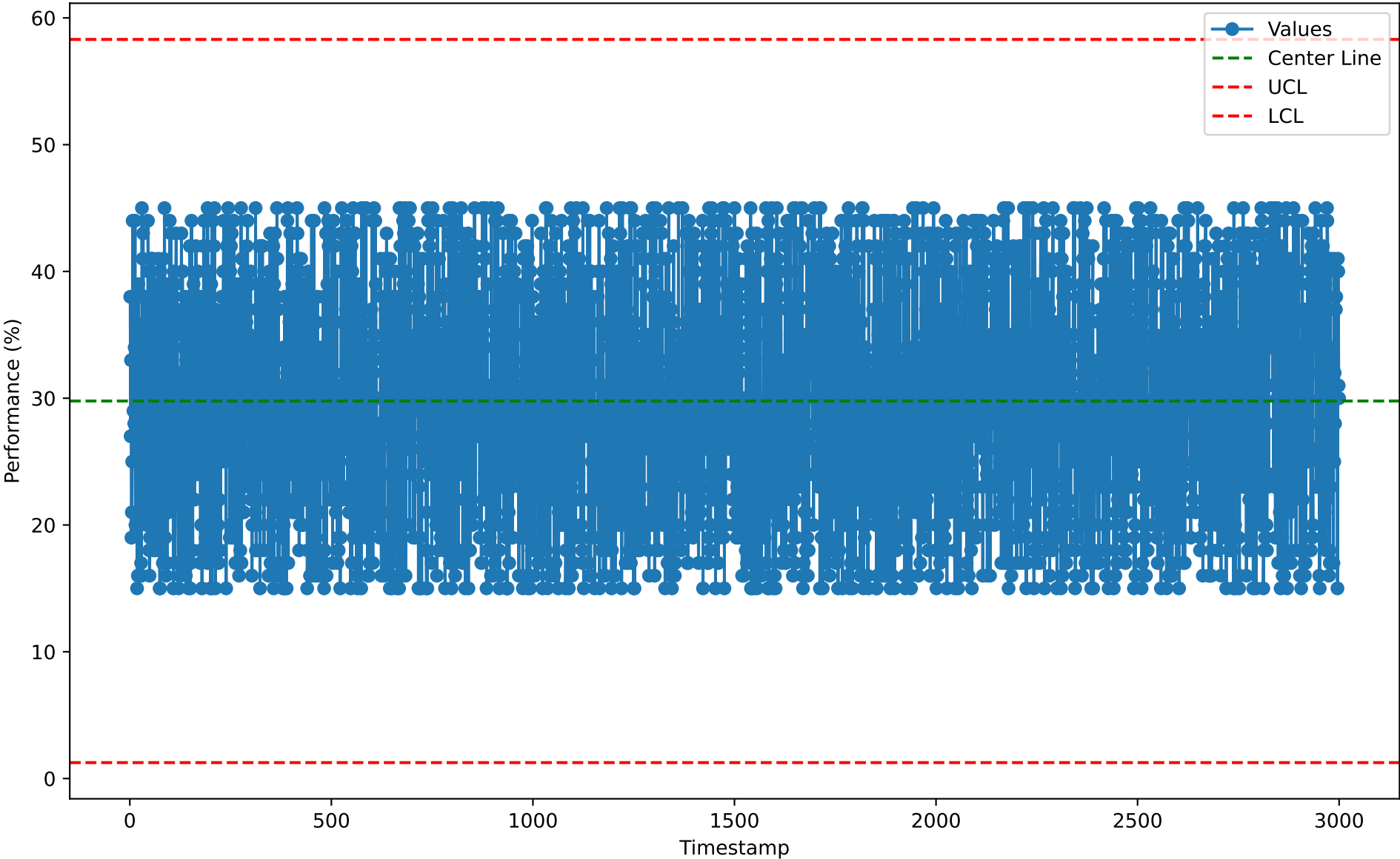
Individuals Chart for SUP10122 (2026-01-07)
