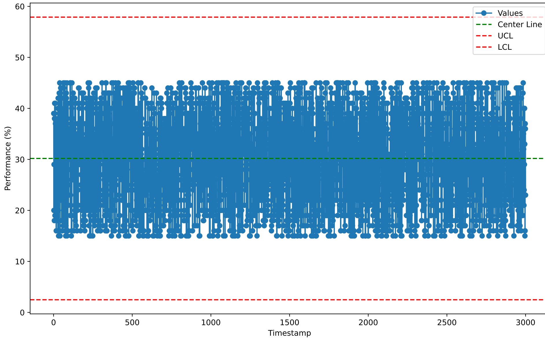
Individuals Chart for PFR10123 (2026-01-07)
