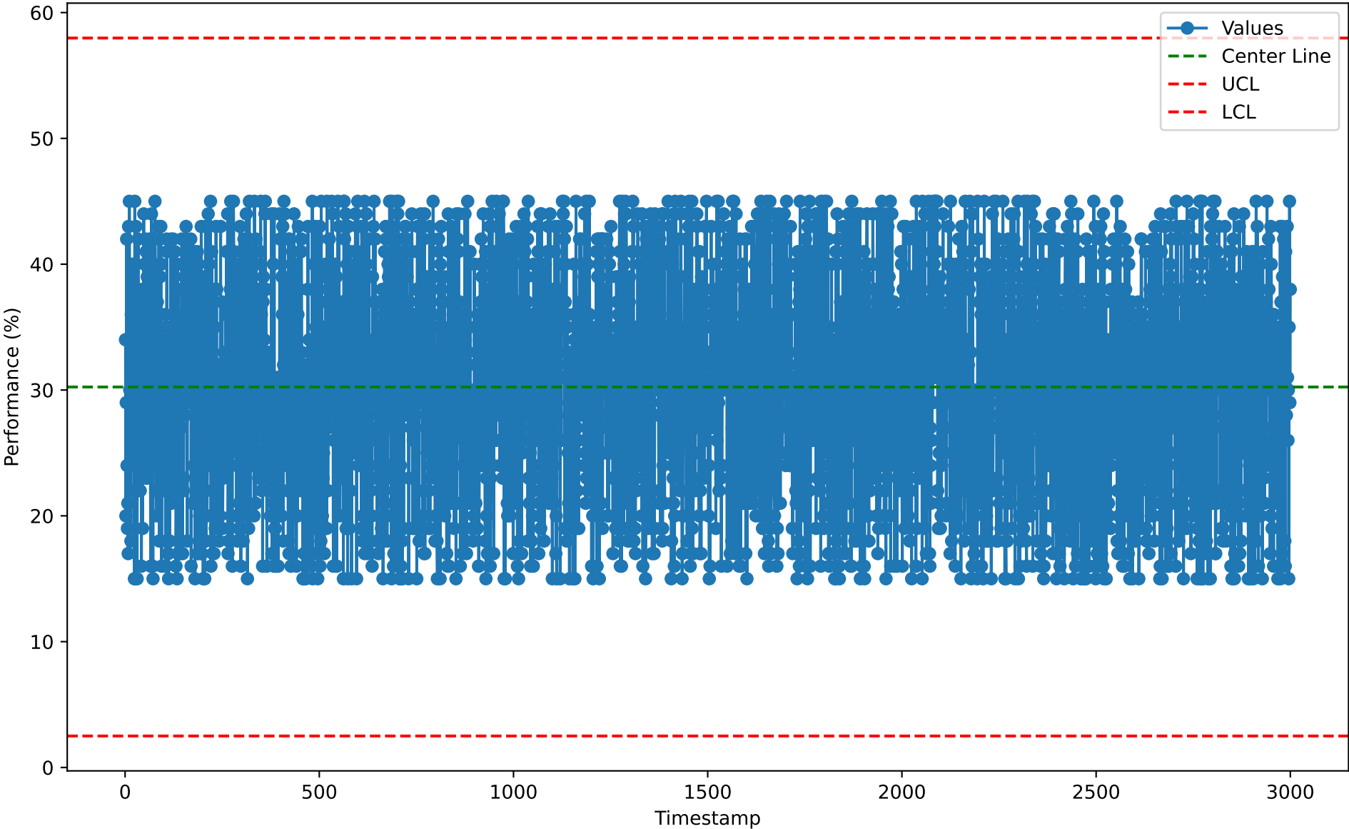
Individuals Chart for SUP10117 (2026-01-07)
