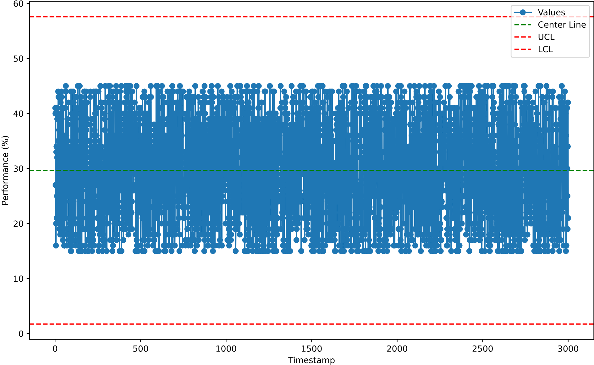
Individuals Chart for ORC10107 (2026-01-07)
