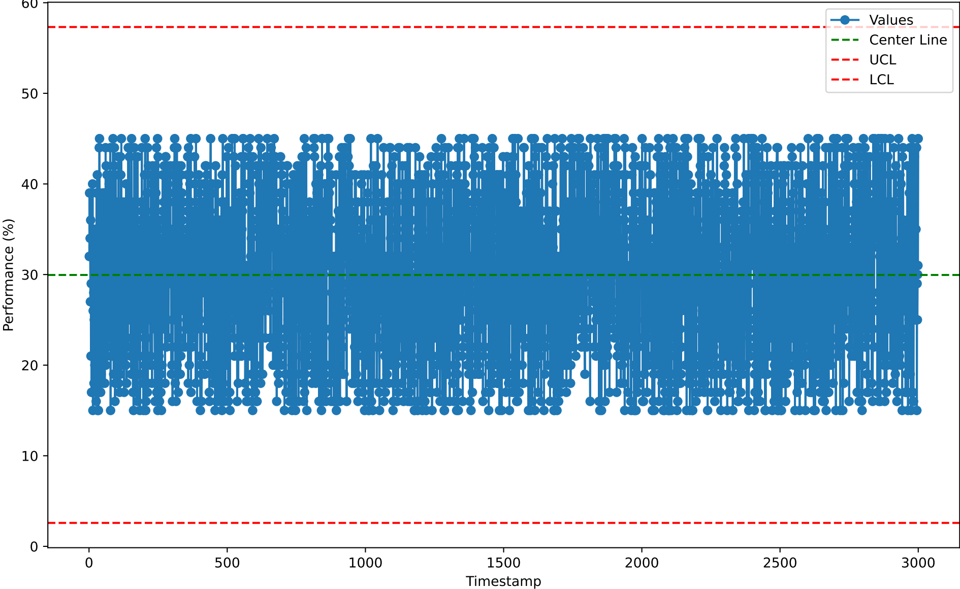
Individuals Chart for PRB10116 (2026-01-07)
