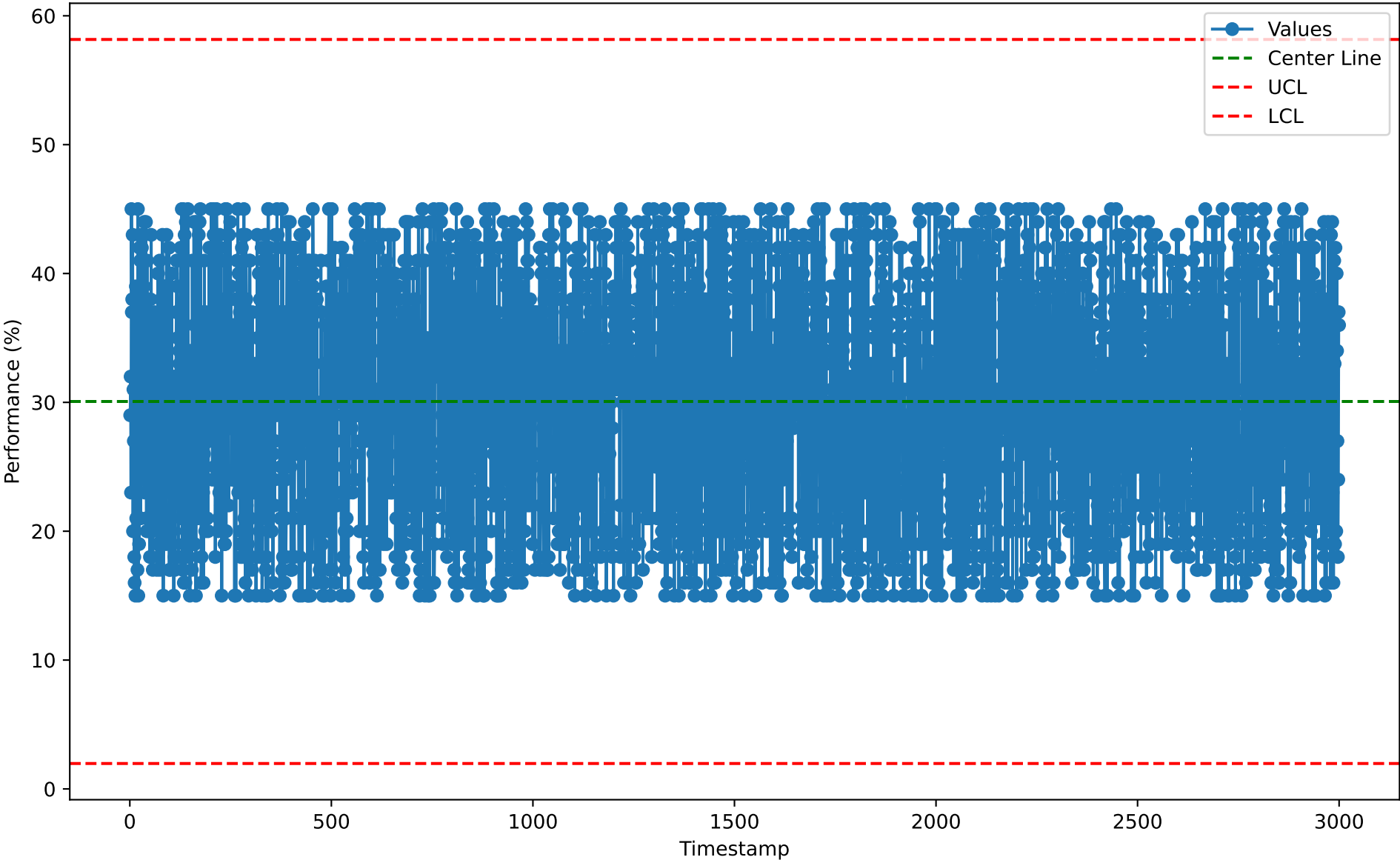
Individuals Chart for PRB10106 (2026-01-07)
