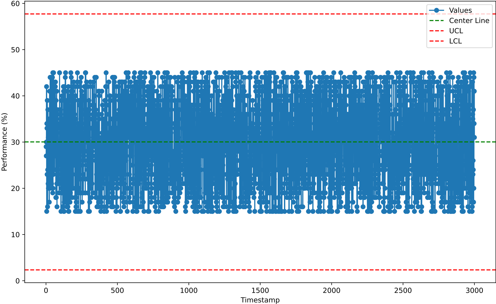
Individuals Chart for PRB10118 (2026-01-07)
