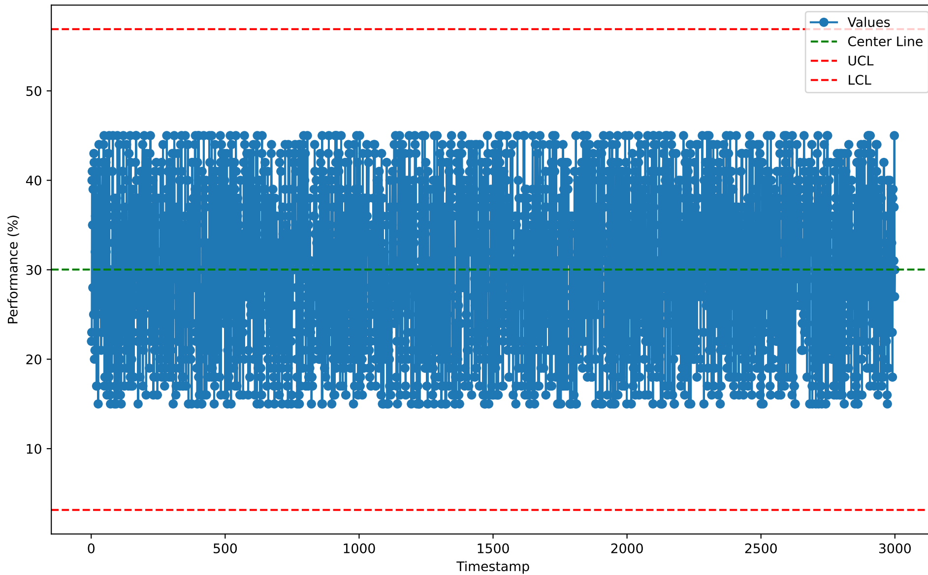
Individuals Chart for PFR10114 (2026-01-07)
