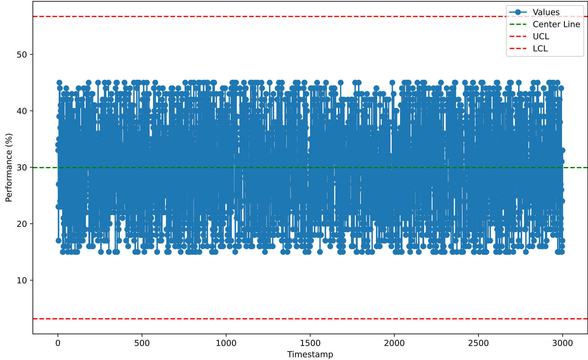
Individuals Chart for ALM10105 (2026-01-07)
