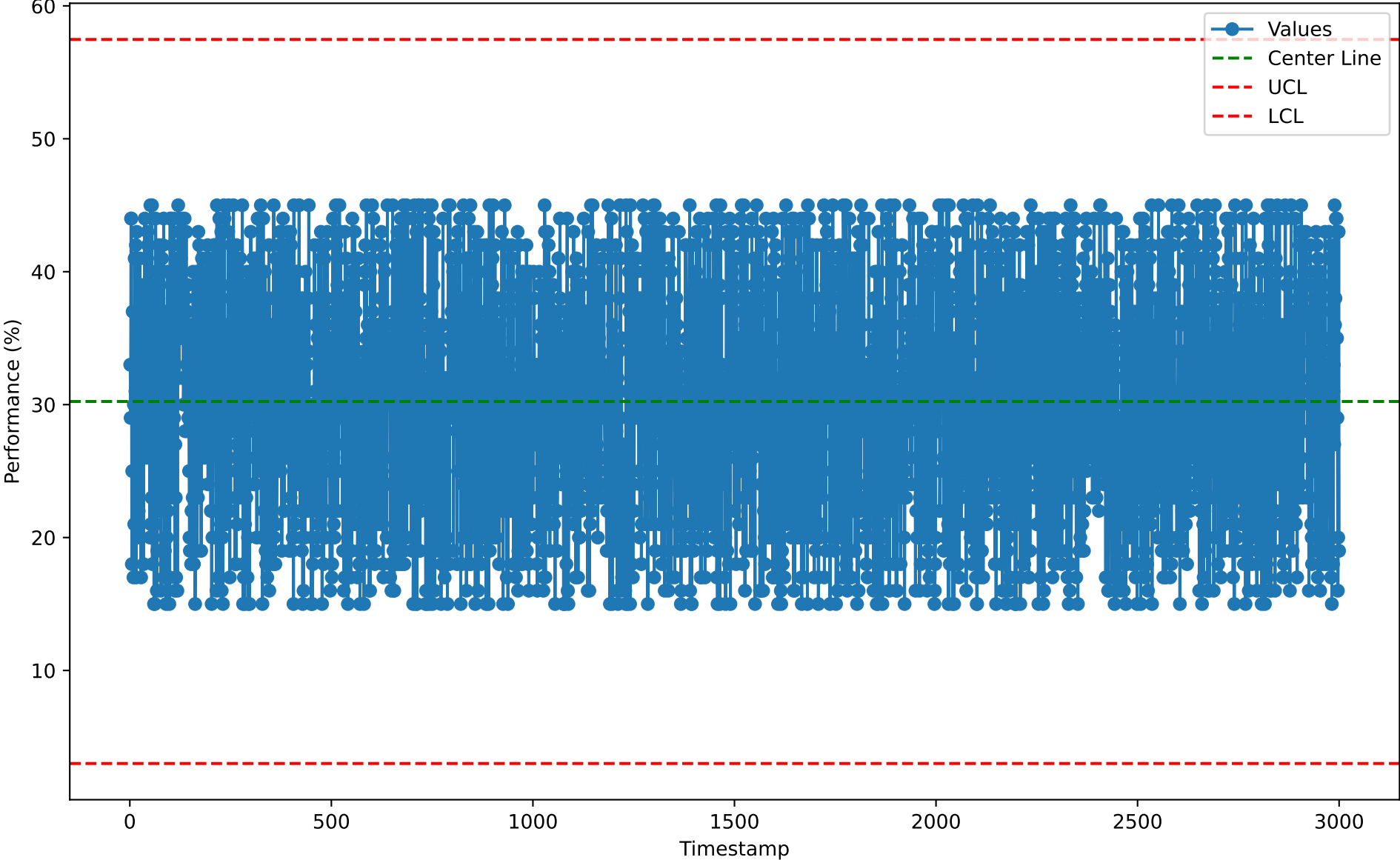
Individuals Chart for SCC10125 (2026-01-07)
