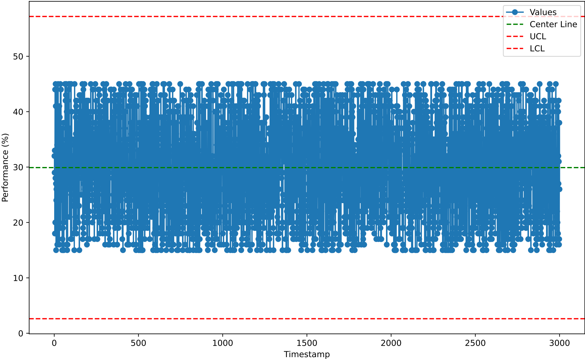
Individuals Chart for CLC10114 (2026-01-07)
