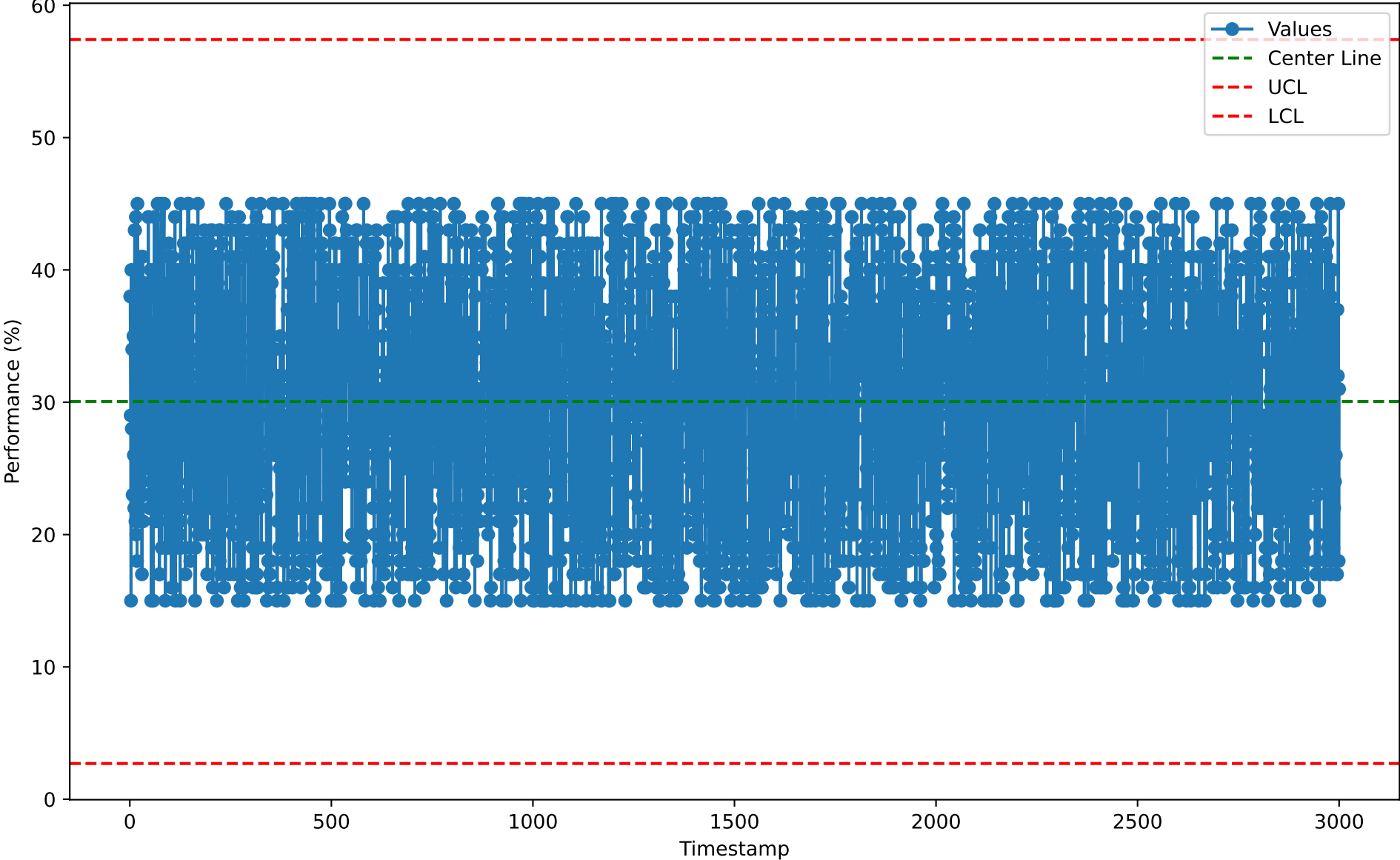
Individuals Chart for CPD10122 (2026-01-07)
