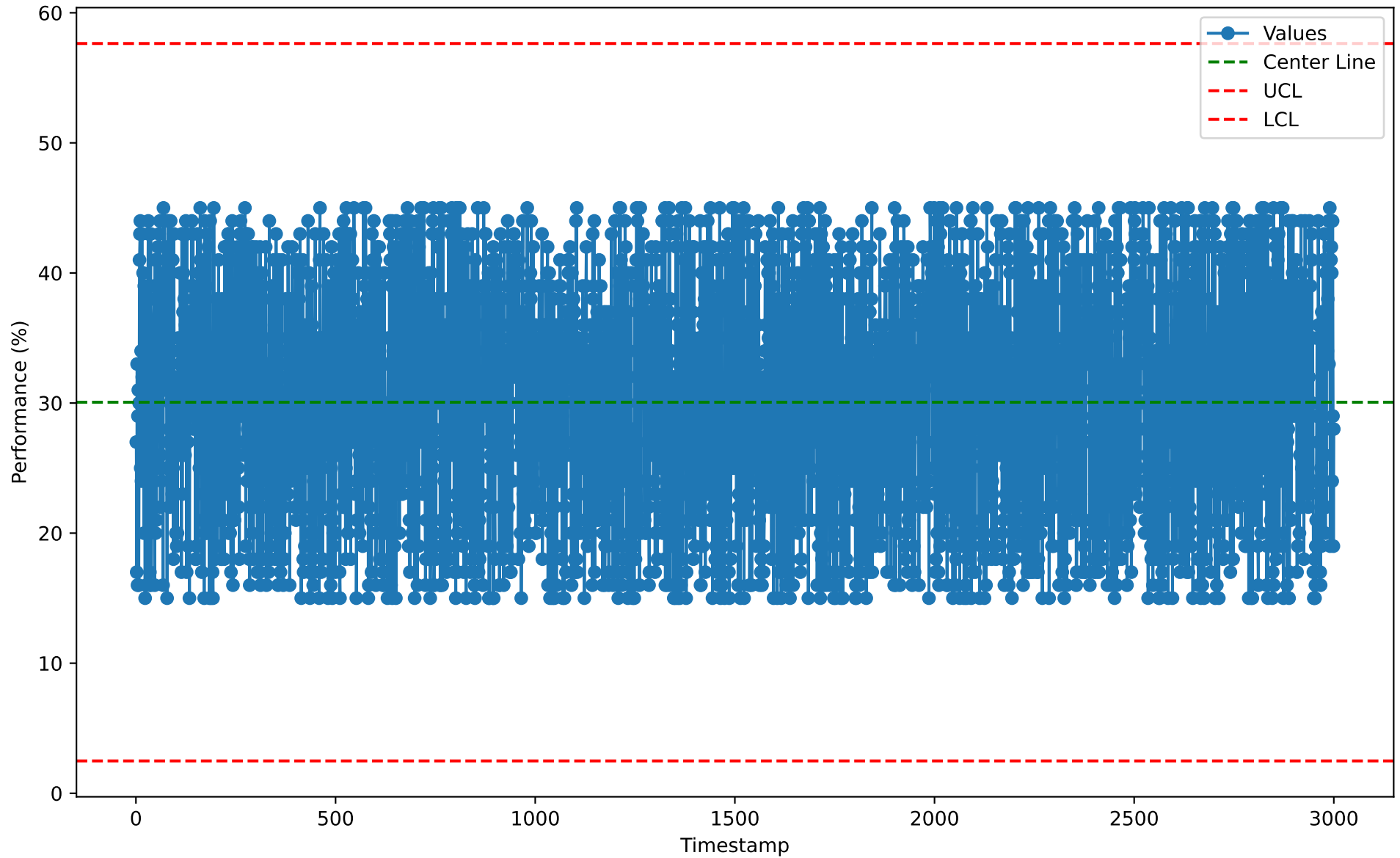
Individuals Chart for GMD10111 (2026-01-07)
