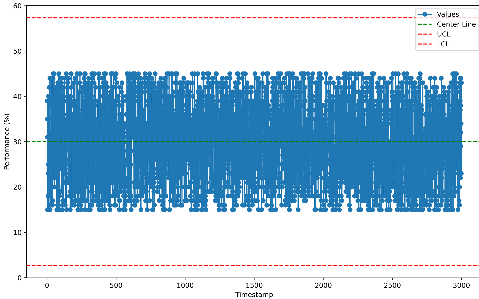
Individuals Chart for PFR10113 (2026-01-07)
