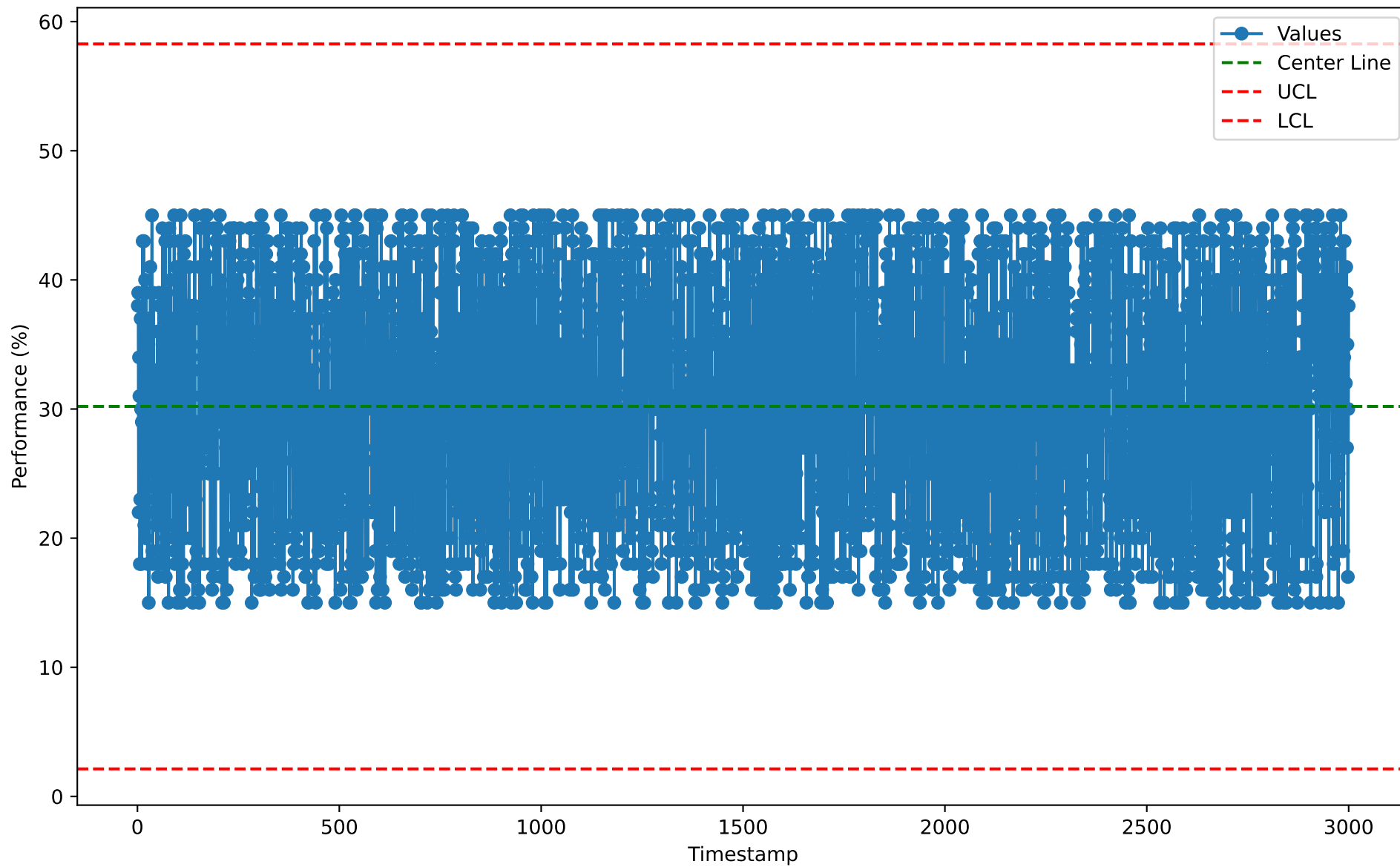
Individuals Chart for PFR10108 (2026-01-07)
