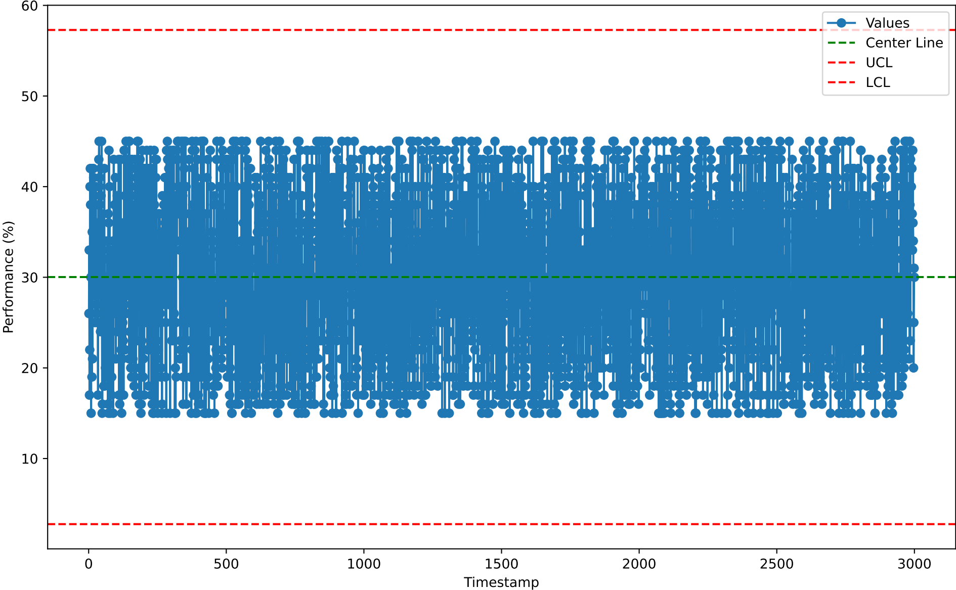
Individuals Chart for CLC10115 (2026-01-07)
