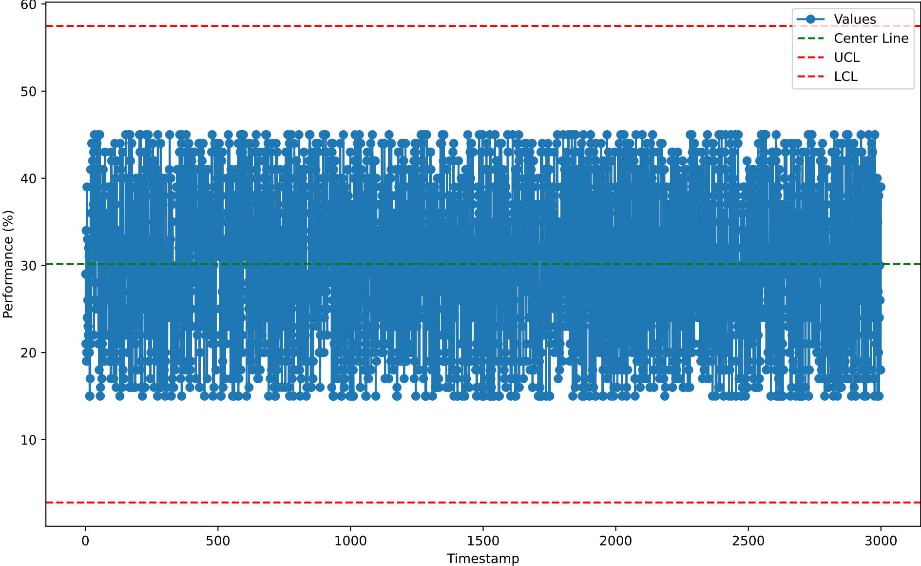
Individuals Chart for SCP10111 (2026-01-07)
