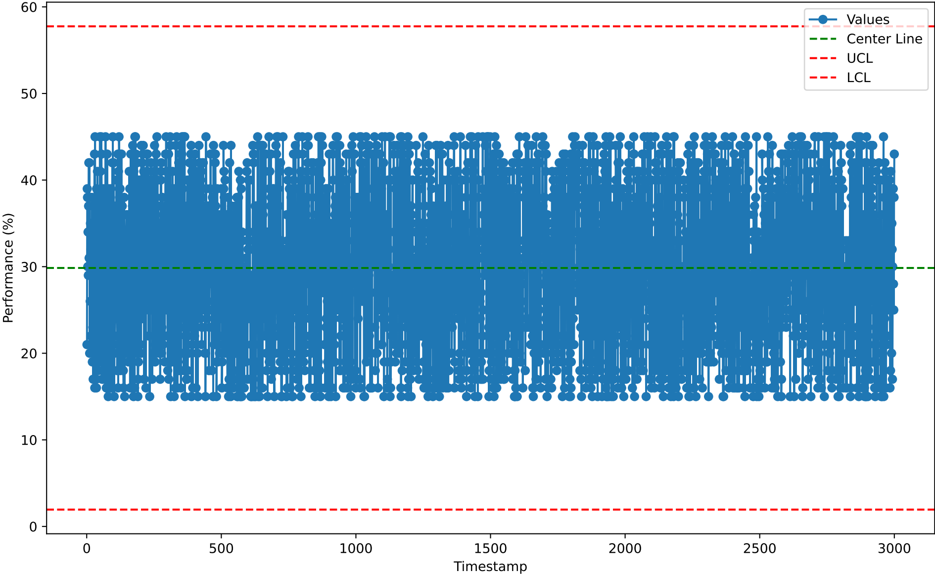
Individuals Chart for CLC10104 (2026-01-07)
