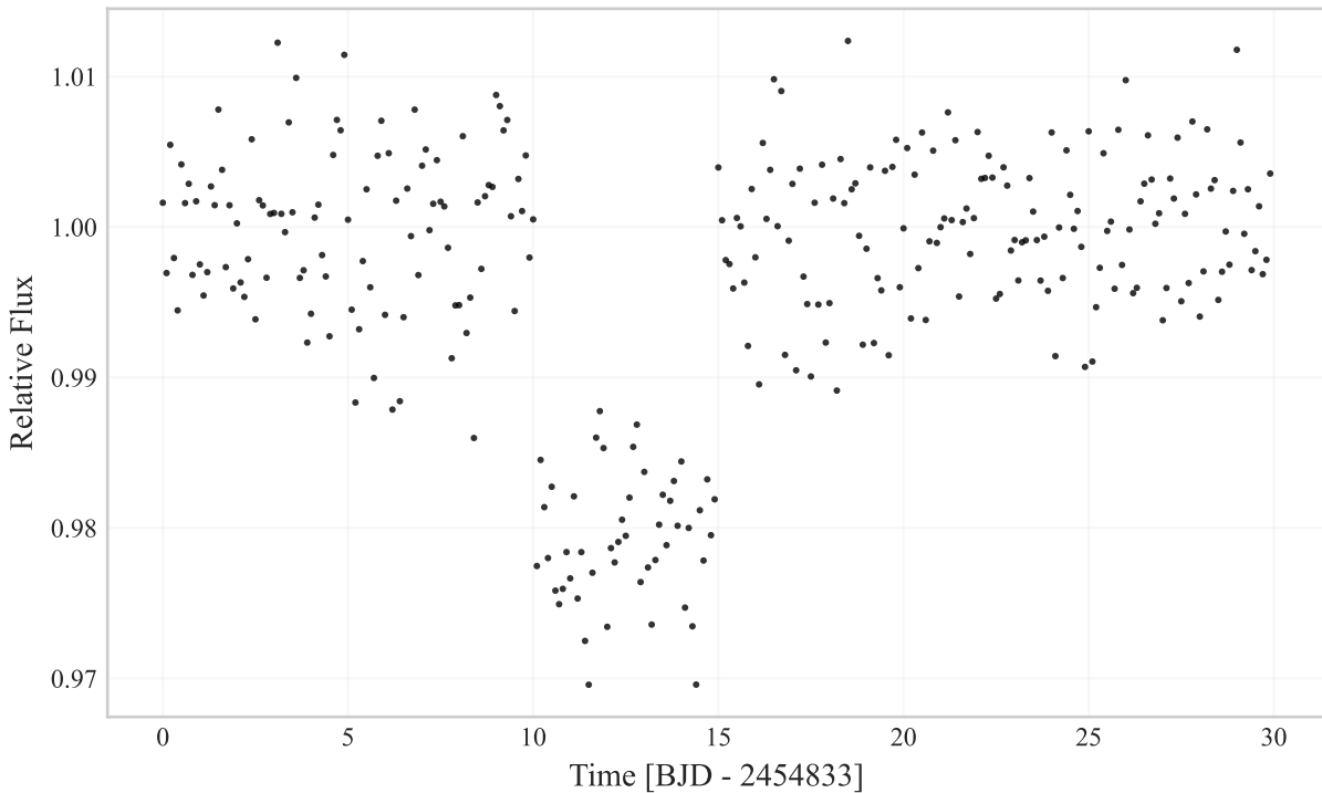
Exoplanet Transit Light Curve
