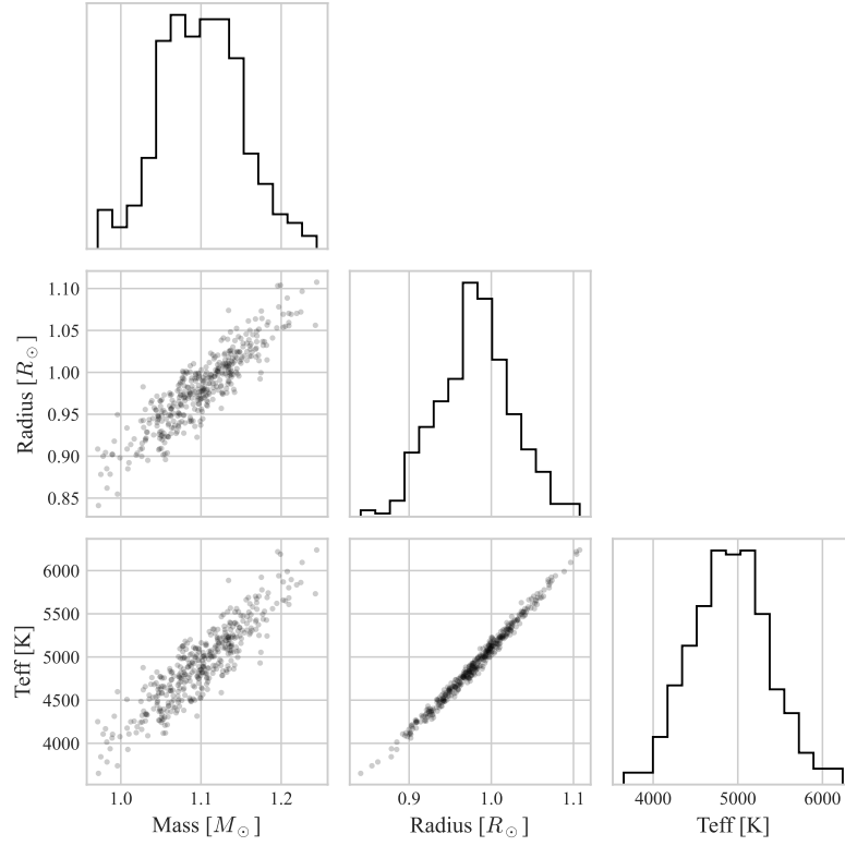
Figure 2: Posterior distributions for the optimal model parameters.
