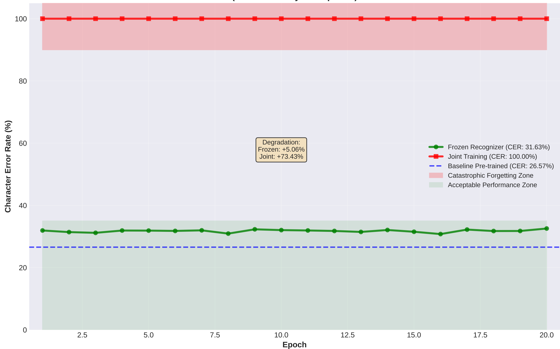
Frozen vs Joint Training: CER Comparison (Ablation Study - 20 Epochs)
