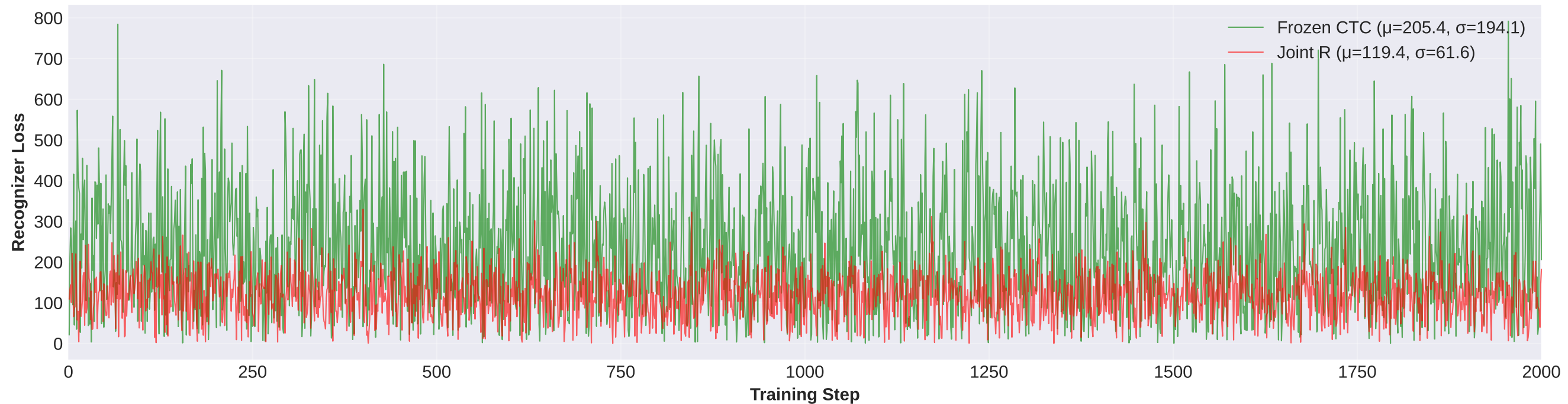
Recognizer/CTC Loss Trajectory (High variance in frozen due to curriculum learning, not instability)
