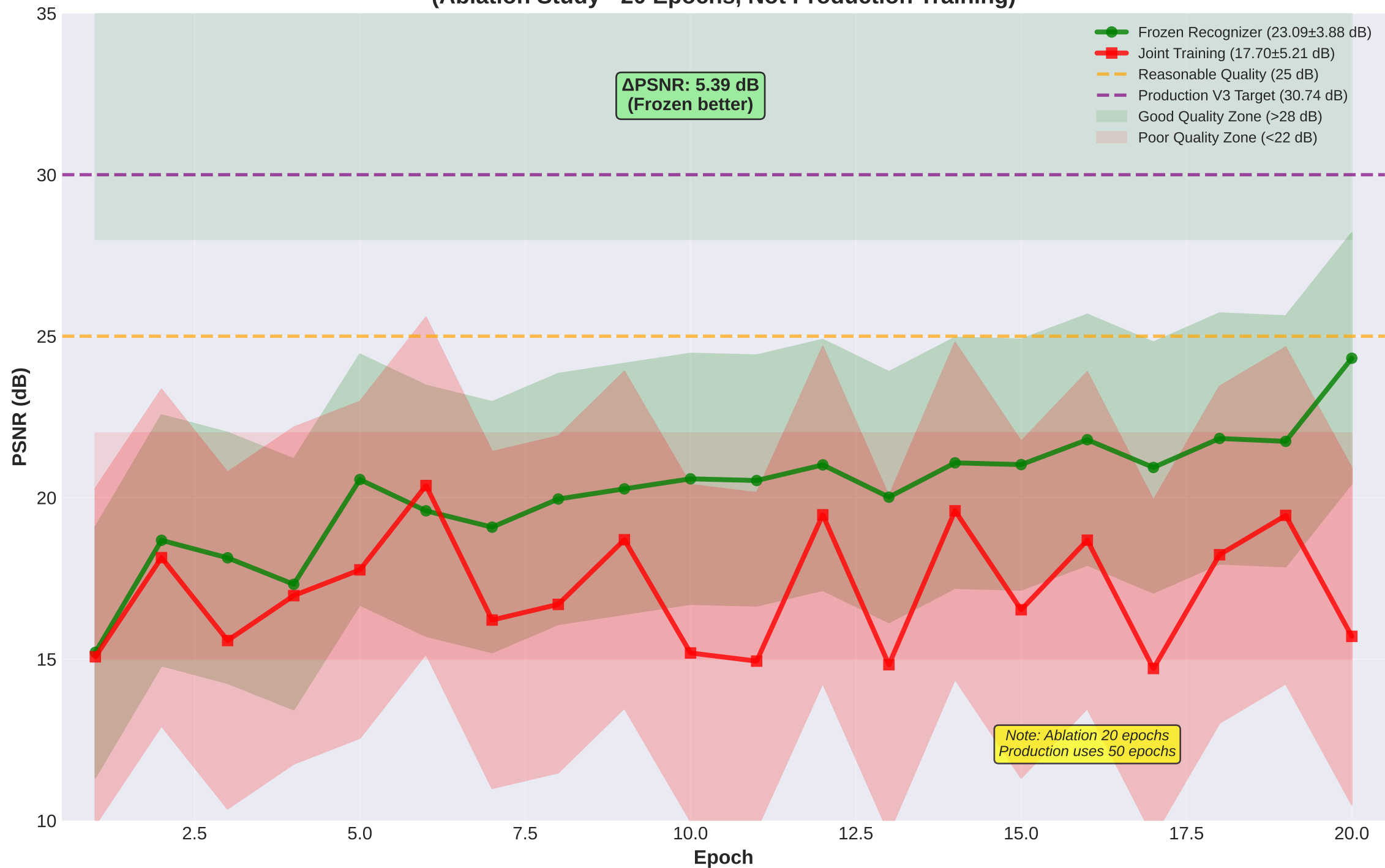
Frozen vs Joint Training: PSNR Comparison (Ablation Study - 20 Epochs, Not Production Training)
