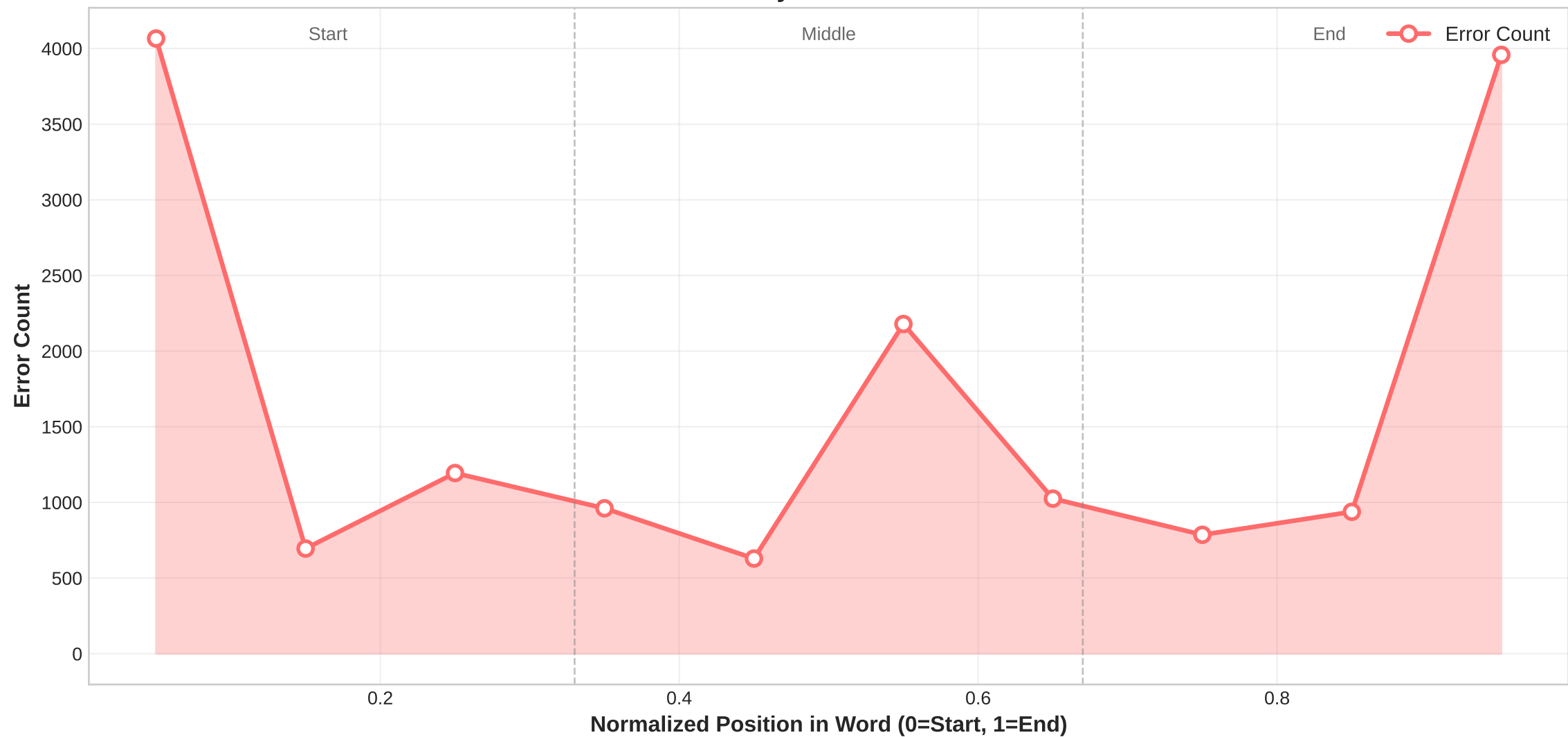
Error Distribution by Normalized Word Position
