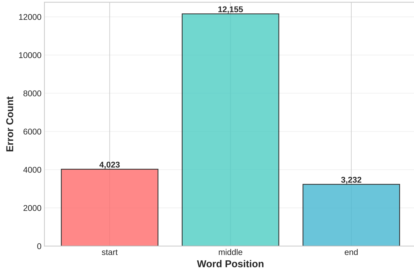
Error Distribution by Word Position (Absolute)
