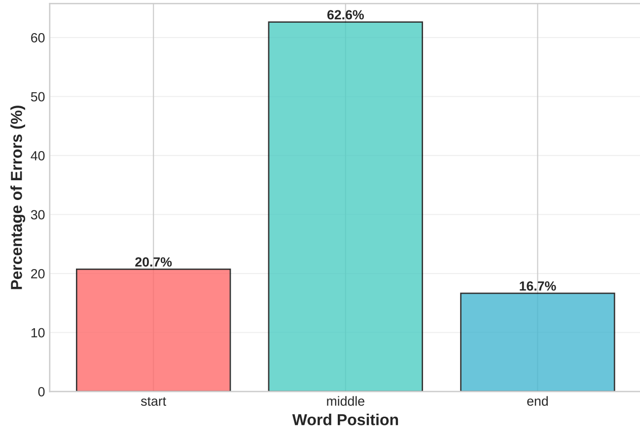
Error Distribution by Word Position (Relative)
