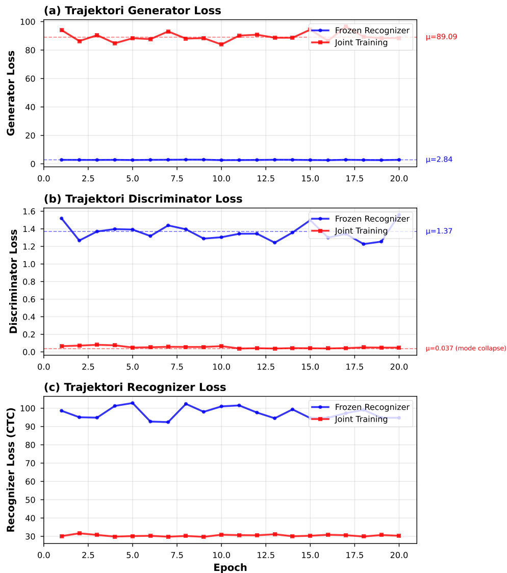
Gambar V.5 Trajektori loss selama 20 epoch. (a) Generator: fluktuasi frozen akibat curriculum learning vs osilasi ekstrem joint . (b) Discriminator: keseimbangan frozen vs mode collapse pada joint . (c) CTC: pembelajaran adaptif frozen vs ketidakstabilan joint .
