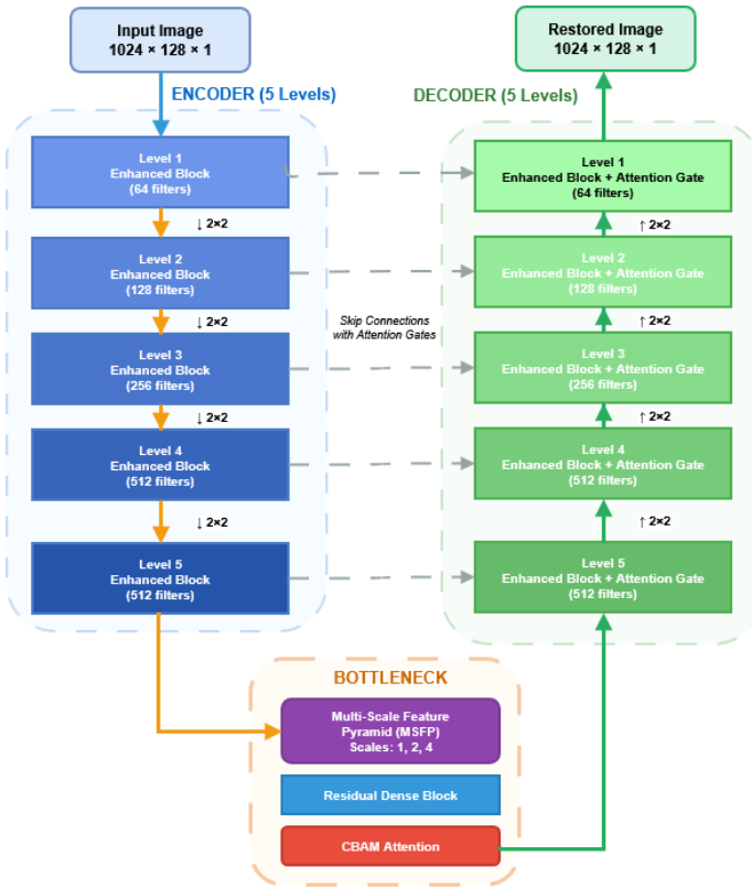
Fig. 3: Arsitektur Generator U-Net Enhanced: encoder 5-level (RDB+CBAM), bottleneck MSFP (512 kanal), decoder dengan attention gates. Skip connections mempertahankan detail spasial.
