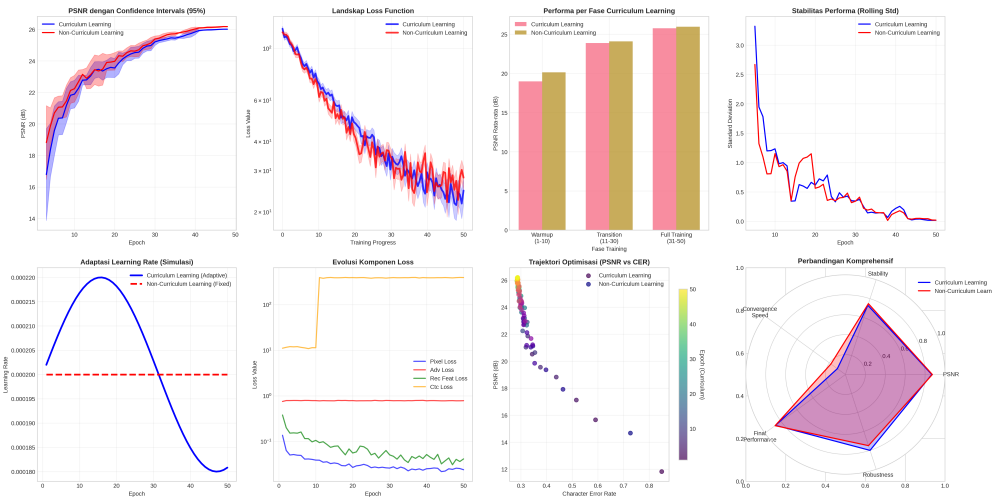
Gambar 9: Analisis scientific lanjutan: (a) PSNR dengan confidence intervals 95%, (b) loss landscape visualization, (c) performa per fase, (d) stabilitas performa, (e) learning rate adaptation, (f) evolusi komponen loss, (g) trajektori optimisasi PSNR vs CER, dan (h) radar chart perbandingan komprehensif.
