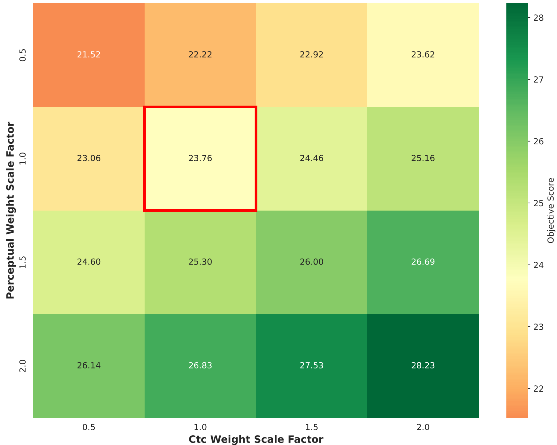
2D Grid Search: Ctc vs Perceptual
