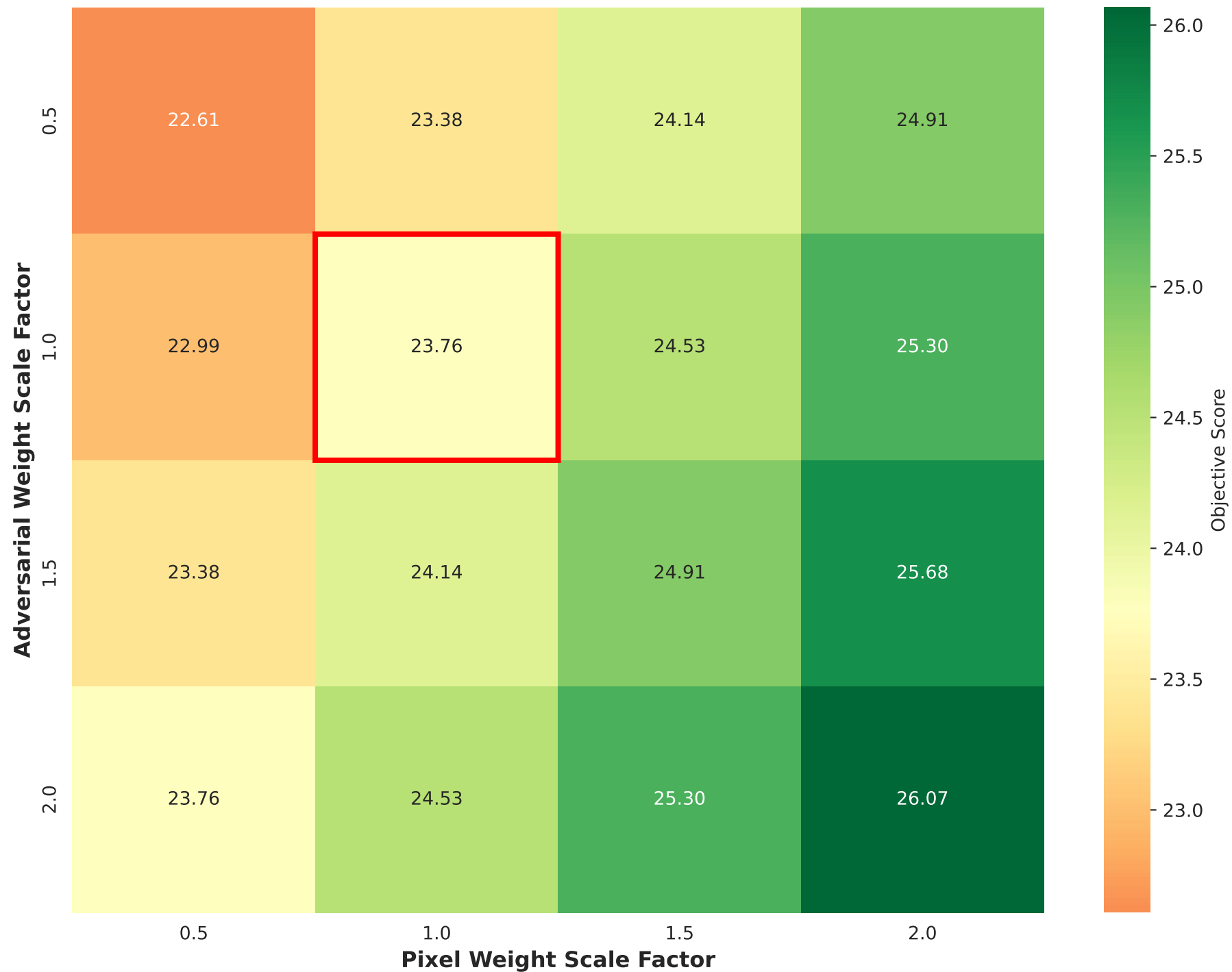
2D Grid Search: Pixel vs Adversarial
