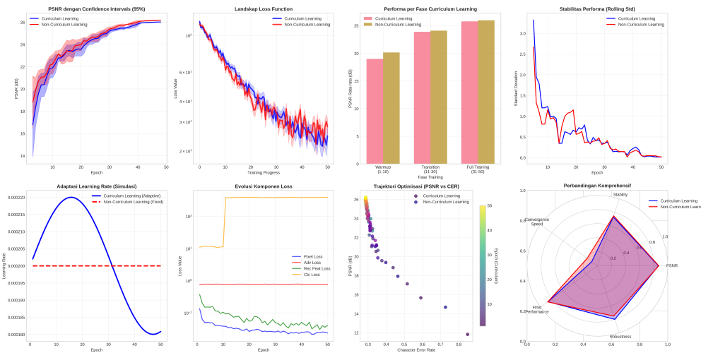
Gambar V.11 Analisis scientific lanjutan: (a) PSNR dengan confidence intervals 95%, (b) loss landscape visualization, (c) performa per fase, (d) stabilitas performa, (e) learning rate adaptation, (f) evolusi komponen loss, (g) trajektori optimisasi PSNR vs CER, dan (h) radar chart perbandingan.
