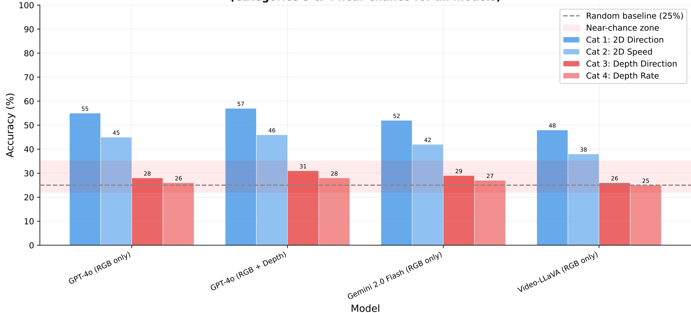
Motion-Blindness Benchmark: 2D Motion vs Depth-Axis Motion Accuracy (Categories 3 & 4 near chance for all models)
