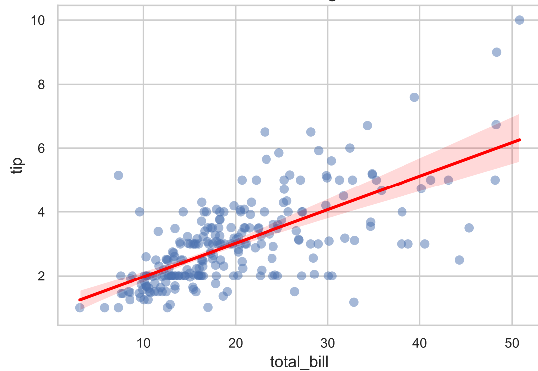
Scatter with Regression
