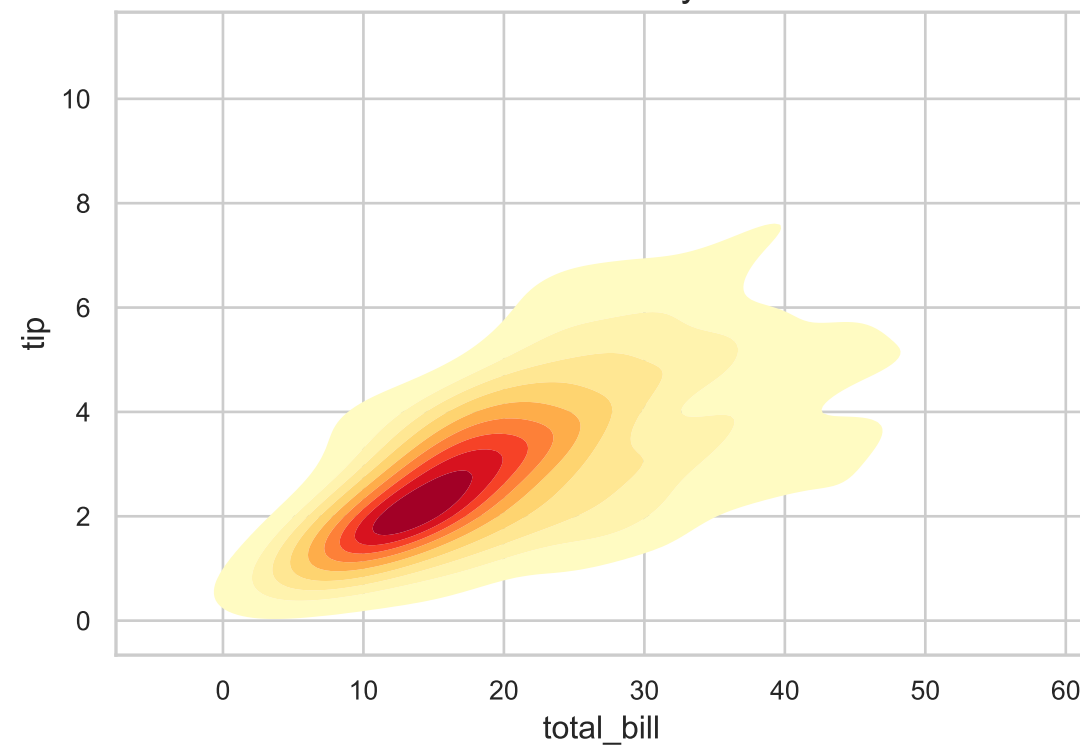
2D KDE Density Plot
