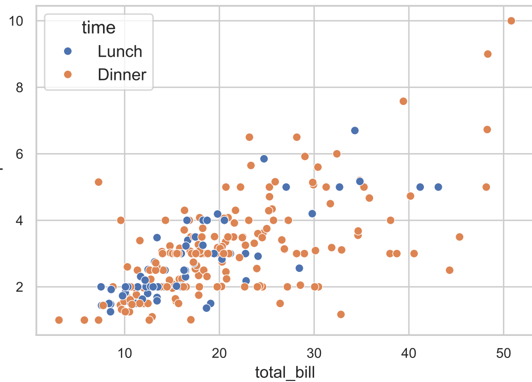
Basic Scatter Plot
