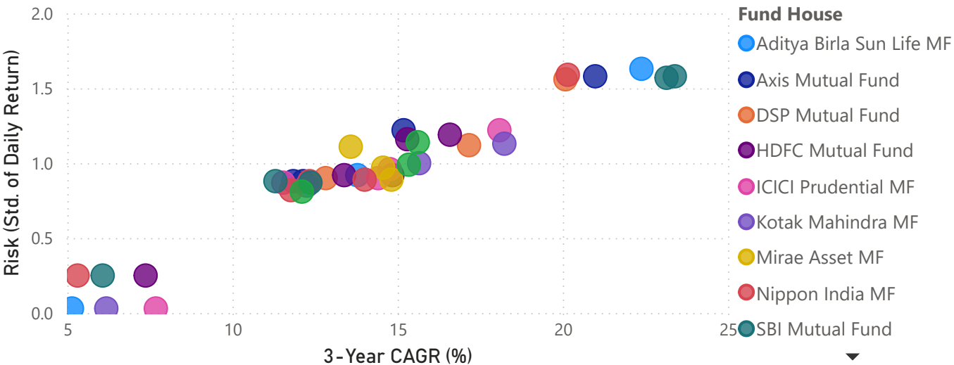
Score Board
